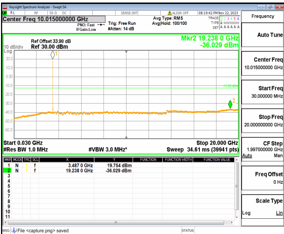
n77(3450-3550MHz) (30MHz-20GHz) 30M DFT-s-OFDM BPSK Edge 1RB Left Mid
