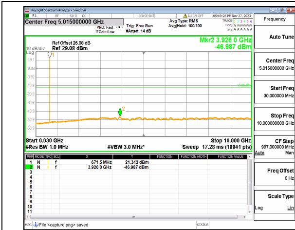
n71 (30MHz-10GHz) 20M DFT-s-OFDM BPSK Edge_1RB_Left_Mid
