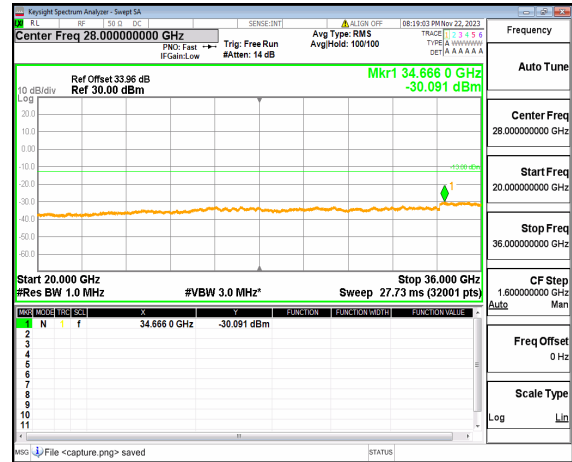
n77(3450-3550MHz) (20GHz-36GHz) 30M DFT-s-OFDM QPSK Edge 1RB Right Low
