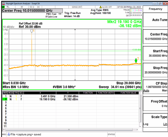
n77(3450-3550MHz) (30MHz-20GHz) 20M DFT-s-OFDM BPSK Edge 1RB Left Mid
