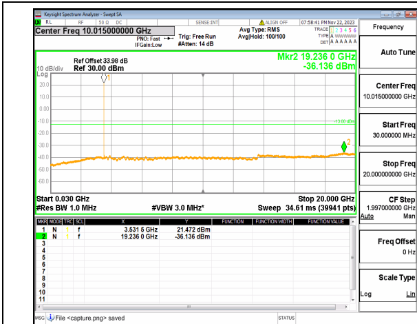
n77(3450-3550MHz) (30MHz-20GHz) 20M DFT-s-OFDM BPSK Edge_1RB_Left_High
