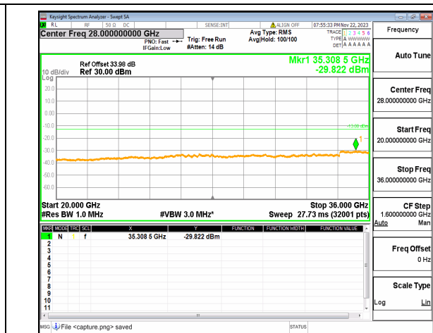
n77(3450-3550MHz) (20GHz-36GHz) 20M DFT-s-OFDM BPSK Edge_1RB_Right Mid
