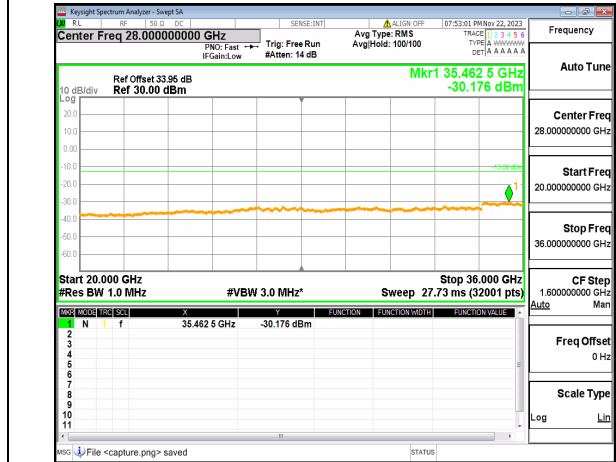
n77(3450-3550MHz) (20GHz-36GHz) 20M DFT-s-OFDM QPSK Edge 1RB Right Low
