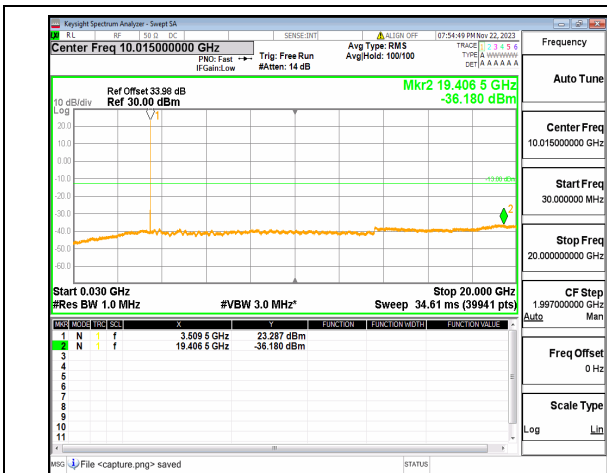
n77(3450-3550MHz) (30MHz-20GHz) 20M DFT-s-OFDM BPSK Edge_1RB_Right Mid
