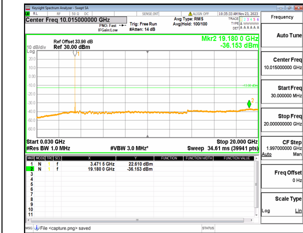
n77(3450-3550MHz) (30MHz-20GHz) 60M DFT-s-OFDM QPSK Edge_1RB_Left Mid
