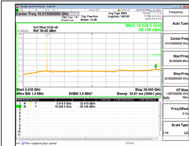
n77(3450-3550MHz) (30MHz-20GHz) 30M DFT-s-OFDM BPSK Edge_1RB_Right Mid
