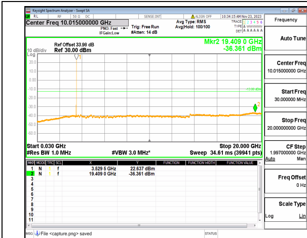
n77(3450-3550MHz) (30MHz-20GHz) 60M DFT-s-OFDM BPSK Edge_1RB_Right Mid
