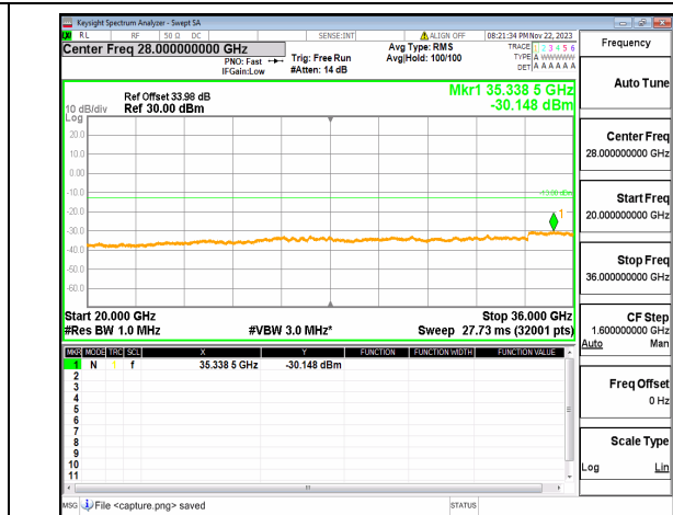
n77(3450-3550MHz) (20GHz-36GHz) 30M DFT-s-OFDM BPSK Edge_1RB_Right Mid
