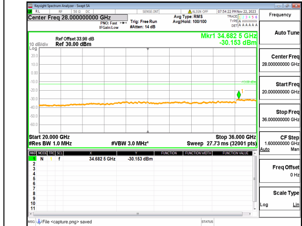
n77(3450-3550MHz) (20GHz-36GHz) 20M DFT-s-OFDM BPSK Edge 1RB Left Mid
