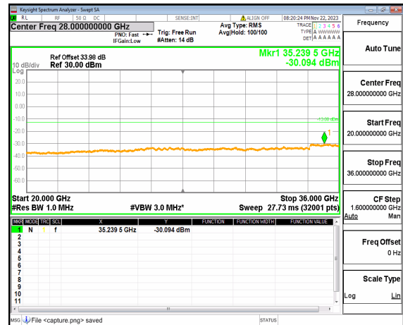
n77(3450-3550MHz) (20GHz-36GHz) 30M DFT-s-OFDM BPSK Edge 1RB Left Mid
