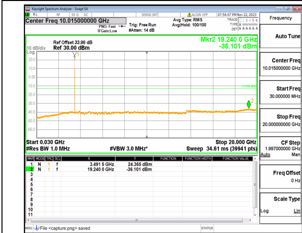
n77(3450-3550MHz) (30MHz-20GHz) 20M DFT-s-OFDM QPSK Edge_1RB_Left Mid
