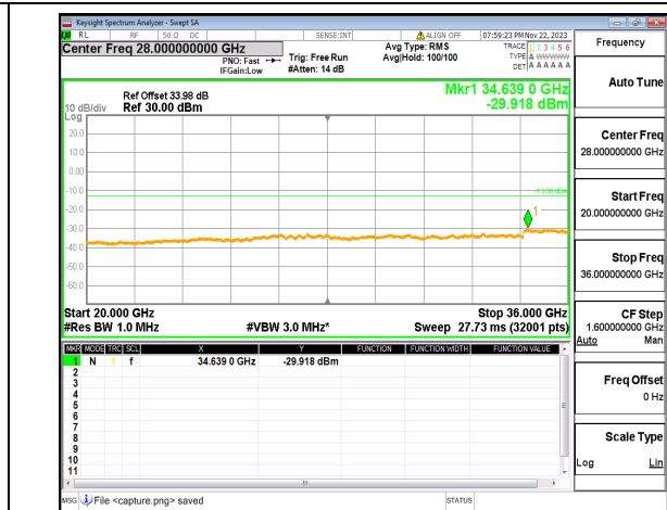
n77(3450-3550MHz) (20GHz-36GHz) 20M DFT-s-OFDM BPSK Edge_1RB_Left_High
