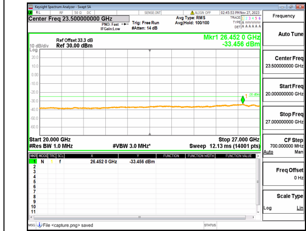
n41 (20GHz-27GHz) 60M DFT-s-OFDM QPSK Outer_Full Mid
