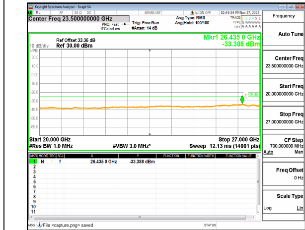
n41 (20GHz-27GHz) 60M DFT-s-OFDM BPSK Outer_Full High
