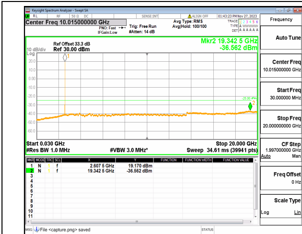
n41 (30MHz-20GHz) 30M DFT-s-OFDM QPSK Edge_1RB_Right Mid
