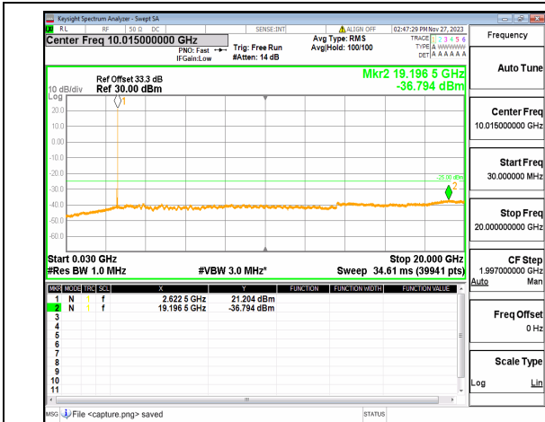
n41 (30MHz-20GHz) 60M DFT-s-OFDM QPSK Edge_1RB_Right Mid
