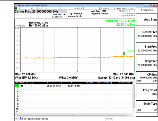
n41 (20GHz-27GHz) 60M DFT-s-OFDM QPSK Edge_1RB_Right Mid
