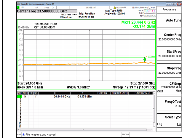
n38 (20GHz-27GHz) 30M DFT-s-OFDM BPSK Edge_1RB_Right_High
