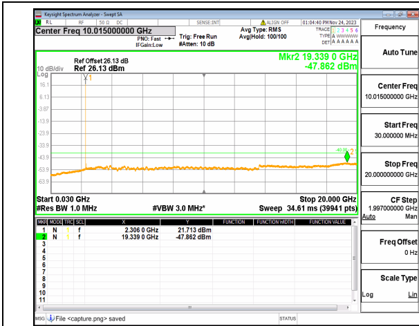
n30 (30MHz-20GHz) 10M DFT-s-OFDM BPSK Edge_1RB_Left Mid
