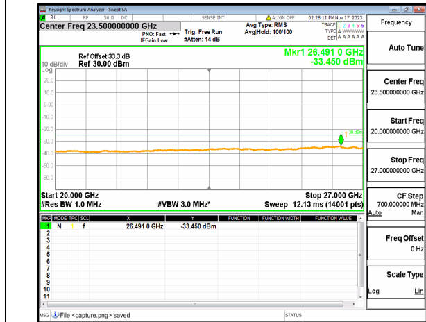
n38 (20GHz-27GHz) 30M DFT-s-OFDM BPSK Edge_1RB_Left_Low
