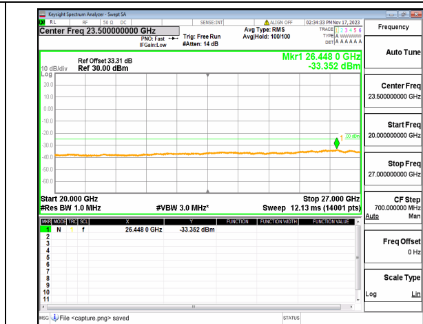
n38 (20GHz-27GHz) 30M DFT-s-OFDM BPSK Edge_1RB_Right Mid
