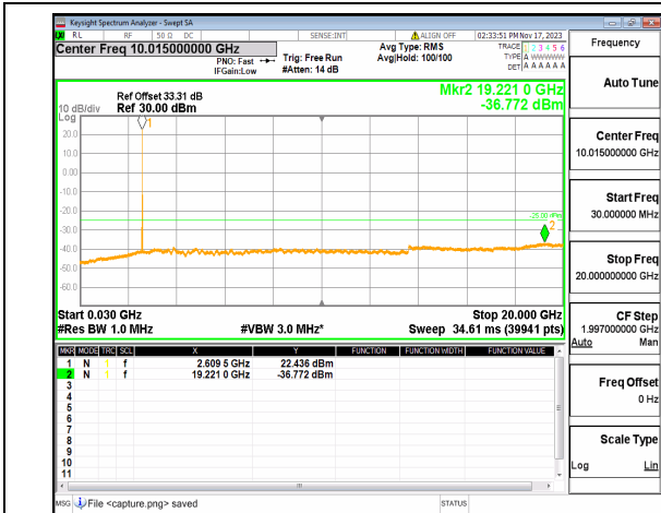
n38 (30MHz-20GHz) 30M DFT-s-OFDM BPSK Edge_1RB_Right Mid
