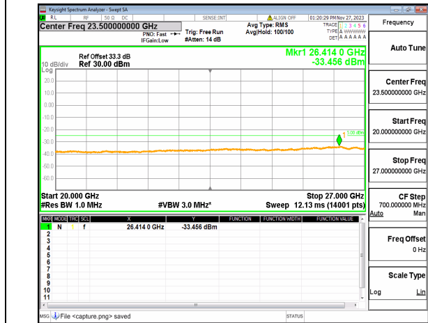
n41 (20GHz-27GHz) 20M DFT-s-OFDM QPSK Outer_Full Mid
