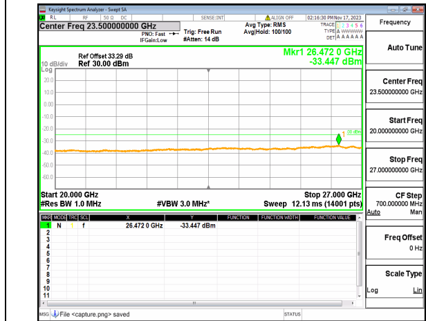
n38 (20GHz-27GHz) 20M DFT-s-OFDM QPSK Edge_1RB_Right_Low
