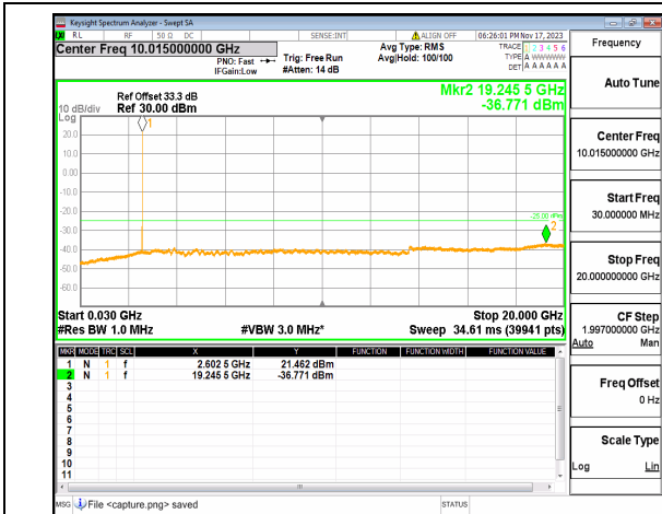
n41 (30MHz-20GHz) 20M DFT-s-OFDM BPSK Edge_1RB_Right Mid
