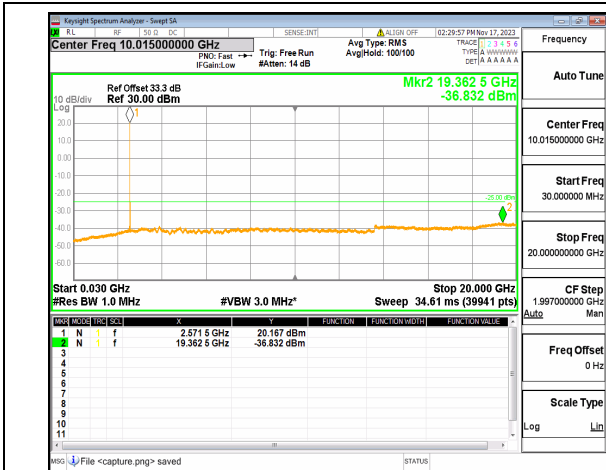
n38 (30MHz-20GHz) 30M DFT-s-OFDM QPSK Edge_1RB_Left Low
