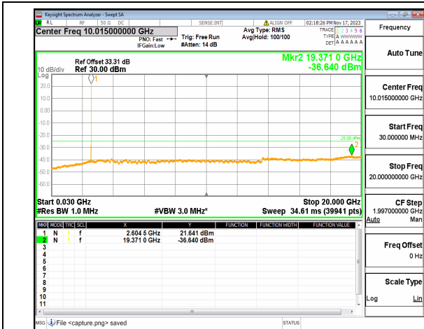
n38 (30MHz-20GHz) 20M DFT-s-OFDM BPSK Edge_1RB_Right Mid
