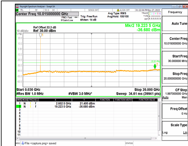
n41 (30MHz-20GHz) 20M DFT-s-OFDM QPSK Edge_1RB_Right Mid
