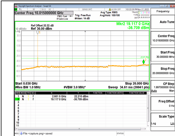
n38 (30MHz-20GHz) 20M DFT-s-OFDM BPSK Edge_1RB_Left_High
