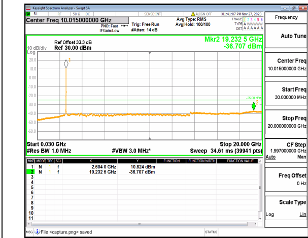
n41 (30MHz-20GHz) 30M DFT-s-OFDM QPSK Outer_Full Mid
