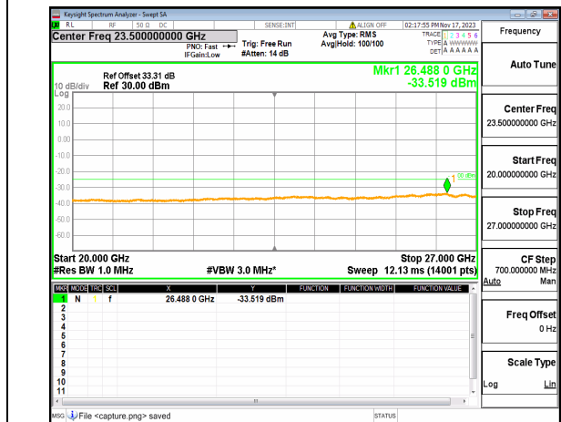
n38 (20GHz-27GHz) 20M DFT-s-OFDM BPSK Edge_1RB_Left_Mid
