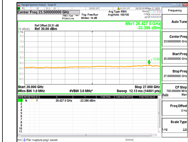
n38 (20GHz-27GHz) 30M DFT-s-OFDM BPSK Edge_1RB_Left Mid
