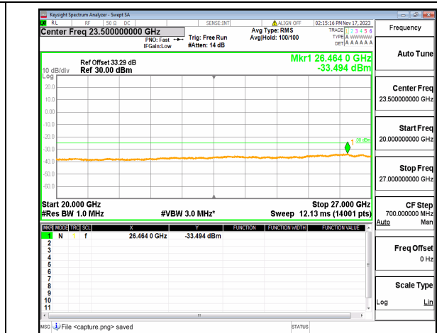
n38 (20GHz-27GHz) 20M DFT-s-OFDM QPSK Edge_1RB_Left_Low
