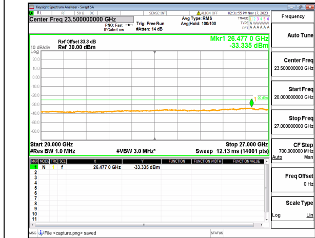
n38 (20GHz-27GHz) 30M DFT-s-OFDM QPSK Edge_1RB_Right Low
