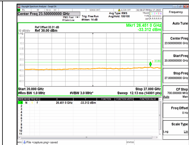
n38 (20GHz-27GHz) 30M DFT-s-OFDM BPSK Edge_1RB_Left_High
