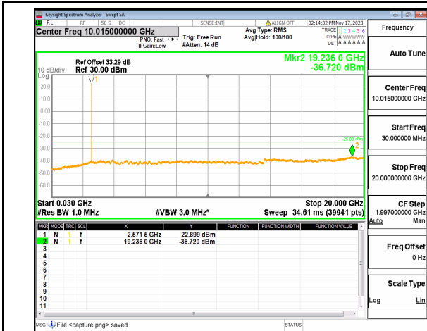
n38 (30MHz-20GHz) 20M DFT-s-OFDM QPSK Edge_1RB_Left_Low
