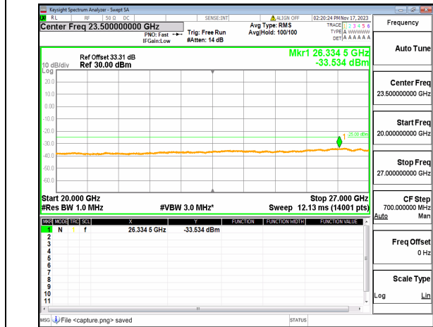
n38 (20GHz-27GHz) 20M DFT-s-OFDM QPSK Edge_1RB_Left Mid
