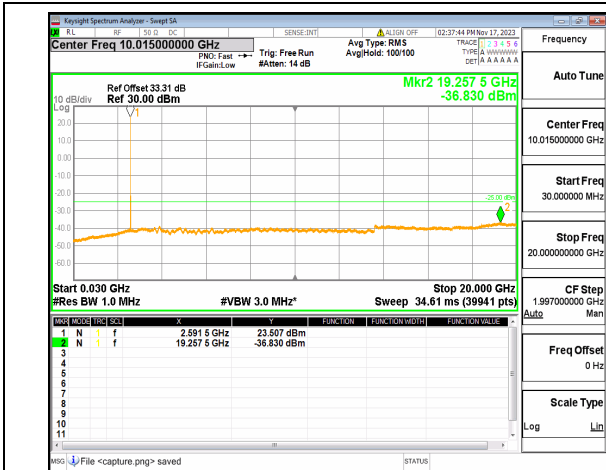
n38 (30MHz-20GHz) 30M DFT-s-OFDM BPSK Edge_1RB_Left_High
