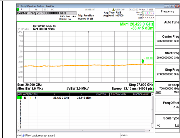
n38 (20GHz-27GHz) 20M DFT-s-OFDM BPSK Edge_1RB_Left_High
