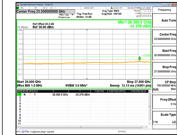
n41 (20GHz-27GHz) 30M DFT-s-OFDM QPSK Outer_Full Mid
