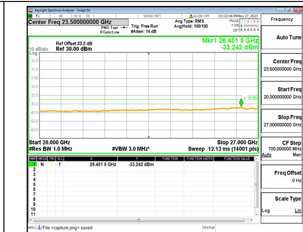
n41 (20GHz-27GHz) 20M DFT-s-OFDM QPSK Edge_1RB_Right Mid
