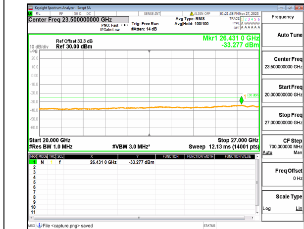
n41 (20GHz-27GHz) 20M DFT-s-OFDM QPSK Edge_1RB_Left Mid
