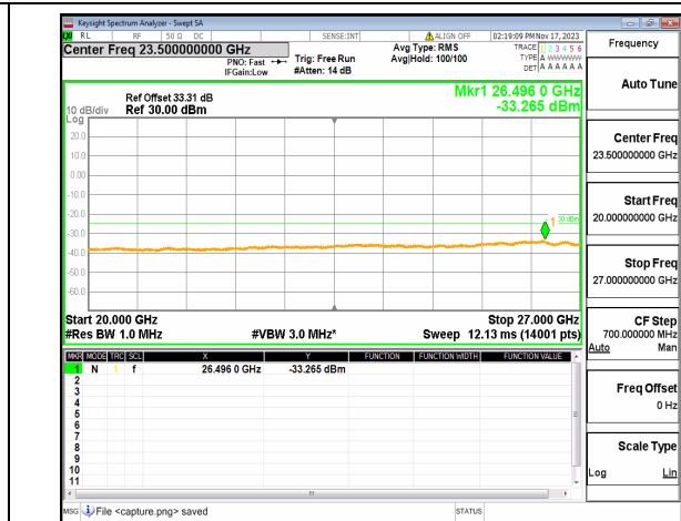
n38 (20GHz-27GHz) 20M DFT-s-OFDM BPSK Edge_1RB_Right Mid
