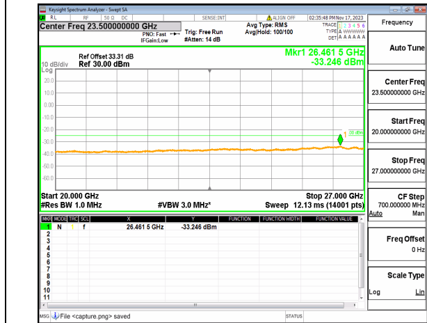
n38 (20GHz-27GHz) 30M DFT-s-OFDM QPSK Edge_1RB_Left Mid
