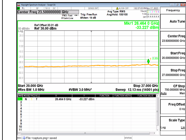
n38 (20GHz-27GHz) 30M DFT-s-OFDM QPSK Edge_1RB_Right Mid
