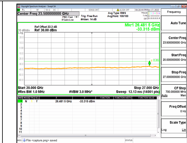
n41 (20GHz-27GHz) 20M DFT-s-OFDM BPSK Edge_1RB_Right Mid
