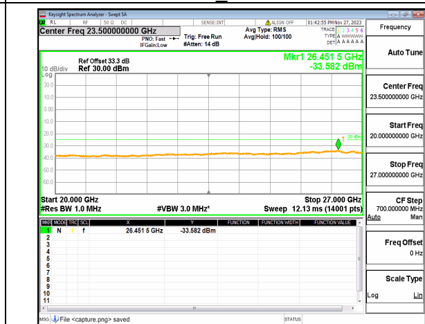
n41 (20GHz-27GHz) 30M DFT-s-OFDM QPSK Edge_1RB_Left Mid
