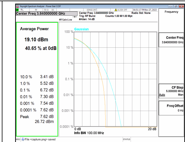
n77(3700-3980MHz) 100M CP-OFDM 256QAM Outer_Full Mid
