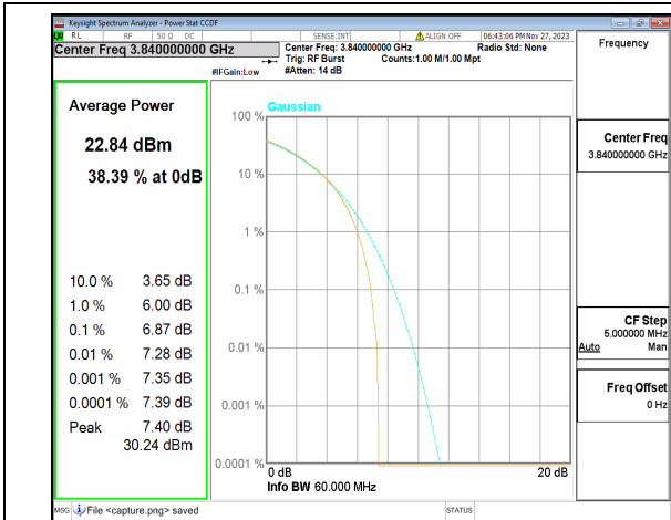
n77(3700-3980MHz) 60M CP-OFDM QPSK Outer_Full Mid
