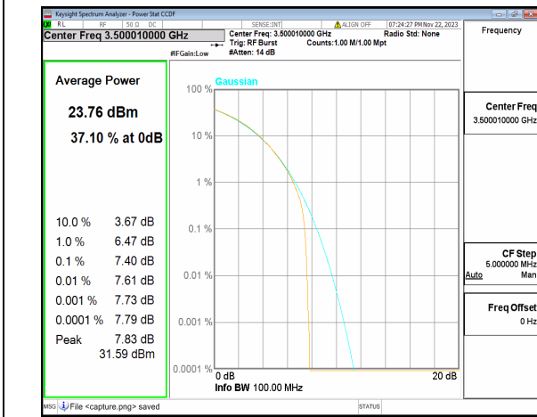
n77(3450-3550MHz) 100M CP-OFDM QPSK Outer_Full Mid
