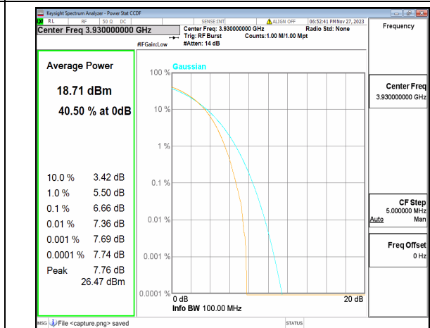
n77(3700-3980MHz) 100M CP-OFDM 256QAM Outer_Full High
