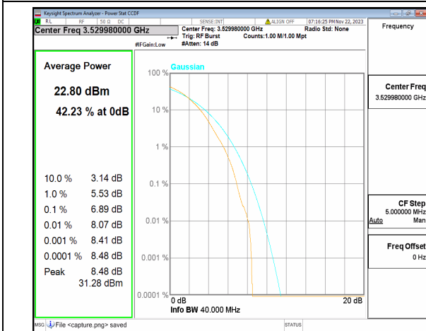
n77(3450-3550MHz) 40M CP-OFDM QPSK Outer_Full High
