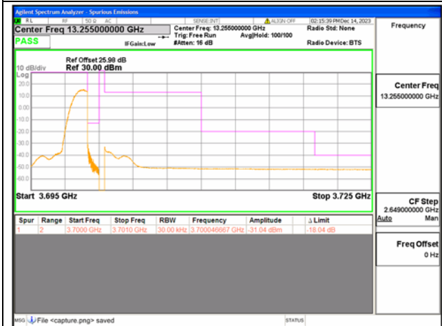
B43(3600-3700) / 5MHz / High CH / QPSK / 1 RB
