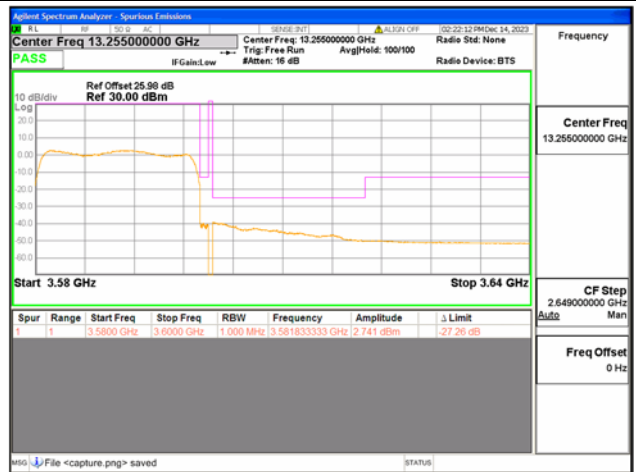
B42(3550-3600) / 20MHz / High CH / QPSK / FULL RB
