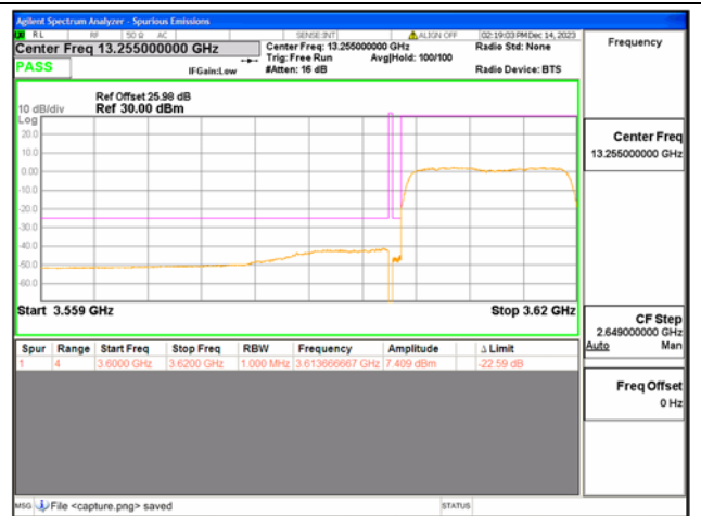
B43(3600-3700) / 20MHz / Low CH / QPSK / FULL RB
