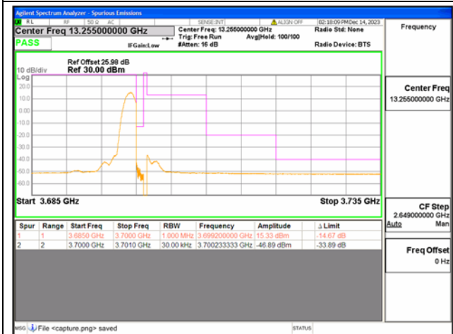
B43(3600-3700) / 15MHz / High CH / QPSK / 1 RB
