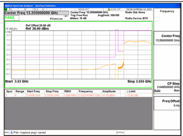
B42(3550-3600) / 5MHz / Low CH / QPSK / FULL RB
