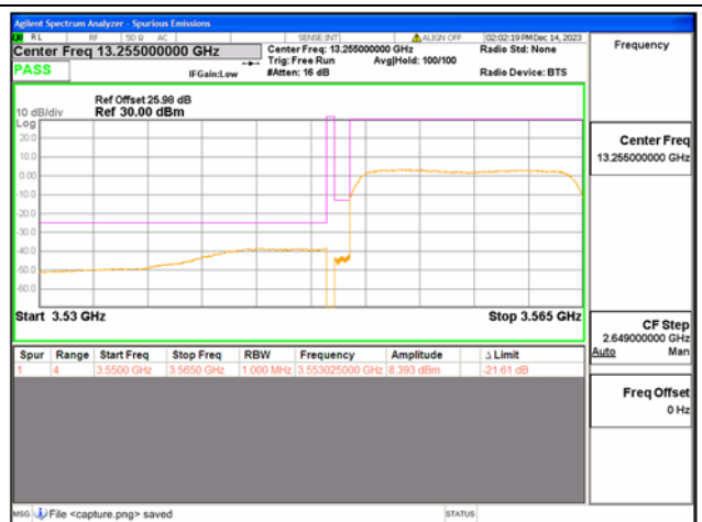
B42(3550-3600) / 15MHz / Low CH / QPSK / FULL RB
