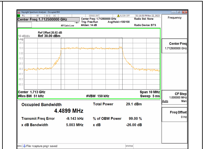
n66 5M DFT-s-OFDM QPSK Outer_Full Low
