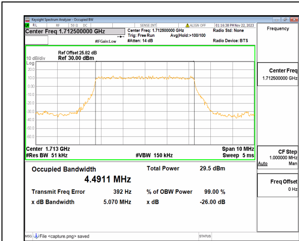
n66 5M DFT-s-OFDM BPSK Outer_Full Low
