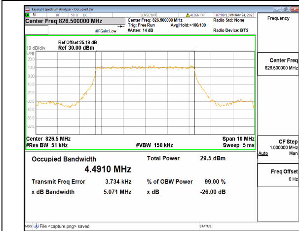
n26(824-849MHz) 5M DFT-s-OFDM BPSK Outer_Full Low
