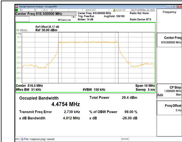
n26(814-824MHz) 5M DFT-s-OFDM BPSK Outer_Full Low
