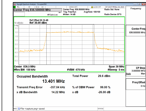
n26(824-849MHz) 15M DFT-s-OFDM QPSK Outer_Full Mid
