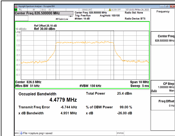
n26(824-849MHz) 5M DFT-s-OFDM 256QAM Outer_Full Low
