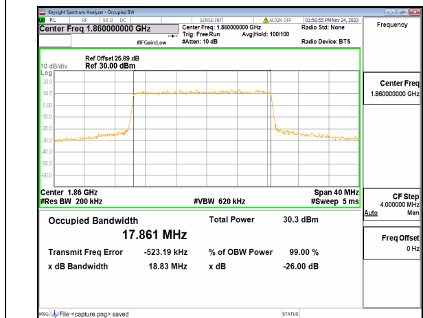
n25 20M DFT-s-OFDM QPSK Outer_Full Low
