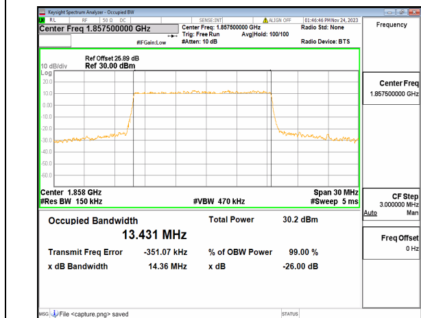
n25 15M DFT-s-OFDM QPSK Outer_Full Low
