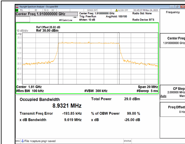
n25 10M DFT-s-OFDM 16QAM Outer_Full High
