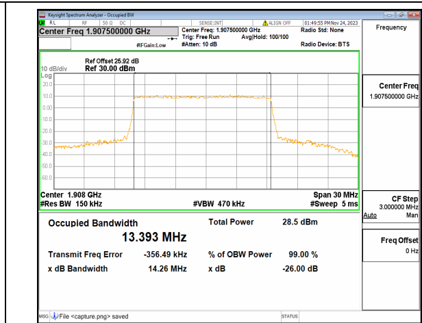
n25 15M DFT-s-OFDM 64QAM Outer_Full High
