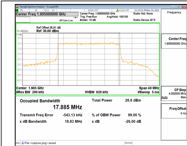
n25 20M DFT-s-OFDM 16QAM Outer_Full High
