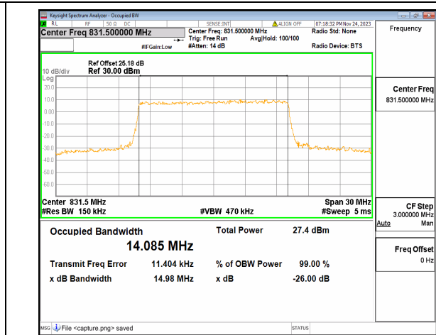
n26(824-849MHz) 15M CP-OFDM QPSK Outer_Full Low
