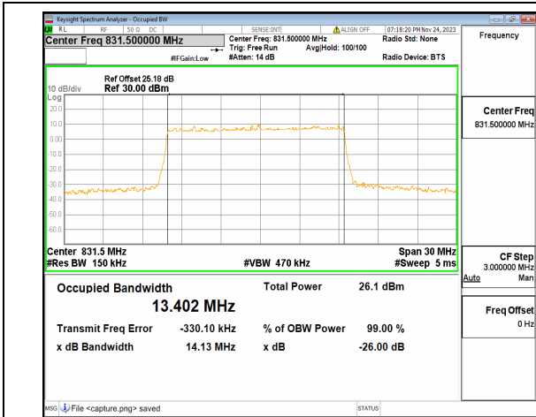
n26(824-849MHz) 15M DFT-s-OFDM 256QAM Outer_Full Low
