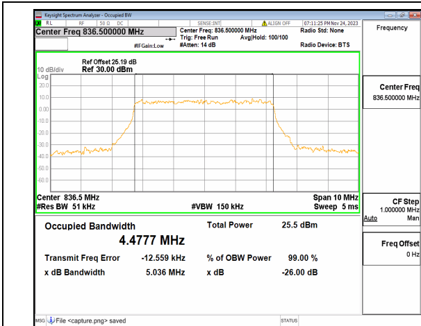
n26(824-849MHz) 5M DFT-s-OFDM 256QAM Outer_Full Mid
