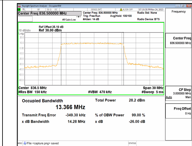
n26(824-849MHz) 15M DFT-s-OFDM 64QAM Outer_Full Mid
