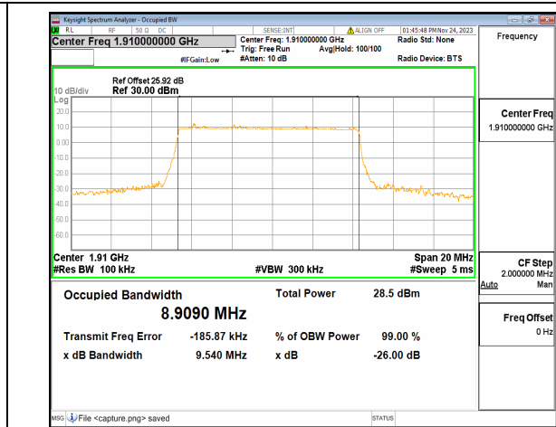
n25 10M DFT-s-OFDM 64QAM Outer_Full High
