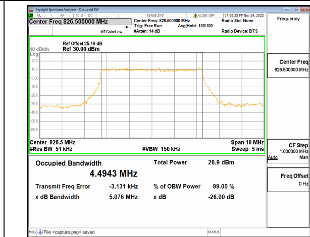
n26(824-849MHz) 5M DFT-s-OFDM QPSK Outer_Full Low
