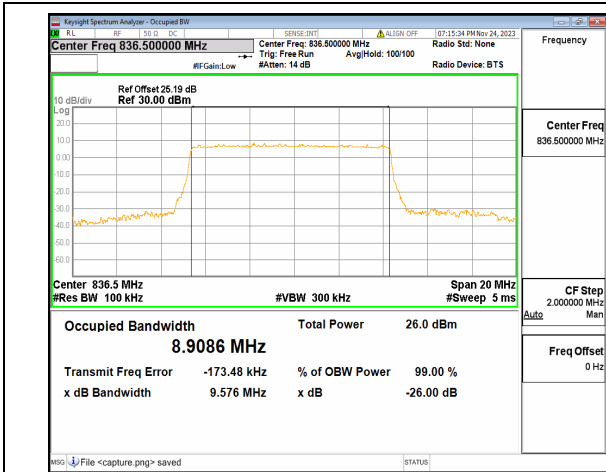
n26(824-849MHz) 10M DFT-s-OFDM 256QAM Outer_Full Mid
