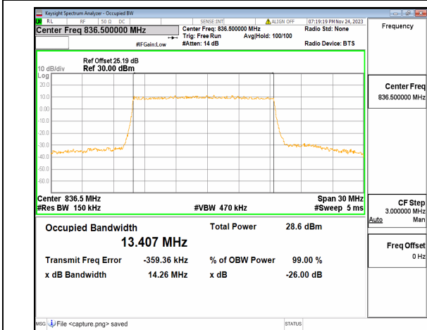
n26(824-849MHz) 15M DFT-s-OFDM 16QAM Outer_Full Mid
