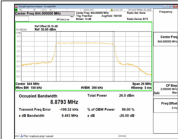
n26(824-849MHz) 10M DFT-s-OFDM 256QAM Outer_Full High
