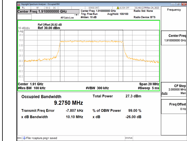
n25 10M CP-OFDM QPSK Outer_Full High
