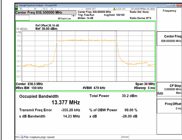
n26(824-849MHz) 15M DFT-s-OFDM BPSK Outer_Full Mid
