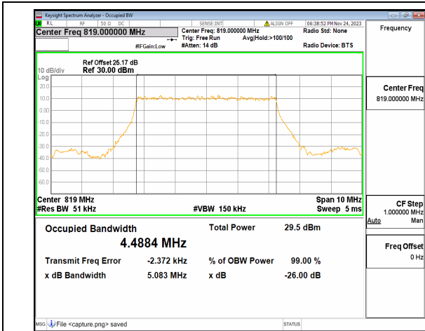
n26(814-824MHz) 5M DFT-s-OFDM BPSK Outer_Full Mid
