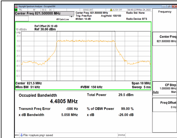
n26(814-824MHz) 5M DFT-s-OFDM BPSK Outer_Full High
