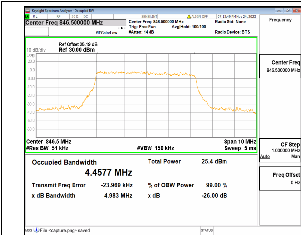
n26(824-849MHz) 5M DFT-s-OFDM 256QAM Outer_Full High
