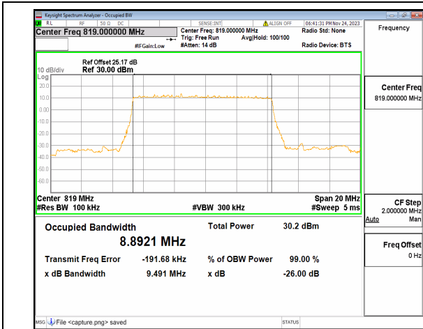
n26(814-824MHz) 10M DFT-s-OFDM BPSK Outer_Full Mid
