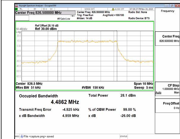
n26(824-849MHz) 5M DFT-s-OFDM 16QAM Outer_Full Low
