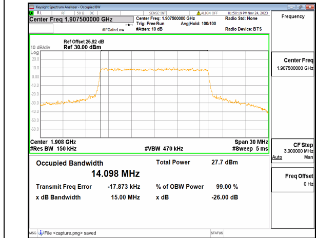
n25 15M CP-OFDM QPSK Outer_Full High
