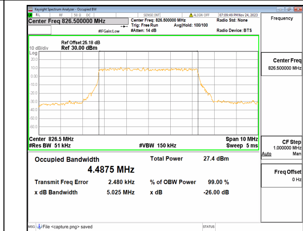
n26(824-849MHz) 5M DFT-s-OFDM 64QAM Outer_Full Low
