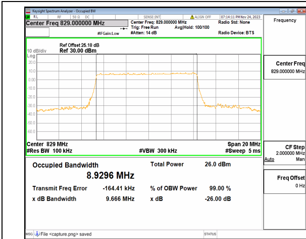
n26(824-849MHz) 10M DFT-s-OFDM 256QAM Outer_Full Low
