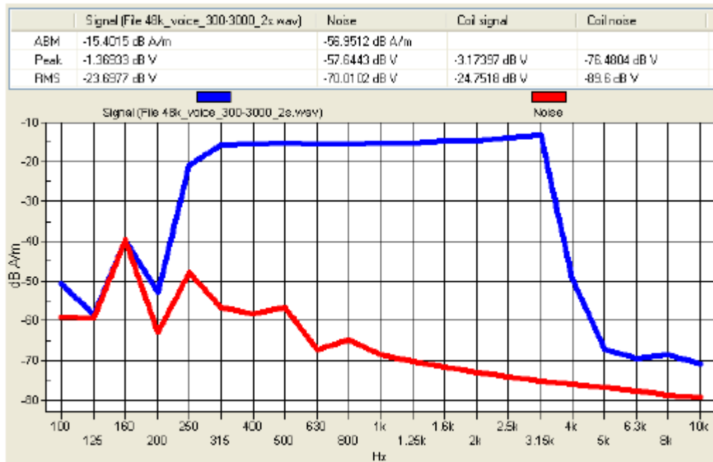
Figure 8: Audio Signal Spectrum of the Broadband Signal
