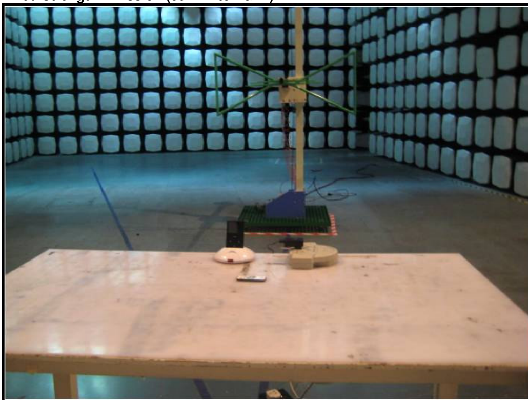
Flied Strength Emission (30MHz to 1GHz)
