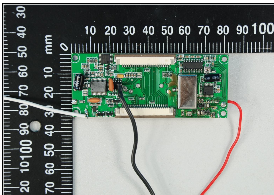
RF portion and Antenna(red copper wire)
