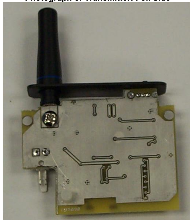
Photograph of Transmitter: Foil Side
