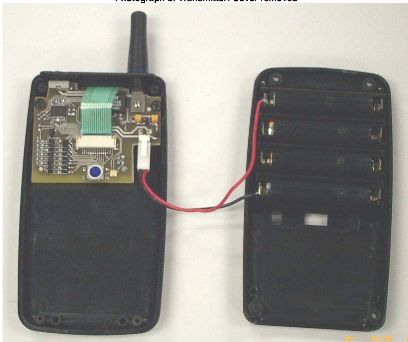
Photograph of Transmitter: Cover removed
