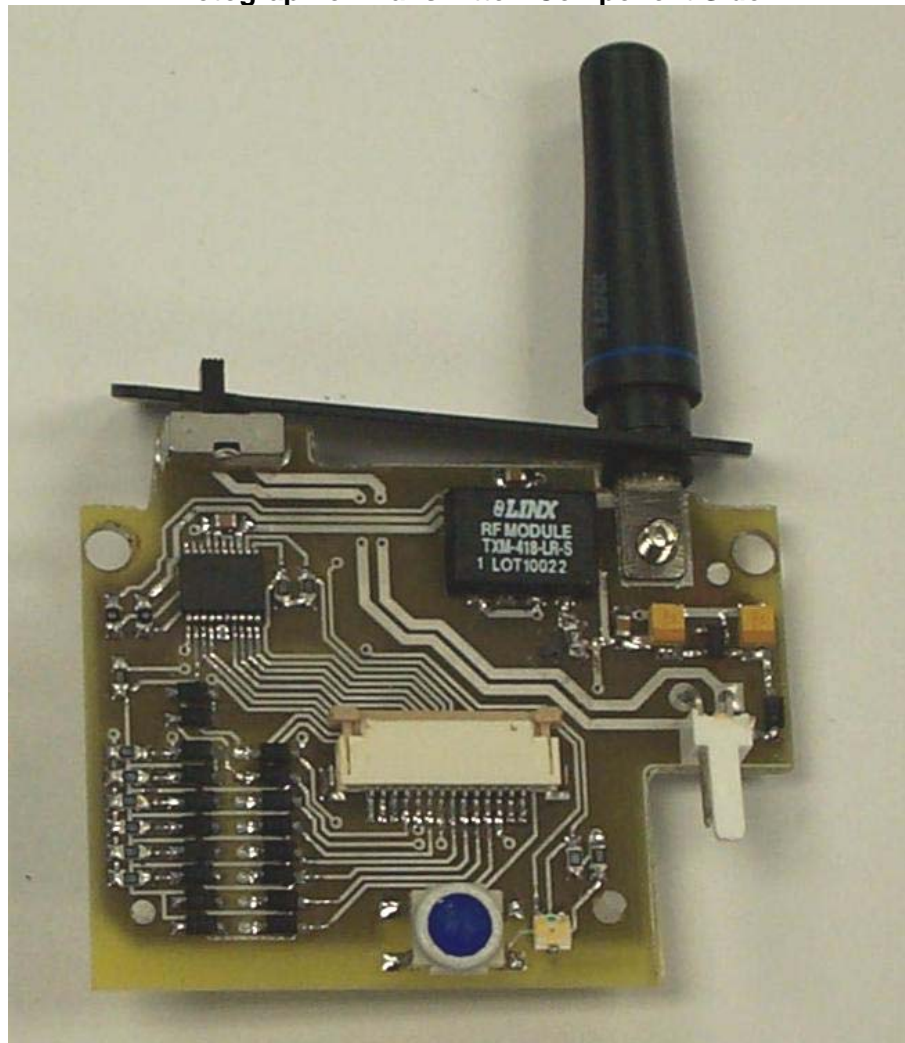
Photograph of Transmitter: Foil Side
