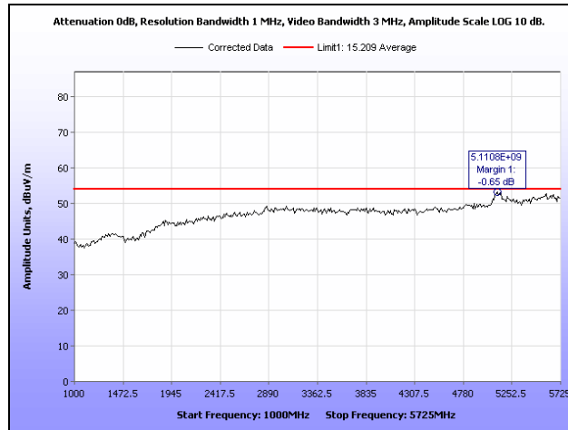
Plot 31. Radiated Spurious Emissions, High Channel, 1 GHz – 5.725 GHz, Average Detector, HT20
