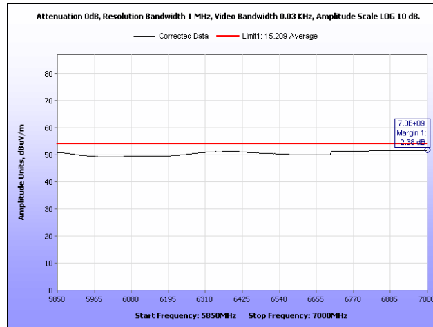
Plot 19. Radiated Spurious Emissions, Low Channel, 5.850 GHz – 7 GHz, Average, HT20
