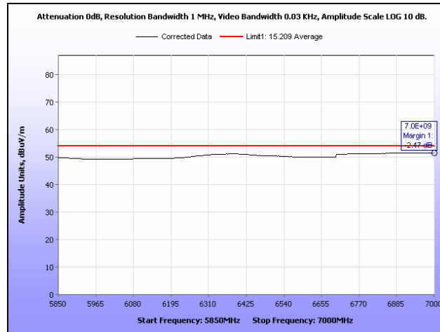
Plot 40. Radiated Spurious Emissions, Low Channel, 5.850 GHz – 7 GHz, Average, HT40
