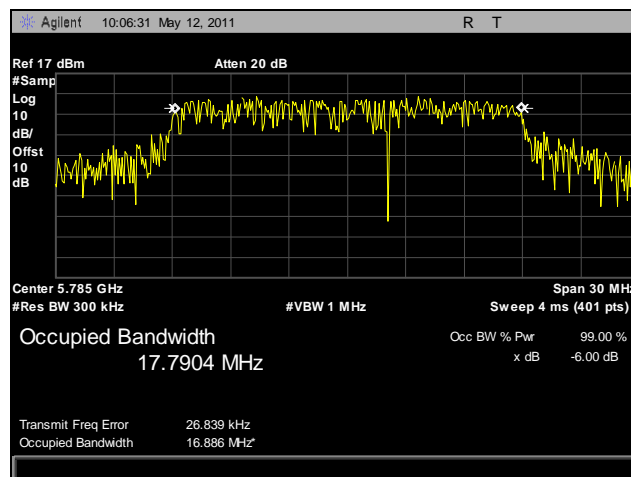
Plot 7. 99% Occupied Bandwidth, Mid Channel, HT20
