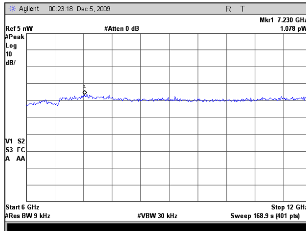
Plot 80. Receiver Spurious Emission, 6 GHz – 12 GHz, HT20
