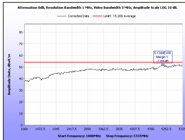
Plot 45. Radiated Spurious Emissions, High Channel, 1 GHz – 5.725 GHz, Average Detector, HT40
