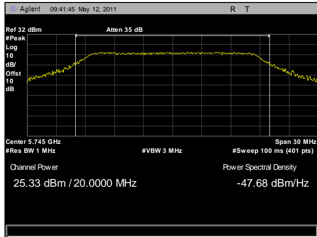
Plot 11. Peak Power Output, Low Channel, HT20
