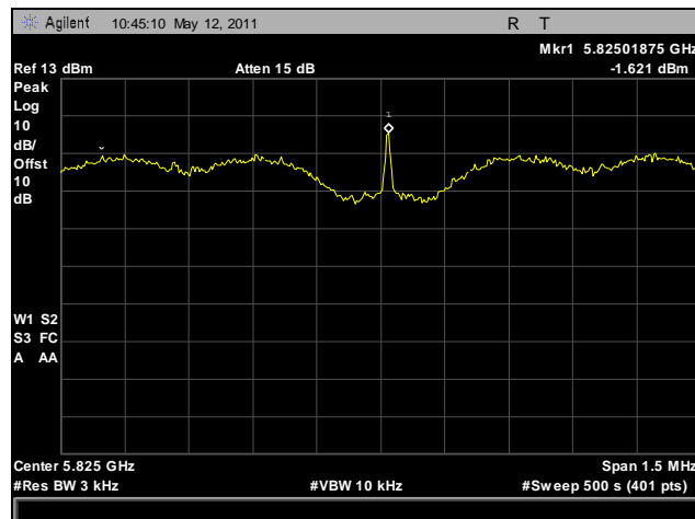
Plot 75. Peak Power Spectral Density, High Channel, HT20
