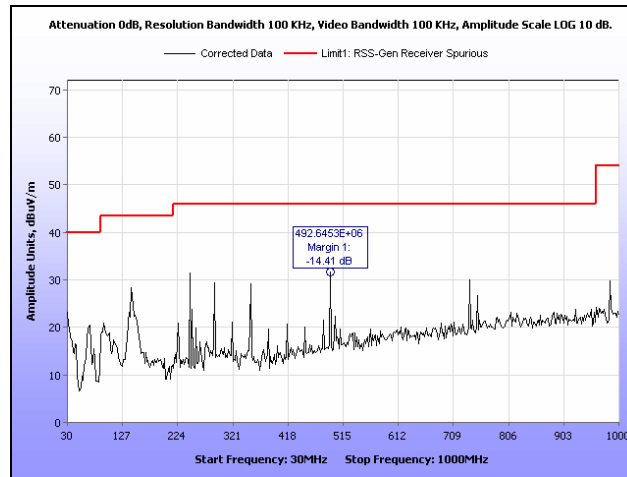
Plot 82. Receiver Spurious Emission, 30 MHz – 1 GHz, HT40
