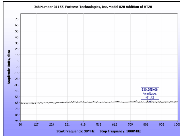
Plot 54. Conducted Spurious Emissions, Mid Channel, 30 MHz – 1 GHz, HT20
