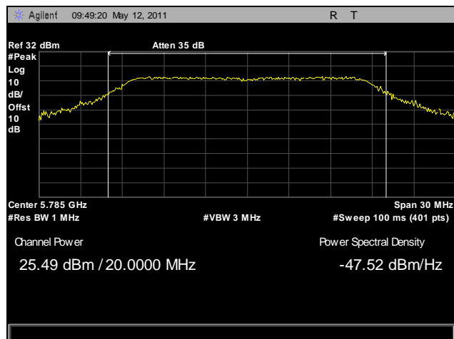
Plot 12. Peak Power Output, Mid Channel, HT20
