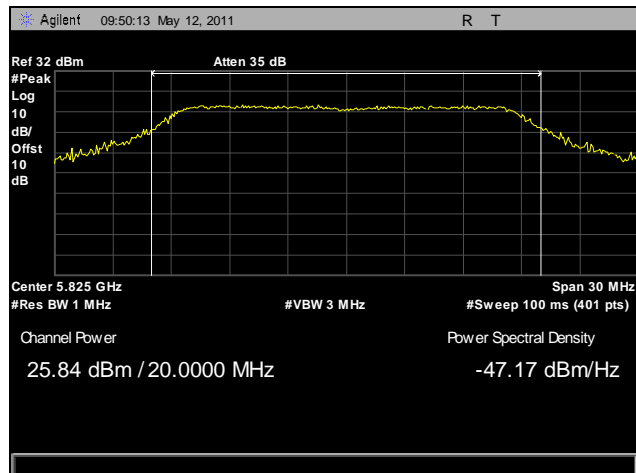
Plot 13. Peak Power Output, High Channel, HT20
