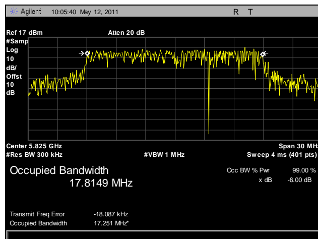
Plot 8. 99% Occupied Bandwidth, High Channel, HT20
