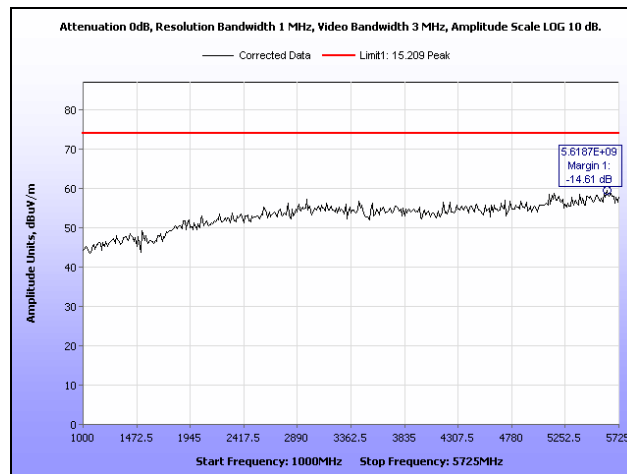
Plot 18. Radiated Spurious Emissions, Low Channel, 1 GHz – 5.725 GHz, Peak, HT20
