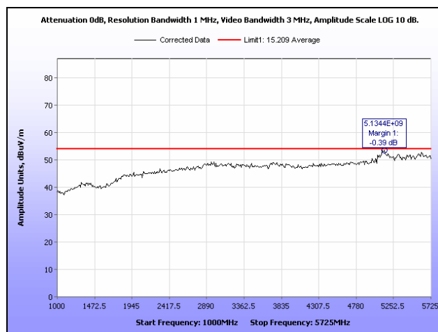
Plot 24. Radiated Spurious Emissions, Mid Channel, 1 GHz – 5.725 GHz, Average Detector, HT20
