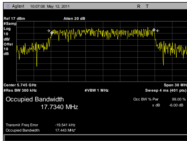
Plot 6. 99% Occupied Bandwidth, Low Channel, HT20
