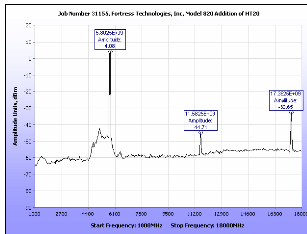
Plot 55. Conducted Spurious Emissions, Mid Channel, 1 GHz – 18 GHz, HT20
