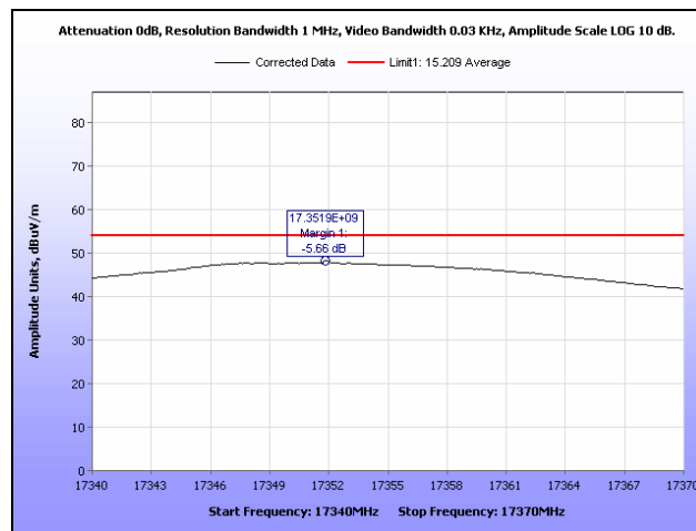
Plot 29. Radiated Spurious Emissions, Mid Channel, 3 rd Harmonic, Average, HT20
