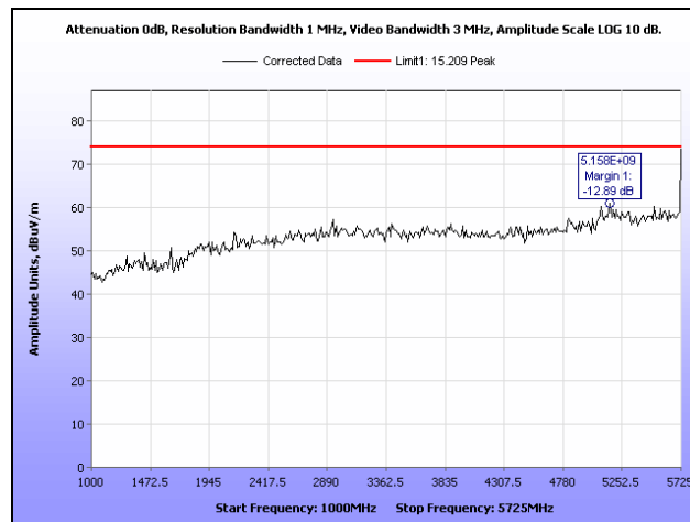
Plot 39. Radiated Spurious Emissions, Low Channel, 1 GHz – 5.725 GHz, Peak, HT40
