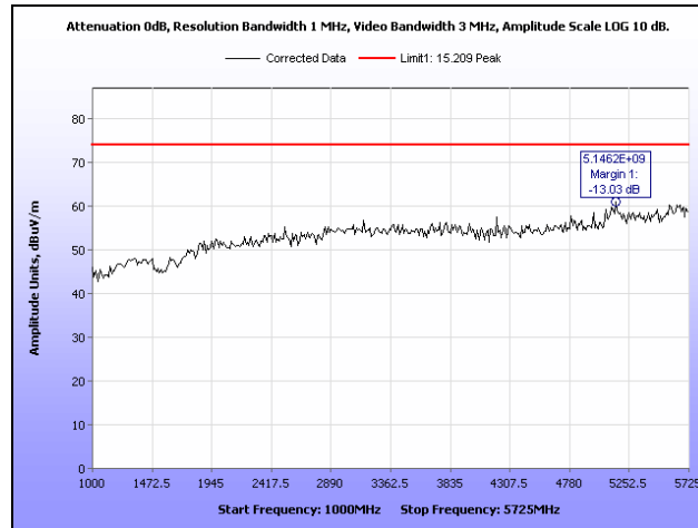
Plot 25. Radiated Spurious Emissions, Mid Channel, 1 GHz – 5.725 GHz, Peak, HT20
