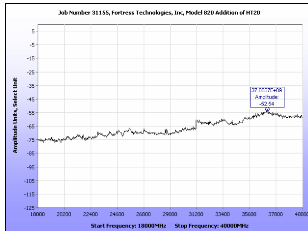
Plot 53. Conducted Spurious Emissions, Low Channel, 18 GHz – 40 GHz, HT20
