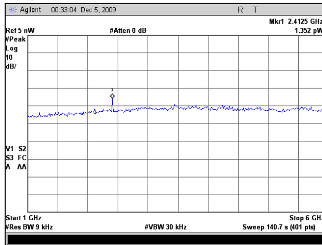
Plot 79. Receiver Spurious Emission, 1 GHz – 6 GHz, HT20
