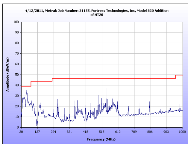
Plot 23. Radiated Spurious Emissions, Mid Channel, 30 MHz – 1 GHz, HT20
