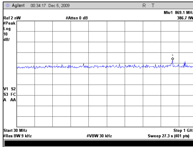
Plot 78. Receiver Spurious Emission, 30 MHz – 1 GHz, HT20
