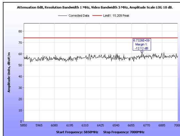
Plot 48. Radiated Spurious Emissions, High Channel, 5.850 GHz – 7 GHz, Peak, HT40
