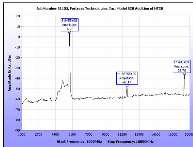
Plot 58. Conducted Spurious Emissions, High Channel, 1 GHz – 18 GHz, HT20
