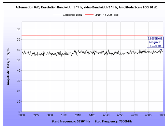
Plot 20. Radiated Spurious Emissions, Low Channel, 5.850 GHz – 7 GHz, Peak, HT20
