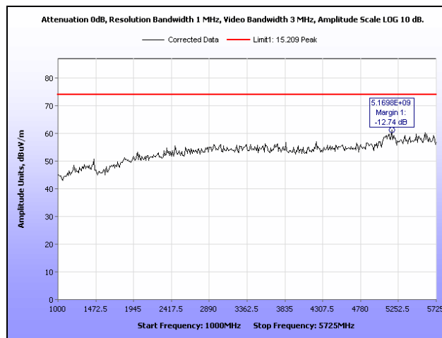
Plot 32. Radiated Spurious Emissions, High Channel, 1 GHz – 5.725 GHz, Peak, HT20
