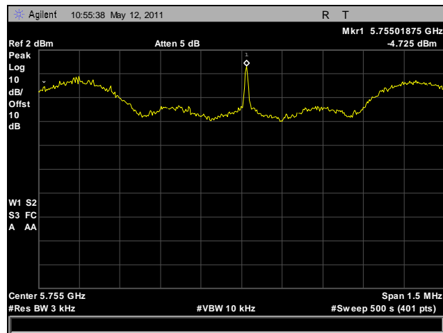
Plot 76. Peak Power Spectral Density, Low Channel, HT40
