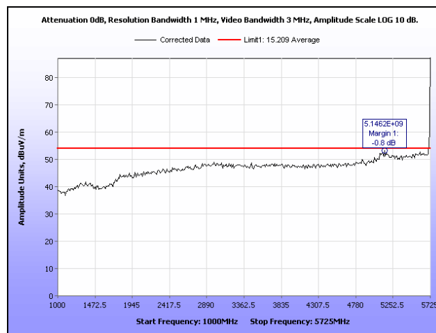
Plot 38. Radiated Spurious Emissions, Low Channel, 1 GHz – 5.725 GHz, Average Detector, HT40
