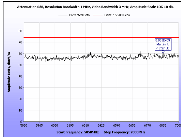
Plot 34. Radiated Spurious Emissions, High Channel, 5.850 GHz – 7 GHz, Peak, HT20
