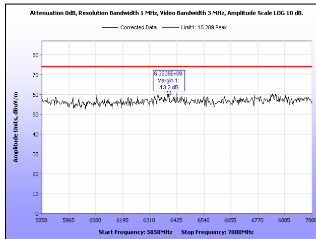
Plot 27. Radiated Spurious Emissions, Mid Channel, 5.850 GHz – 7 GHz, Peak, HT20
