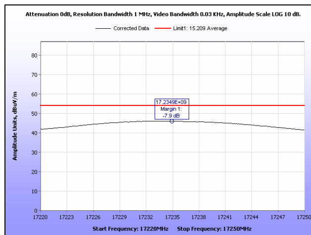
Plot 22. Radiated Spurious Emissions, Low Channel, 3 rd Harmonic, Average, HT20
