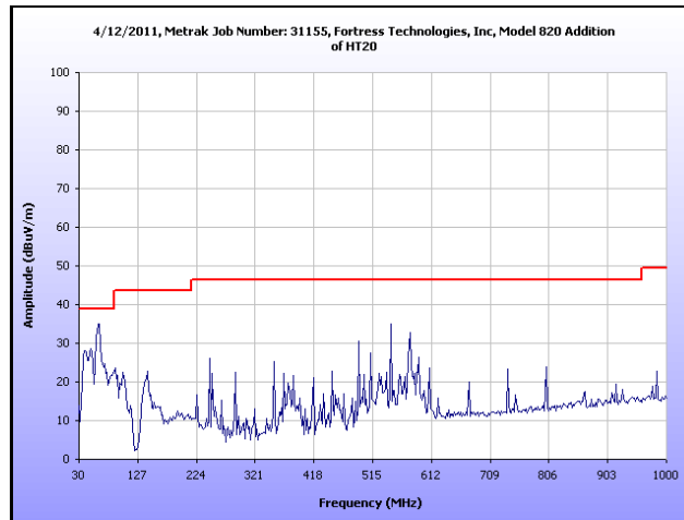
Plot 16. Radiated Spurious Emissions, Low Channel, 30 MHz – 1 GHz, HT20
