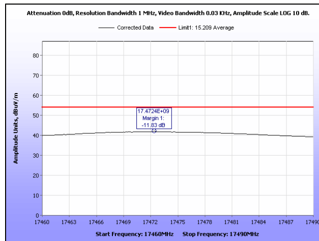
Plot 36. Radiated Spurious Emissions, High Channel, 3 rd Harmonic, Average, HT20
