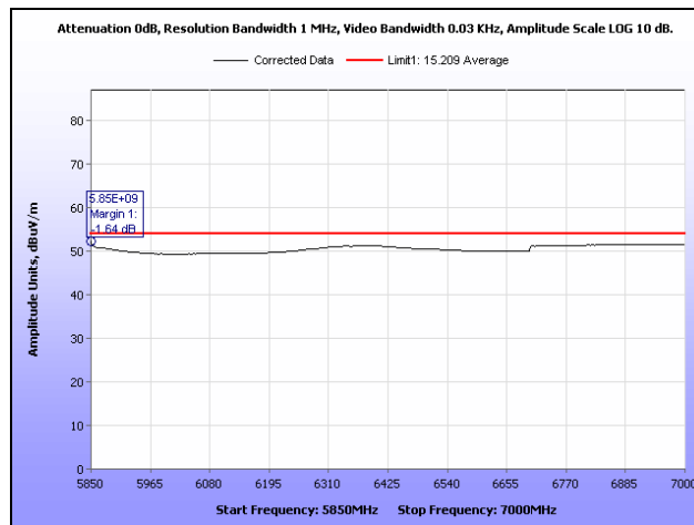
Plot 33. Radiated Spurious Emissions, High Channel, 5.850 GHz – 7 GHz, Average, HT20
