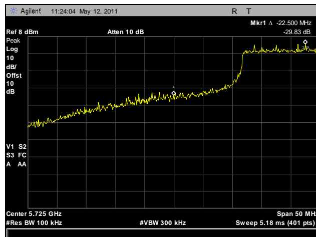
Plot 71. Conducted Band Edge, Low Channel, HT40
