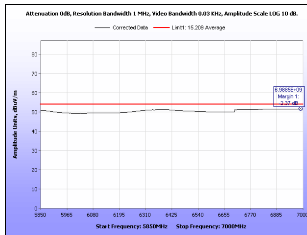
Plot 26. Radiated Spurious Emissions, Mid Channel, 5.850 GHz – 7 GHz, Average, HT20
