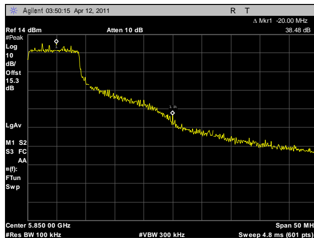
Plot 70. Conducted Band Edge, High Channel, HT20
