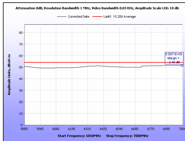
Plot 47. Radiated Spurious Emissions, High Channel, 5.850 GHz – 7 GHz, Average, HT40
