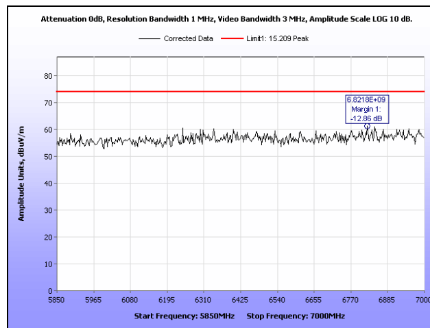
Plot 41. Radiated Spurious Emissions, Low Channel, 5.850 GHz – 7 GHz, Peak, HT40
