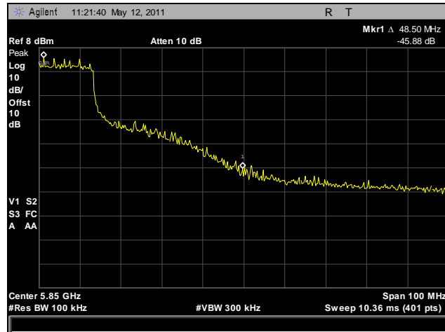
Plot 72. Conducted Band Edge, High Channel, HT40
