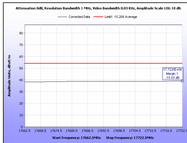
Plot 50. Radiated Spurious Emissions, High Channel, 3 rd Harmonic, Average, HT40
