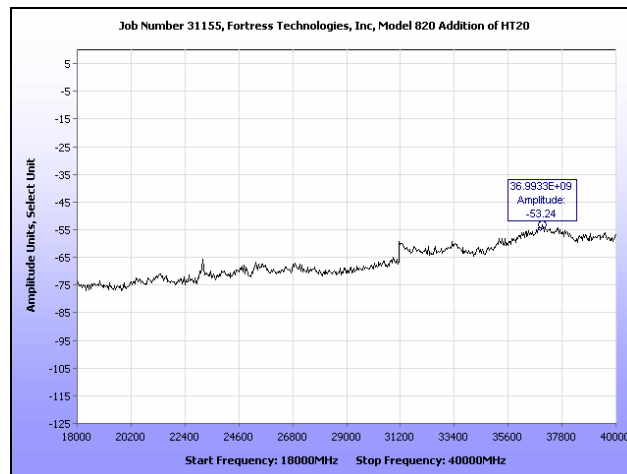
Plot 56. Conducted Spurious Emissions, Mid Channel, 18 GHz – 40 GHz, HT20
