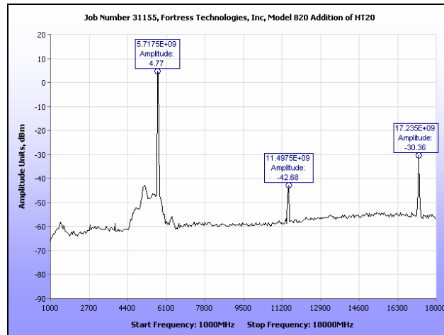
Plot 52. Conducted Spurious Emissions, Low Channel, 1 GHz – 18 GHz, HT20
