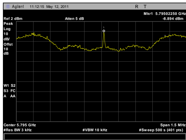
Plot 77. Peak Power Spectral Density, High Channel, HT40
