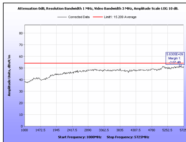
Plot 17. Radiated Spurious Emissions, Low Channel, 1 GHz – 5.725 GHz, Average Detector, HT20
