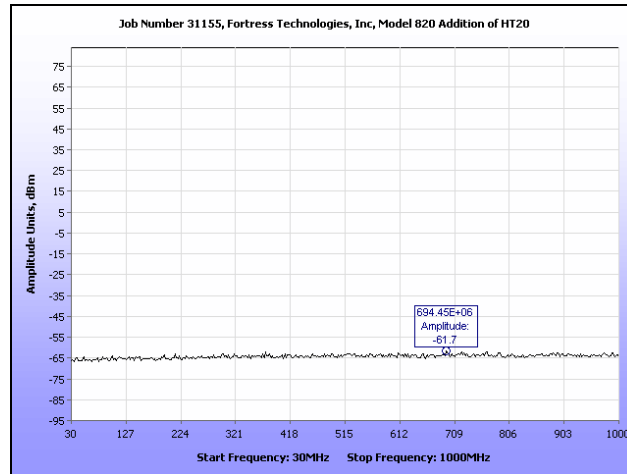
Plot 57. Conducted Spurious Emissions, High Channel, 30 MHz – 1 GHz, HT20
