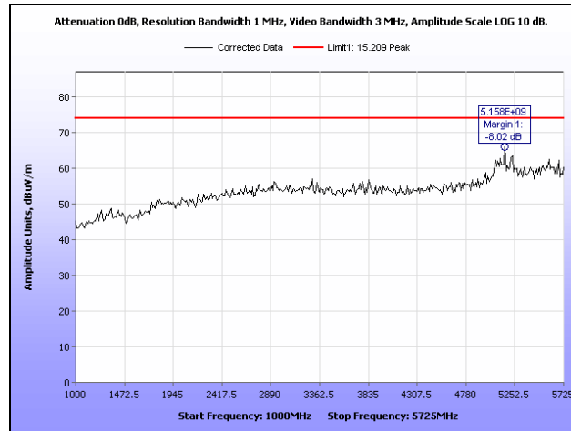
Plot 46. Radiated Spurious Emissions, High Channel, 1 GHz – 5.725 GHz, Peak, HT40
