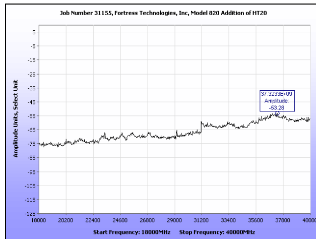
Plot 59. Conducted Spurious Emissions, High Channel, 18 GHz – 40 GHz, HT20
