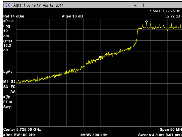
Plot 69. Conducted Band Edge, Low Channel, HT20
