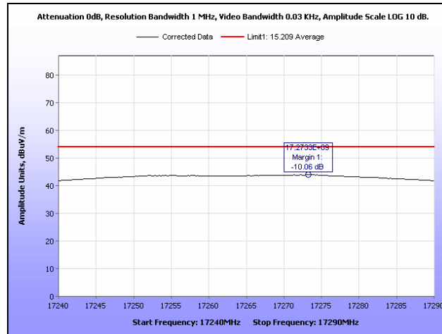
Plot 43. Radiated Spurious Emissions, Low Channel, 3 rd Harmonic, Average, HT40
