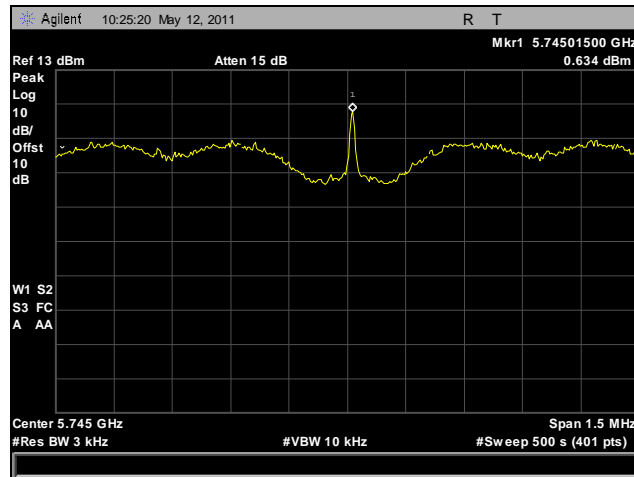
Plot 73. Peak Power Spectral Density, Low Channel, HT20
