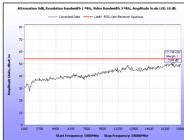
Plot 83. Receiver Spurious Emission, 1 GHz – 18 GHz, HT40
