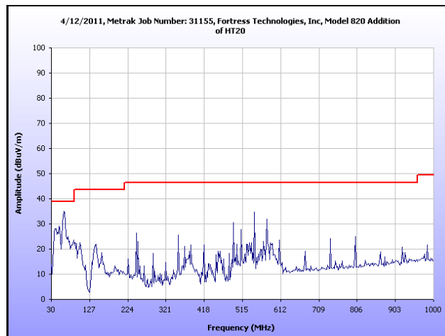
Plot 30. Radiated Spurious Emissions, High Channel, 30 MHz – 1 GHz, HT20
