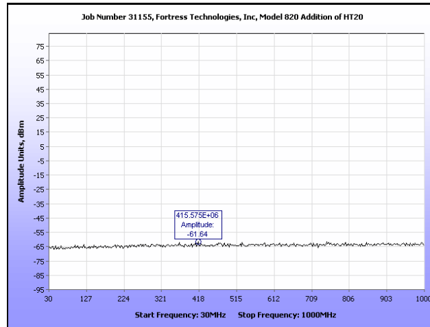
Plot 51. Conducted Spurious Emissions, Low Channel, 30 MHz – 1 GHz, HT20
