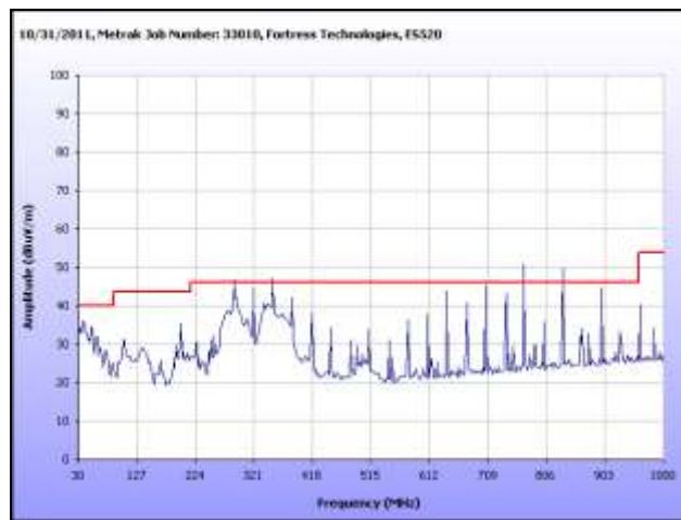
Plot 40. Radiated Spurious Emissions, 5300 MHz, 30 MHz – 1 GHz, Omni Antenna
