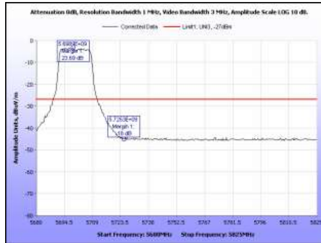
Plot 63. EIRP, 5700 MHz, Band Edge, Omni Antenna
