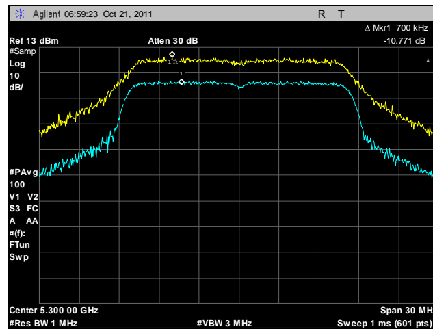
Plot 31. Peak Excursion Ratio, 5300 MHz
