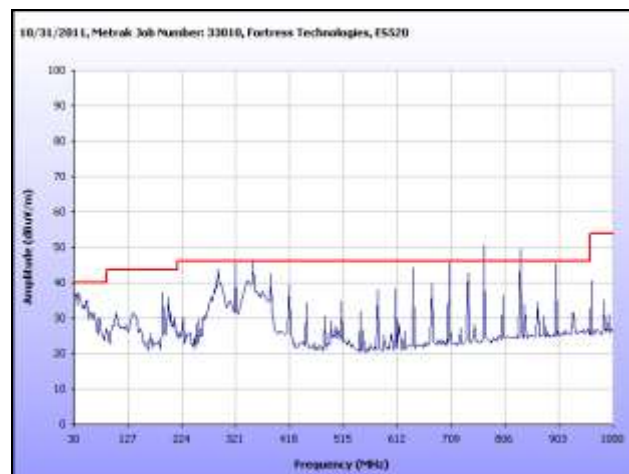
Plot 56. Radiated Spurious Emissions, 5700 MHz, 30 MHz – 1 GHz, Omni Antenna
