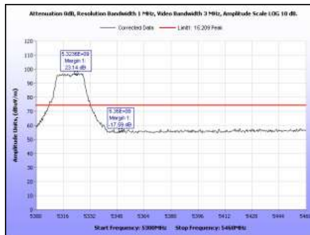
Plot 65. Radiated Restricted Band, 5320 MHz, Peak
