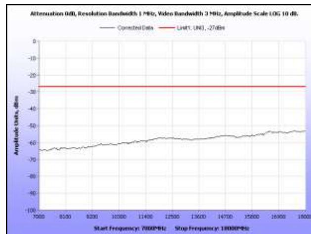
Plot 38. Radiated Spurious Emissions, 5260 MHz, 7 GHz – 18 GHz, Omni Antenna
