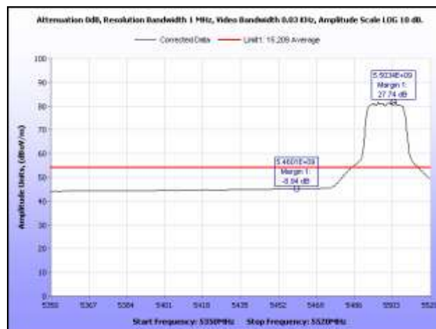
Plot 66. Radiated Restricted Band, 5500 MHz, Average
