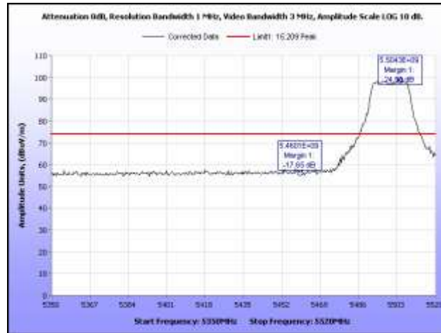
Plot 67. Radiated Restricted Band, 5500 MHz, Peak
