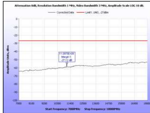
Plot 54. Radiated Spurious Emissions, 5560 MHz, 7 GHz – 18 GHz, Omni Antenna
