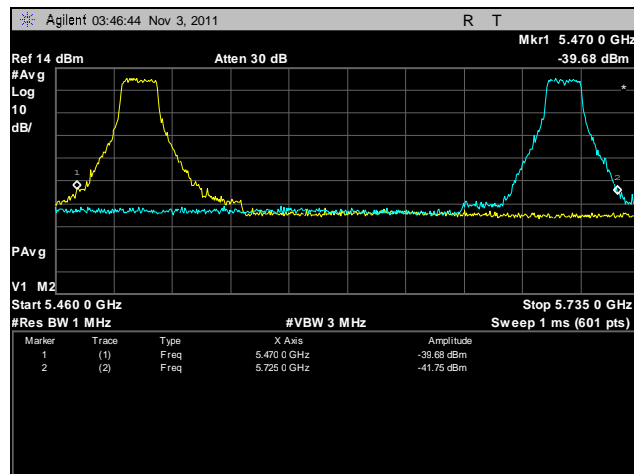
Plot 81. Frequency Stability, 5470 – 5725 MHz, -20°C, 120 V
