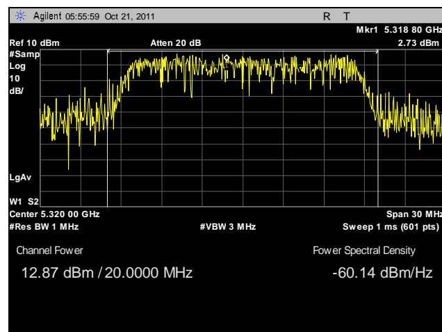
Plot 20. RF Power Output, 5320 MHz
