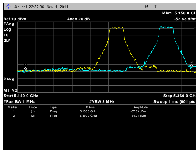
Plot 74. Frequency Stability, 5250 – 5350 MHz, 20°C, 108 V
