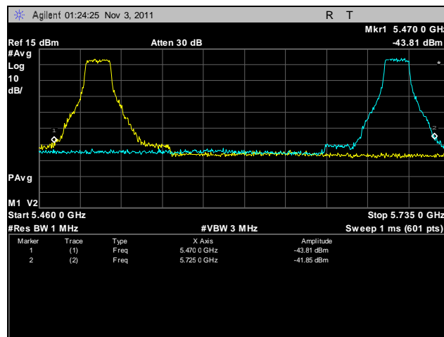
Plot 83. Frequency Stability, 5470 – 5725 MHz, 0°C, 120 V
