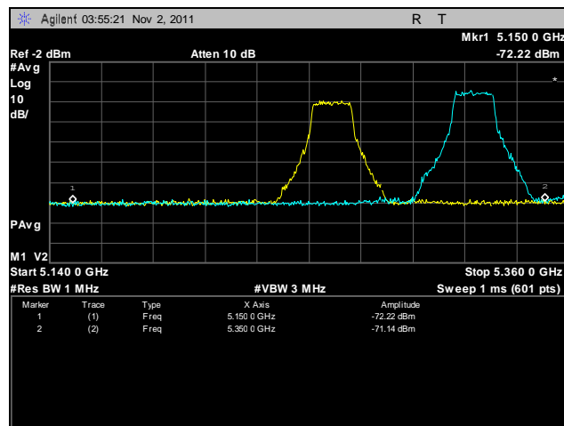
Plot 80. Frequency Stability, 5250 – 5350 MHz, 55°C, 120 V
