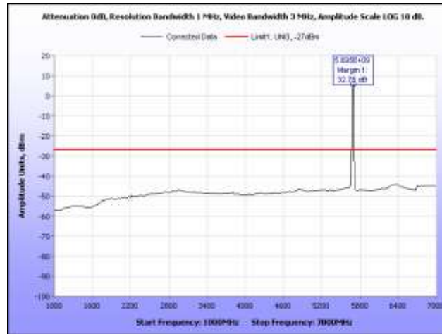
Plot 57. Radiated Spurious Emissions, 5700 MHz, 1 GHz – 7 GHz, Omni Antenna
