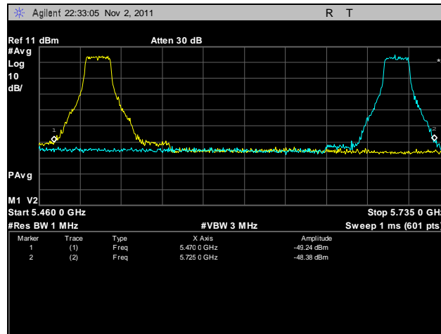
Plot 86. Frequency Stability, 5470 – 5725 MHz, 20°C, 120 V
