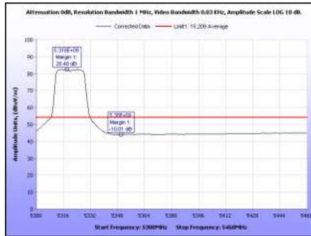
Plot 64. Radiated Restricted Band, 5320 MHz, Average
