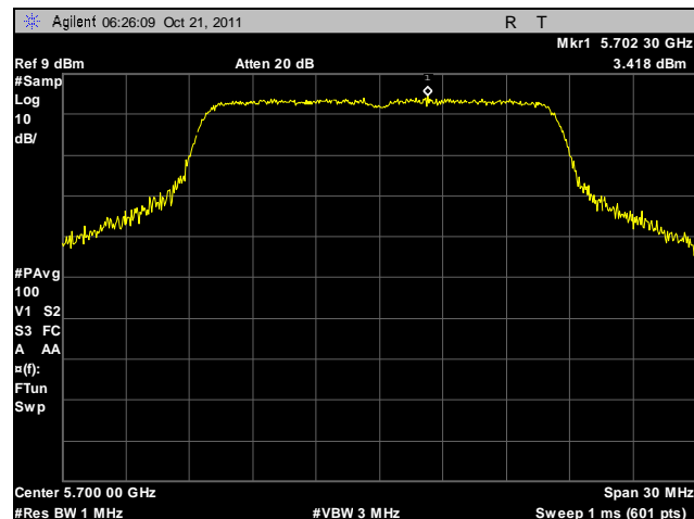
Plot 29. Power Spectral Density, 5700 MHz
