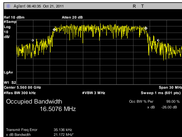
Plot 16. 99% Occupied Bandwidth, 5560 MHz
