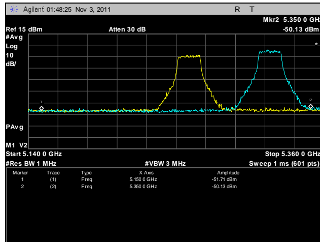
Plot 71. Frequency Stability, 5250 – 5350 MHz, -10°C, 120 V
