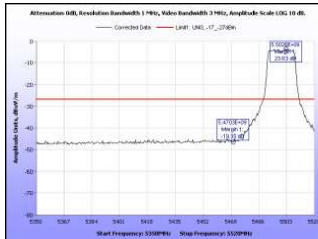
Plot 62. EIRP, 5500 MHz, Band Edge, Omni Antenna
