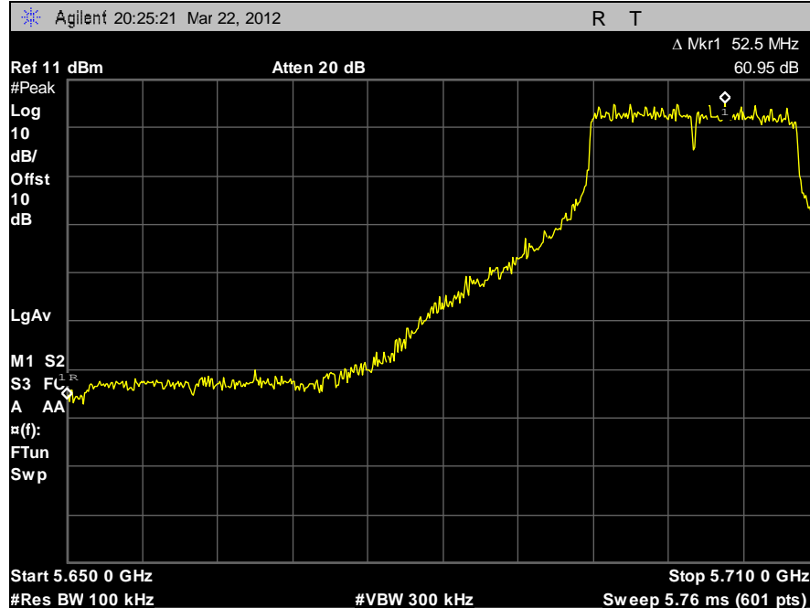
Plot 69. 5700 MHz, 20 dB
