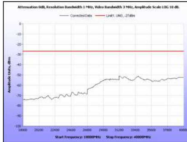
Plot 51. Radiated Spurious Emissions, 5500 MHz, 18 GHz – 40 GHz, Omni Antenna
