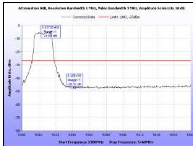
Plot 61. EIRP, 5320 MHz, Band Edge, Omni Antenna
