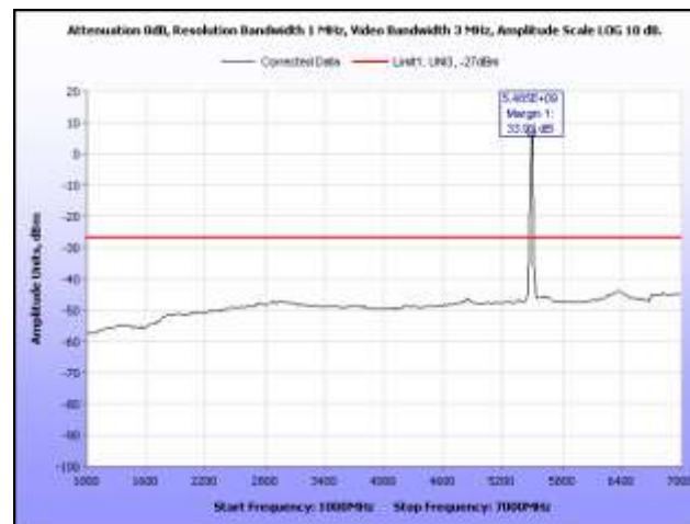
Plot 49. Radiated Spurious Emissions, 5500 MHz, 1 GHz – 7 GHz, Omni Antenna
