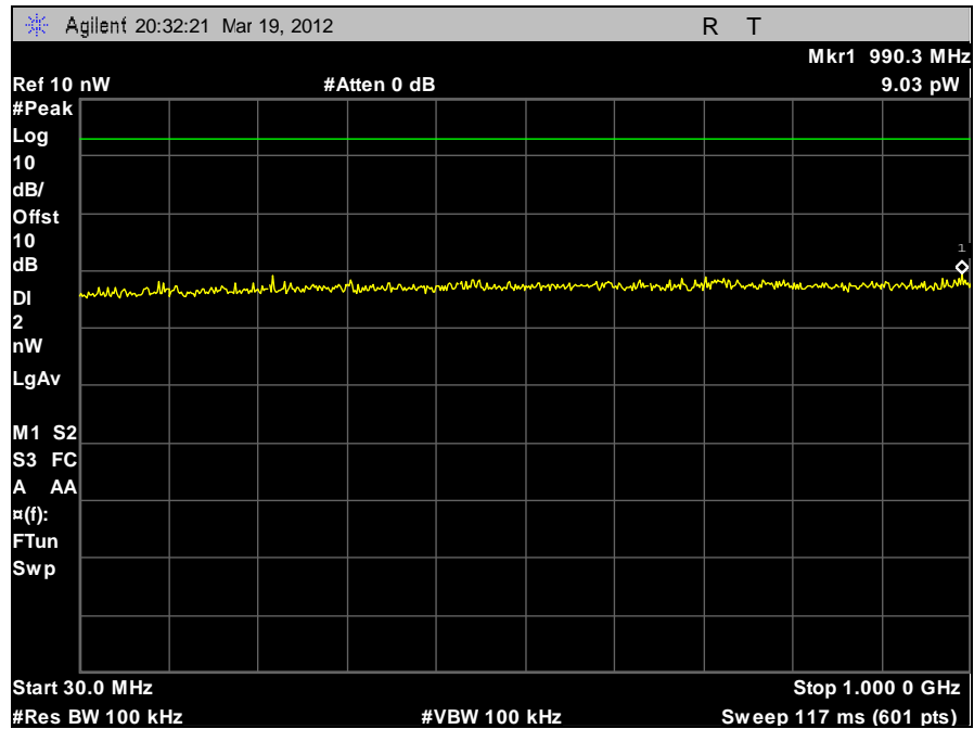
Plot 92. Receiver Spurious Emission, 30 MHz – 1 GHz
