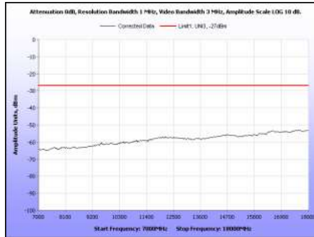
Plot 42. Radiated Spurious Emissions, 5300 MHz, 7 GHz – 18 GHz, Omni Antenna
