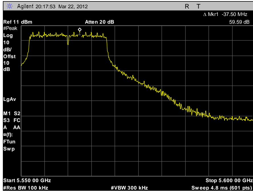
Plot 68. 5560 MHz, 20 dB
