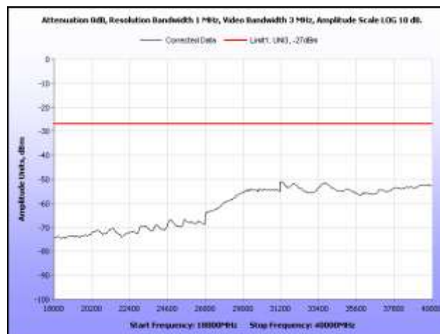
Plot 43. Radiated Spurious Emissions, 5300 MHz, 18 GHz – 40 GHz, Omni Antenna
