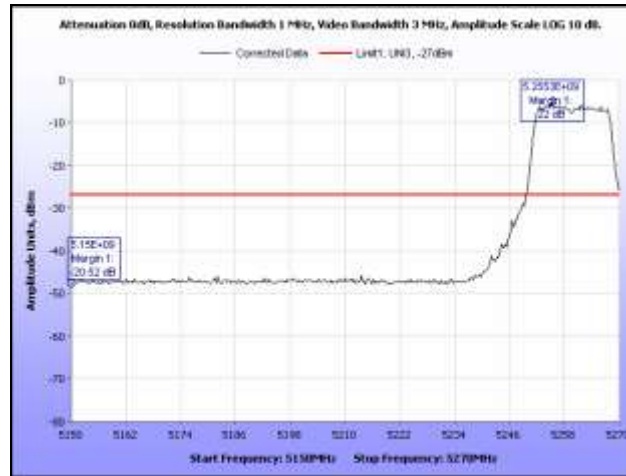
Plot 60. EIRP, 5260 MHz, Band Edge, Omni Antenna
