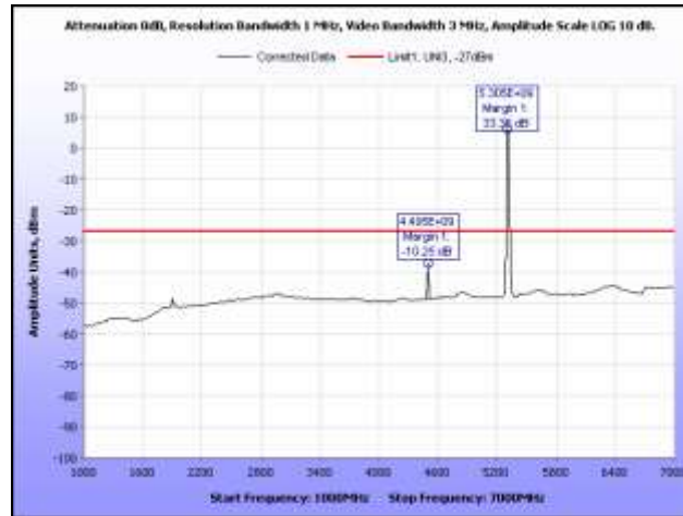
Plot 45. Radiated Spurious Emissions, 5320 MHz, 1 GHz – 7 GHz, Omni Antenna
