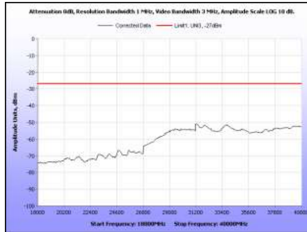
Plot 39. Radiated Spurious Emissions, 5260 MHz, 18 GHz – 40 GHz, Omni Antenna
