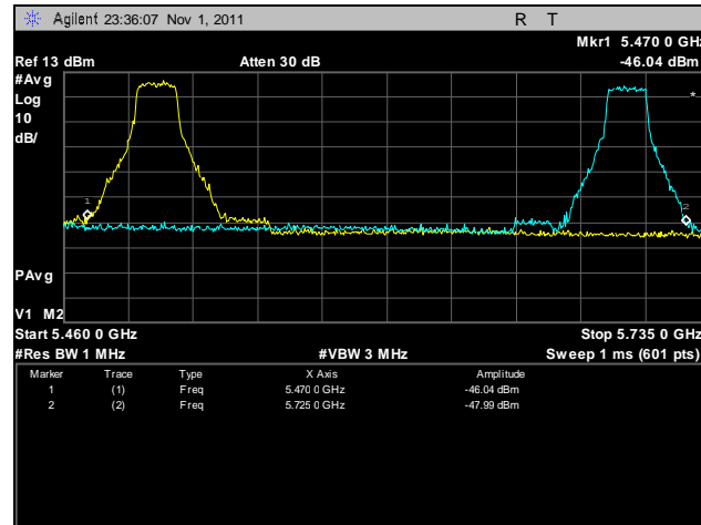
Plot 88. Frequency Stability, 5470 – 5725 MHz, 30°C, 120 V
