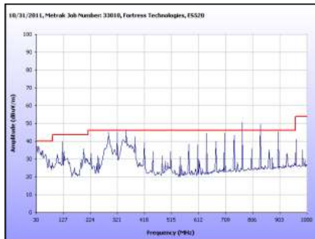
Plot 52. Radiated Spurious Emissions, 5560 MHz, 30 MHz – 1 GHz, Omni Antenna
