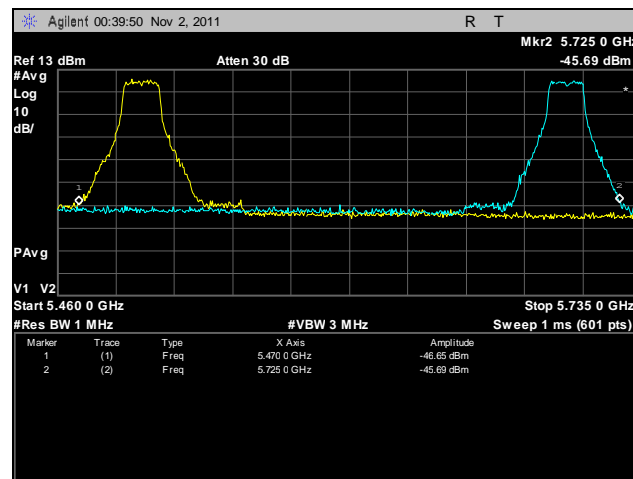
Plot 89. Frequency Stability, 5470 – 5725 MHz, 40°C, 120 V
