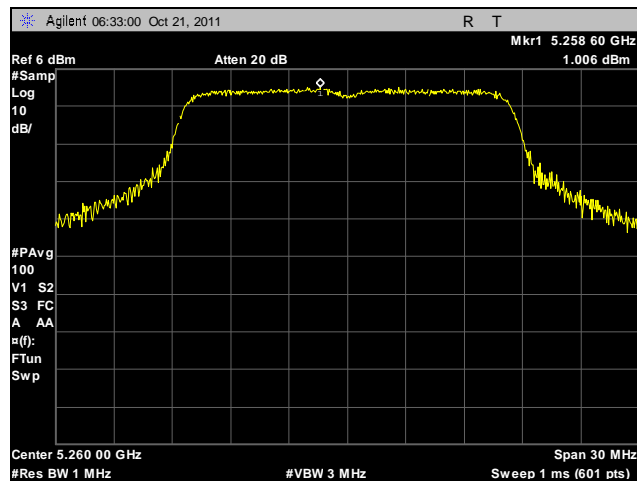
Plot 24. Power Spectral Density, 5260 MHz
