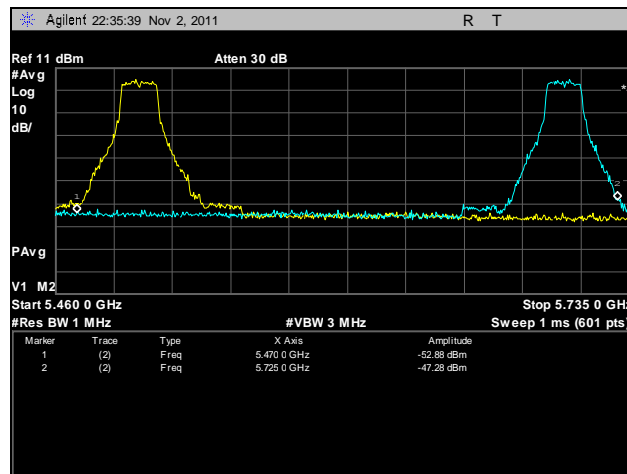
Plot 87. Frequency Stability, 5470 – 5725 MHz, 20°C, 132 V
