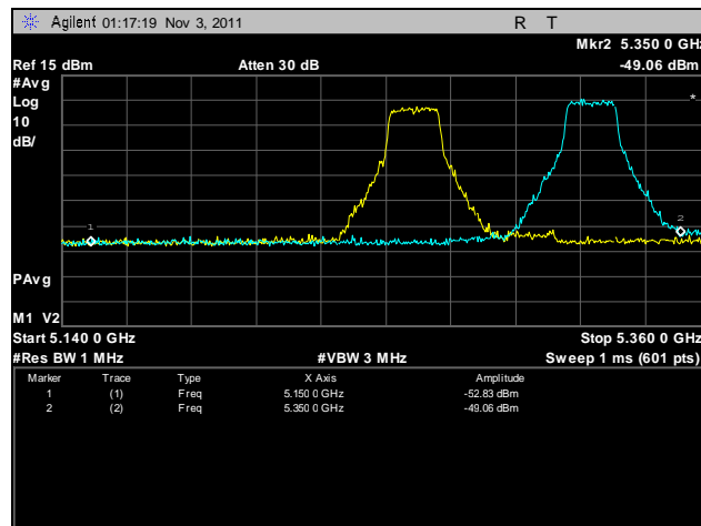
Plot 72. Frequency Stability, 5250 – 5350 MHz, 0°C, 120 V
