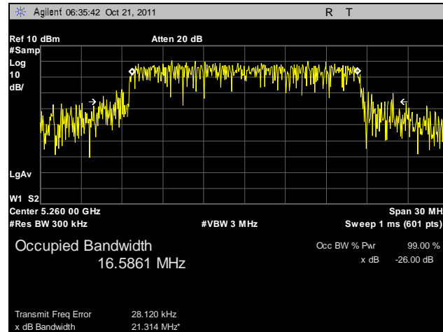
Plot 12. 99% Occupied Bandwidth, 5260 MHz
