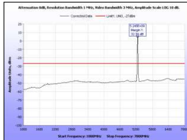
Plot 37. Radiated Spurious Emissions, 5260 MHz, 1 GHz – 7 GHz, Omni Antenna
