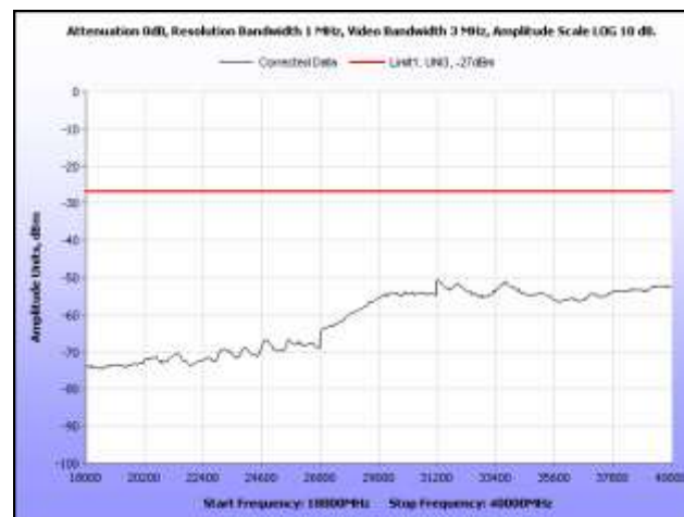
Plot 55. Radiated Spurious Emissions, 5560 MHz, 18 GHz – 40 GHz, Omni Antenna
