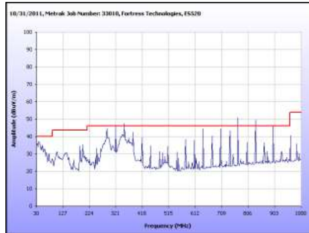
Plot 48. Radiated Spurious Emissions, 5500 MHz, 30 MHz – 1 GHz, Omni Antenna
