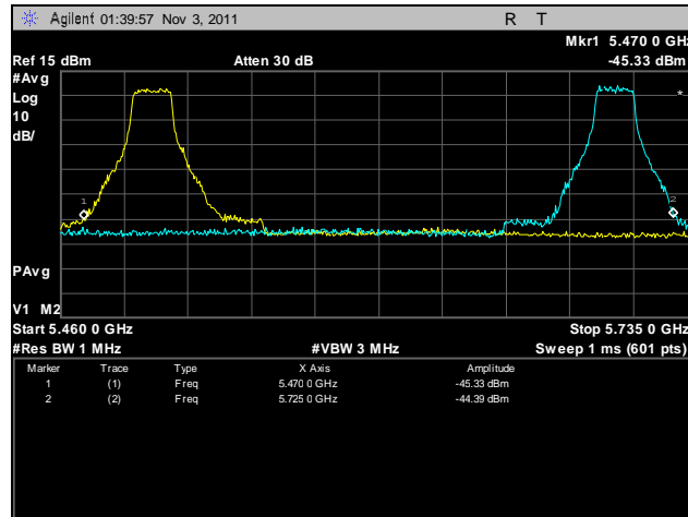
Plot 82. Frequency Stability, 5470 – 5725 MHz, -10°C, 120 V
