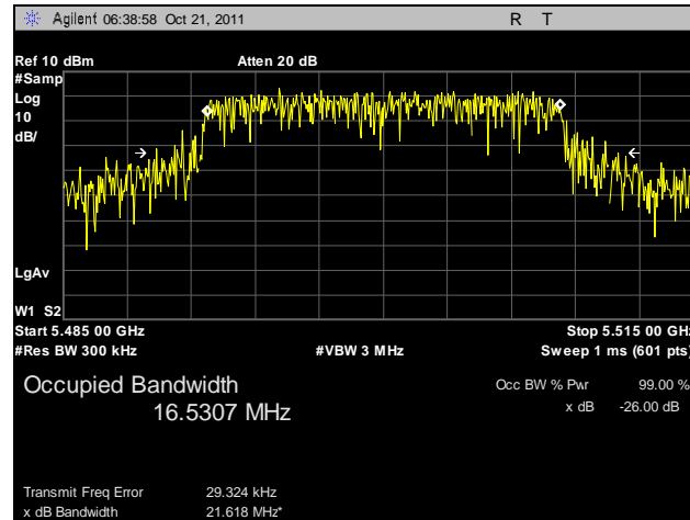
Plot 15. 99% Occupied Bandwidth, 5500 MHz
