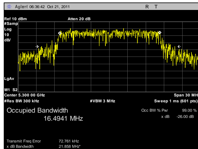
Plot 13. 99% Occupied Bandwidth, 5300 MHz
