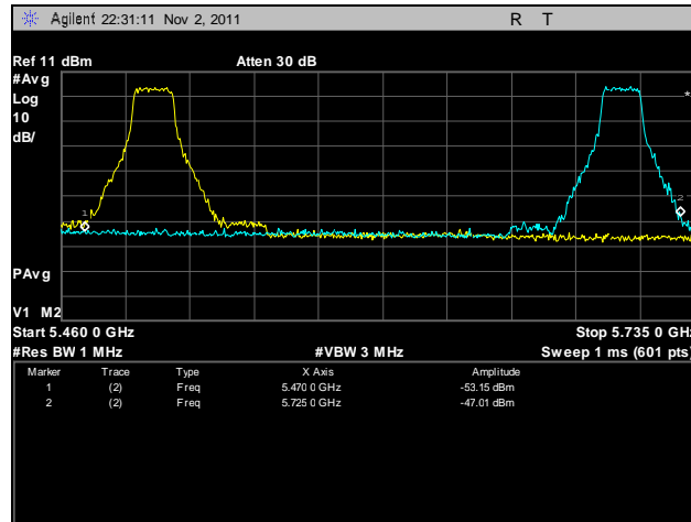
Plot 85. Frequency Stability, 5470 – 5725 MHz, 20°C, 108 V
