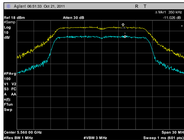
Plot 34. Peak Excursion Ratio, 5560 MHz
