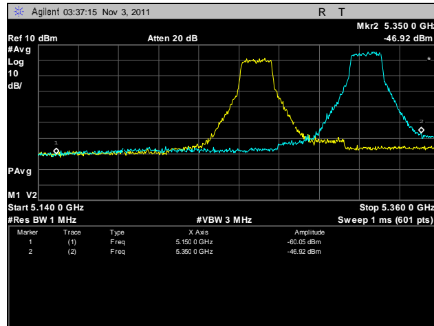
Plot 70. Frequency Stability, 5250 – 5350 MHz, -20°C, 120 V
