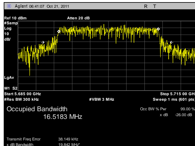
Plot 17. 99% Occupied Bandwidth, 5700 MHz
