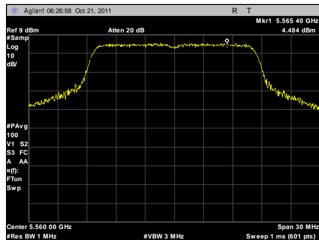
Plot 28. Power Spectral Density, 5560 MHz
