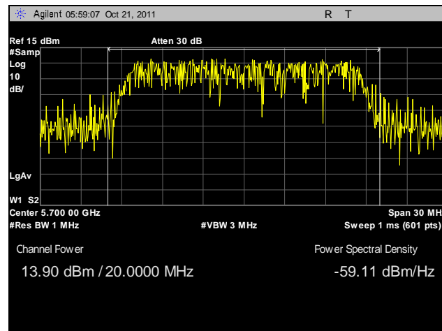
Plot 23. RF Power Output, 5700 MHz
