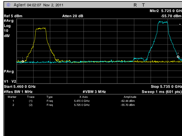
Plot 91. Frequency Stability, 5470 – 5725 MHz, 55°C, 120 V
