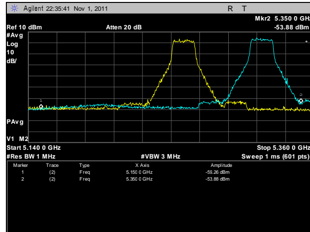
Plot 76. Frequency Stability, 5250 – 5350 MHz, 20°C, 132 V
