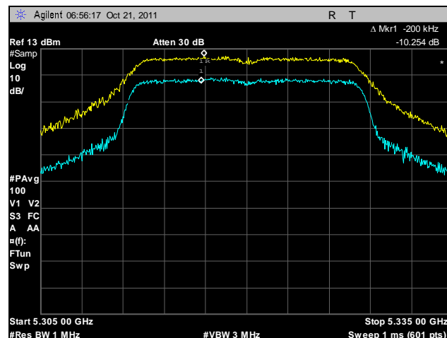
Plot 32. Peak Excursion Ratio, 5320 MHz
