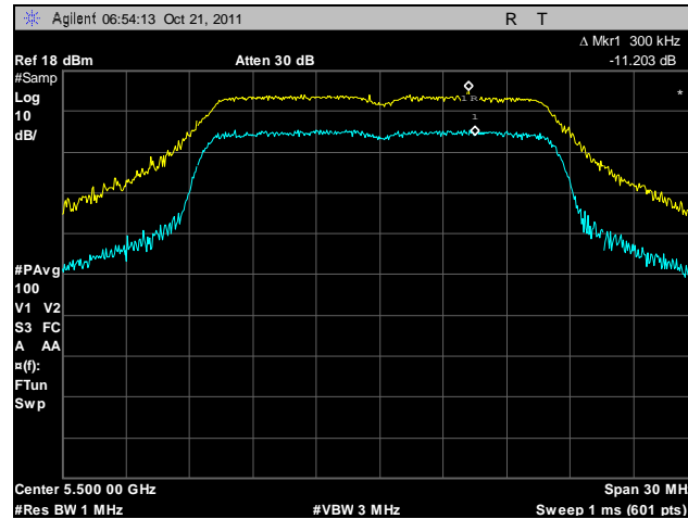
Plot 33. Peak Excursion Ratio, 5500 MHz
