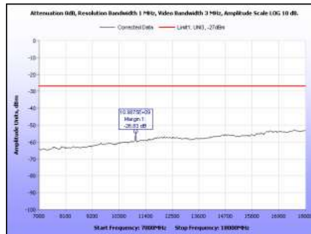
Plot 50. Radiated Spurious Emissions, 5500 MHz, 7 GHz – 18 GHz, Omni Antenna
