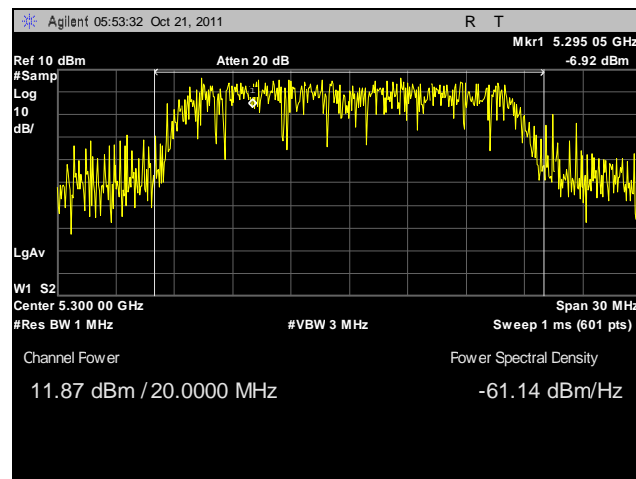
Plot 19. RF Power Output, 5300 MHz
