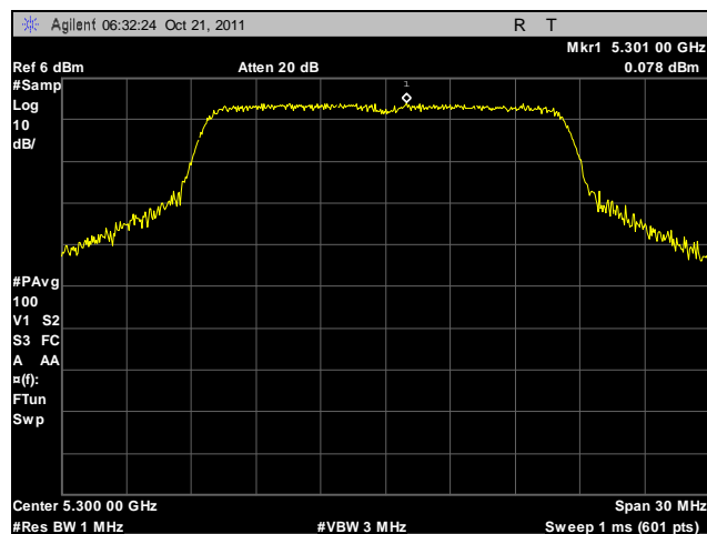
Plot 25. Power Spectral Density, 5300 MHz
