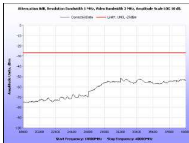
Plot 59. Radiated Spurious Emissions, 5700 MHz, 18 GHz – 40 GHz, Omni Antenna
