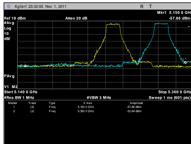
Plot 77. Frequency Stability, 5250 – 5350 MHz, 30°C, 120 V
