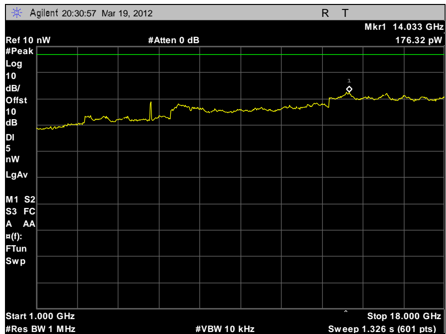
Plot 93. Receiver Spurious Emission, 1 GHz – 18 GHz
