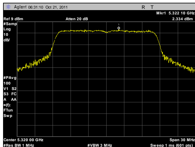
Plot 26. Power Spectral Density, 5320 MHz
