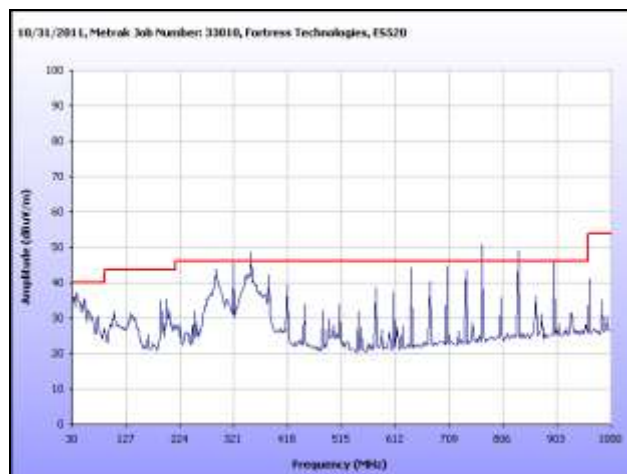
Plot 44. Radiated Spurious Emissions, 5320 MHz, 30 MHz – 1 GHz, Omni Antenna
