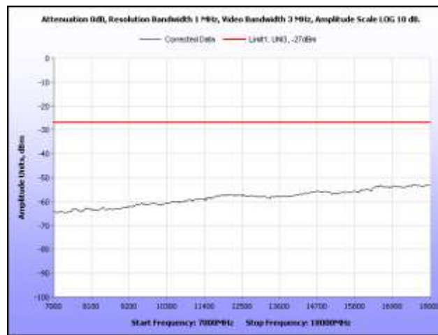
Plot 46. Radiated Spurious Emissions, 5320 MHz, 7 GHz – 18 GHz, Omni Antenna
