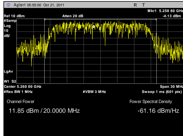
Plot 18. RF Power Output, 5260 MHz
