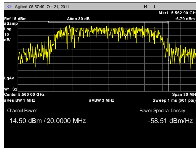
Plot 22. RF Power Output, 5560 MHz
