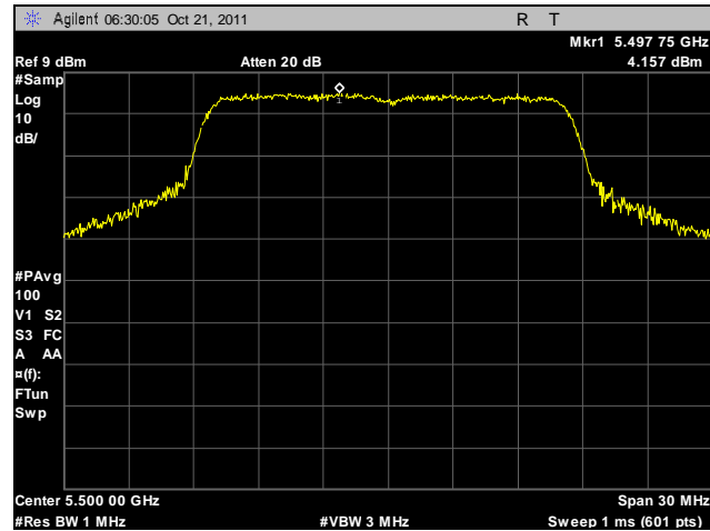
Plot 27. Power Spectral Density, 5500 MHz
