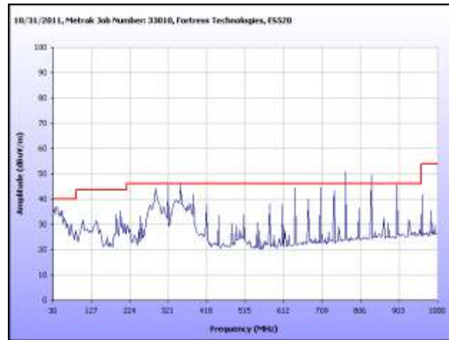
Plot 36. Radiated Spurious Emissions, 5260 MHz, 30 MHz – 1 GHz, Omni Antenna
