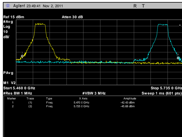
Plot 84. Frequency Stability, 5470 – 5725 MHz, 10°C, 120 V
