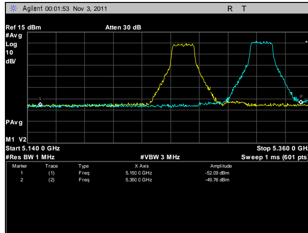
Plot 73. Frequency Stability, 5250 – 5350 MHz, 10°C, 120 V
