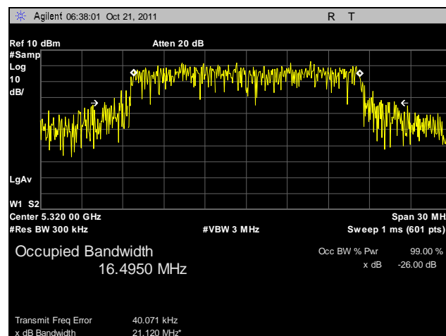
Plot 14. 99% Occupied Bandwidth, 5320 MHz
