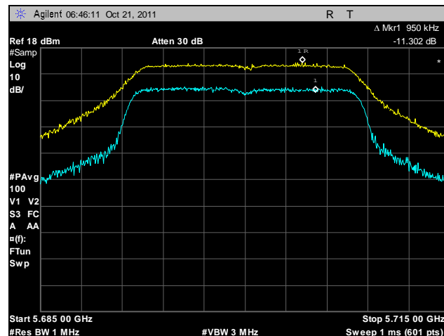
Plot 35. Peak Excursion Ratio, 5700 MHz
