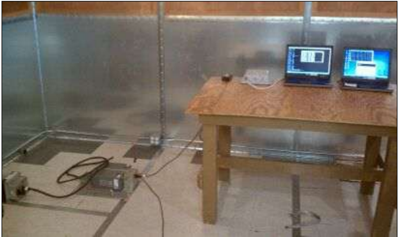
Photograph 4. Conducted Emissions, Test Setup
