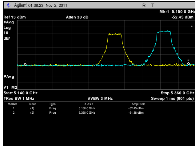
Plot 79. Frequency Stability, 5250 – 5350 MHz, 50°C, 120 V
