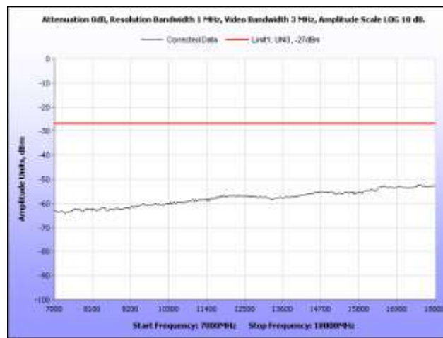
Plot 58. Radiated Spurious Emissions, 5700 MHz, 7 GHz – 18 GHz, Omni Antenna
