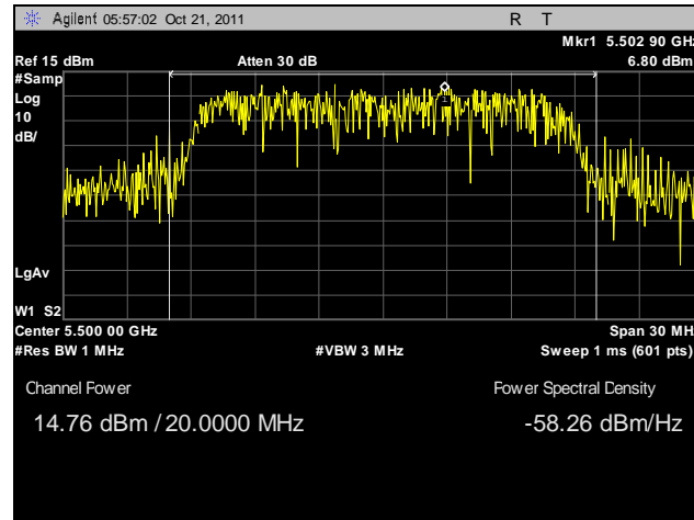
Plot 21. RF Power Output, 5500 MHz
