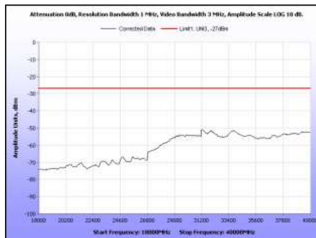
Plot 47. Radiated Spurious Emissions, 5320 MHz, 18 GHz – 40 GHz, Omni Antenna
