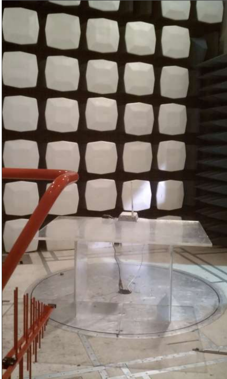
Photograph 2. Radiated Emission, Test Setup
