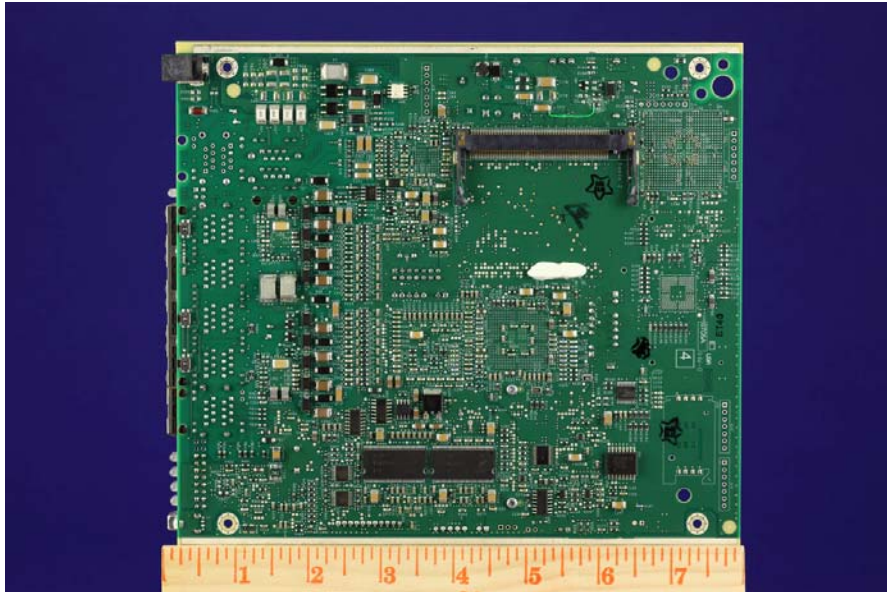
Main Board Bottom View
