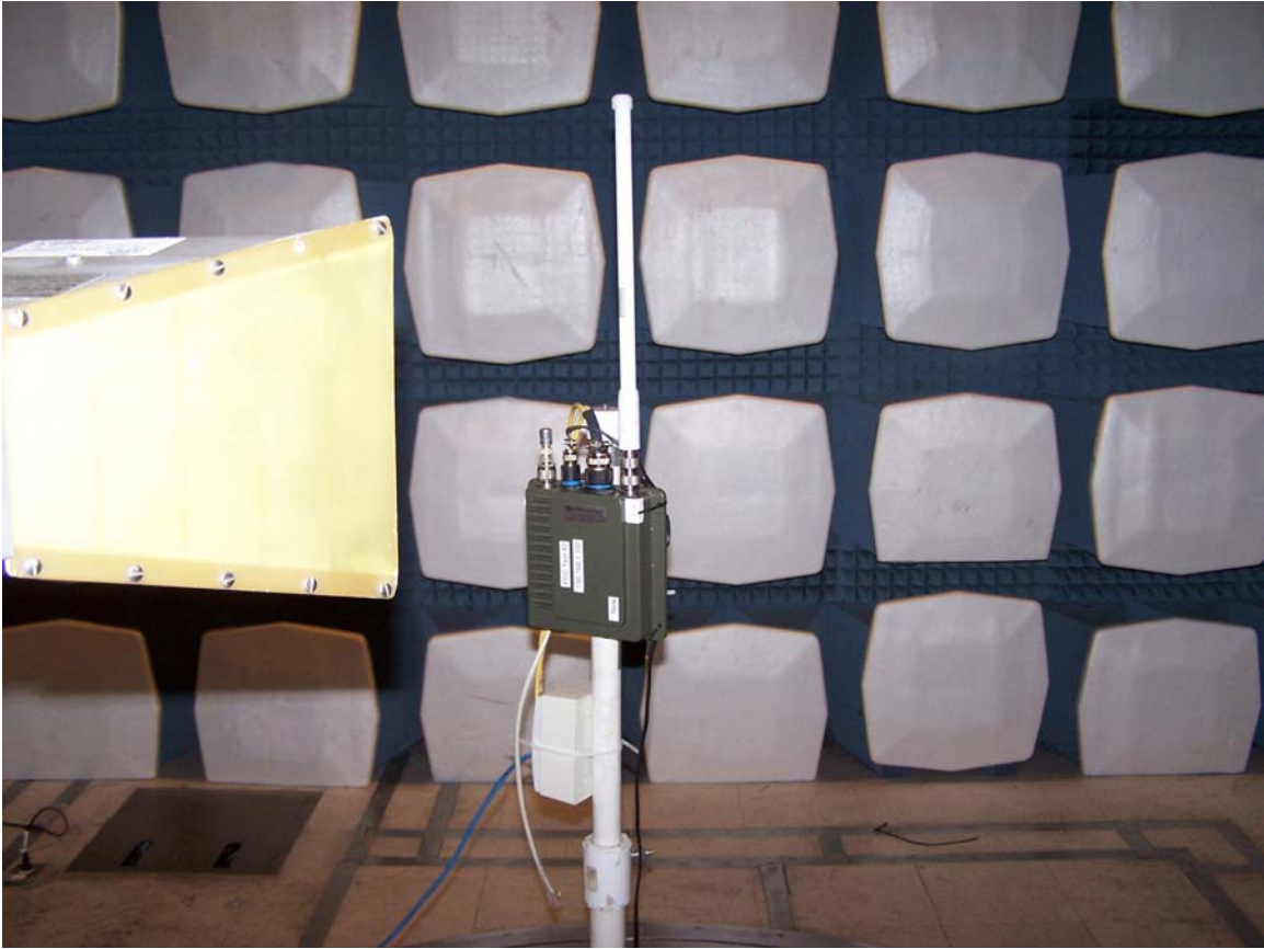
Photograph 5. Radiated Spurious Emissions
