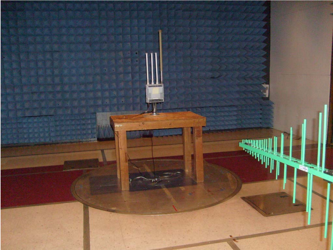
Photograph 2. Radiated Emissions, 30 MHz – 1 GHz
