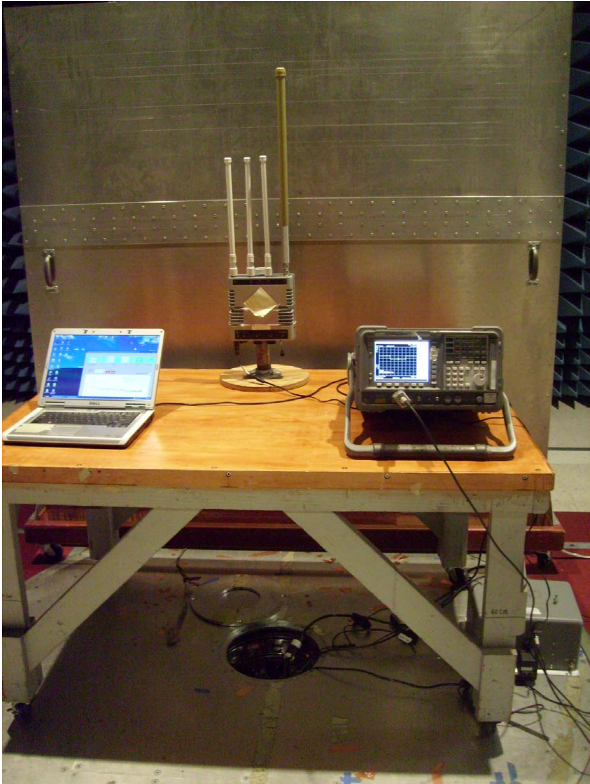
Photograph 1. Conducted Emissions
