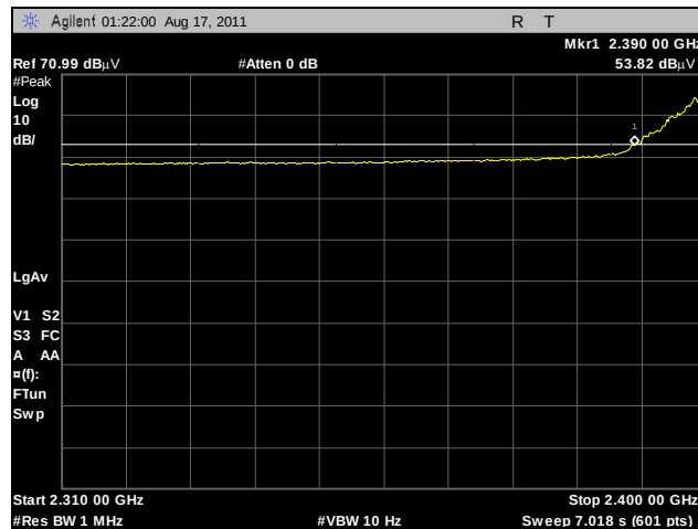
Plot 387. Radiated Restricted Band Edge, Low Channel, 2.4 GHz, 802.11g, Average, Sector
