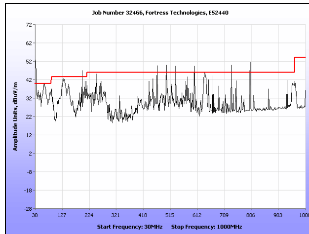
Plot 349. Radiated Spurs, Low Channel, 5.8 GHz, 802.11n 40 MHz, 30 MHz – 1 GHz, Sector
