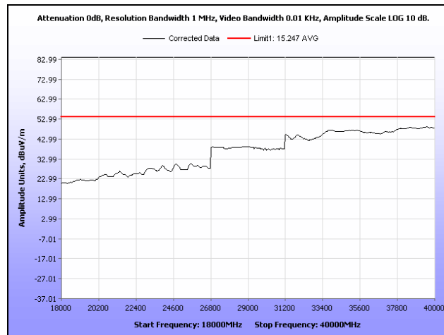
Plot 182. Radiated Spurs, High Channel, 2.4 GHz, 802.11g HT20, 18 GHz – 40 GHz, Average, Omni
