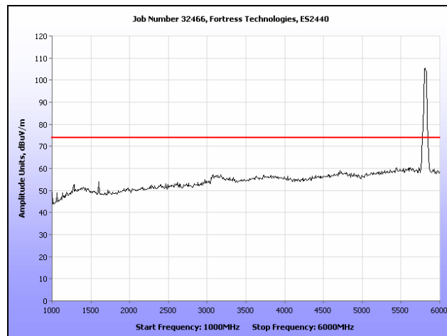
Plot 309. Radiated Spurs, High Channel, 5.8 GHz, 802.11n 40 MHz, 1 GHz – 6 GHz, Peak, Omni
