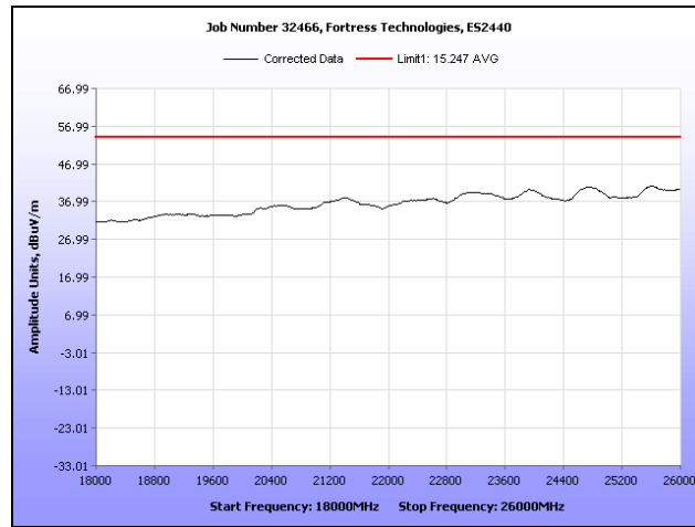
Plot 247. Radiated Spurs, Low Channel, 2.4 GHz, 802.11g HT40, 18 GHz – 26 GHz, Average, Sector
