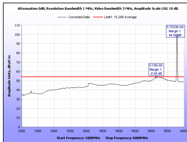
Plot 320. Radiated Spurs, Mid Channel, 5.8 GHz, 802.11a, 1 GHz – 6 GHz, Average, Sector
