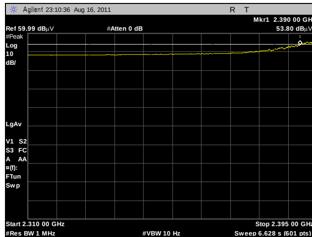
Plot 379. Radiated Restricted Band Edge, Low Channel, 2.4 GHz, 802.11g HT40, Average, Omni
