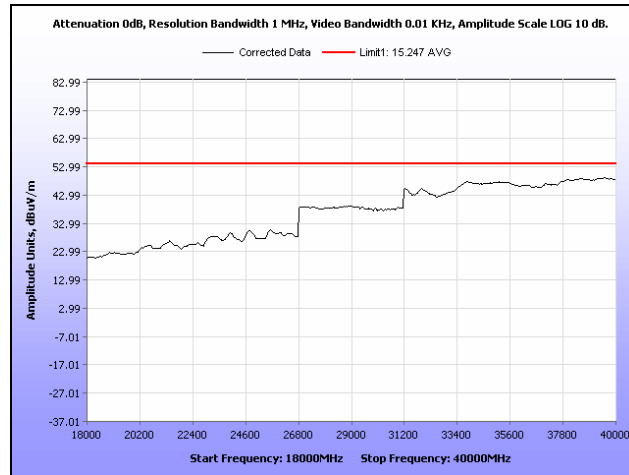
Plot 152. Radiated Spurs, High Channel, 2.4 GHz, 802.11b, 18 GHz – 40 GHz, Average, Omni
