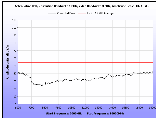
Plot 262. Radiated Spurs, Low Channel, 5.8 GHz, 802.11a, 6 GHz – 18 GHz, Peak under Avg., Omni
