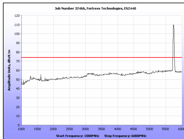
Plot 279. Radiated Spurs, Low Channel, 5.8 GHz, 802.11n 20 MHz, 1 GHz – 6 GHz, Peak, Omni
