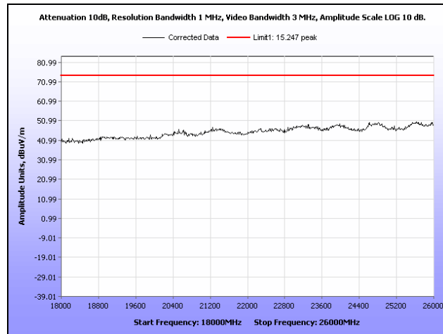
Plot 238. Radiated Spurs, Mid Channel, 2.4 GHz, 802.11g HT20, 18 GHz – 26 GHz, Peak, Sector
