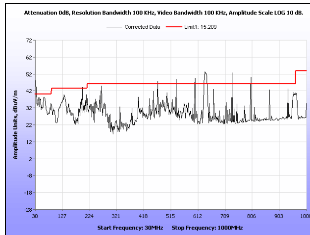
Plot 331. Radiated Spurs, Low Channel, 5.8 GHz, 802.11n 20 MHz, 30 MHz – 1 GHz, Sector
