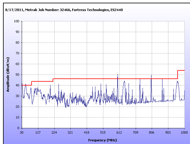
Plot 189. Radiated Spurs, Mid Channel, 2.4 GHz, 802.11g HT40, 30 MHz – 1 GHz, Omni
