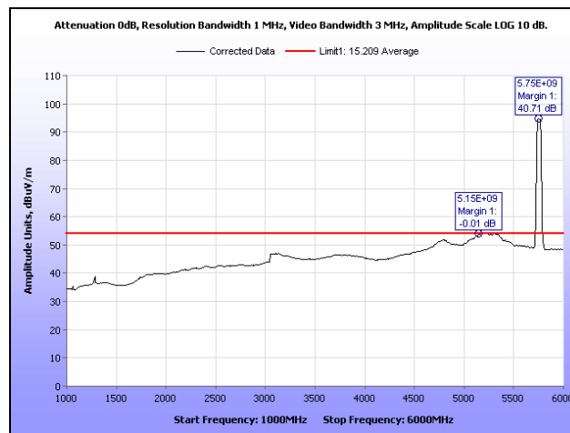
Plot 350. Radiated Spurs, Low Channel, 5.8 GHz, 802.11n 40 MHz, 1 GHz – 6 GHz, Average, Sector
