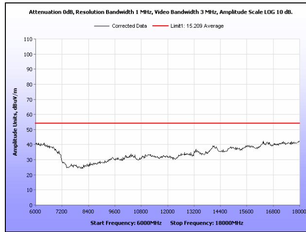
Plot 298. Radiated Spurs, Low Channel, 5.8 GHz, 802.11n 40 MHz, 6 GHz – 18 GHz, Peak under Avg., Omni
