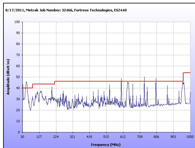
Plot 179. Radiated Spurs, High Channel, 2.4 GHz, 802.11g HT20, 30 MHz – 1 GHz, Omni
