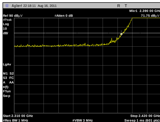
Plot 372. Radiated Restricted Band Edge, Low Channel, 2.4 GHz, 802.11g, Peak, Omni
