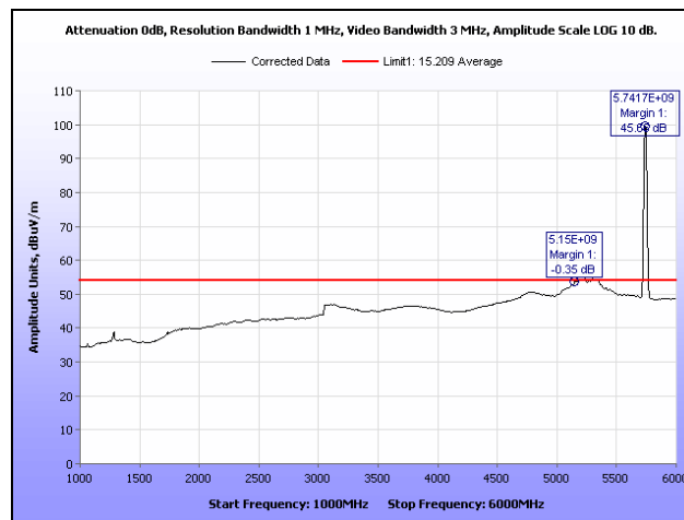
Plot 332. Radiated Spurs, Low Channel, 5.8 GHz, 802.11n 20 MHz, 1 GHz – 6 GHz, Average, Sector
