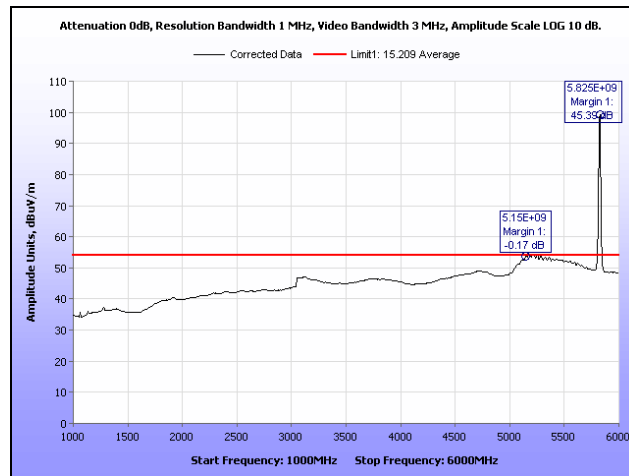
Plot 290. Radiated Spurs, High Channel, 5.8 GHz, 802.11n 20 MHz, 1 GHz – 6 GHz, Average, Omni
