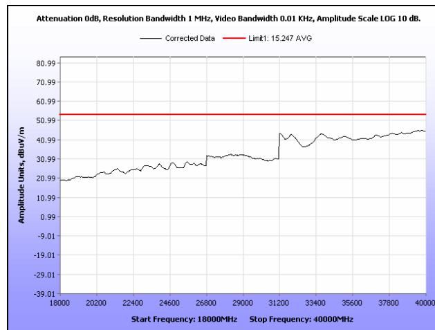
Plot 365. Radiated Spurs, High Channel, 5.8 GHz, 802.11n 40 MHz, 18 GHz – 40 GHz, Average, Sector
