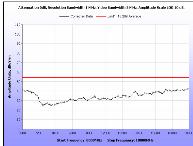
Plot 304. Radiated Spurs, Mid Channel, 5.8 GHz, 802.11n 40 MHz, 6 GHz – 18 GHz, Peak under Avg., Omni
