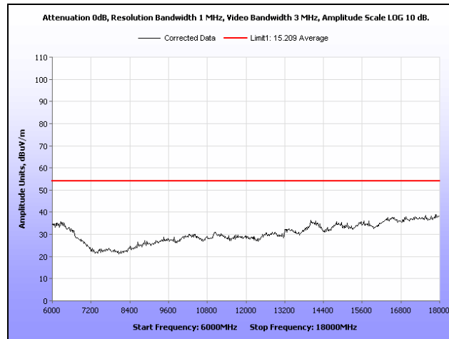
Plot 316. Radiated Spurs, Low Channel, 5.8 GHz, 802.11a, 6 GHz – 18 GHz, Peak under Avg., Sector
