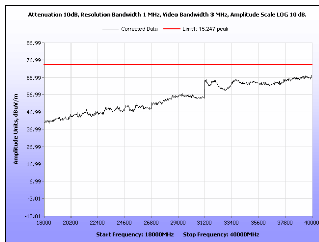
Plot 366. Radiated Spurs, High Channel, 5.8 GHz, 802.11n 40 MHz, 18 GHz – 40 GHz, Peak, Sector
