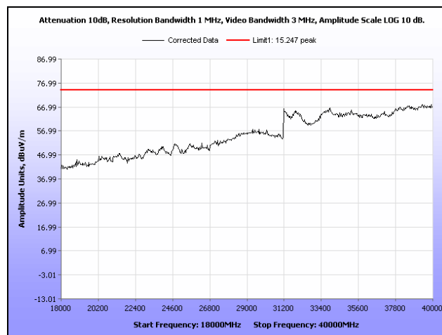
Plot 330. Radiated Spurs, High Channel, 5.8 GHz, 802.11a, 18 GHz – 40 GHz, Peak, Sector
