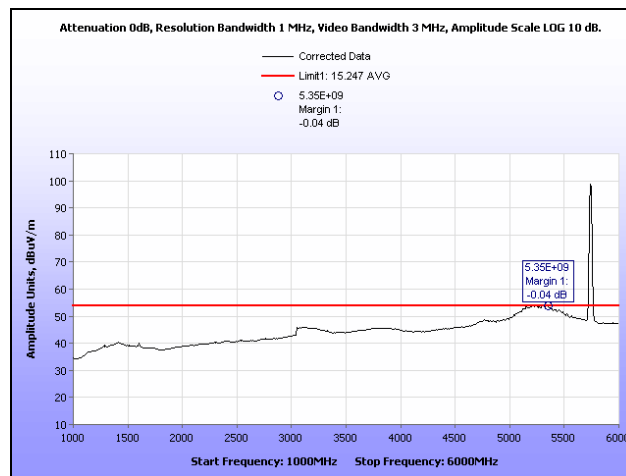
Plot 314. Radiated Spurs, Low Channel, 5.8 GHz, 802.11a, 1 GHz – 6 GHz, Average, Sector
