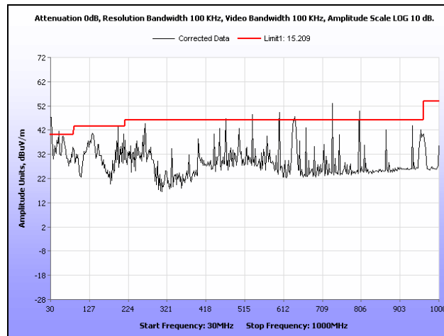
Plot 313. Radiated Spurs, Low Channel, 5.8 GHz, 802.11a, 30 MHz – 1 GHz, Sector
