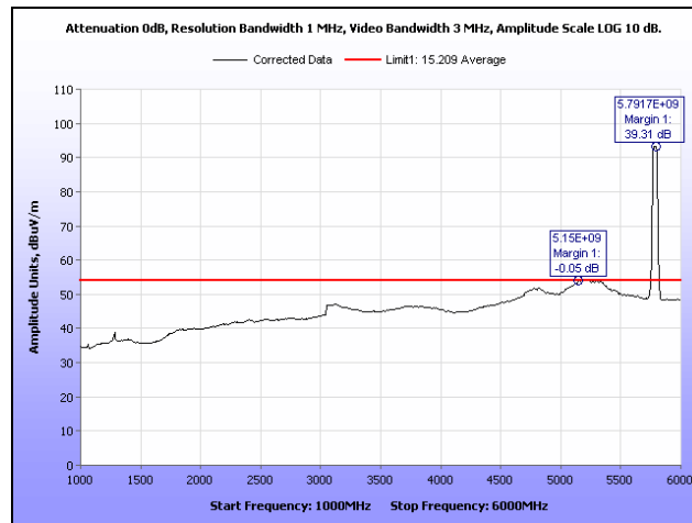
Plot 356. Radiated Spurs, Mid Channel, 5.8 GHz, 802.11n 40 MHz, 1 GHz – 6 GHz, Average, Sector
