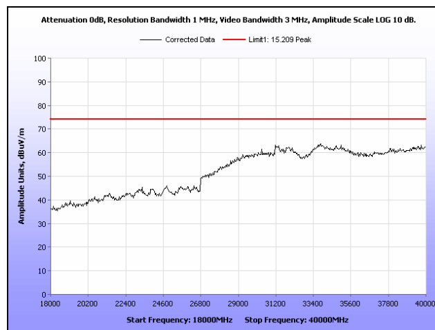
Plot 312. Radiated Spurs, High Channel, 5.8 GHz, 802.11n 40 MHz, 18 GHz – 40 GHz, Peak, Omni
