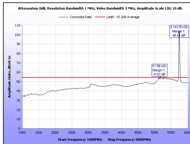
Plot 278. Radiated Spurs, Low Channel, 5.8 GHz, 802.11n 20 MHz, 1 GHz – 6 GHz, Average, Omni
