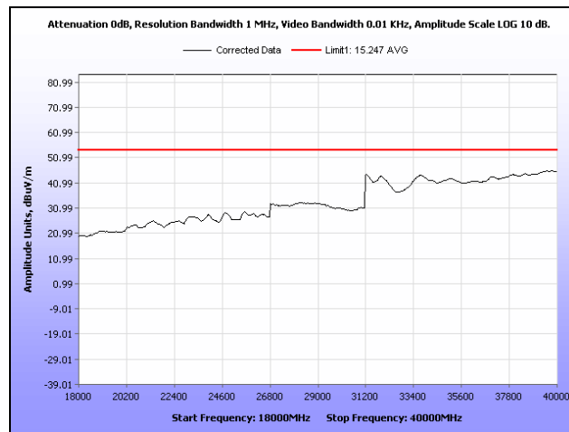
Plot 335. Radiated Spurs, Low Channel, 5.8 GHz, 802.11n 20 MHz, 18 GHz – 40 GHz, Average, Sector
