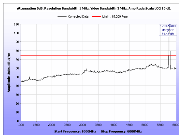
Plot 321. Radiated Spurs, Mid Channel, 5.8 GHz, 802.11a, 1 GHz – 6 GHz, Peak, Sector
