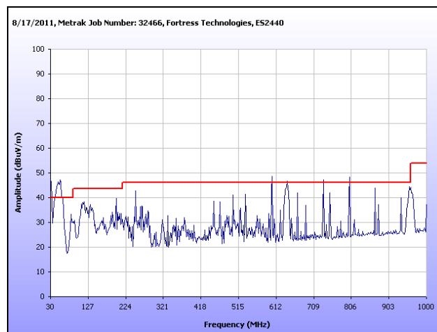
Plot 224. Radiated Spurs, High Channel, 2.4 GHz, 802.11g, 30 MHz – 1 GHz, Sector
