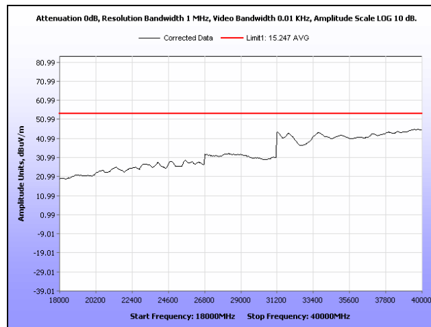
Plot 323. Radiated Spurs, Mid Channel, 5.8 GHz, 802.11a, 18 GHz – 40 GHz, Average, Sector
