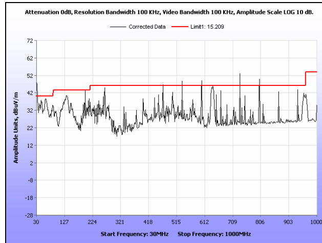
Plot 319. Radiated Spurs, Mid Channel, 5.8 GHz, 802.11a, 30 MHz – 1 GHz, Sector
