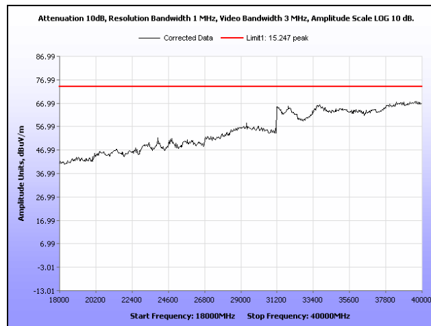
Plot 348. Radiated Spurs, High Channel, 5.8 GHz, 802.11n 20 MHz, 18 GHz – 40 GHz, Peak, Sector
