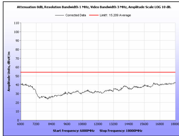
Plot 310. Radiated Spurs, High Channel, 5.8 GHz, 802.11n 40 MHz, 6 GHz – 18 GHz, Peak under Avg., Omni
