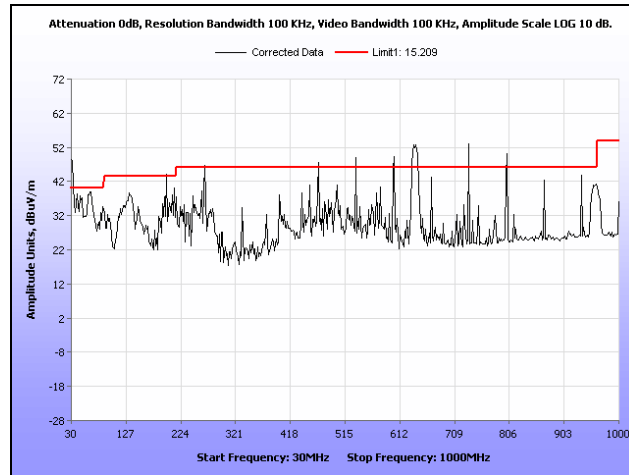
Plot 337. Radiated Spurs, Mid Channel, 5.8 GHz, 802.11n 20 MHz, 30 MHz – 1 GHz, Sector Note: Emissions which exceed the limit are digital emissions.
