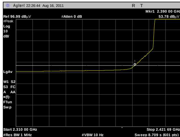
Plot 371. Radiated Restricted Band Edge, Low Channel, 2.4 GHz, 802.11g, Average, Omni
