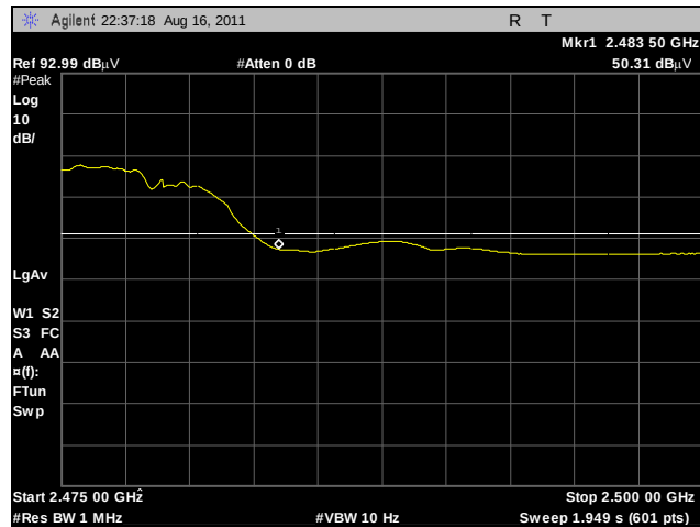
Plot 369. Radiated Restricted Band Edge, High Channel, 2.4 GHz, 802.11b, Average, Omni
