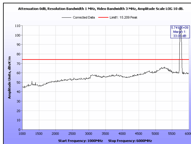
Plot 351. Radiated Spurs, Low Channel, 5.8 GHz, 802.11n 40 MHz, 1 GHz – 6 GHz, Peak, Sector
