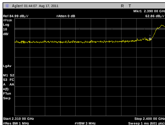
Plot 384. Radiated Restricted Band Edge, Low Channel, 2.4 GHz, 802.11b, Peak, Sector
