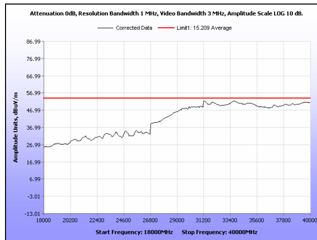
Plot 293. Radiated Spurs, High Channel, 5.8 GHz, 802.11n 20 MHz, 18 GHz – 40 GHz, Average, Omni
