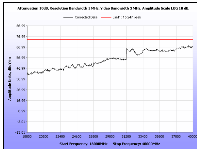
Plot 360. Radiated Spurs, Mid Channel, 5.8 GHz, 802.11n 40 MHz, 18 GHz – 40 GHz, Peak, Sector
