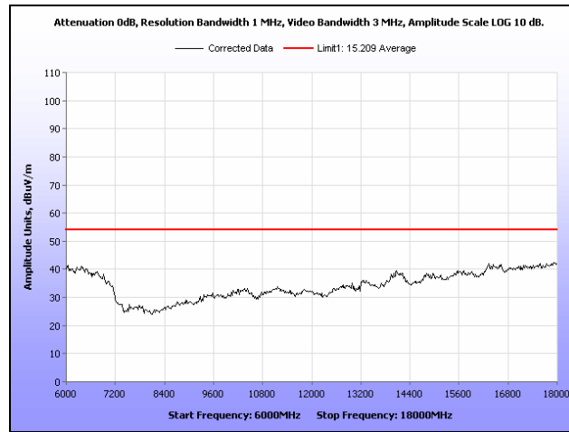
Plot 268. Radiated Spurs, Mid Channel, 5.8 GHz, 802.11a, 6 GHz – 18 GHz, Peak under Avg., Omni
