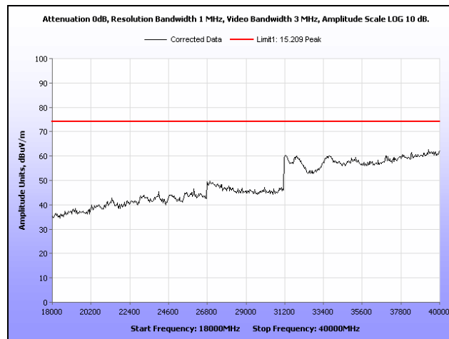
Plot 264. Radiated Spurs, Low Channel, 5.8 GHz, 802.11a, 18 GHz – 40 GHz, Peak, Omni
