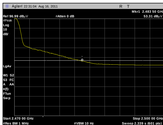
Plot 373. Radiated Restricted Band Edge, High Channel, 2.4 GHz, 802.11g, Average, Omni
