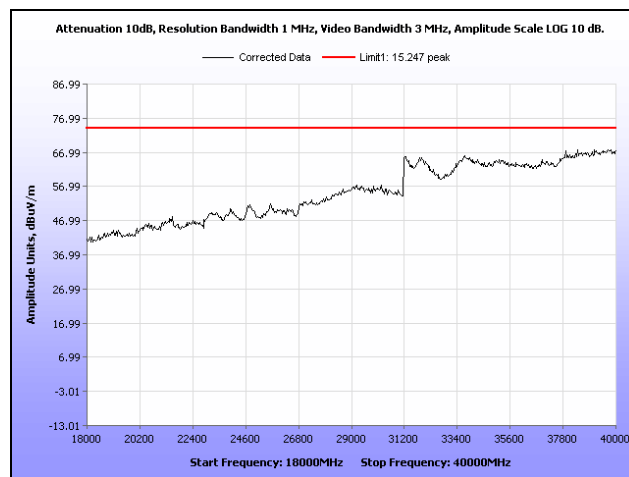
Plot 336. Radiated Spurs, Low Channel, 5.8 GHz, 802.11n 20 MHz, 18 GHz – 40 GHz, Peak, Sector
