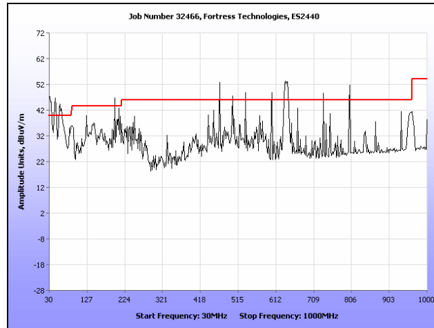
Plot 307. Radiated Spurs, High Channel, 5.8 GHz, 802.11n 40 MHz, 30 MHz – 1 GHz, Omni Note: Emissions which exceed the limit are digital emissions.
