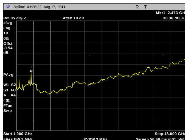
Plot 180. Radiated Spurs, High Channel, 2.4 GHz, 802.11g HT20, 1 GHz – 18 GHz, Average, Omni
