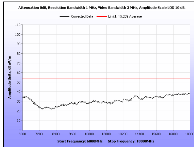
Plot 322. Radiated Spurs, Mid Channel, 5.8 GHz, 802.11a, 6 GHz – 18 GHz, Peak under Avg., Sector
