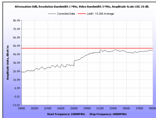
Plot 305. Radiated Spurs, Mid Channel, 5.8 GHz, 802.11n 40 MHz, 18 GHz – 40 GHz, Average, Omni
