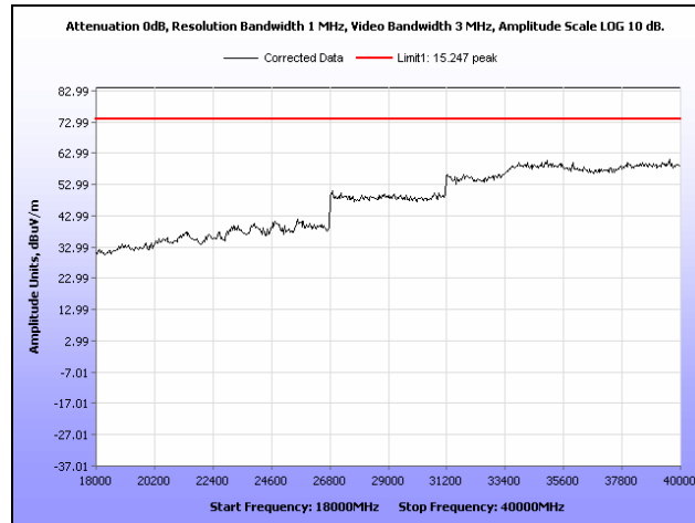
Plot 188. Radiated Spurs, Low Channel, 2.4 GHz, 802.11g HT40, 18 GHz – 40 GHz, Peak, Omni
