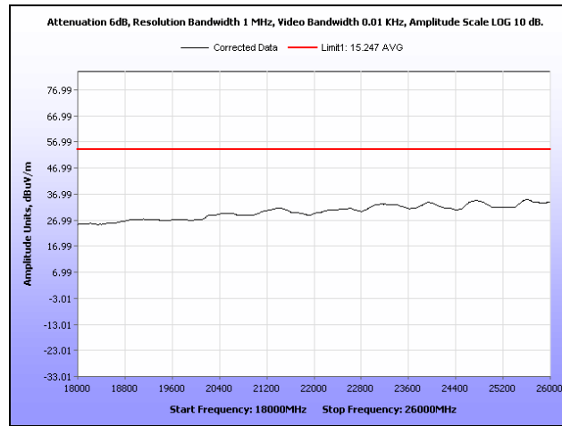
Plot 217. Radiated Spurs, Low Channel, 2.4 GHz, 802.11g, 18 GHz – 26 GHz, Average, Sector
