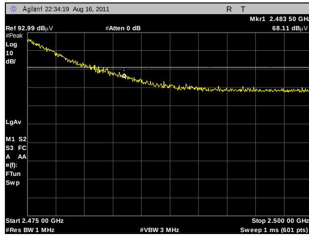
Plot 374. Radiated Restricted Band Edge, High Channel, 2.4 GHz, 802.11g, Peak, Omni
