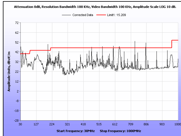
Plot 271. Radiated Spurs, High Channel, 5.8 GHz, 802.11a, 30 MHz – 1 GHz, Omni
