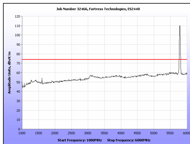
Plot 267. Radiated Spurs, Mid Channel, 5.8 GHz, 802.11a, 1 GHz – 6 GHz, Peak, Omni
