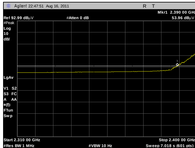
Plot 375. Radiated Restricted Band Edge, Low Channel, 2.4 GHz, 802.11g HT20, Average, Omni
