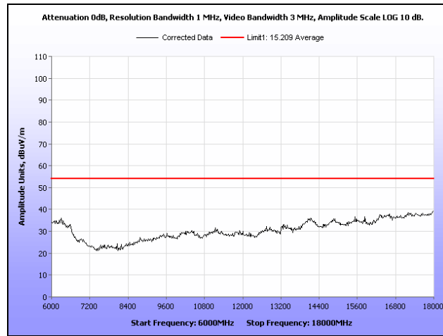
Plot 352. Radiated Spurs, Low Channel, 5.8 GHz, 802.11n 40 MHz, 6 GHz – 18 GHz, Peak under Avg., Sector
