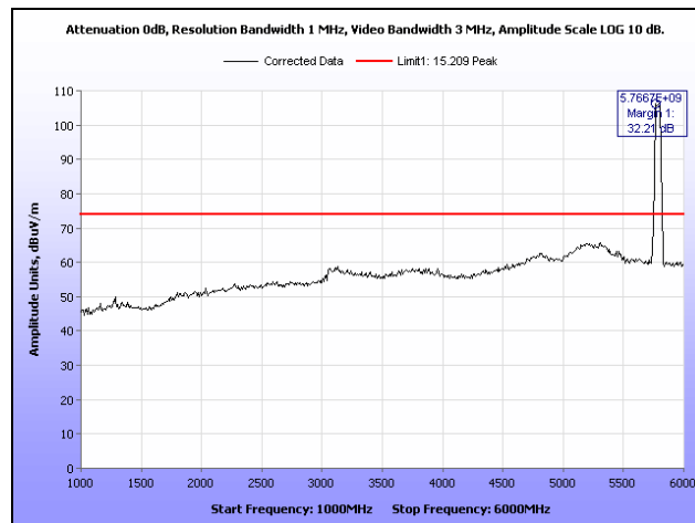
Plot 357. Radiated Spurs, Mid Channel, 5.8 GHz, 802.11n 40 MHz, 1 GHz – 6 GHz, Peak, Sector
