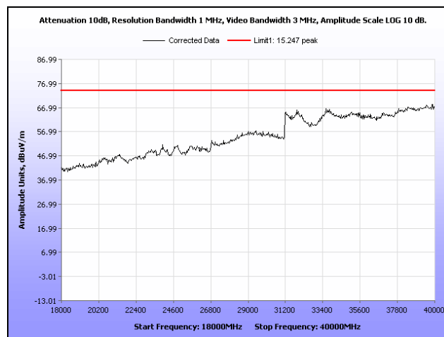
Plot 324. Radiated Spurs, Mid Channel, 5.8 GHz, 802.11a, 18 GHz – 40 GHz, Peak, Sector
