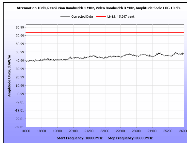
Plot 223. Radiated Spurs, Mid Channel, 2.4 GHz, 802.11g, 18 GHz – 26 GHz, Peak, Sector
