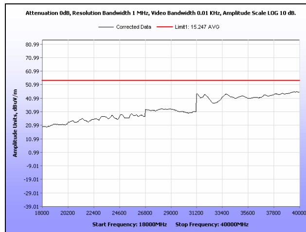
Plot 353. Radiated Spurs, Low Channel, 5.8 GHz, 802.11n 40 MHz, 18 GHz – 40 GHz, Average, Sector
