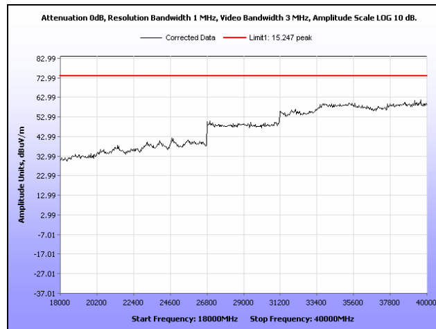
Plot 158. Radiated Spurs, Low Channel, 2.4 GHz, 802.11g, 18 GHz – 40 GHz, Peak, Omni
