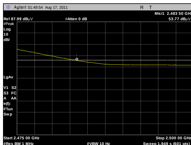
Plot 393. Radiated Restricted Band Edge, High Channel, 2.4 GHz, 802.11g HT20, Average, Sector
