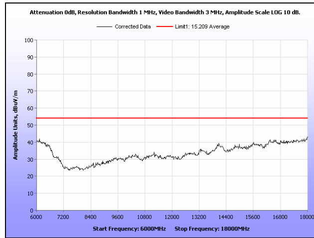
Plot 340. Radiated Spurs, Mid Channel, 5.8 GHz, 802.11n 20 MHz, 6 GHz – 18 GHz, Peak under Avg., Sector
