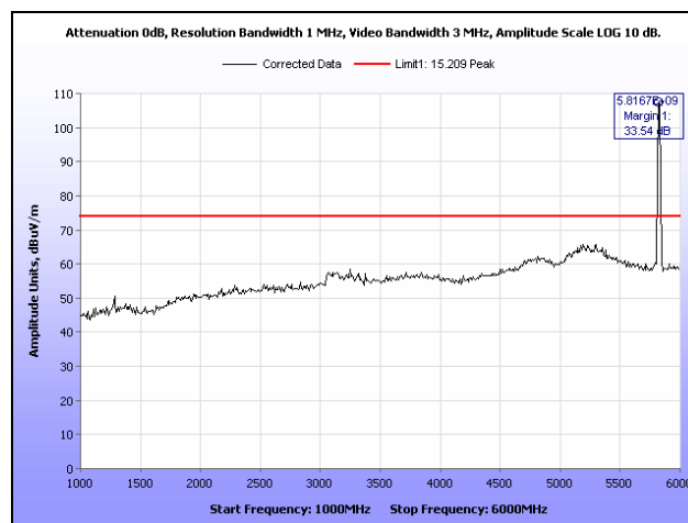
Plot 345. Radiated Spurs, High Channel, 5.8 GHz, 802.11n 20 MHz, 1 GHz – 6 GHz, Peak, Sector
