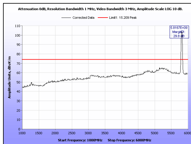
Plot 363. Radiated Spurs, High Channel, 5.8 GHz, 802.11n 40 MHz, 1 GHz – 6 GHz, Peak, Sector
