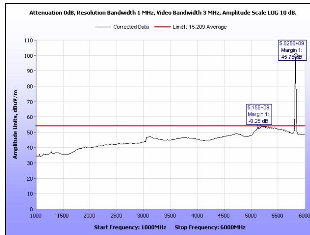
Plot 272. Radiated Spurs, High Channel, 5.8 GHz, 802.11a, 1 GHz – 6 GHz, Average, Omni
