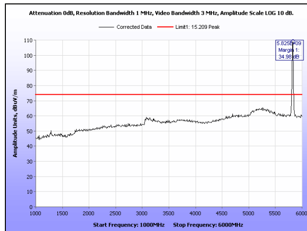
Plot 327. Radiated Spurs, High Channel, 5.8 GHz, 802.11a, 1 GHz – 6 GHz, Peak, Sector
