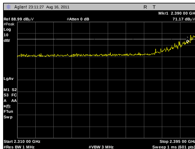
Plot 380. Radiated Restricted Band Edge, Low Channel, 2.4 GHz, 802.11g HT40, Peak, Omni
