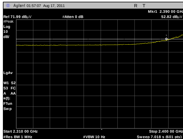
Plot 395. Radiated Restricted Band Edge, Low Channel, 2.4 GHz, 802.11g HT40, Average, Sector
