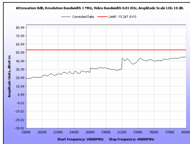
Plot 347. Radiated Spurs, High Channel, 5.8 GHz, 802.11n 20 MHz, 18 GHz – 40 GHz, Average, Sector
