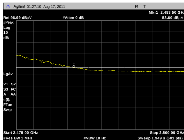
Plot 389. Radiated Restricted Band Edge, High Channel, 2.4 GHz, 802.11g, Average, Sector
