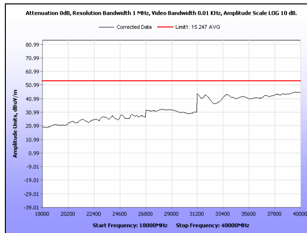
Plot 329. Radiated Spurs, High Channel, 5.8 GHz, 802.11a, 18 GHz – 40 GHz, Average, Sector
