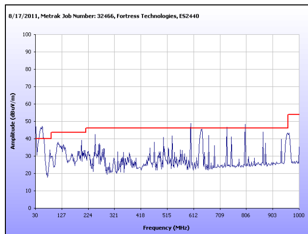
Plot 219. Radiated Spurs, Mid Channel, 2.4 GHz, 802.11g, 30 MHz – 1 GHz, Sector
