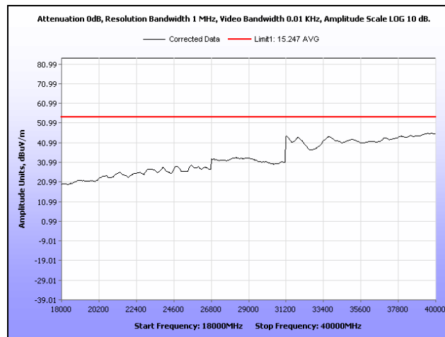
Plot 359. Radiated Spurs, Mid Channel, 5.8 GHz, 802.11n 40 MHz, 18 GHz – 40 GHz, Average, Sector
