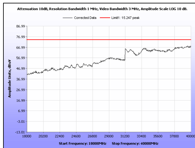
Plot 318. Radiated Spurs, Low Channel, 5.8 GHz, 802.11a, 18 GHz – 40 GHz, Peak, Sector
