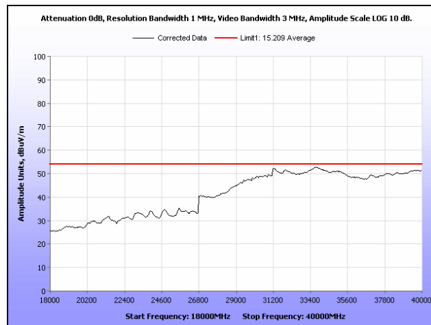
Plot 311. Radiated Spurs, High Channel, 5.8 GHz, 802.11n 40 MHz, 18 GHz – 40 GHz, Average, Omni
