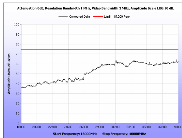
Plot 294. Radiated Spurs, High Channel, 5.8 GHz, 802.11n 20 MHz, 18 GHz – 40 GHz, Peak, Omni
