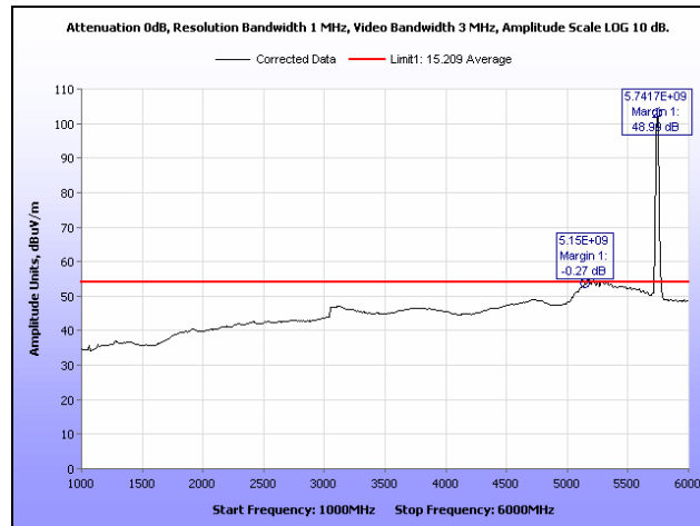
Plot 260. Radiated Spurs, Low Channel, 5.8 GHz, 802.11a, 1 GHz – 6 GHz, Average, Omni
