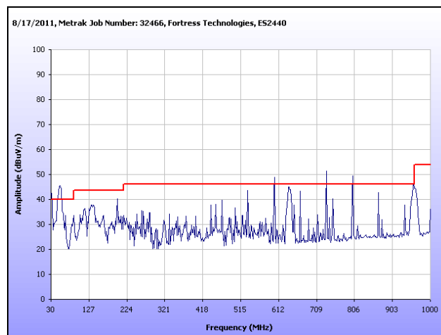
Plot 164. Radiated Spurs, High Channel, 2.4 GHz, 802.11g, 30 MHz – 1 GHz, Omni
