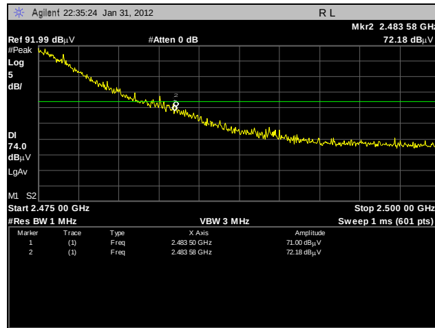
Plot 390. Radiated Restricted Band Edge, High Channel, 2.4 GHz, 802.11g, Peak, Sector
