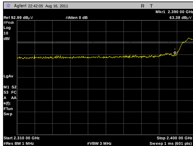
Plot 368. Radiated Restricted Band Edge, Low Channel, 2.4 GHz, 802.11b, Peak, Omni
