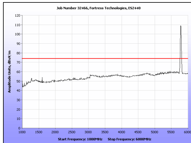
Plot 285. Radiated Spurs, Mid Channel, 5.8 GHz, 802.11n 20 MHz, 1 GHz – 6 GHz, Peak, Omni
