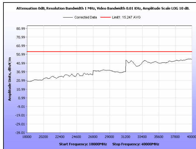
Plot 341. Radiated Spurs, Mid Channel, 5.8 GHz, 802.11n 20 MHz, 18 GHz – 40 GHz, Average, Sector
