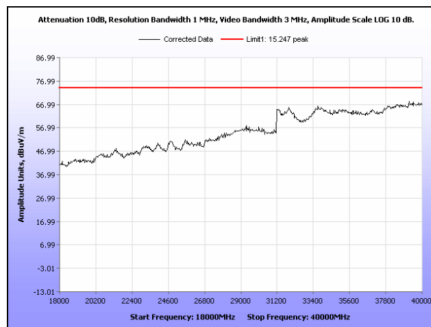
Plot 342. Radiated Spurs, Mid Channel, 5.8 GHz, 802.11n 20 MHz, 18 GHz – 40 GHz, Peak, Sector
