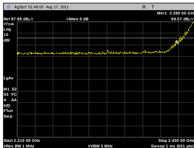
Plot 392. Radiated Restricted Band Edge, Low Channel, 2.4 GHz, 802.11g HT20, Peak, Sector
