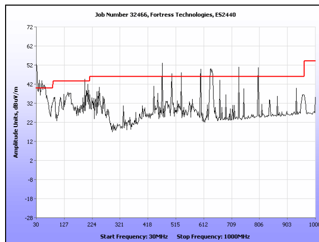
Plot 209. Radiated Spurs, High Channel, 2.4 GHz, 802.11b, 30 MHz – 1 GHz, Sector
