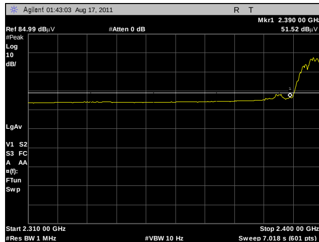
Plot 383. Radiated Restricted Band Edge, Low Channel, 2.4 GHz, 802.11b, Average, Sector
