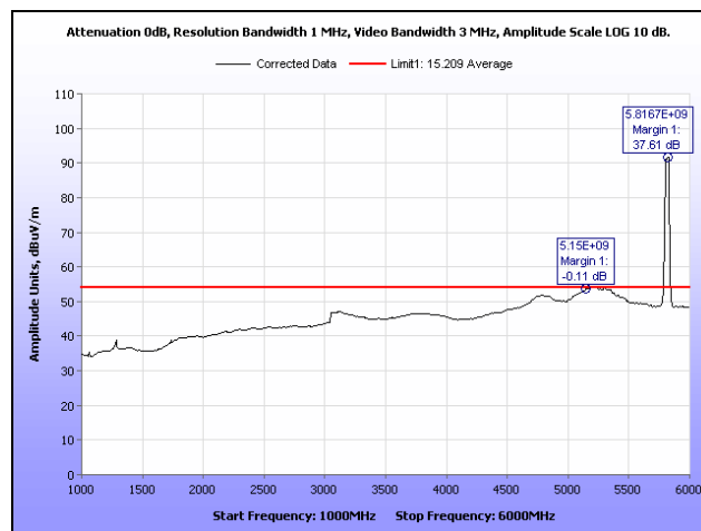
Plot 362. Radiated Spurs, High Channel, 5.8 GHz, 802.11n 40 MHz, 1 GHz – 6 GHz, Average, Sector
