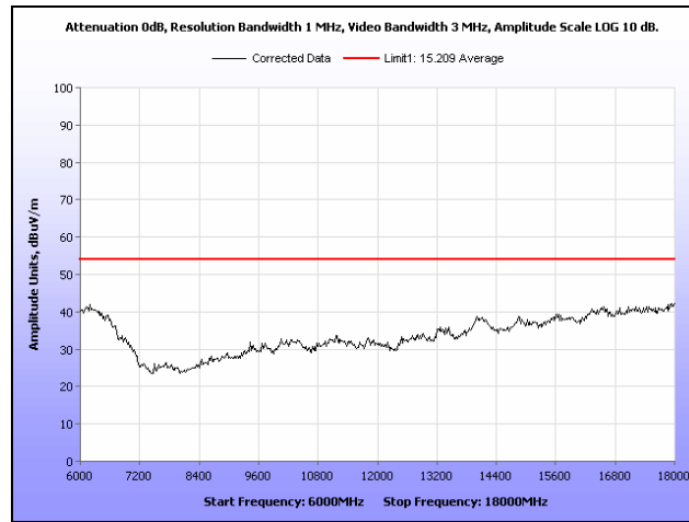
Plot 346. Radiated Spurs, High Channel, 5.8 GHz, 802.11n 20 MHz, 6 GHz – 18 GHz, Peak under Avg., Sector
