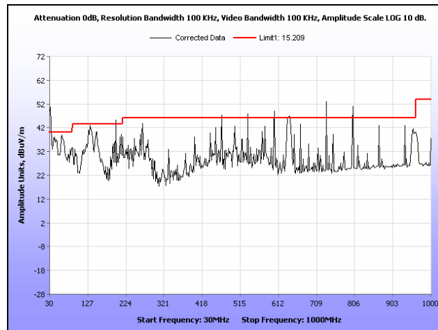
Plot 229. Radiated Spurs, Low Channel, 2.4 GHz, 802.11g HT20, 30 MHz – 1 GHz, Sector
