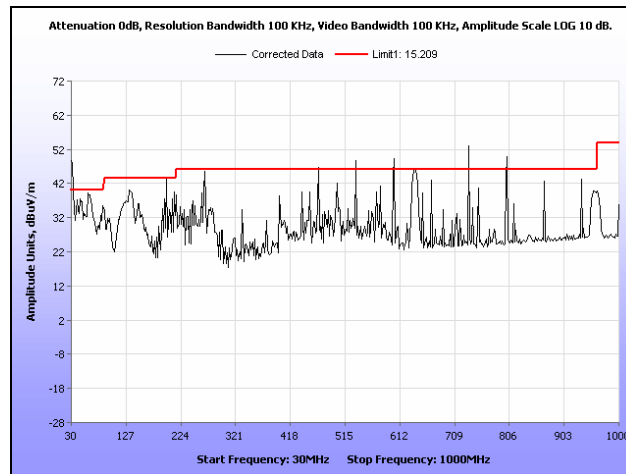
Plot 343. Radiated Spurs, High Channel, 5.8 GHz, 802.11n 20 MHz, 30 MHz – 1 GHz, Sector
