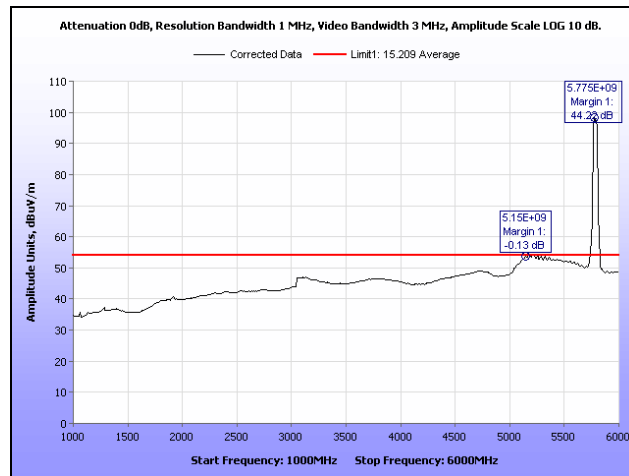
Plot 302. Radiated Spurs, Mid Channel, 5.8 GHz, 802.11n 40 MHz, 1 GHz – 6 GHz, Average, Omni
