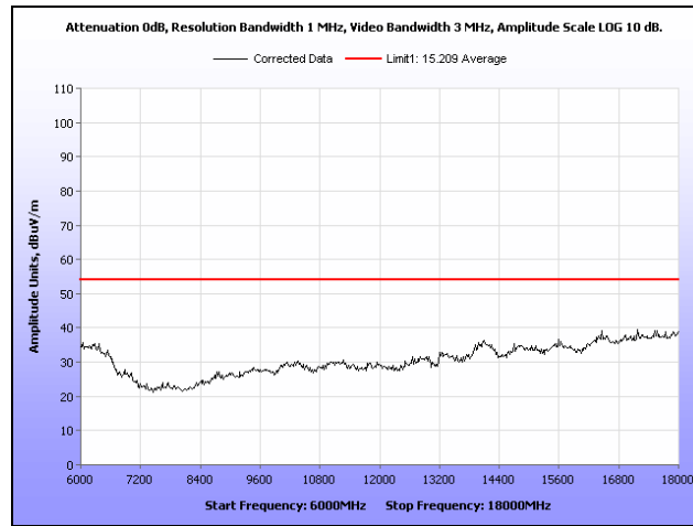
Plot 364. Radiated Spurs, High Channel, 5.8 GHz, 802.11n 40 MHz, 6 GHz – 18 GHz, Peak under Avg., Sector
