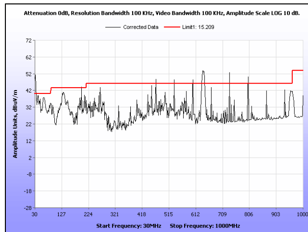
Plot 239. Radiated Spurs, High Channel, 2.4 GHz, 802.11g HT20, 30 MHz – 1 GHz, Sector
