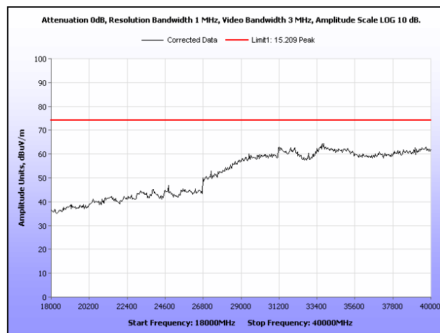
Plot 300. Radiated Spurs, Low Channel, 5.8 GHz, 802.11n 40 MHz, 18 GHz – 40 GHz, Peak, Omni
