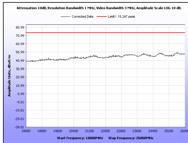
Plot 253. Radiated Spurs, Mid Channel, 2.4 GHz, 802.11g HT40, 18 GHz – 26 GHz, Peak, Sector
