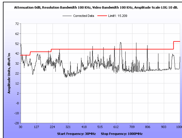
Plot 244. Radiated Spurs, Low Channel, 2.4 GHz, 802.11g HT40, 30 MHz – 1 GHz, Sector
