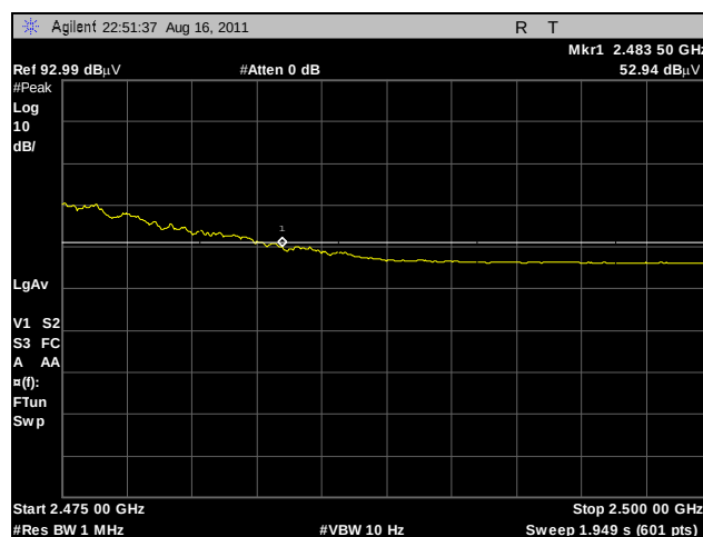
Plot 377. Radiated Restricted Band Edge, High Channel, 2.4 GHz, 802.11g HT20, Average, Omni
