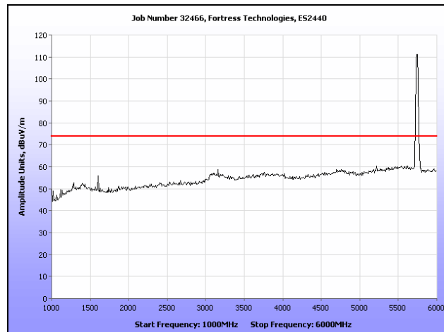
Plot 261. Radiated Spurs, Low Channel, 5.8 GHz, 802.11a, 1 GHz – 6 GHz, Peak, Omni
