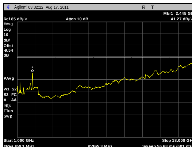
Plot 195. Radiated Spurs, High Channel, 2.4 GHz, 802.11g HT40, 1 GHz – 18 GHz, Average, Omni
