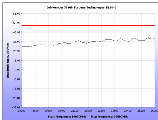
Plot 252. Radiated Spurs, Mid Channel, 2.4 GHz, 802.11g HT40, 18 GHz – 26 GHz, Average, Sector
