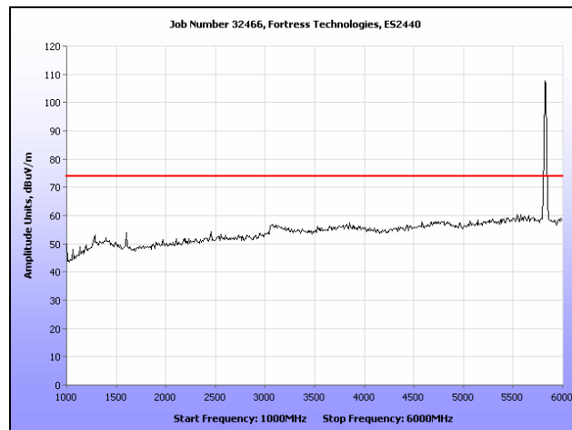
Plot 291. Radiated Spurs, High Channel, 5.8 GHz, 802.11n 20 MHz, 1 GHz – 6 GHz, Peak, Omni
