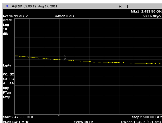
Plot 397. Radiated Restricted Band Edge, High Channel, 2.4 GHz, 802.11g HT40, Average, Sector
