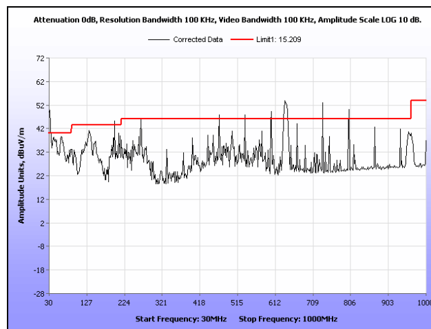
Plot 234. Radiated Spurs, Mid Channel, 2.4 GHz, 802.11g HT20, 30 MHz – 1 GHz, Sector
