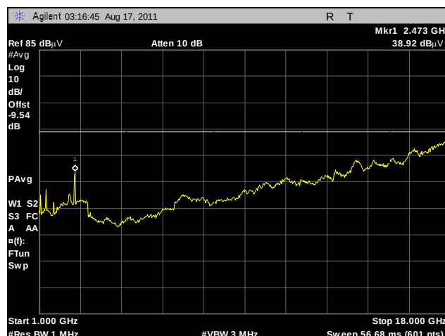
Plot 165. Radiated Spurs, High Channel, 2.4 GHz, 802.11g, 1 GHz – 18 GHz, Average, Omni
