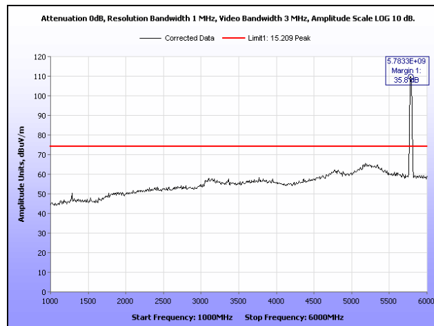
Plot 339. Radiated Spurs, Mid Channel, 5.8 GHz, 802.11n 20 MHz, 1 GHz – 6 GHz, Peak, Sector
