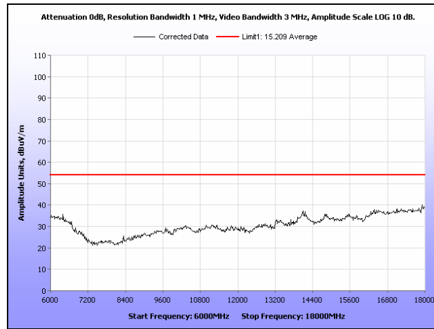
Plot 328. Radiated Spurs, High Channel, 5.8 GHz, 802.11a, 6 GHz – 18 GHz, Peak under Avg., Sector
