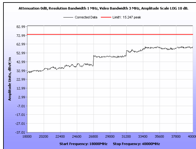
Plot 163. Radiated Spurs, Mid Channel, 2.4 GHz, 802.11g, 18 GHz – 40 GHz, Peak, Omni
