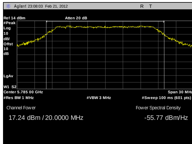
Plot 131. Peak Power Output, Mid Channel, 5.8 GHz, 802.11n 20 MHz, Port B, Sector Antenna
