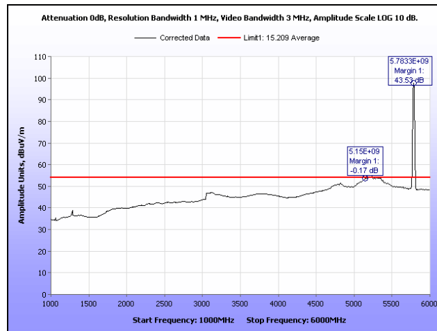
Plot 338. Radiated Spurs, Mid Channel, 5.8 GHz, 802.11n 20 MHz, 1 GHz – 6 GHz, Average, Sector
