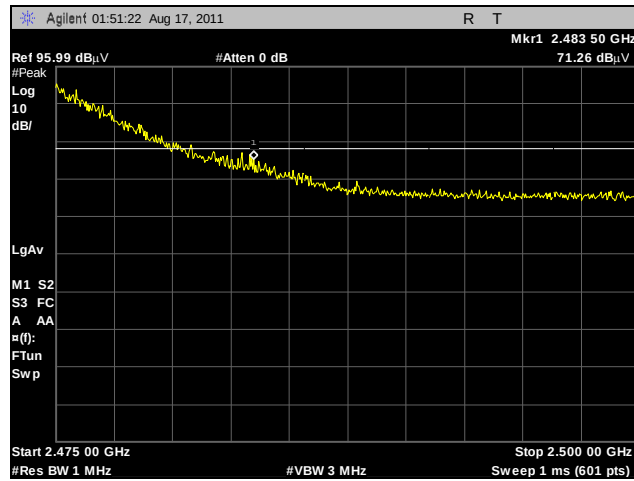
Plot 394. Radiated Restricted Band Edge, High Channel, 2.4 GHz, 802.11g HT20, Peak, Sector
