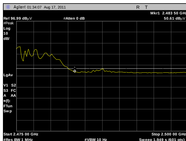
Plot 385. Radiated Restricted Band Edge, High Channel, 2.4 GHz, 802.11b, Average, Sector
