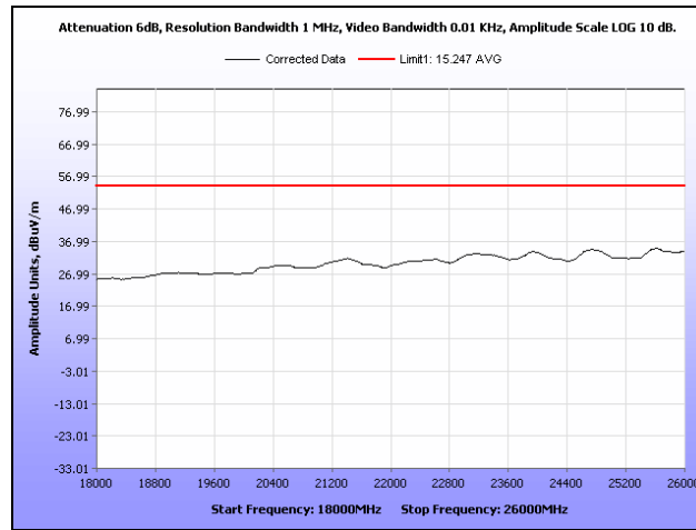
Plot 232. Radiated Spurs, Low Channel, 2.4 GHz, 802.11g HT20, 18 GHz – 26 GHz, Average, Sector
