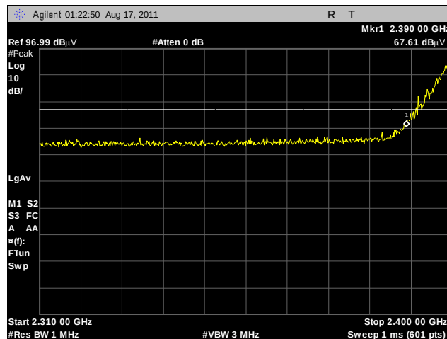
Plot 388. Radiated Restricted Band Edge, Low Channel, 2.4 GHz, 802.11g, Peak, Sector
