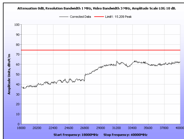
Plot 306. Radiated Spurs, Mid Channel, 5.8 GHz, 802.11n 40 MHz, 18 GHz – 40 GHz, Peak, Omni
