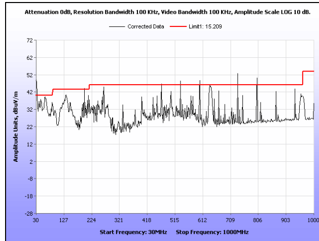
Plot 325. Radiated Spurs, High Channel, 5.8 GHz, 802.11a, 30 MHz – 1 GHz, Sector
