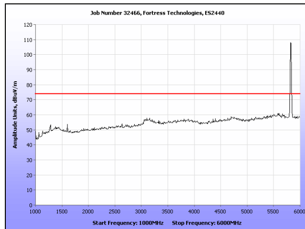
Plot 273. Radiated Spurs, High Channel, 5.8 GHz, 802.11a, 1 GHz – 6 GHz, Peak, Omni
