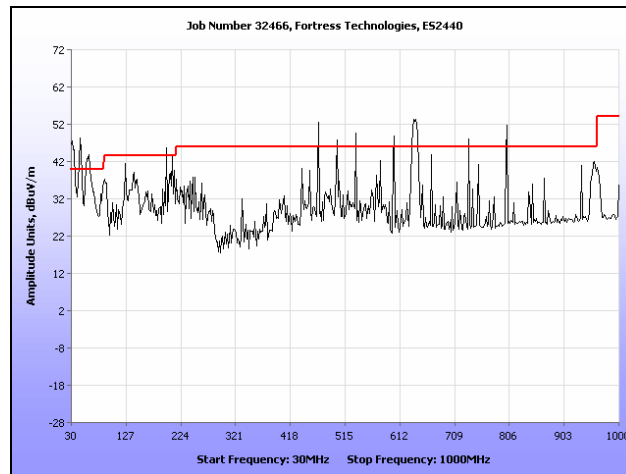
Plot 295. Radiated Spurs, Low Channel, 5.8 GHz, 802.11n 40 MHz, 30 MHz – 1 GHz, Omni
