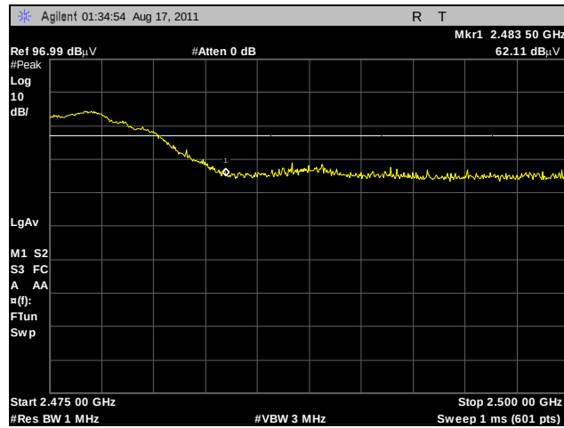
Plot 386. Radiated Restricted Band Edge, High Channel, 2.4 GHz, 802.11b, Peak, Sector
