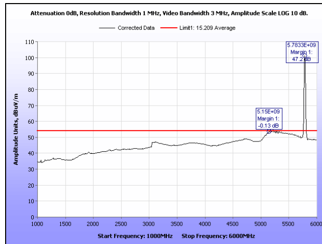
Plot 284. Radiated Spurs, Mid Channel, 5.8 GHz, 802.11n 20 MHz, 1 GHz – 6 GHz, Average, Omni
