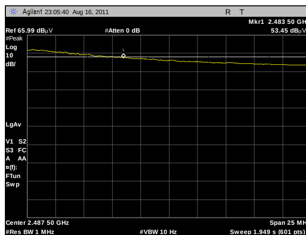
Plot 381. Radiated Restricted Band Edge, High Channel, 2.4 GHz, 802.11g HT40, Average, Omni
