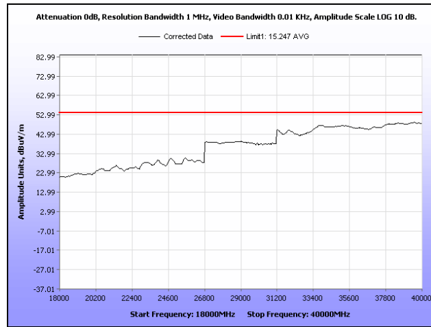
Plot 187. Radiated Spurs, Low Channel, 2.4 GHz, 802.11g HT40, 18 GHz – 40 GHz, Average, Omni
