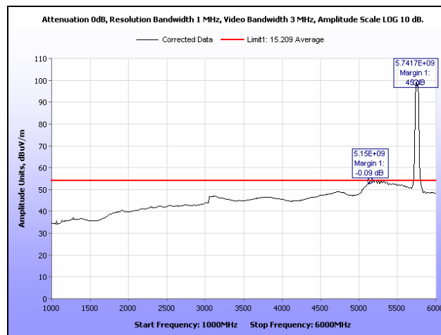
Plot 296. Radiated Spurs, Low Channel, 5.8 GHz, 802.11n 40 MHz, 1 GHz – 6 GHz, Average, Omni
