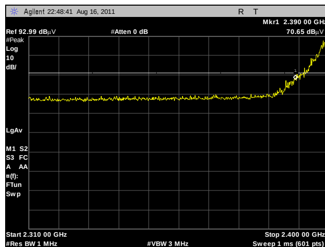
Plot 376. Radiated Restricted Band Edge, Low Channel, 2.4 GHz, 802.11g HT20, Peak, Omni
