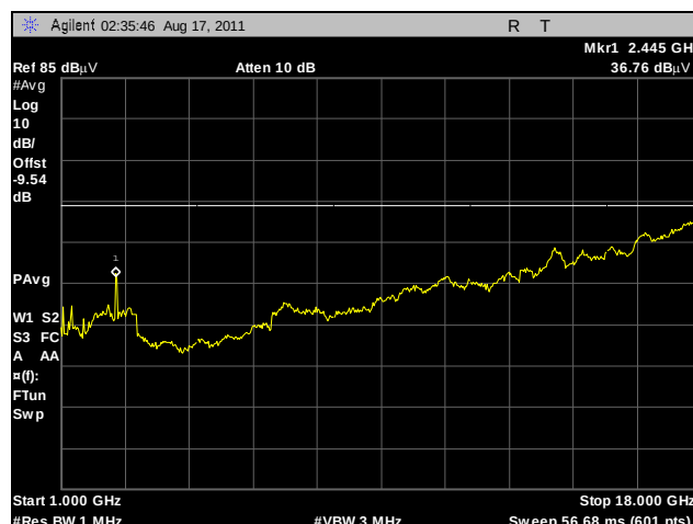
Plot 210. Radiated Spurs, High Channel, 2.4 GHz, 802.11b, 1 GHz – 18 GHz, Average, Sector
