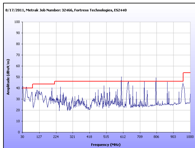
Plot 194. Radiated Spurs, High Channel, 2.4 GHz, 802.11g HT40, 30 MHz – 1 GHz, Omni
