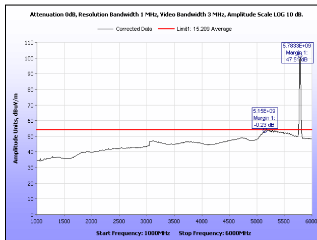
Plot 266. Radiated Spurs, Mid Channel, 5.8 GHz, 802.11a, 1 GHz – 6 GHz, Average, Omni
