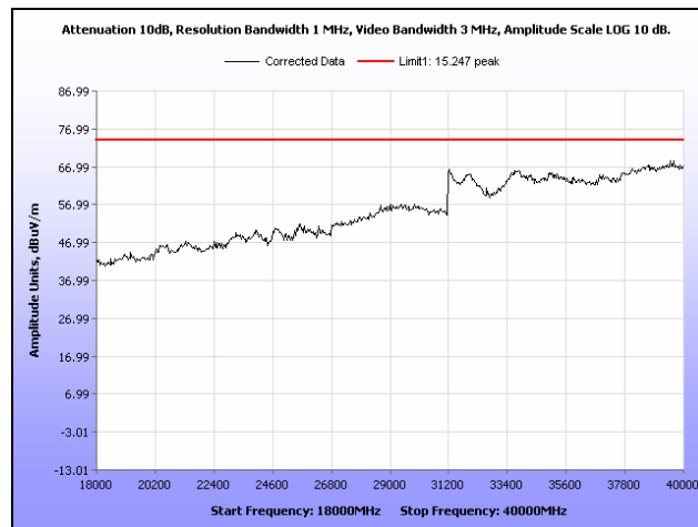
Plot 354. Radiated Spurs, Low Channel, 5.8 GHz, 802.11n 40 MHz, 18 GHz – 40 GHz, Peak, Sector
