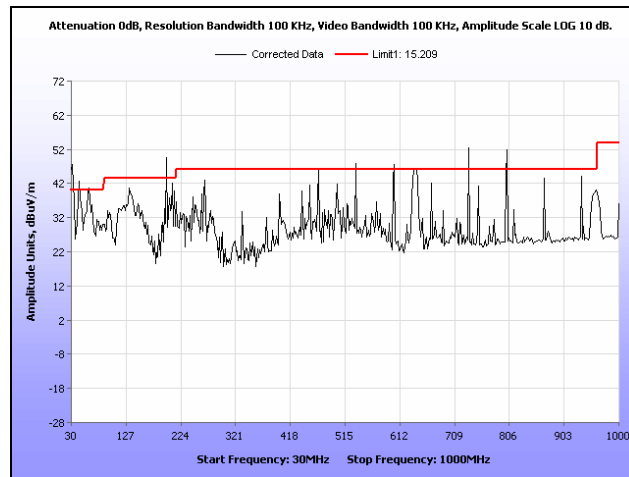
Plot 259. Radiated Spurs, Low Channel, 5.8 GHz, 802.11a, 30 MHz – 1 GHz, Omni
