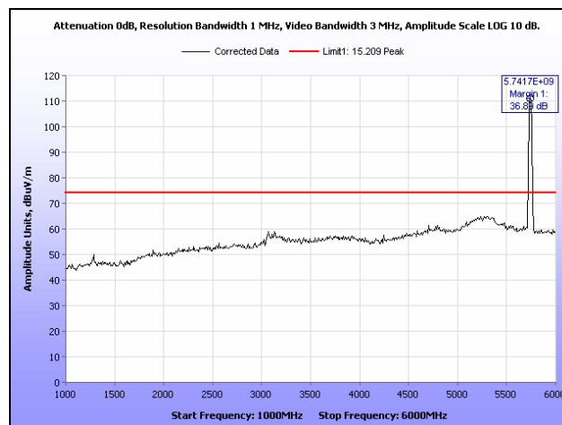
Plot 333. Radiated Spurs, Low Channel, 5.8 GHz, 802.11n 20 MHz, 1 GHz – 6 GHz, Peak, Sector
