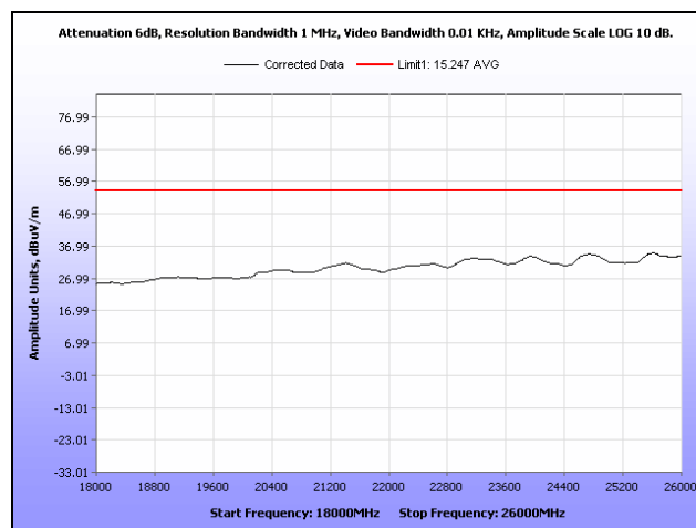
Plot 207. Radiated Spurs, Mid Channel, 2.4 GHz, 802.11b, 18 GHz – 26 GHz, Average, Sector
