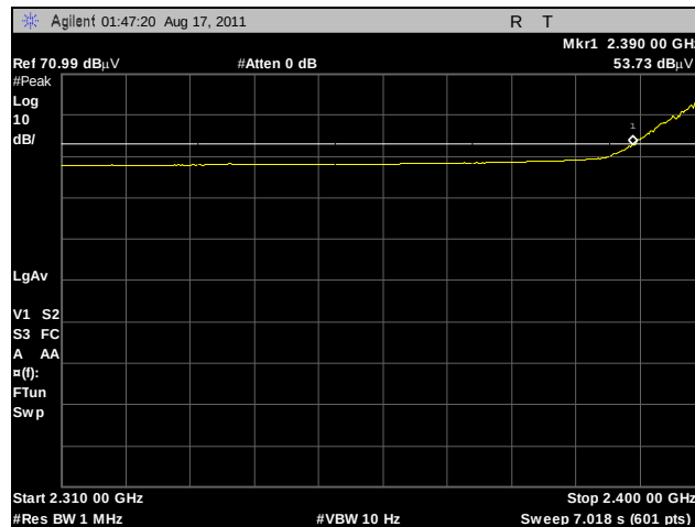
Plot 391. Radiated Restricted Band Edge, Low Channel, 2.4 GHz, 802.11g HT20, Average, Sector
