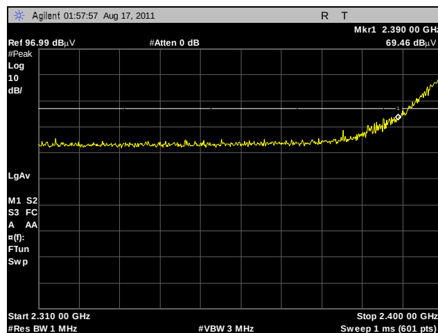
Plot 396. Radiated Restricted Band Edge, Low Channel, 2.4 GHz, 802.11g HT40, Peak, Sector
