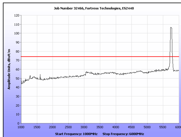
Plot 297. Radiated Spurs, Low Channel, 5.8 GHz, 802.11n 40 MHz, 1 GHz – 6 GHz, Peak, Omni
