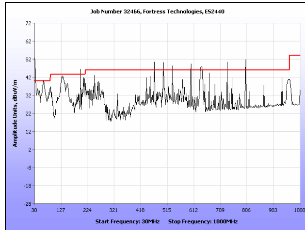
Plot 355. Radiated Spurs, Mid Channel, 5.8 GHz, 802.11n 40 MHz, 30 MHz – 1 GHz, Sector Note: Emissions which exceed the limit are digital emissions.
