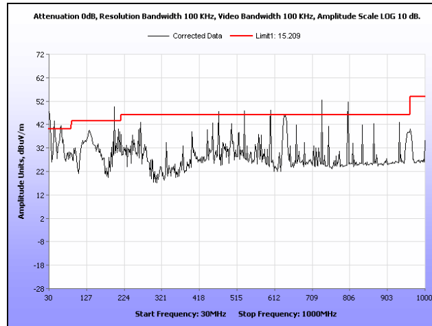
Plot 283. Radiated Spurs, Mid Channel, 5.8 GHz, 802.11n 20 MHz, 30 MHz – 1 GHz, Omni Note: Emissions which exceed the limit are digital emissions.
