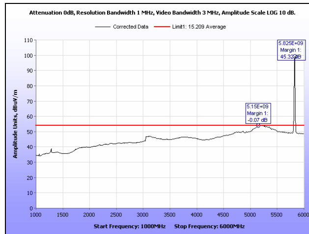
Plot 326. Radiated Spurs, High Channel, 5.8 GHz, 802.11a, 1 GHz – 6 GHz, Average, Sector
