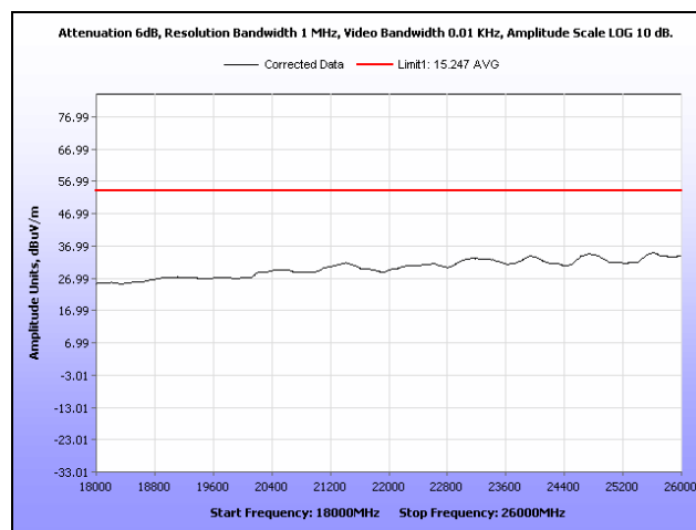
Plot 222. Radiated Spurs, Mid Channel, 2.4 GHz, 802.11g, 18 GHz – 26 GHz, Average, Sector
