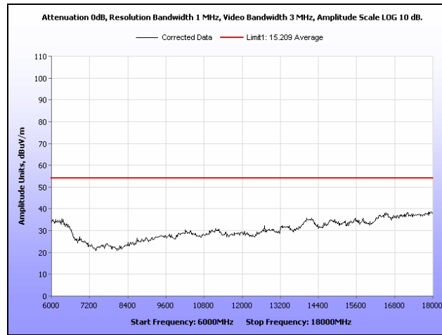
Plot 358. Radiated Spurs, Mid Channel, 5.8 GHz, 802.11n 40 MHz, 6 GHz – 18 GHz, Peak under Avg., Sector
