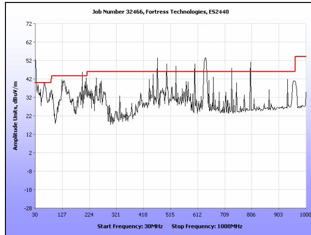
Plot 361. Radiated Spurs, High Channel, 5.8 GHz, 802.11n 40 MHz, 30 MHz – 1 GHz, Sector Note: Emissions which exceed the limit are digital emissions.
