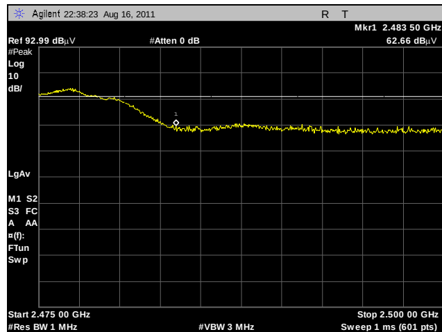
Plot 370. Radiated Restricted Band Edge, High Channel, 2.4 GHz, 802.11b, Peak, Omni
