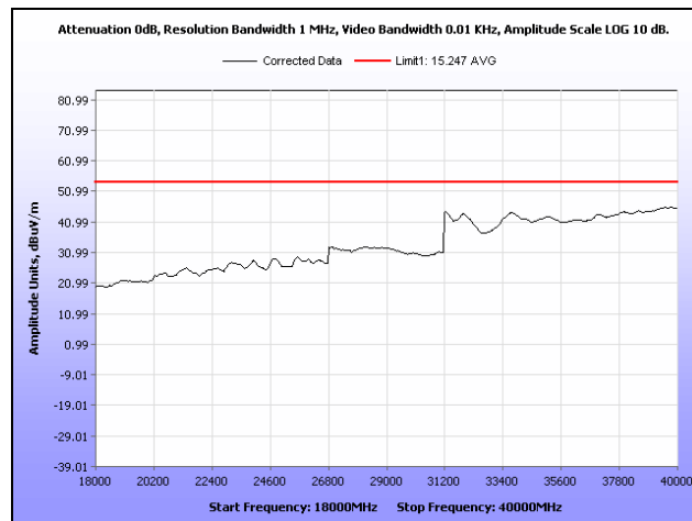
Plot 317. Radiated Spurs, Low Channel, 5.8 GHz, 802.11a, 18 GHz – 40 GHz, Average, Sector
