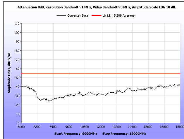
Plot 292. Radiated Spurs, High Channel, 5.8 GHz, 802.11n 20 MHz, 6 GHz – 18 GHz, Peak under Avg., Omni
