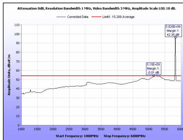
Plot 344. Radiated Spurs, High Channel, 5.8 GHz, 802.11n 20 MHz, 1 GHz – 6 GHz, Average, Sector
