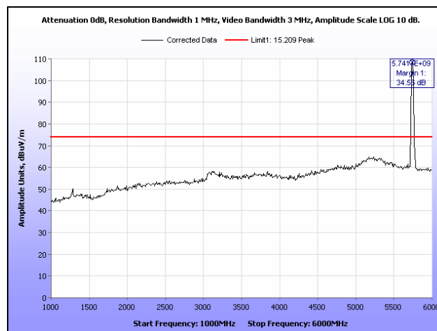
Plot 315. Radiated Spurs, Low Channel, 5.8 GHz, 802.11a, 1 GHz – 6 GHz, Peak, Sector
