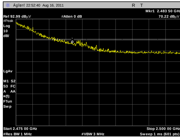
Plot 378. Radiated Restricted Band Edge, High Channel, 2.4 GHz, 802.11g HT20, Peak, Omni
