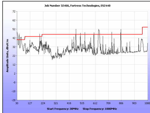
Plot 301. Radiated Spurs, Mid Channel, 5.8 GHz, 802.11n 40 MHz, 30 MHz – 1 GHz, Omni Note: Emissions which exceed the limit are digital emissions.
