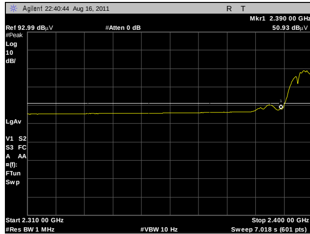
Plot 367. Radiated Restricted Band Edge, Low Channel, 2.4 GHz, 802.11b, Average, Omni
