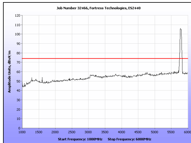
Plot 303. Radiated Spurs, Mid Channel, 5.8 GHz, 802.11n 40 MHz, 1 GHz – 6 GHz, Peak, Omni
