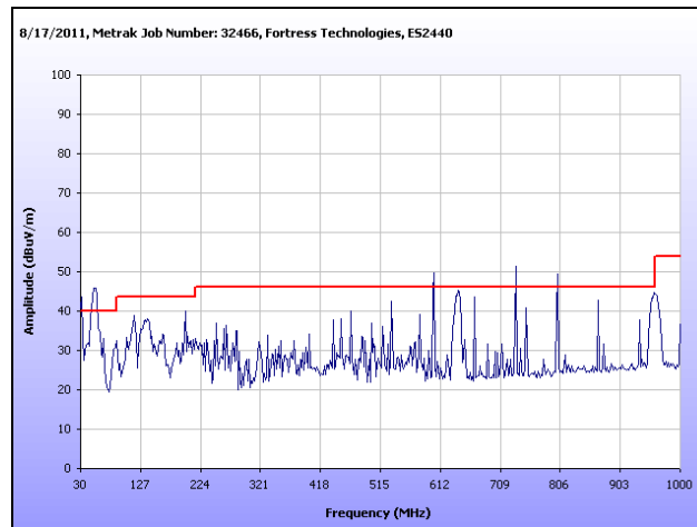
Plot 154. Radiated Spurs, Low Channel, 2.4 GHz, 802.11g, 30 MHz – 1 GHz, Omni
