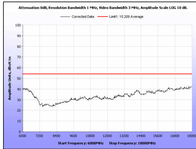
Plot 334. Radiated Spurs, Low Channel, 5.8 GHz, 802.11n 20 MHz, 6 GHz – 18 GHz, Peak under Avg., Sector
