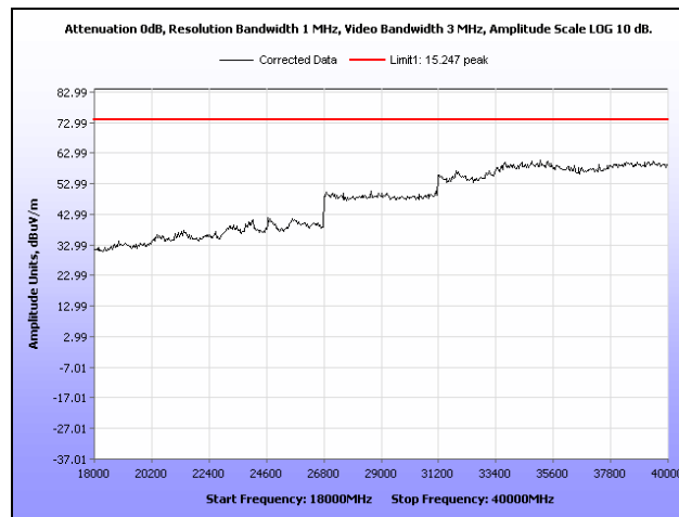
Plot 193. Radiated Spurs, Mid Channel, 2.4 GHz, 802.11g HT40, 18 GHz – 40 GHz, Peak, Omni
