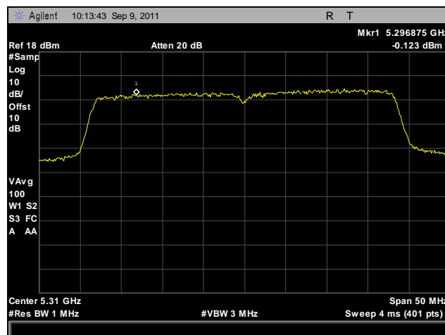
Plot 152. Peak Spectral Density, 802.11n 40 MHz, Port B, 5310 MHz
