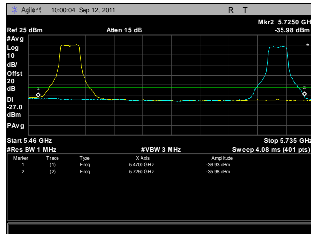
Plot 446. Frequency Stability, 802.11n 20 MHz, 5470 MHz – 5725 MHz @ 20°C, 120 V
