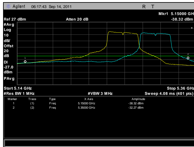
Plot 453. Frequency Stability, 802.11n 40 MHz, 5250 MHz – 5350 MHz @ -10°C, 120 V
