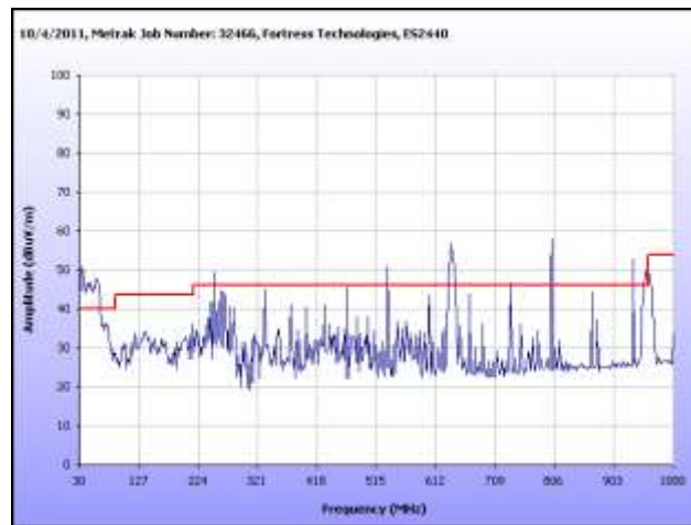
Plot 340. Radiated Spurious, 802.11n 40 MHz, 5300 MHz, 30 MHz – 1 GHz, Sector Antenna
