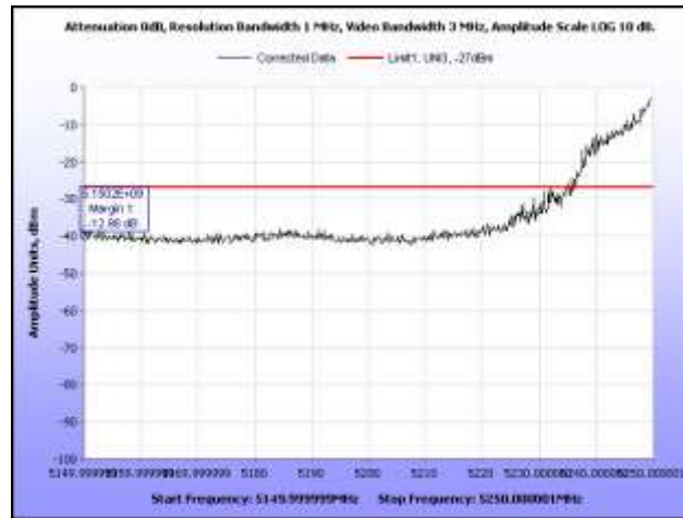
Plot 360. EIRP, 802.11a, 5260 MHz, Band Edge, Omni Antenna
