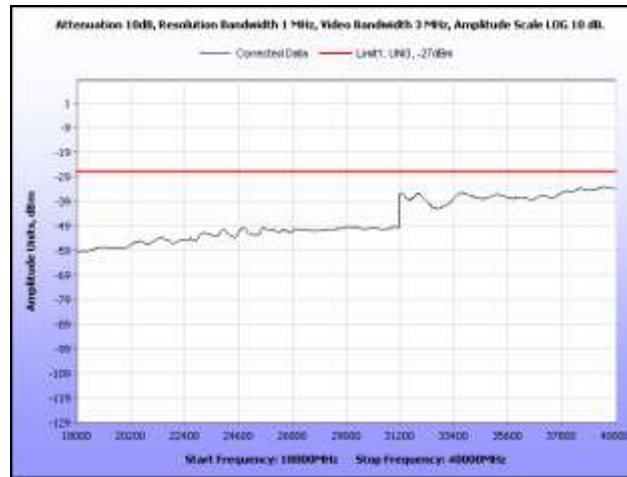
Plot 315. Radiated Spurious, 802.11n 20 MHz, 5260 MHz, 18 GHz – 40 GHz, Sector Antenna
