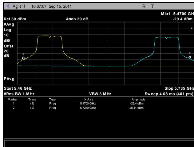
Plot 471. Frequency Stability, 802.11n 40 MHz, 5470 MHz – 5725 MHz @ 40°C, 120 V
