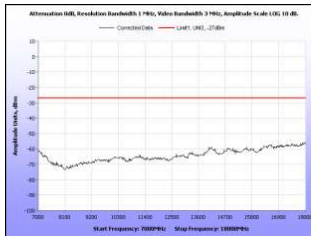
Plot 350. Radiated Spurious, 802.11n 40 MHz, 5510 MHz, 7 GHz – 18 GHz, Sector Antenna
