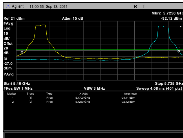
Plot 419. Frequency Stability, 802.11a, 5470 MHz – 5725 MHz @ -20°C, 120 V
