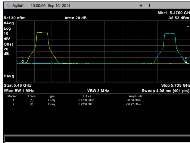
Plot 427. Frequency Stability, 802.11a, 5470 MHz – 5725 MHz @ 40°C, 120 V
