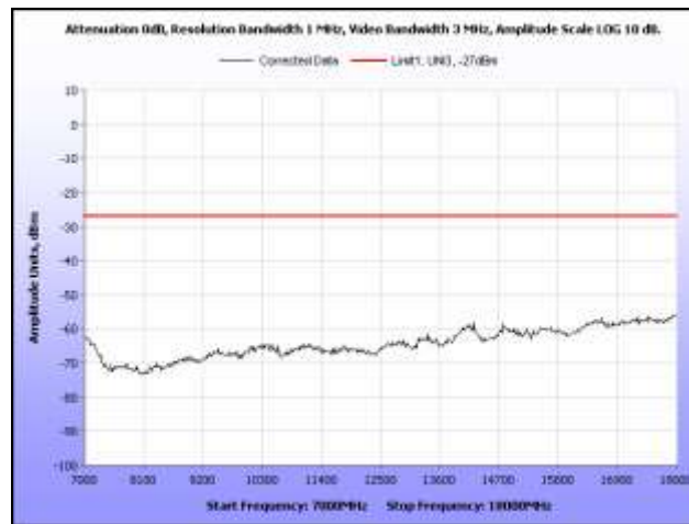
Plot 310. Radiated Spurious, 802.11a, 5700 MHz, 7 GHz – 18 GHz, Sector Antenna
