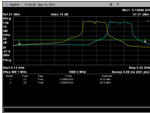
Plot 455. Frequency Stability, 802.11n 40 MHz, 5250 MHz – 5350 MHz @ 10°C, 120 V
