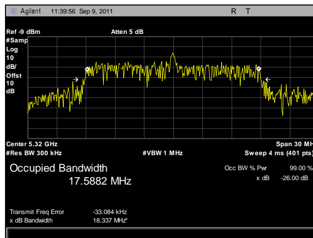
Plot 50. 99% Occupied Bandwidth, 802.11n 20 MHz, Port B, 5320 MHz
