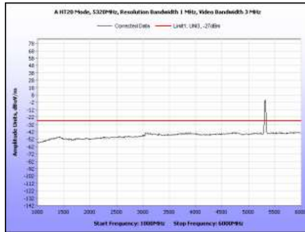
Plot 249. Radiated Spurious, 802.11n 20 MHz, 5320 MHz, 1 GHz – 6 GHz, Omni Antenna
