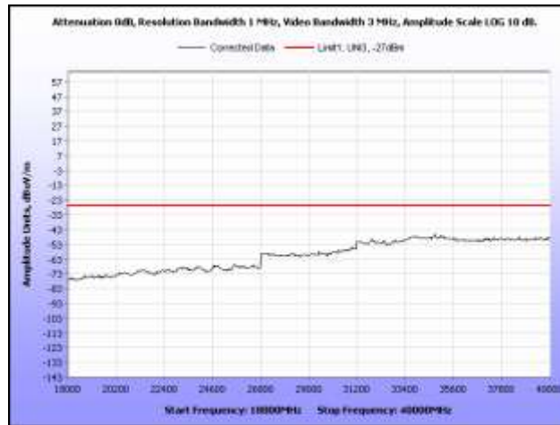
Plot 271. Radiated Spurious, 802.11n 40 MHz, 5300 MHz, 18 GHz – 40 GHz, Omni Antenna
