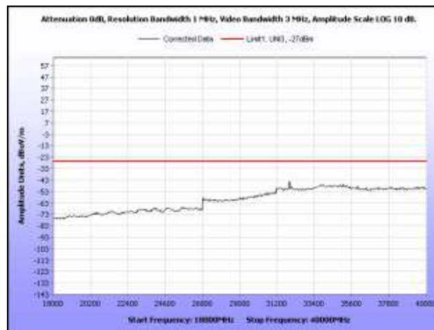
Plot 227. Radiated Spurious, 802.11a, 5320 MHz, 18 GHz – 40 GHz, Omni Antenna
