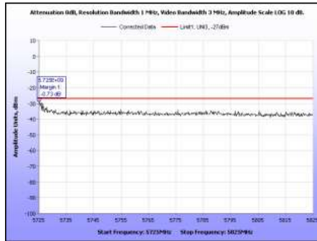
Plot 379. EIRP, 802.11n 20 MHz, 5700 MHz, Band Edge, Sector Antenna
