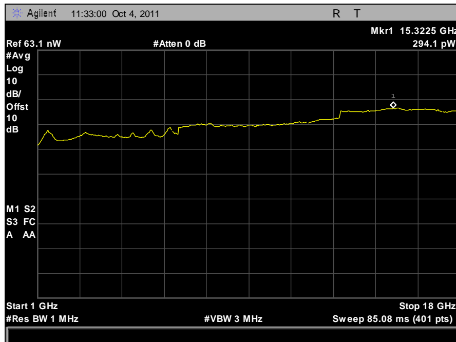
Plot 475. Receiver Spurious Emission, 1 GHz – 18 GHz, Port A
