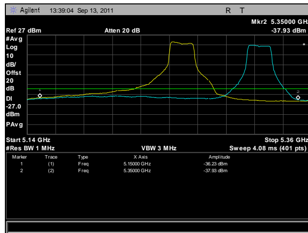
Plot 431. Frequency Stability, 802.11n 20 MHz, 5250 MHz – 5350 MHz @ -10°C, 120 V
