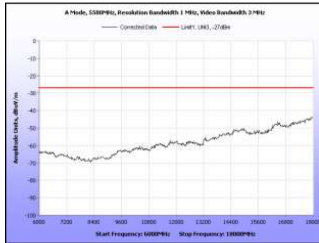
Plot 234. Radiated Spurious, 802.11a, 5580 MHz, 6 GHz – 18 GHz, Omni Antenna
