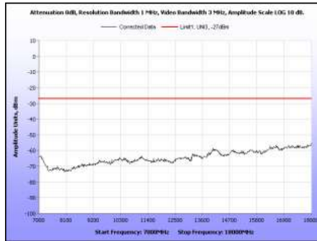
Plot 294. Radiated Spurious, 802.11a, 5300 MHz, 7 GHz – 18 GHz, Sector Antenna
