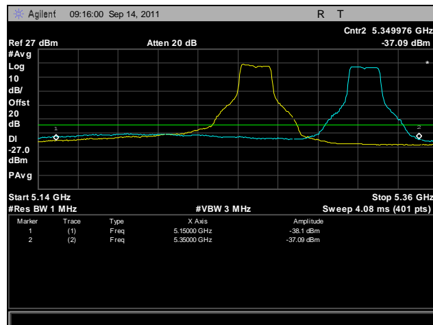
Plot 410. Frequency Stability, 802.11a, 5250 MHz – 5350 MHz @ 0°C, 120 V
