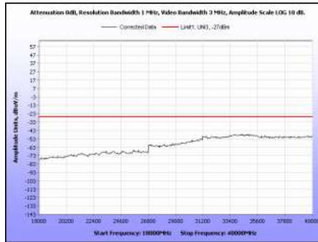
Plot 219. Radiated Spurious, 802.11a, 5260 MHz, 18 GHz – 40 GHz, Omni Antenna
