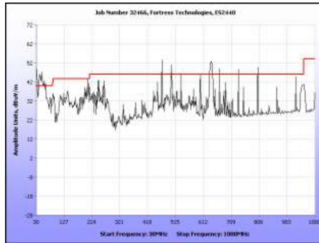
Plot 300. Radiated Spurious, 802.11a, 5500 MHz, 30 MHz – 1 GHz, Sector Antenna
