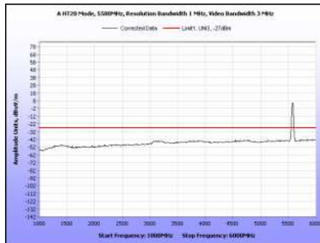
Plot 257. Radiated Spurious, 802.11n 20 MHz, 5580 MHz, 1 GHz – 6 GHz, Omni Antenna
