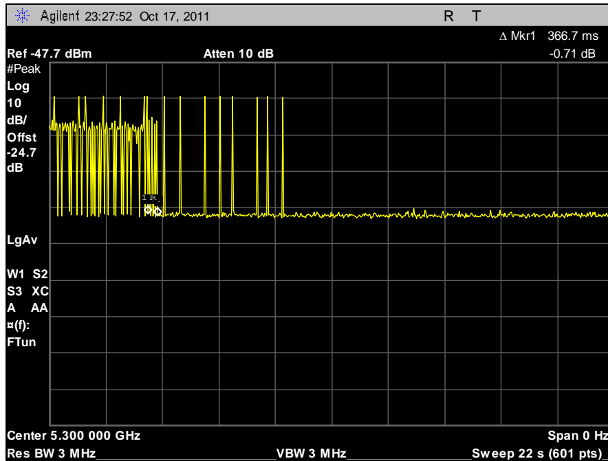
Plot 488. Channel Move Time, Bin 5
