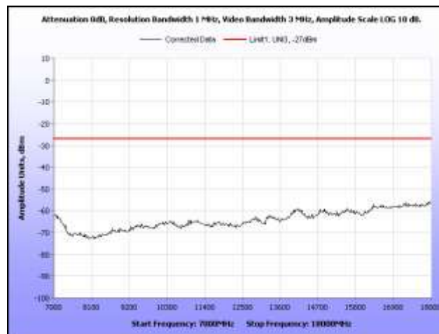
Plot 326. Radiated Spurious, 802.11n 20 MHz, 5500 MHz, 7 GHz – 18 GHz, Sector Antenna
