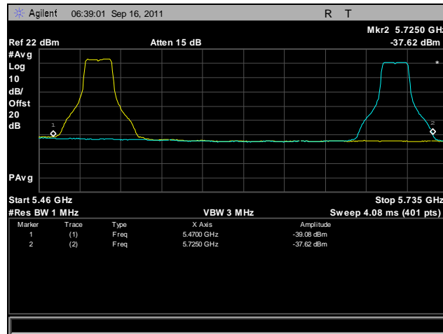
Plot 451. Frequency Stability, 802.11n 20 MHz, 5470 MHz – 5725 MHz @ 55°C, 120 V
