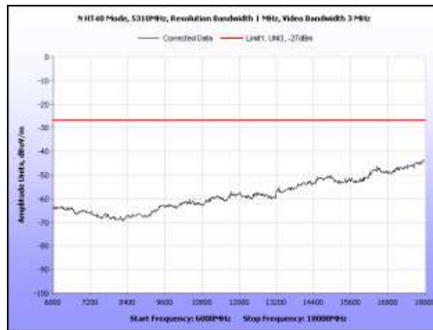
Plot 274. Radiated Spurious, 802.11n 40 MHz, 5310 MHz, 6 GHz – 18 GHz, Omni Antenna
