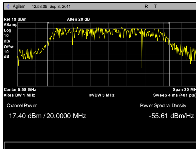
Plot 82. Conducted Output Power, 802.11n 20 MHz, Port B, 5580 MHz
