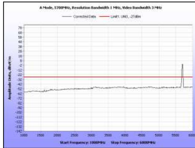
Plot 237. Radiated Spurious, 802.11a, 5700 MHz, 1 GHz – 6 GHz, Omni Antenna
