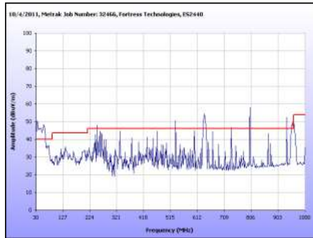
Plot 324. Radiated Spurious, 802.11n 20 MHz, 5500 MHz, 30 MHz – 1 GHz, Sector Antenna
