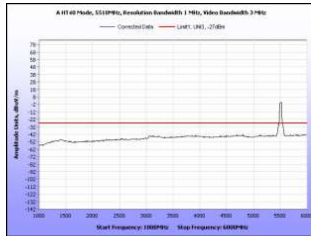
Plot 277. Radiated Spurious, 802.11n 40 MHz, 5510 MHz, 1 GHz – 6 GHz, Omni Antenna
