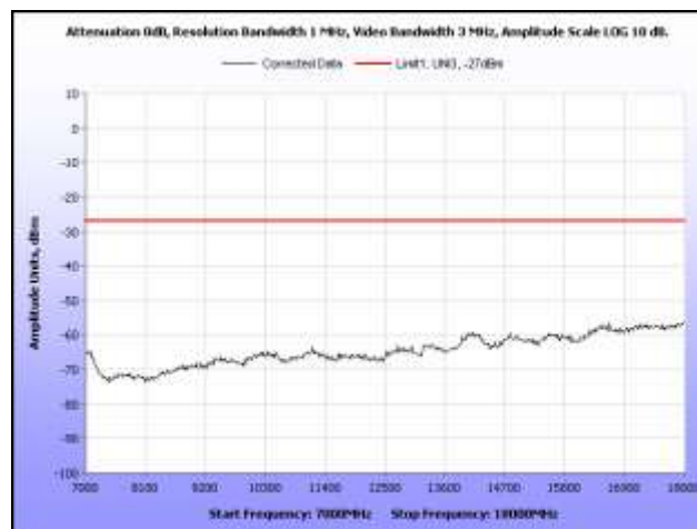
Plot 290. Radiated Spurious, 802.11a, 5260 MHz, 7 GHz – 18 GHz, Sector Antenna
