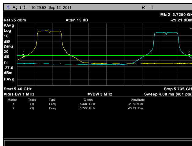
Plot 469. Frequency Stability, 802.11n 40 MHz, 5470 MHz – 5725 MHz @ 20°C, 132 V
