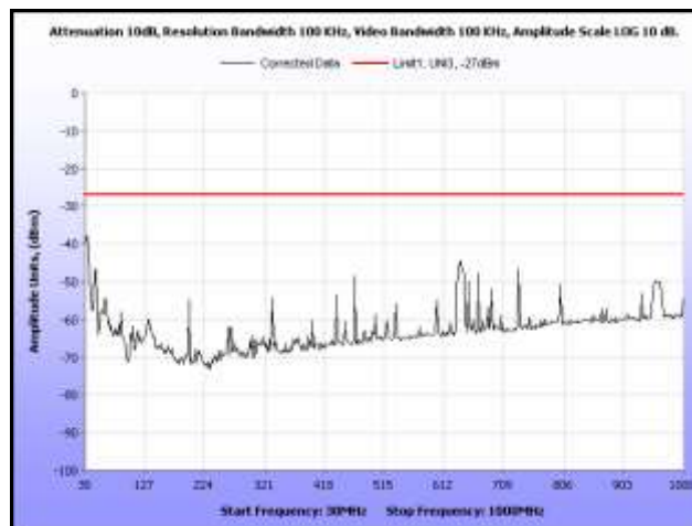
Plot 260. Radiated Spurious, 802.11n 20 MHz, 5700 MHz, 30 MHz – 1 GHz, Omni Antenna
