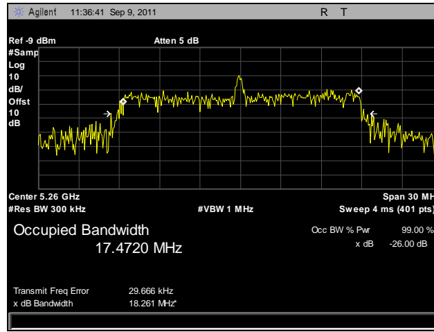
Plot 48. 99% Occupied Bandwidth, 802.11n 20 MHz, Port B, 5260 MHz
