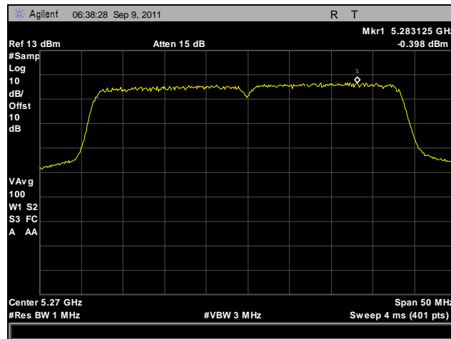
Plot 150. Peak Spectral Density, 802.11n 40 MHz, Port B, 5270 MHz
