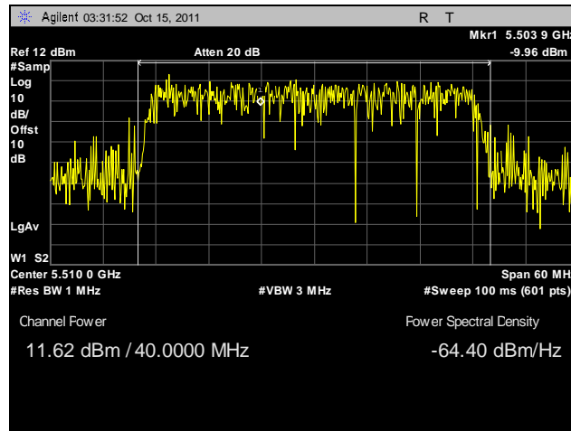
Plot 93. Conducted Output Power, 802.11n 40 MHz, Port B, 5510 MHz
