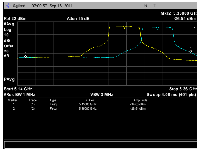
Plot 462. Frequency Stability, 802.11n 40 MHz, 5250 MHz – 5350 MHz @ 55°C, 120 V
