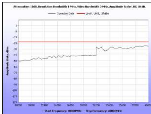
Plot 311. Radiated Spurious, 802.11a, 5700 MHz, 18 GHz – 40 GHz, Sector Antenna
