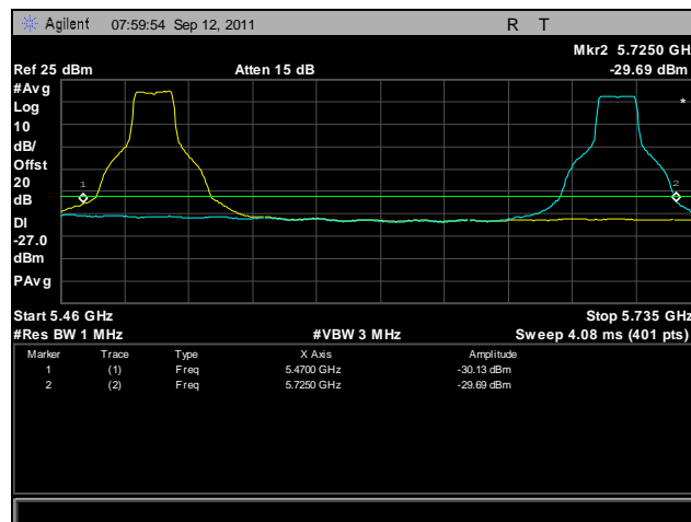
Plot 425. Frequency Stability, 802.11a, 5470 MHz – 5725 MHz @ 20°C, 132 V
