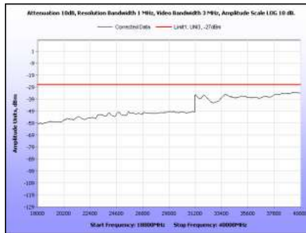
Plot 331. Radiated Spurious, 802.11n 20 MHz, 5580 MHz, 18 GHz – 40 GHz, Sector Antenna
