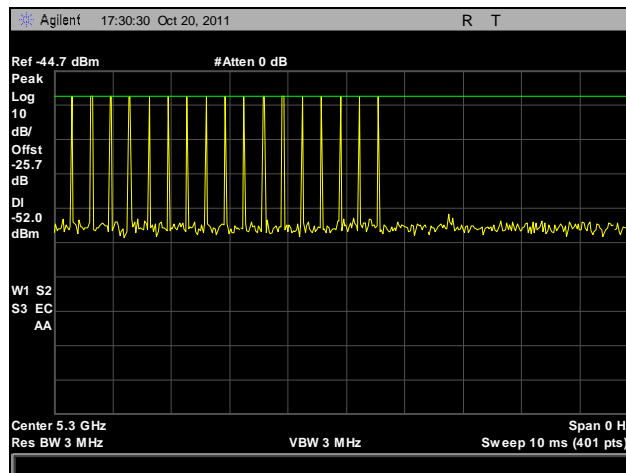
Plot 480. Radar Calibration, Bin 3
