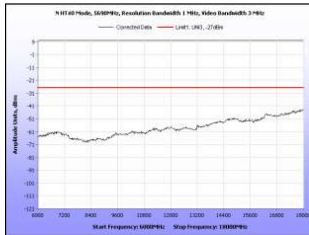
Plot 286. Radiated Spurious, 802.11n 40 MHz, 5690 MHz, 6 GHz – 18 GHz, Omni Antenna
