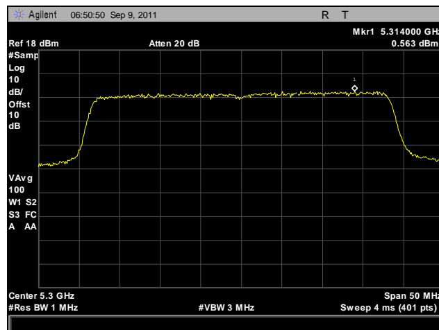
Plot 151. Peak Spectral Density, 802.11n 40 MHz, Port B, 5300 MHz
