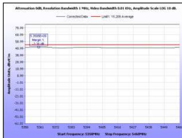
Plot 390. Restricted Band, 802.11n 20 MHz, 5500 MHz, Average, Omni Antenna
