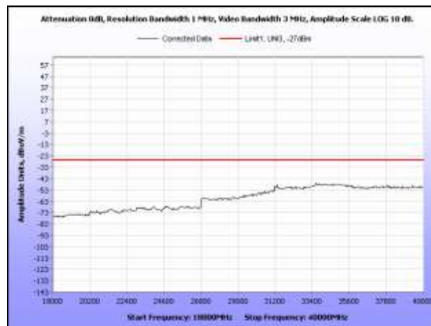
Plot 239. Radiated Spurious, 802.11a, 5700 MHz, 18 GHz – 40 GHz, Omni Antenna
