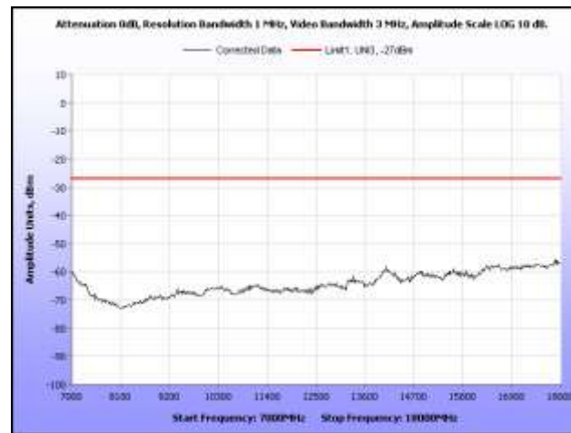
Plot 358. Radiated Spurious, 802.11n 40 MHz, 5690 MHz, 7 GHz – 18 GHz, Sector Antenna
