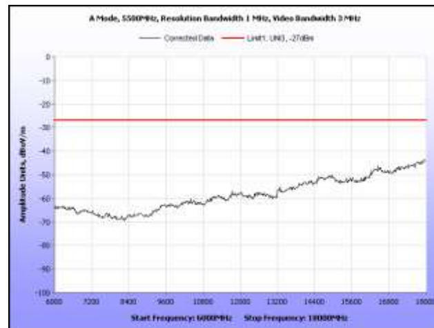
Plot 230. Radiated Spurious, 802.11a, 5500 MHz, 6 GHz – 18 GHz, Omni Antenna
