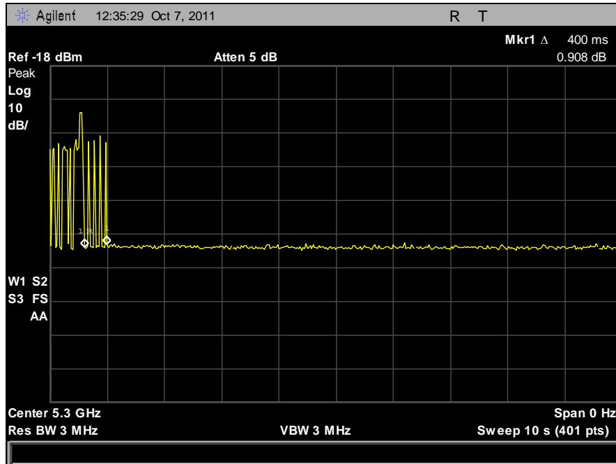
Plot 487. Channel Move Time
