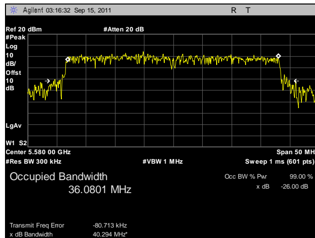
Plot 34. Occupied Bandwidth, 802.11n 40 MHz, Port B, 5580 MHz
