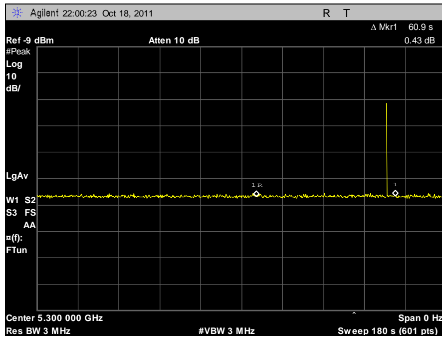
Plot 486. Radar Burst at the End of CACT
