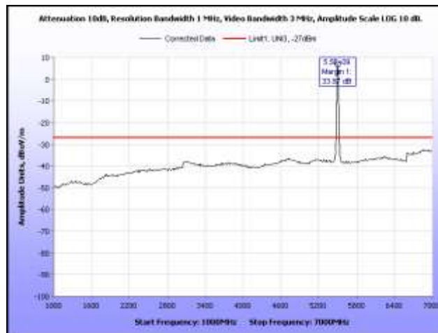
Plot 301. Radiated Spurious, 802.11a, 5500 MHz, 1 GHz – 7 GHz, Sector Antenna
