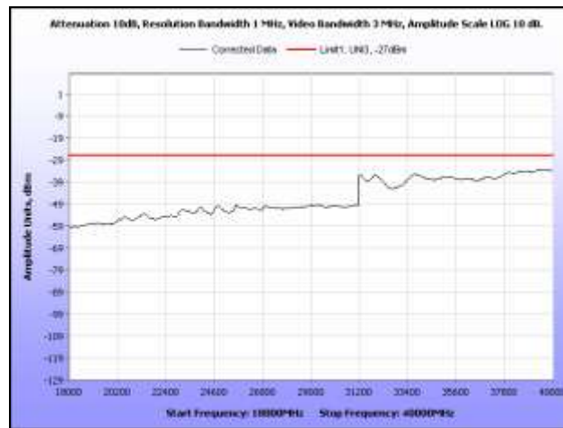
Plot 307. Radiated Spurious, 802.11a, 5580 MHz, 18 GHz – 40 GHz, Sector Antenna
