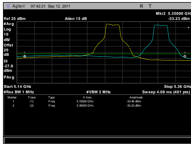
Plot 412. Frequency Stability, 802.11a, 5250 MHz – 5350 MHz @ 20°C, 108 V
