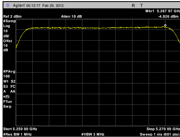
Plot 168. Peak Spectral Density, 802.11n 20 MHz, Port B, 5260 MHz, Sector Antenna
