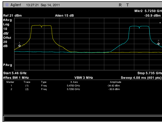
Plot 470. Frequency Stability, 802.11n 40 MHz, 5470 MHz – 5725 MHz @ 30°C, 120 V
