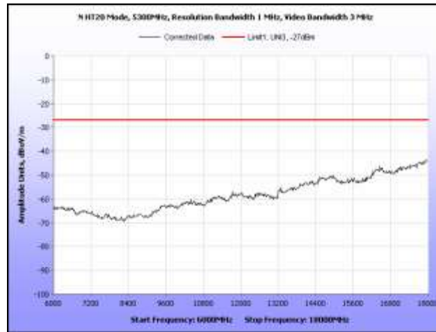
Plot 246. Radiated Spurious, 802.11n 20 MHz, 5300 MHz, 6 GHz – 18 GHz, Omni Antenna
