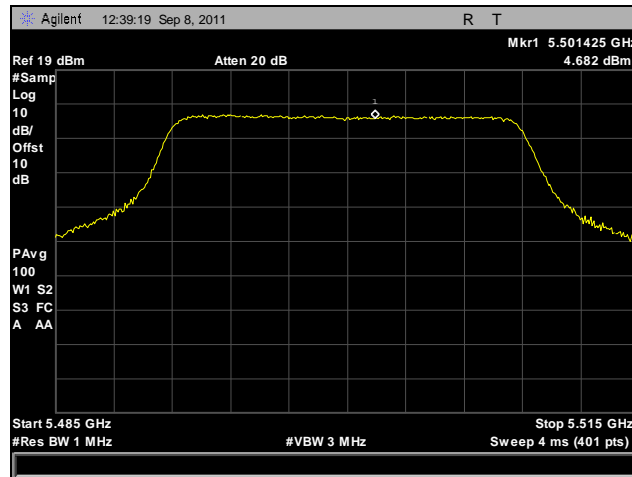
Plot 141. Peak Spectral Density, 802.11n 20 MHz, Port B, 5500 MHz
