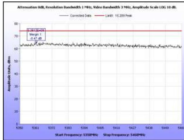
Plot 403. Restricted Band, 802.11n 20 MHz, 5500 MHz, Peak, Sector Antenna
