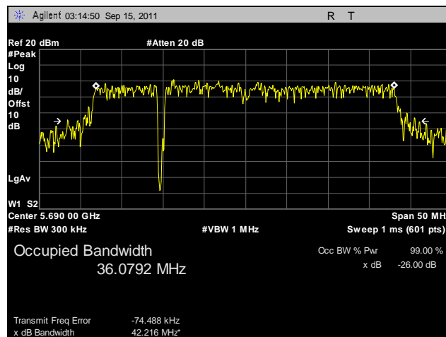
Plot 35. Occupied Bandwidth, 802.11n 40 MHz, Port B, 5690 MHz
