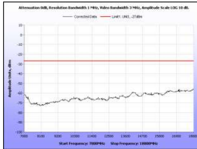
Plot 318. Radiated Spurious, 802.11n 20 MHz, 5300 MHz, 7 GHz – 18 GHz, Sector Antenna
