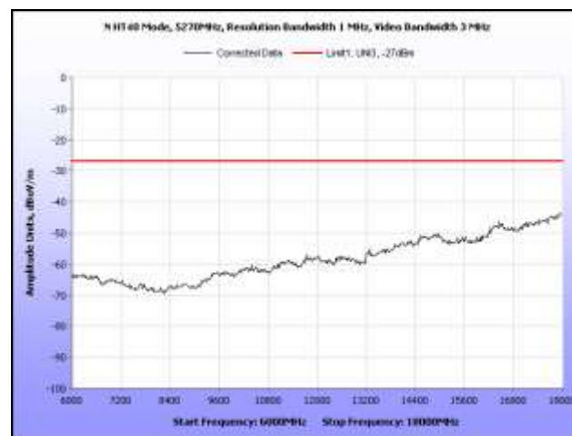
Plot 266. Radiated Spurious, 802.11n 40 MHz, 5270 MHz, 6 GHz – 18 GHz, Omni Antenna
