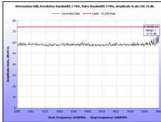
Plot 395. Restricted Band, 802.11n 40 MHz, 5510 MHz, Peak, Omni Antenna
