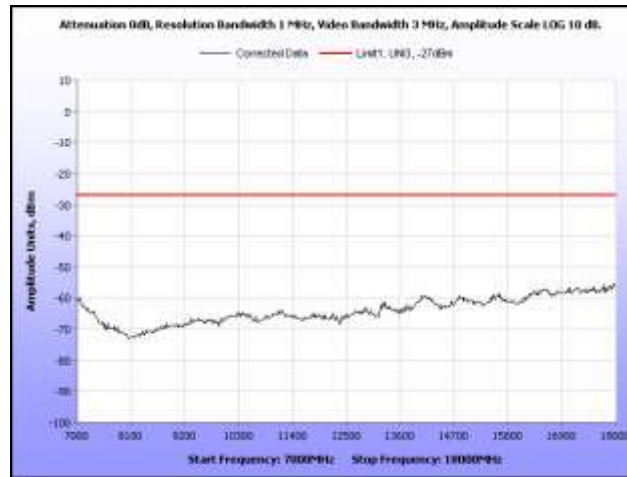
Plot 342. Radiated Spurious, 802.11n 40 MHz, 5300 MHz, 7 GHz – 18 GHz, Sector Antenna
