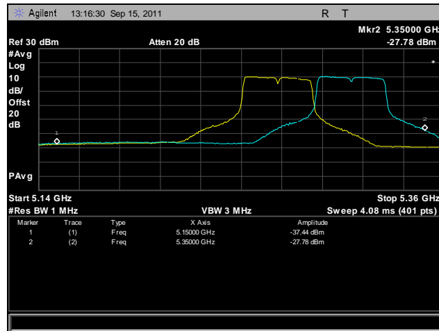
Plot 461. Frequency Stability, 802.11n 40 MHz, 5250 MHz – 5350 MHz @ 50°C, 120 V
