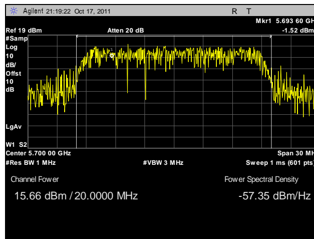
Plot 77. Conducted Output Power, 802.11n 20 MHz, Port A, 5700 MHz
