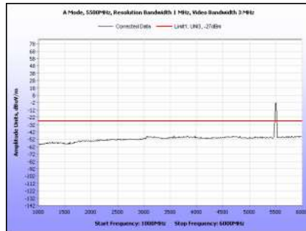
Plot 229. Radiated Spurious, 802.11a, 5500 MHz, 1 GHz – 6 GHz, Omni Antenna
