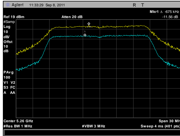
Plot 198. Peak Excursion, 802.11n 20 MHz, Port B, 5260 MHz
