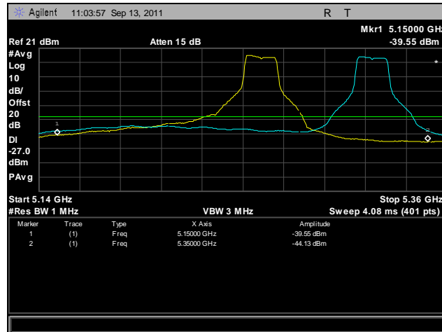
Plot 408. Frequency Stability, 802.11a, 5250 MHz – 5350 MHz @ -20°C, 120 V
