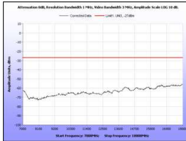
Plot 306. Radiated Spurious, 802.11a, 5580 MHz, 7 GHz – 18 GHz, Sector Antenna
