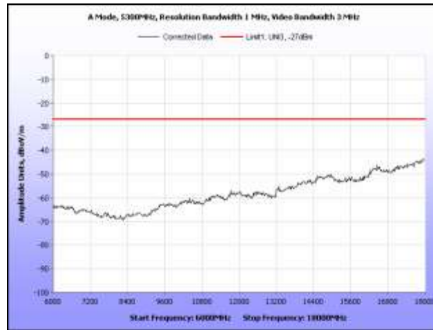
Plot 222. Radiated Spurious, 802.11a, 5300 MHz, 6 GHz – 18 GHz, Omni Antenna
