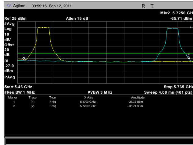
Plot 445. Frequency Stability, 802.11n 20 MHz, 5470 MHz – 5725 MHz @ 20°C, 108 V
