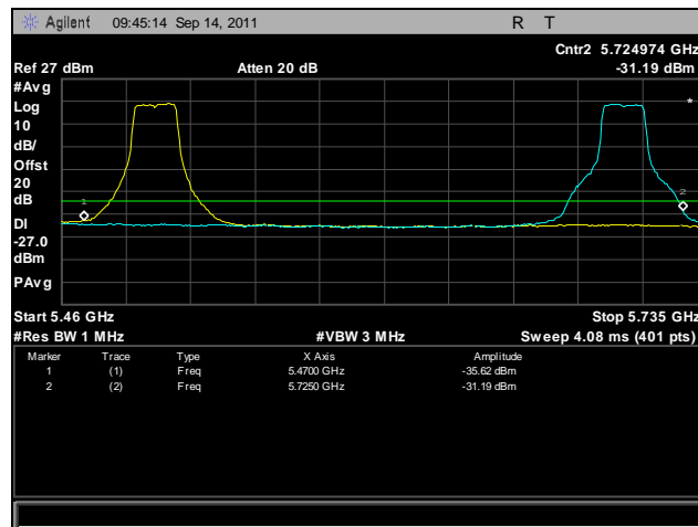
Plot 443. Frequency Stability, 802.11n 20 MHz, 5470 MHz – 5725 MHz @ 0°C, 120 V
