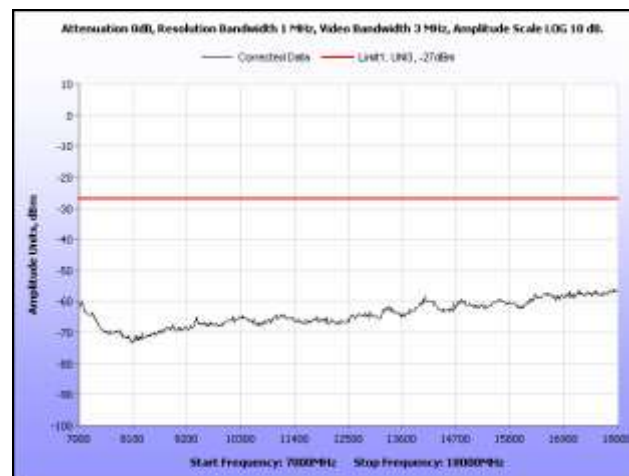
Plot 338. Radiated Spurious, 802.11n 40 MHz, 5270 MHz, 7 GHz – 18 GHz, Sector Antenna
