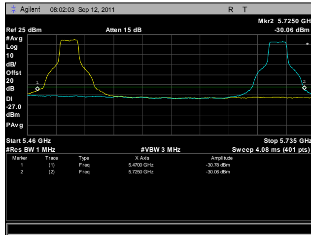
Plot 423. Frequency Stability, 802.11a, 5470 MHz – 5725 MHz @ 20°C, 108 V
