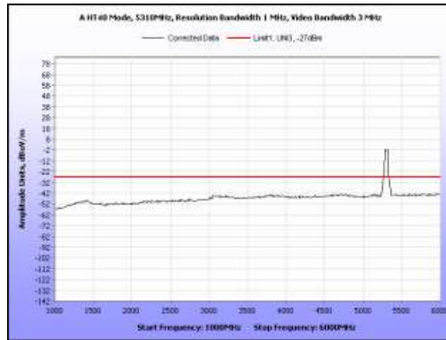
Plot 273. Radiated Spurious, 802.11n 40 MHz, 5310 MHz, 1 GHz – 6 GHz, Omni Antenna
