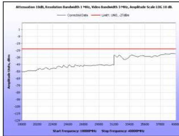
Plot 291. Radiated Spurious, 802.11a, 5260 MHz, 18 GHz – 40 GHz, Sector Antenna
