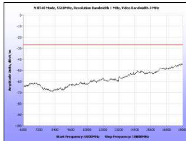
Plot 278. Radiated Spurious, 802.11n 40 MHz, 5510 MHz, 6 GHz – 18 GHz, Omni Antenna
