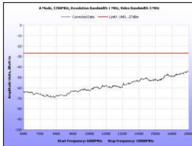
Plot 238. Radiated Spurious, 802.11a, 5700 MHz, 6 GHz – 18 GHz, Omni Antenna
