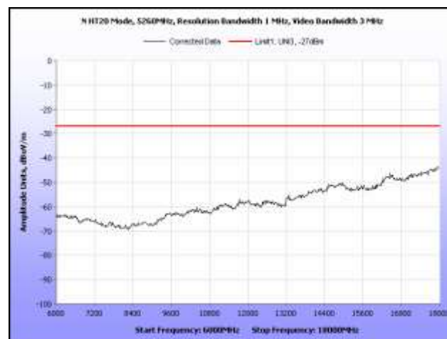
Plot 242. Radiated Spurious, 802.11n 20 MHz, 5260 MHz, 6 GHz – 18 GHz, Omni Antenna
