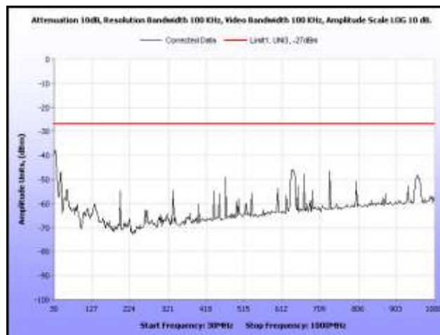
Plot 248. Radiated Spurious, 802.11n 20 MHz, 5320 MHz, 30 MHz – 1 GHz, Omni Antenna
