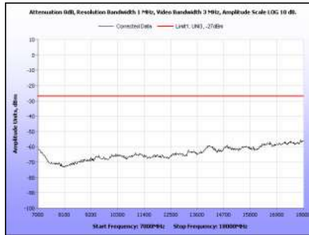
Plot 330. Radiated Spurious, 802.11n 20 MHz, 5580 MHz, 7 GHz – 18 GHz, Sector Antenna
