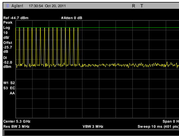
Plot 481. Radar Calibration, Bin 4
