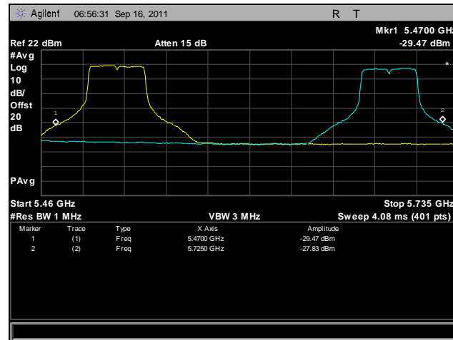
Plot 473. Frequency Stability, 802.11n 40 MHz, 5470 MHz – 5725 MHz @ 55°C, 120 V
