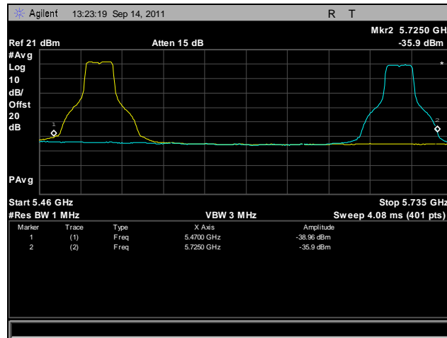
Plot 448. Frequency Stability, 802.11n 20 MHz, 5470 MHz – 5725 MHz @ 30°C, 120 V
