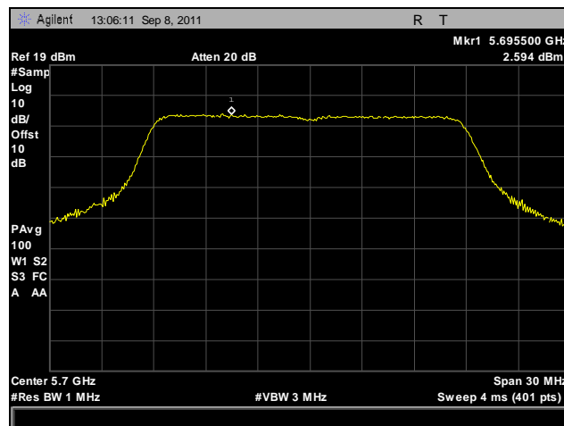
Plot 143. Peak Spectral Density, 802.11n 20 MHz, Port B, 5700 MHz
