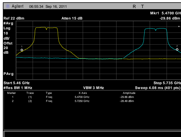
Plot 472. Frequency Stability, 802.11n 40 MHz, 5470 MHz – 5725 MHz @ 50°C, 120 V
