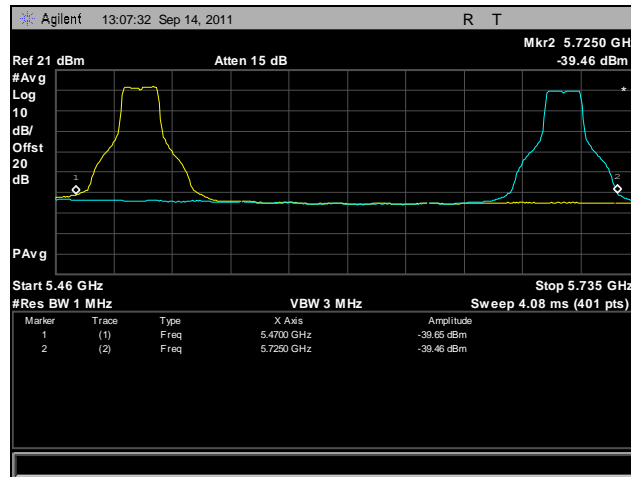
Plot 426. Frequency Stability, 802.11a, 5470 MHz – 5725 MHz @ 30°C, 120 V
