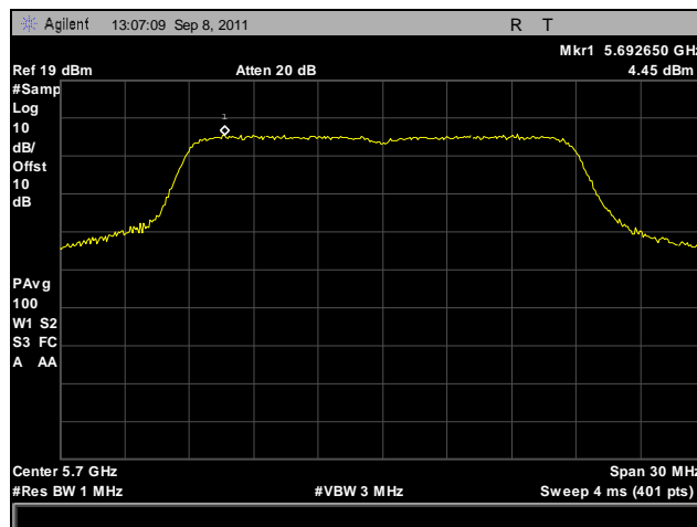
Plot 137. Peak Spectral Density, 802.11n 20 MHz, Port A, 5700 MHz
