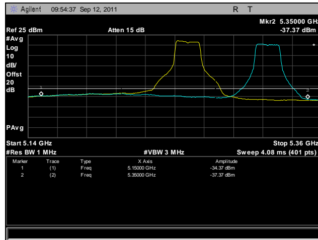
Plot 434. Frequency Stability, 802.11n 20 MHz, 5250 MHz – 5350 MHz @ 20°C, 108 V
