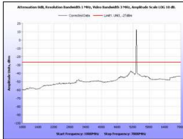
Plot 321. Radiated Spurious, 802.11n 20 MHz, 5320 MHz, 1 GHz – 7 GHz, Sector Antenna
