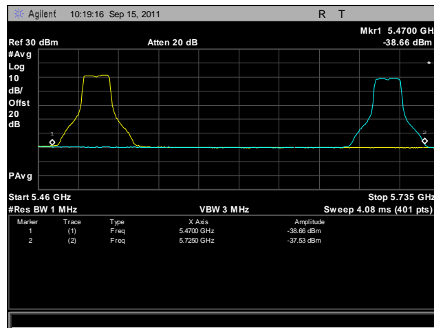
Plot 449. Frequency Stability, 802.11n 20 MHz, 5470 MHz – 5725 MHz @ 40°C, 120 V
