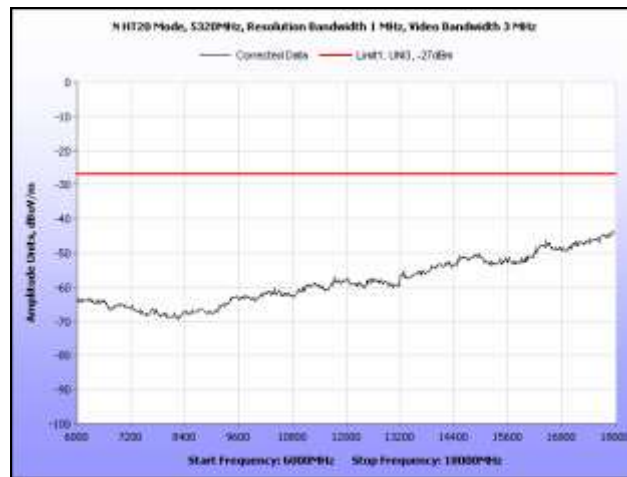
Plot 250. Radiated Spurious, 802.11n 20 MHz, 5320 MHz, 6 GHz – 18 GHz, Omni Antenna
