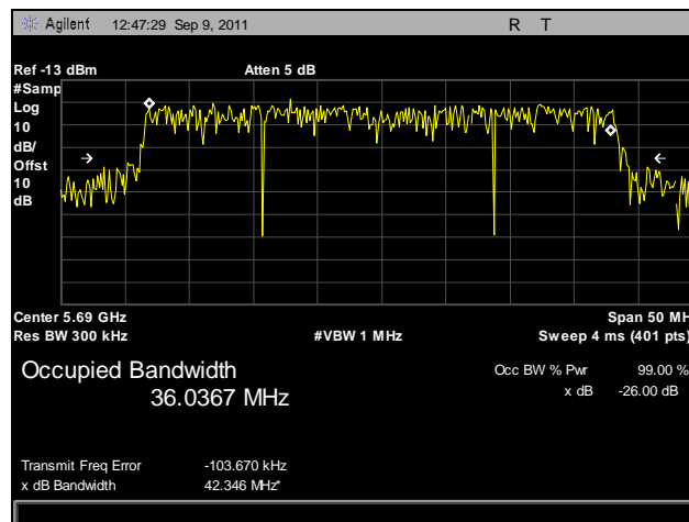
Plot 65. 99% Occupied Bandwidth, 802.11n 40 MHz, Port B, 5690 MHz
