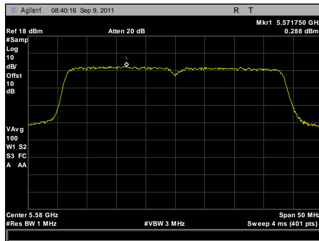
Plot 154. Peak Spectral Density, 802.11n 40 MHz, Port B, 5580 MHz
