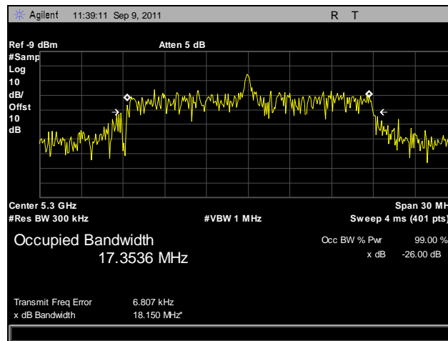
Plot 49. 99% Occupied Bandwidth, 802.11n 20 MHz, Port B, 5300 MHz
