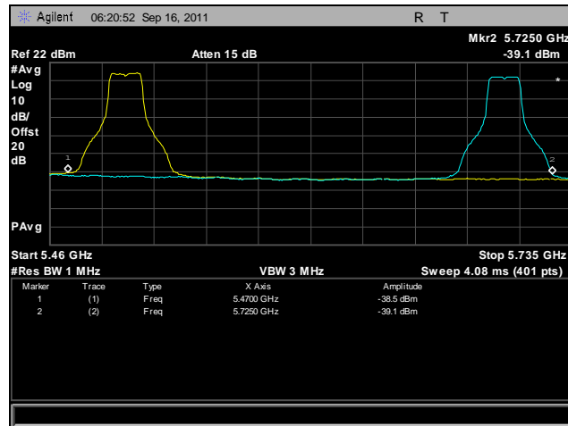
Plot 429. Frequency Stability, 802.11a, 5470 MHz – 5725 MHz @ 55°C, 120 V
