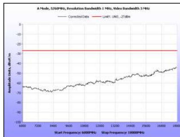
Plot 218. Radiated Spurious, 802.11a, 5260 MHz, 6 GHz – 18 GHz, Omni Antenna
