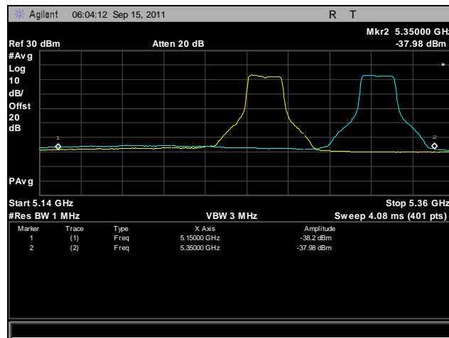
Plot 437. Frequency Stability, 802.11n 20 MHz, 5250 MHz – 5350 MHz @ 30°C, 120 V
