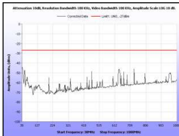
Plot 224. Radiated Spurious, 802.11a, 5320 MHz, 30 MHz – 1 GHz, Omni Antenna
