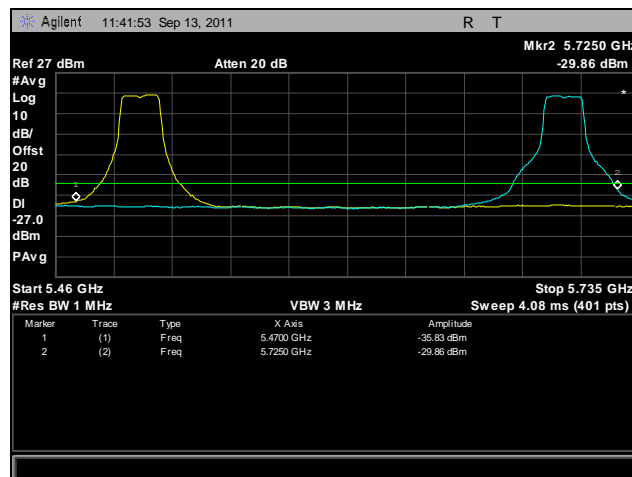
Plot 441. Frequency Stability, 802.11n 20 MHz, 5470 MHz – 5725 MHz @ -20°C, 120 V
