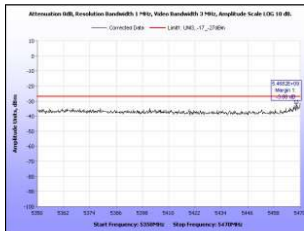
Plot 382. EIRP, 802.11n 40 MHz, 5510 MHz, Band Edge, Sector Antenna
