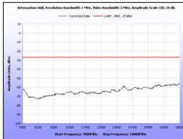
Plot 322. Radiated Spurious, 802.11n 20 MHz, 5320 MHz, 7 GHz – 18 GHz, Sector Antenna
