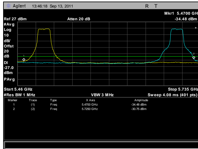
Plot 442. Frequency Stability, 802.11n 20 MHz, 5470 MHz – 5725 MHz @ -10°C, 120 V
