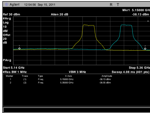
Plot 439. Frequency Stability, 802.11n 20 MHz, 5250 MHz – 5350 MHz @ 50°C, 120 V
