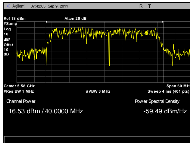
Plot 94. Conducted Output Power, 802.11n 40 MHz, Port B, 5580 MHz
