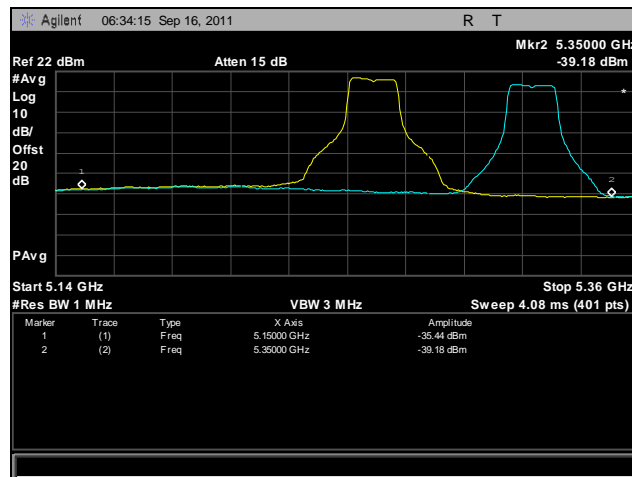
Plot 440. Frequency Stability, 802.11n 20 MHz, 5250 MHz – 5350 MHz @ 55°C, 120 V
