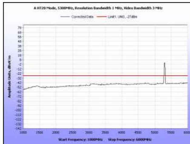
Plot 245. Radiated Spurious, 802.11n 20 MHz, 5300 MHz, 1 GHz – 6 GHz, Omni Antenna
