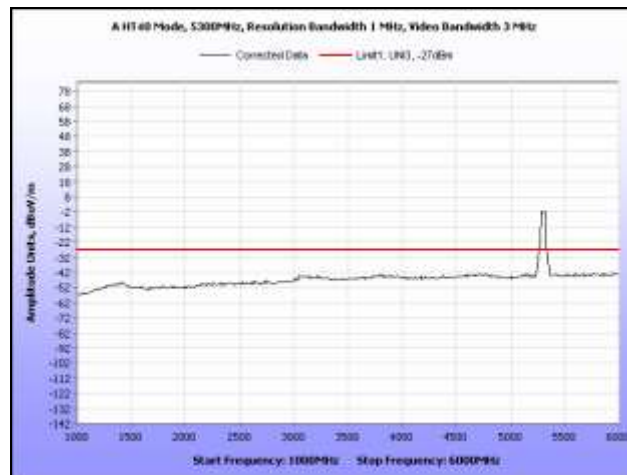
Plot 269. Radiated Spurious, 802.11n 40 MHz, 5300 MHz, 1 GHz – 6 GHz, Omni Antenna
