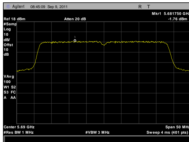
Plot 149. Peak Spectral Density, 802.11n 40 MHz, Port A, 5690 MHz
