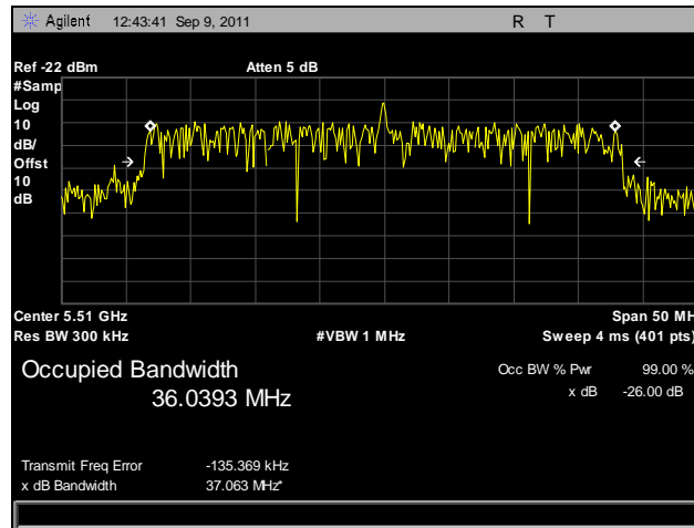
Plot 57. 99% Occupied Bandwidth, 802.11n 40 MHz, Port A, 5510 MHz
