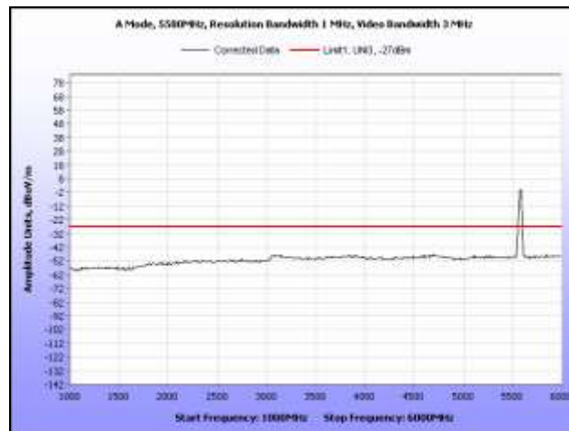
Plot 233. Radiated Spurious, 802.11a, 5580 MHz, 1 GHz – 6 GHz, Omni Antenna
