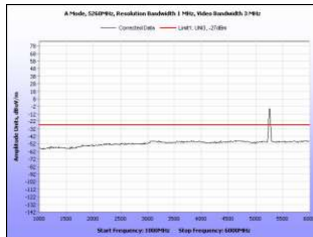
Plot 217. Radiated Spurious, 802.11a, 5260 MHz, 1 GHz – 6 GHz, Omni Antenna
