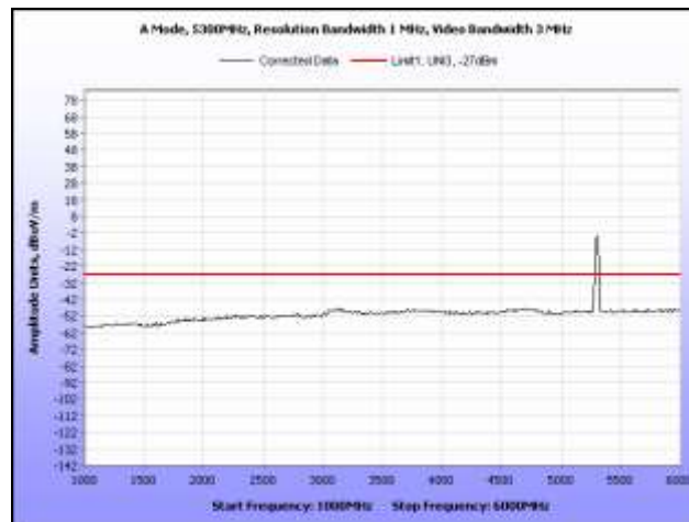
Plot 221. Radiated Spurious, 802.11a, 5300 MHz, 1 GHz – 6 GHz, Omni Antenna
