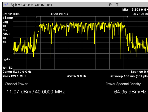
Plot 92. Conducted Output Power, 802.11n 40 MHz, Port B, 5310 MHz
