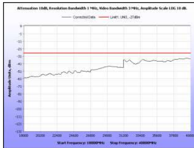
Plot 355. Radiated Spurious, 802.11n 40 MHz, 5580 MHz, 18 GHz – 40 GHz, Sector Antenna
