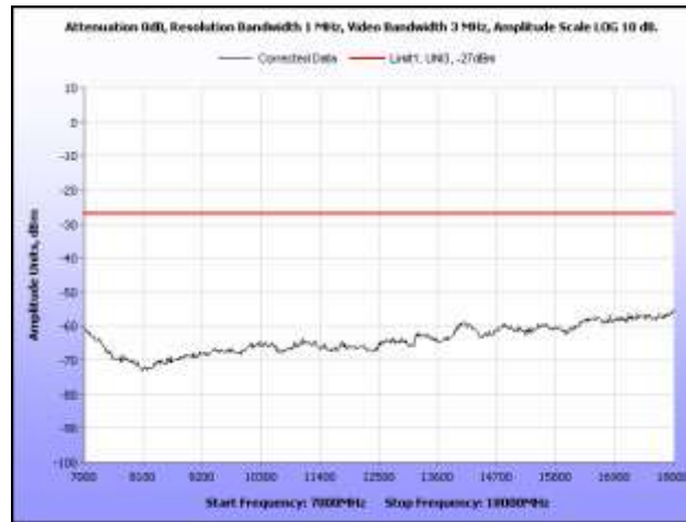
Plot 354. Radiated Spurious, 802.11n 40 MHz, 5580 MHz, 7 GHz – 18 GHz, Sector Antenna
