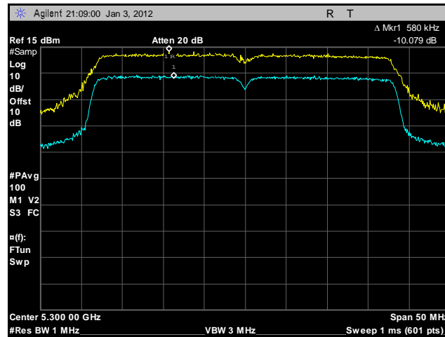
Plot 205. Peak Excursion, 802.11n 40 MHz, Port A, 5300 MHz
