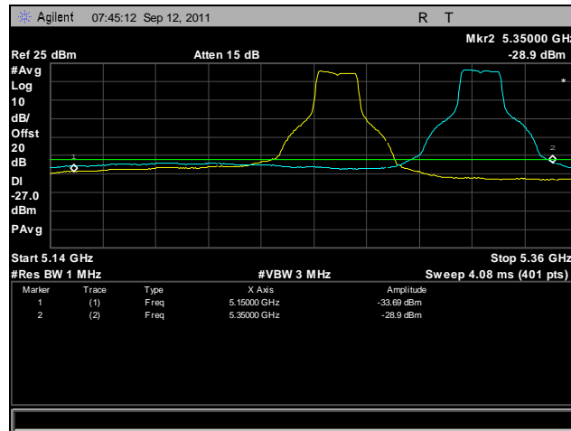
Plot 414. Frequency Stability, 802.11a, 5250 MHz – 5350 MHz @ 20°C, 132 V
