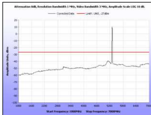
Plot 293. Radiated Spurious, 802.11a, 5300 MHz, 1 GHz – 7 GHz, Sector Antenna
