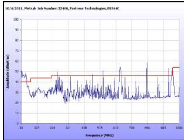
Plot 348. Radiated Spurious, 802.11n 40 MHz, 5510 MHz, 30 MHz – 1 GHz, Sector Antenna
