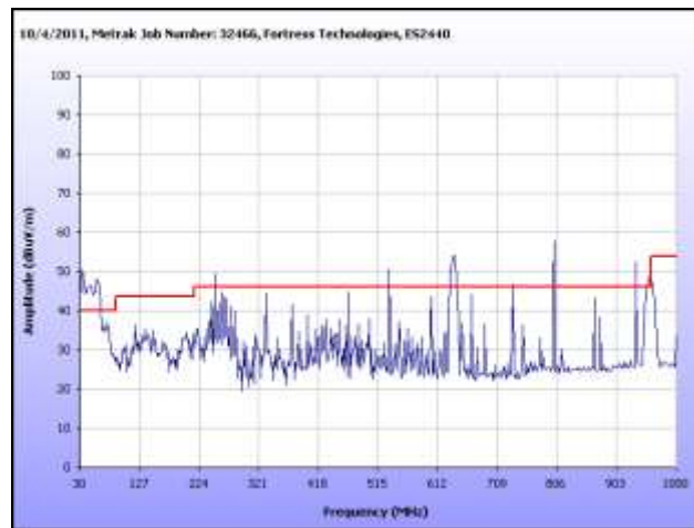
Plot 316. Radiated Spurious, 802.11n 20 MHz, 5300 MHz, 30 MHz – 1 GHz, Sector Antenna
