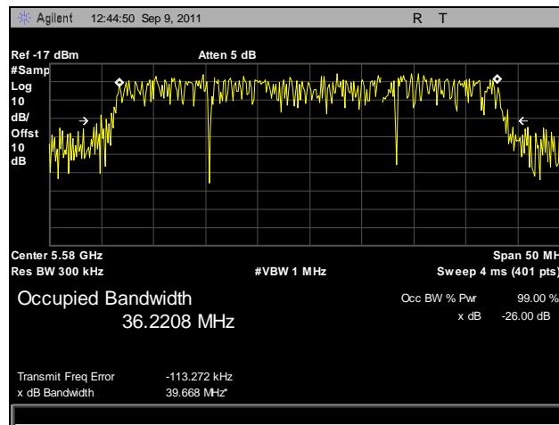
Plot 58. 99% Occupied Bandwidth, 802.11n 40 MHz, Port A, 5580 MHz
