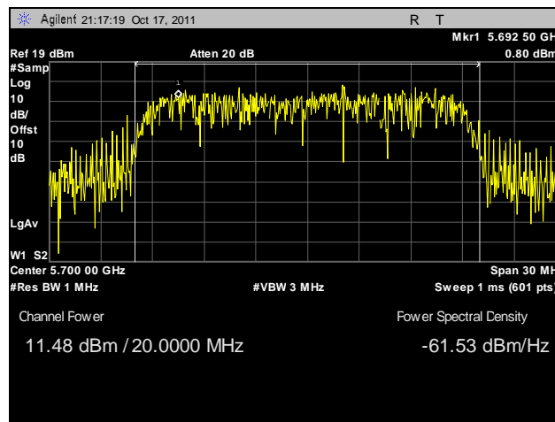
Plot 83. Conducted Output Power, 802.11n 20 MHz, Port B, 5700 MHz
