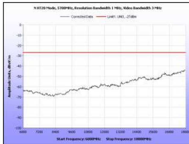
Plot 262. Radiated Spurious, 802.11n 20 MHz, 5700 MHz, 6 GHz – 18 GHz, Omni Antenna
