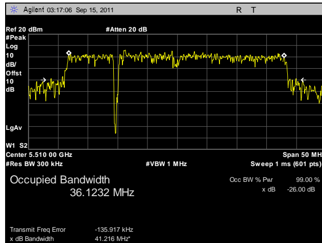
Plot 33. Occupied Bandwidth, 802.11n 40 MHz, Port B, 5510 MHz
