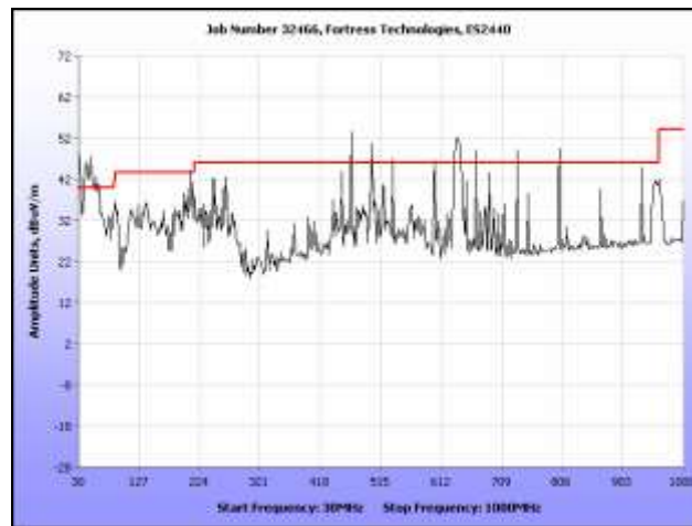
Plot 292. Radiated Spurious, 802.11a, 5300 MHz, 30 MHz – 1 GHz, Sector Antenna
