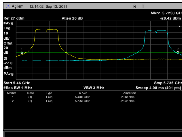
Plot 463. Frequency Stability, 802.11n 40 MHz, 5470 MHz – 5725 MHz @ -20°C, 120 V
