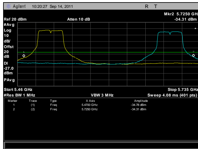
Plot 465. Frequency Stability, 802.11n 40 MHz, 5470 MHz – 5725 MHz @ 0°C, 120 V
