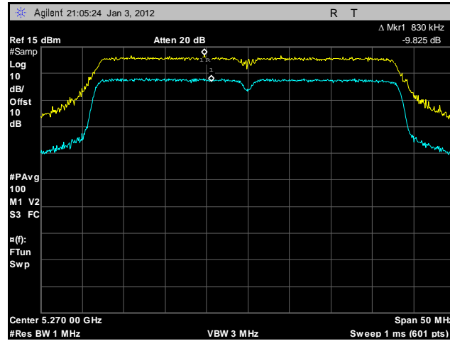
Plot 204. Peak Excursion, 802.11n 40 MHz, Port A, 5270 MHz
