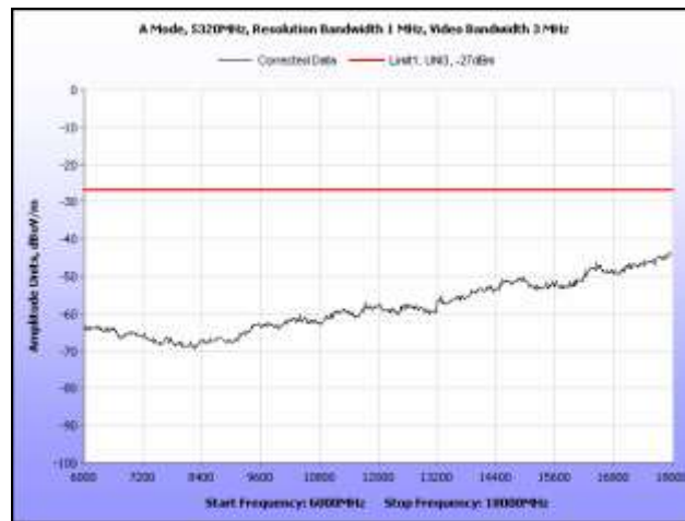
Plot 226. Radiated Spurious, 802.11a, 5320 MHz, 6 GHz – 18 GHz, Omni Antenna
