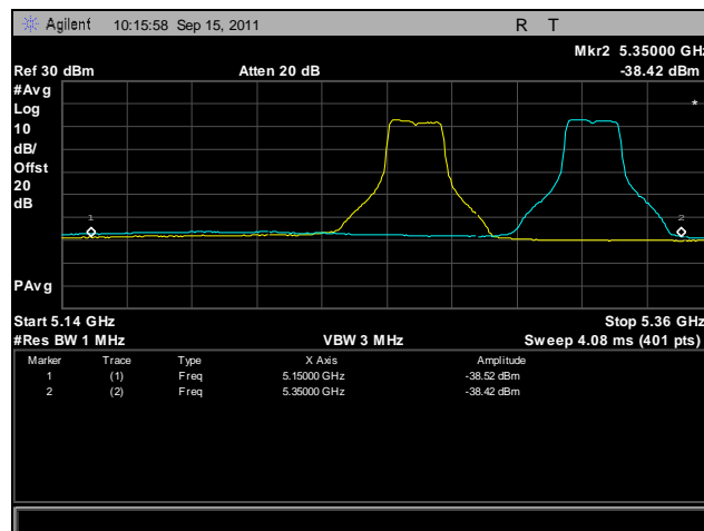
Plot 438. Frequency Stability, 802.11n 20 MHz, 5250 MHz – 5350 MHz @ 40°C, 120 V
