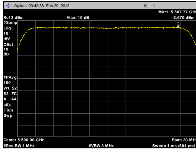
Plot 165. Peak Spectral Density, 802.11n 20 MHz, Port A, 5500 MHz, Sector Antenna
