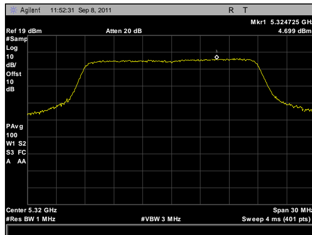
Plot 140. Peak Spectral Density, 802.11n 20 MHz, Port B, 5320 MHz
