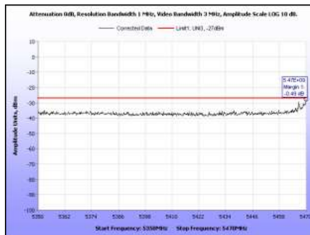
Plot 374. EIRP, 802.11a, 5500 MHz, Band Edge, Sector Antenna
