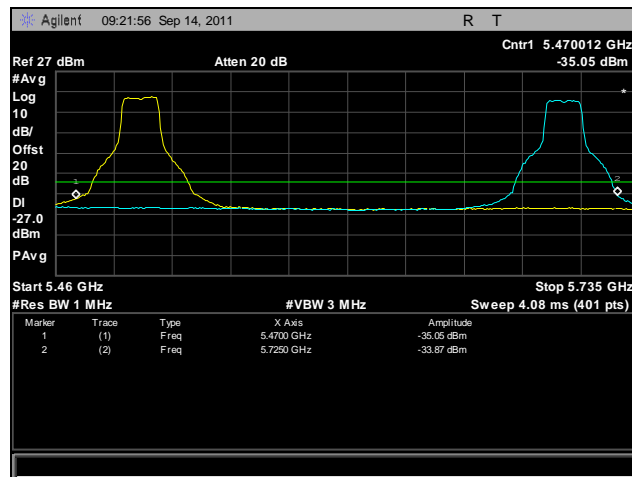
Plot 421. Frequency Stability, 802.11a, 5470 MHz – 5725 MHz @ 0°C, 120 V
