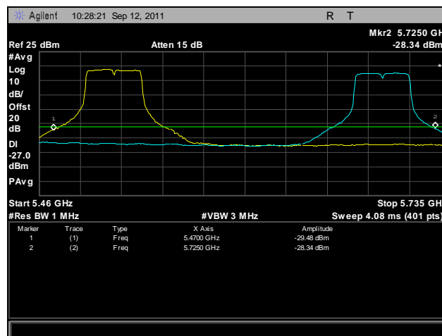
Plot 468. Frequency Stability, 802.11n 40 MHz, 5470 MHz – 5725 MHz @ 20°C, 120 V
