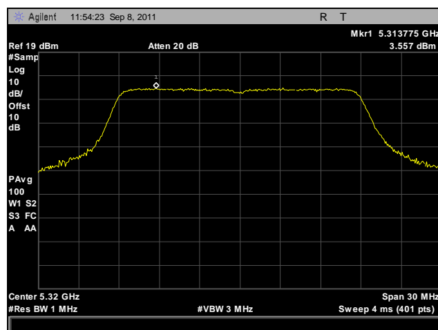
Plot 134. Peak Spectral Density, 802.11n 20 MHz, Port A, 5320 MHz
