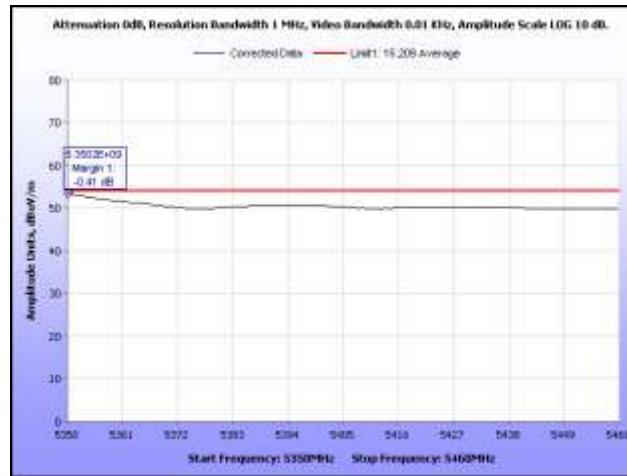
Plot 384. Restricted Band, 802.11a, 5320 MHz, Average, Omni Antenna
