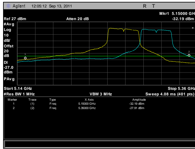
Plot 452. Frequency Stability, 802.11n 40 MHz, 5250 MHz – 5350 MHz @ -20°C, 120 V
