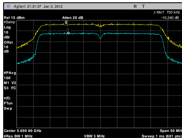
Plot 209. Peak Excursion, 802.11n 40 MHz, Port A, 5690 MHz
