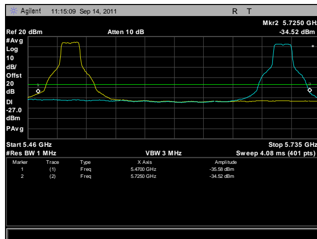
Plot 422. Frequency Stability, 802.11a, 5470 MHz – 5725 MHz @ 10°C, 120 V
