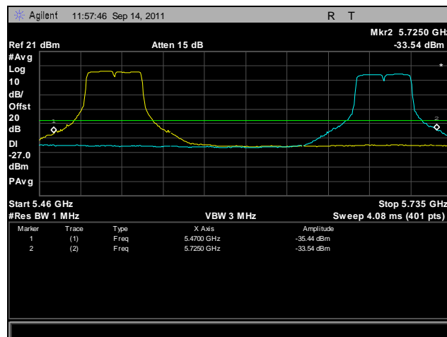
Plot 466. Frequency Stability, 802.11n 40 MHz, 5470 MHz – 5725 MHz @ 10°C, 120 V
