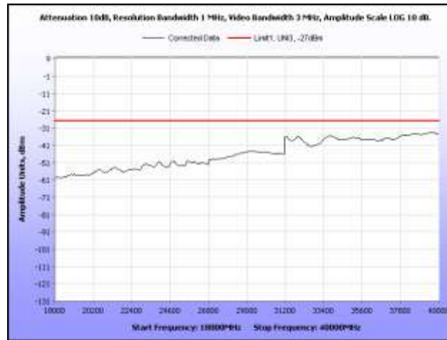
Plot 339. Radiated Spurious, 802.11n 40 MHz, 5270 MHz, 18 GHz – 40 GHz, Sector Antenna
