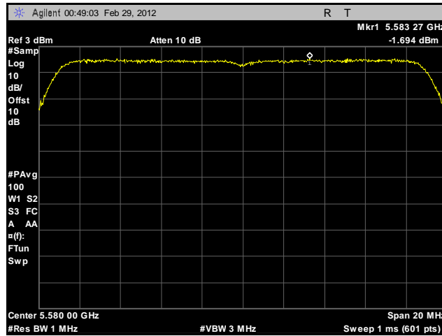
Plot 166. Peak Spectral Density, 802.11n 20 MHz, Port A, 5580 MHz, Sector Antenna
