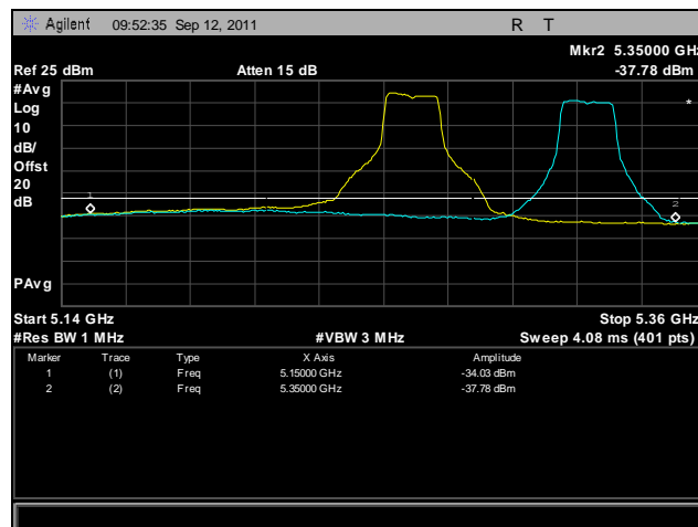
Plot 413. Frequency Stability, 802.11a, 5250 MHz – 5350 MHz @ 20°C, 120 V
