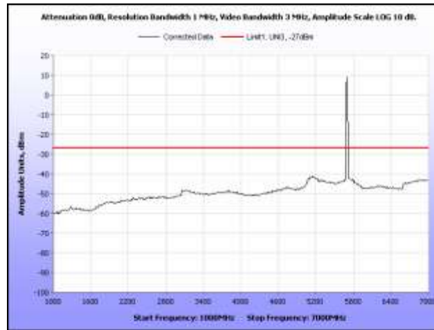
Plot 309. Radiated Spurious, 802.11a, 5700 MHz, 1 GHz – 7 GHz, Sector Antenna
