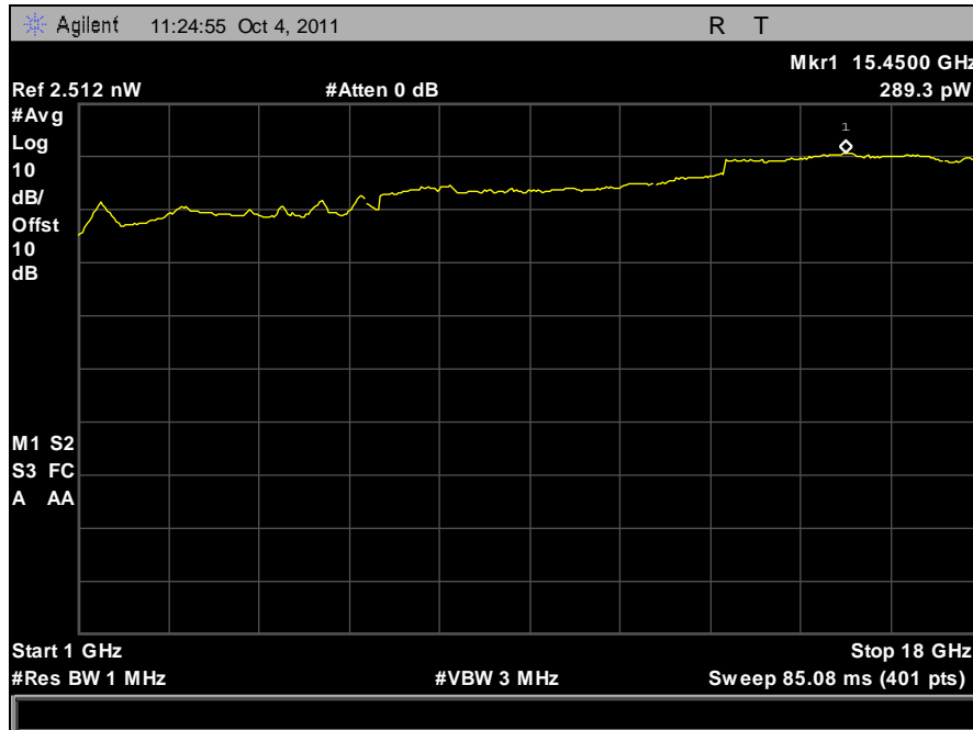
Plot 477. Receiver Spurious Emission, 1 GHz – 18 GHz, Port B
