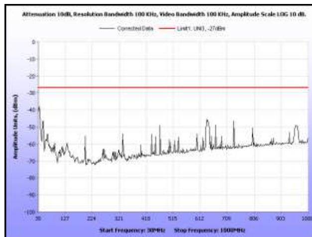
Plot 236. Radiated Spurious, 802.11a, 5700 MHz, 30 MHz – 1 GHz, Omni Antenna
