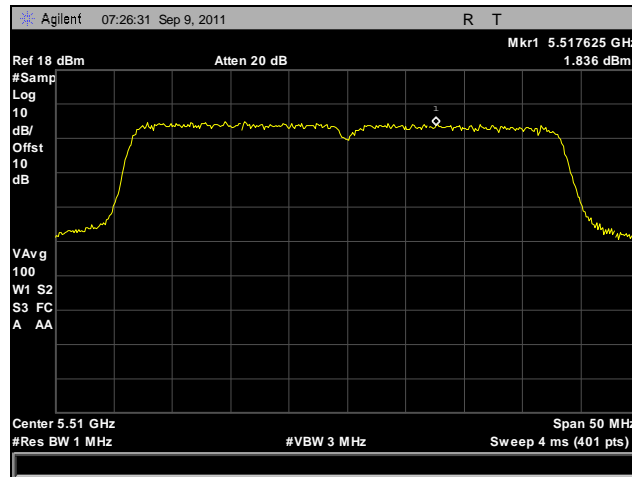
Plot 153. Peak Spectral Density, 802.11n 40 MHz, Port B, 5510 MHz
