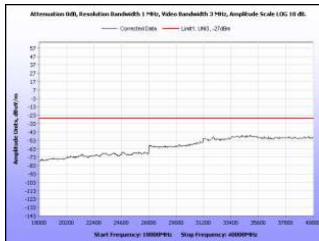
Plot 251. Radiated Spurious, 802.11n 20 MHz, 5320 MHz, 18 GHz – 40 GHz, Omni Antenna
