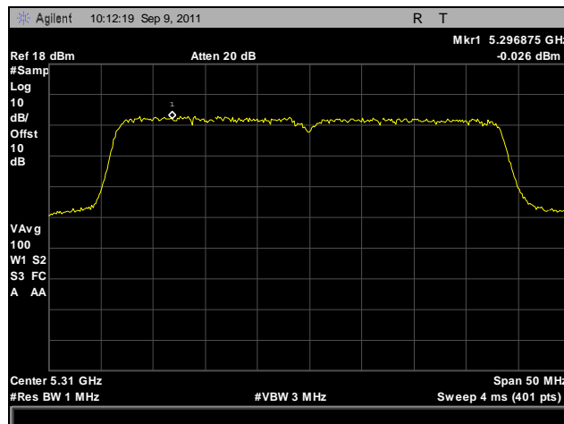
Plot 146. Peak Spectral Density, 802.11n 40 MHz, Port A, 5310 MHz
