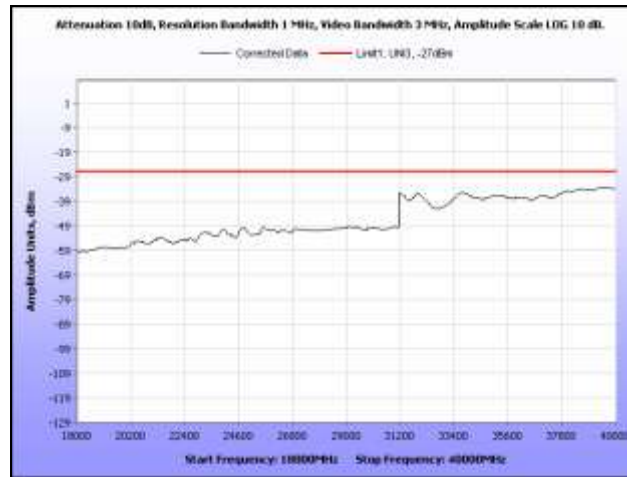
Plot 327. Radiated Spurious, 802.11n 20 MHz, 5500 MHz, 18 MHz – 40 GHz, Sector Antenna
