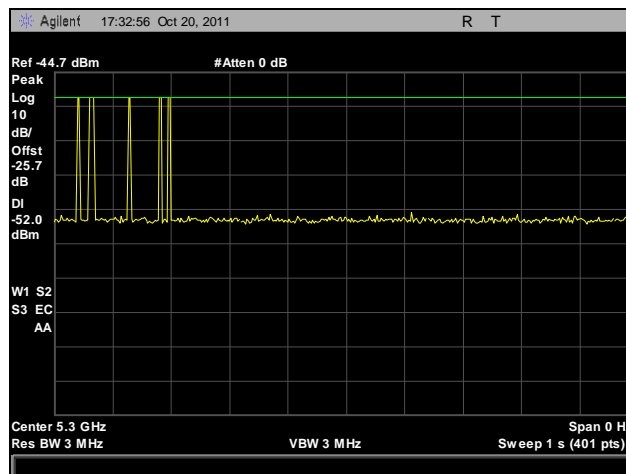
Plot 483. Radar Calibration, Bin 6
