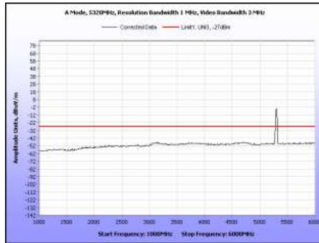
Plot 225. Radiated Spurious, 802.11a, 5320 MHz, 1 GHz – 6 GHz, Omni Antenna
