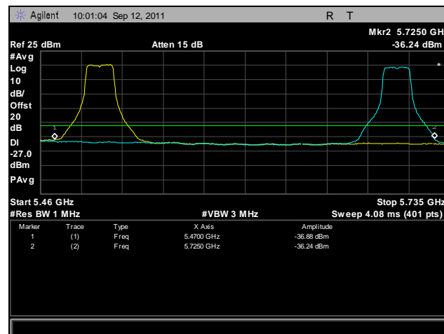
Plot 447. Frequency Stability, 802.11n 20 MHz, 5470 MHz – 5725 MHz @ 20°C, 132 V
