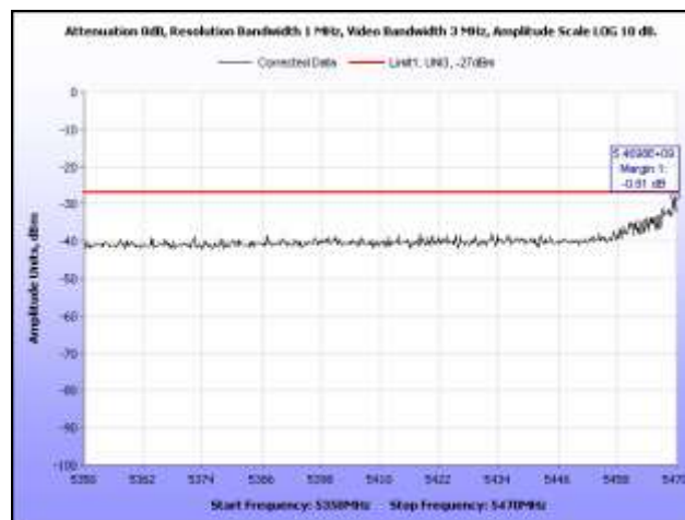
Plot 370. EIRP, 802.11n 40 MHz, 5510 MHz, Band Edge, Omni Antenna
