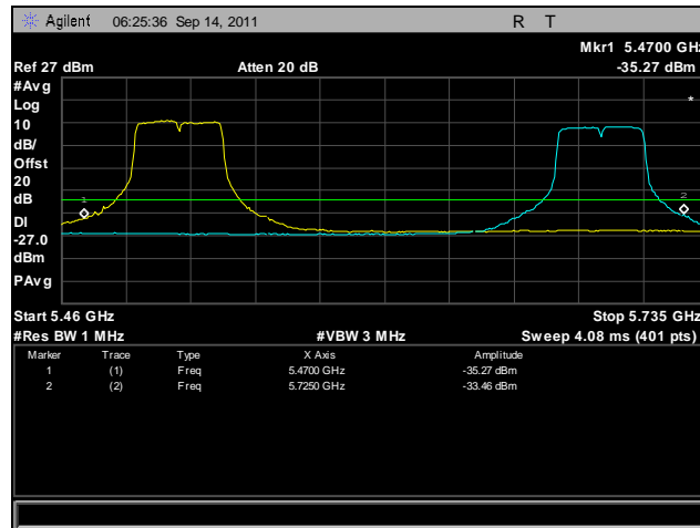
Plot 464. Frequency Stability, 802.11n 40 MHz, 5470 MHz – 5725 MHz @ -10°C, 120 V
