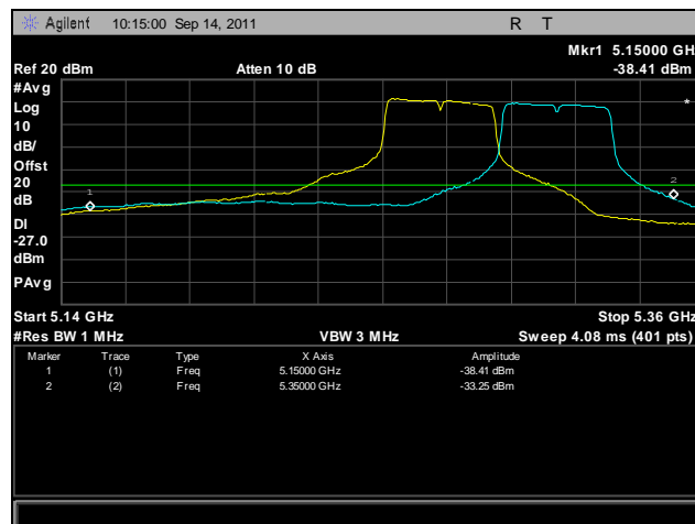
Plot 454. Frequency Stability, 802.11n 40 MHz, 5250 MHz – 5350 MHz @ 0°C, 120 V
