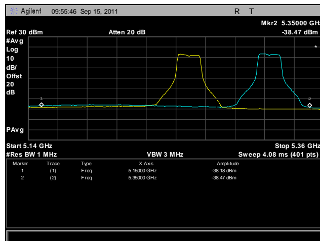
Plot 416. Frequency Stability, 802.11a, 5250 MHz – 5350 MHz @ 40°C, 120 V
