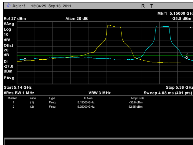
Plot 409. Frequency Stability, 802.11a, 5250 MHz – 5350 MHz @ -10°C, 120 V
