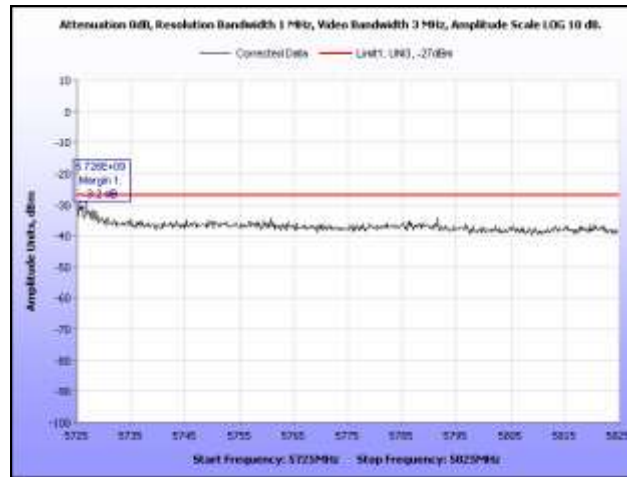
Plot 375. EIRP, 802.11a, 5700 MHz, Band Edge, Sector Antenna
