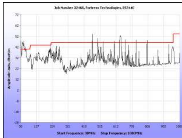
Plot 304. Radiated Spurious, 802.11a, 5580 MHz, 30 MHz – 1 GHz, Sector Antenna
