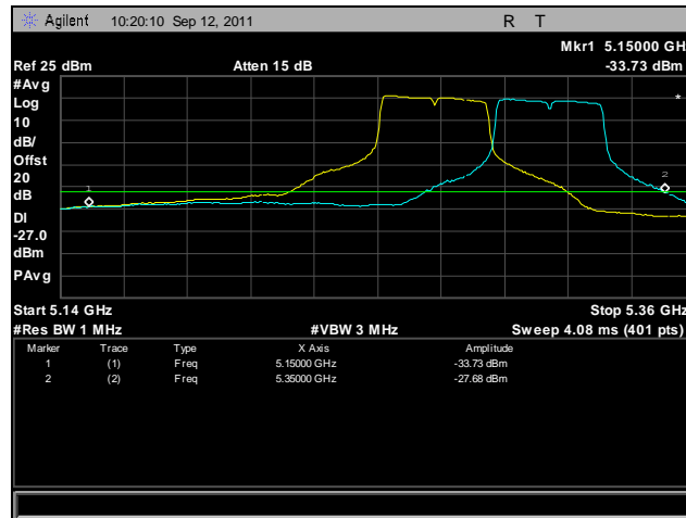
Plot 458. Frequency Stability, 802.11n 40 MHz, 5250 MHz – 5350 MHz @ 20°C, 132 V
