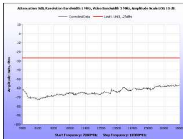
Plot 314. Radiated Spurious, 802.11n 20 MHz, 5260 MHz, 7 GHz – 18 GHz, Sector Antenna
