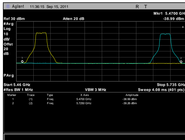
Plot 428. Frequency Stability, 802.11a, 5470 MHz – 5725 MHz @ 50°C, 120 V
