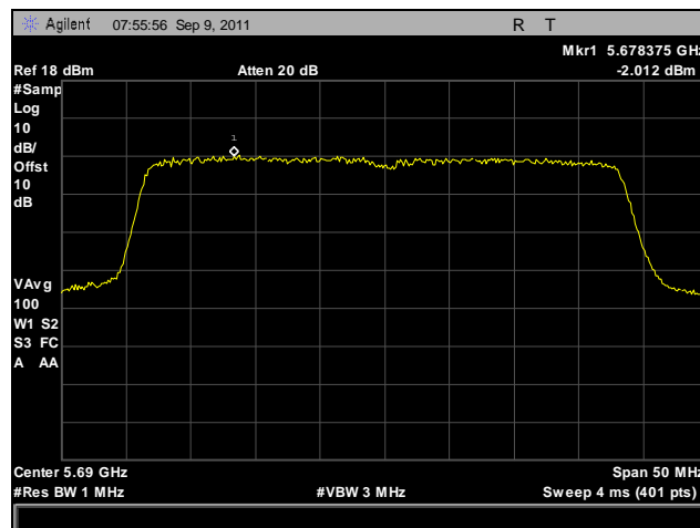
Plot 155. Peak Spectral Density, 802.11n 40 MHz, Port B, 5690 MHz
