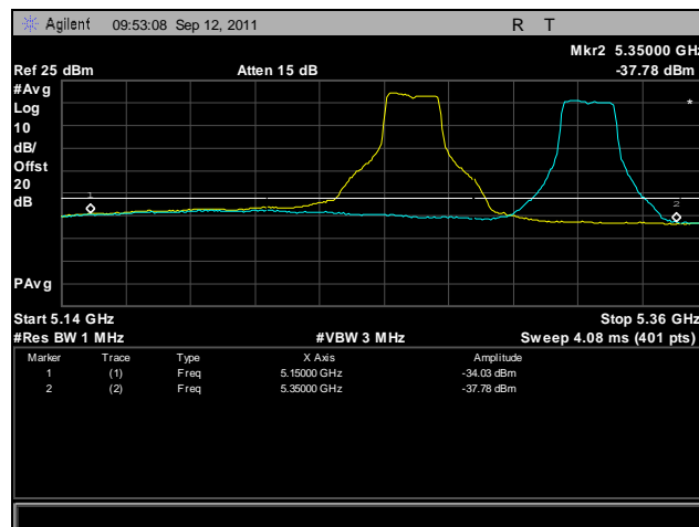
Plot 435. Frequency Stability, 802.11n 20 MHz, 5250 MHz – 5350 MHz @ 20°C, 120 V
