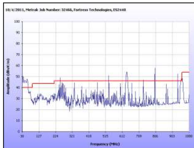
Plot 320. Radiated Spurious, 802.11n 20 MHz, 5320 MHz, 30 MHz – 1 GHz, Sector Antenna
