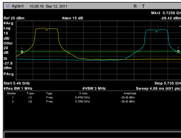
Plot 467. Frequency Stability, 802.11n 40 MHz, 5470 MHz – 5725 MHz @ 20°C, 108 V
