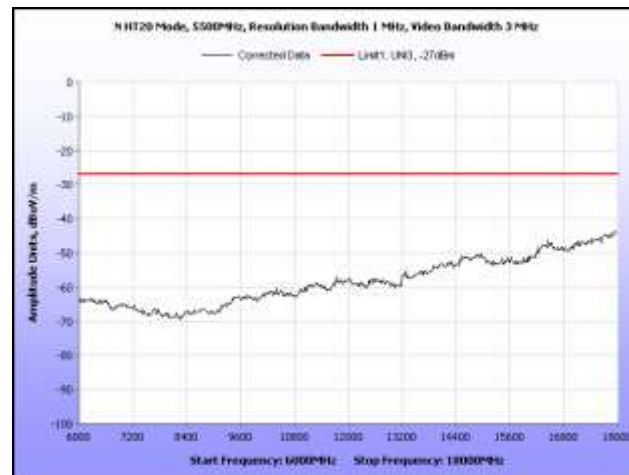
Plot 254. Radiated Spurious, 802.11n 20 MHz, 5500 MHz, 6 GHz – 18 GHz, Omni Antenna
