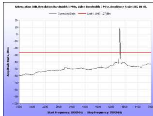
Plot 353. Radiated Spurious, 802.11n 40 MHz, 5580 MHz, 1 GHz – 7 GHz, Sector Antenna
