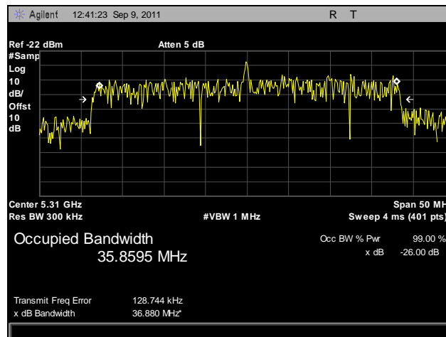
Plot 62. 99% Occupied Bandwidth, 802.11n 40 MHz, Port B, 5310 MHz
