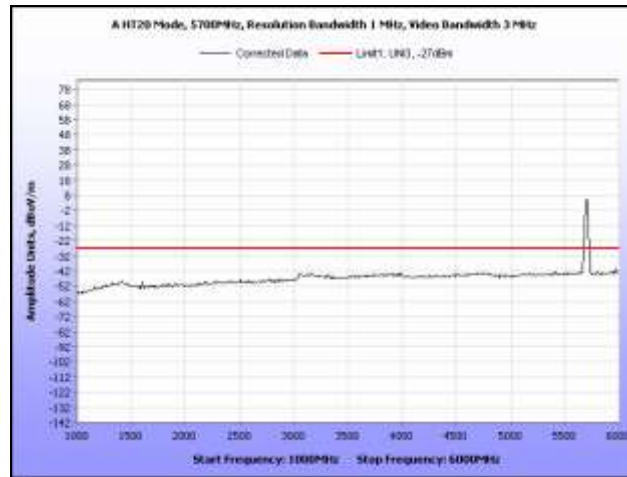
Plot 261. Radiated Spurious, 802.11n 20 MHz, 5700 MHz, 1 GHz – 6 GHz, Omni Antenna
