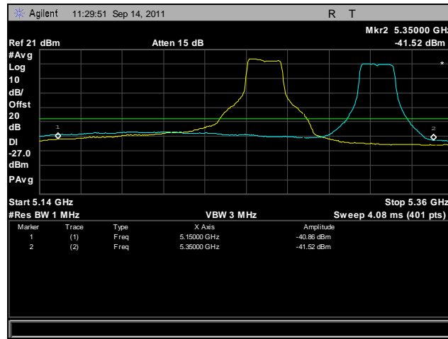
Plot 433. Frequency Stability, 802.11n 20 MHz, 5250 MHz – 5350 MHz @ 10°C, 120 V
