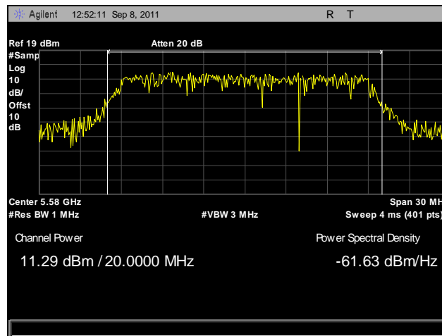
Plot 76. Conducted Output Power, 802.11n 20 MHz, Port A, 5580 MHz
