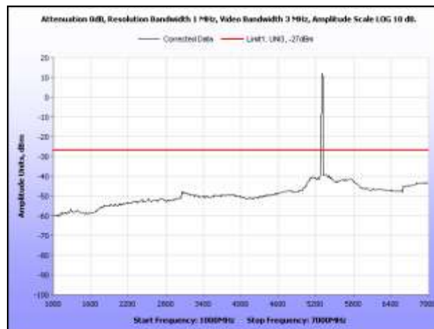
Plot 317. Radiated Spurious, 802.11n 20 MHz, 5300 MHz, 1 GHz – 7 GHz, Sector Antenna
