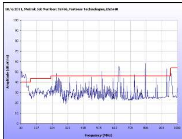
Plot 344. Radiated Spurious, 802.11n 40 MHz, 5310 MHz, 30 MHz – 1 GHz, Sector Antenna
