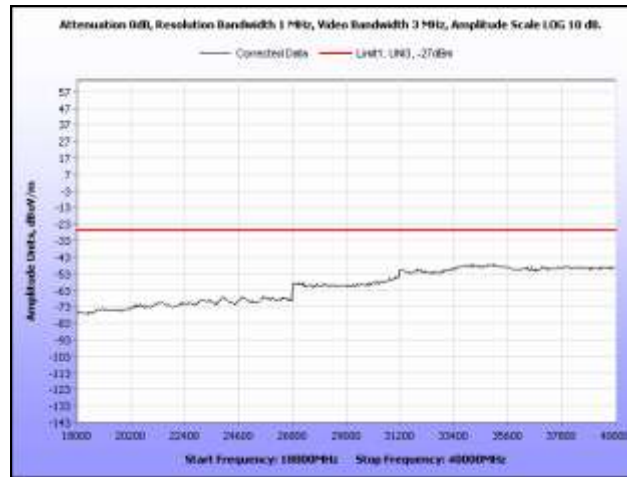
Plot 267. Radiated Spurious, 802.11n 40 MHz, 5270 MHz, 18 GHz – 40 GHz, Omni Antenna
