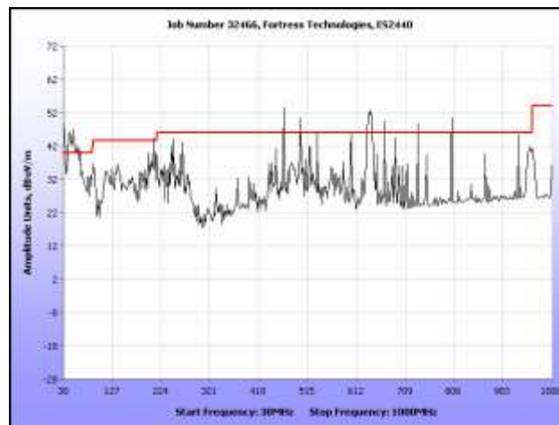
Plot 308. Radiated Spurious, 802.11a, 5700 MHz, 30 MHz – 1 GHz, Sector Antenna
