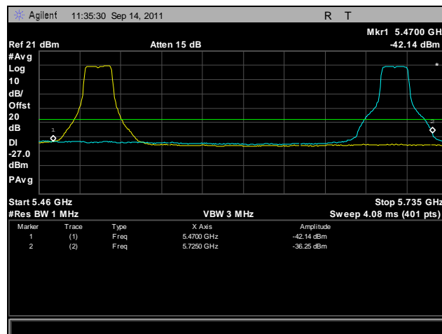
Plot 444. Frequency Stability, 802.11n 20 MHz, 5470 MHz – 5725 MHz @ 10°C, 120 V
