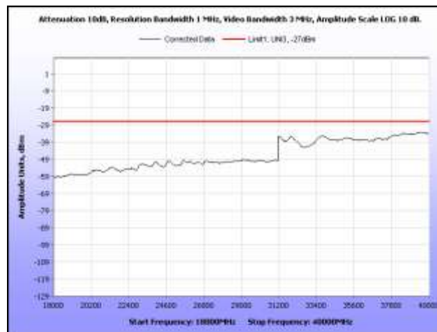
Plot 323. Radiated Spurious, 802.11n 20 MHz, 5320 MHz, 18 GHz – 40 GHz, Sector Antenna
