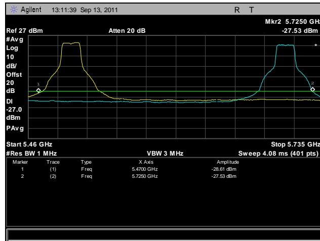
Plot 420. Frequency Stability, 802.11a, 5470 MHz – 5725 MHz @ -10°C, 120 V
