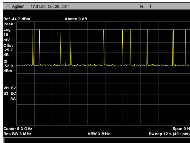
Plot 482. Radar Calibration, Bin 5
