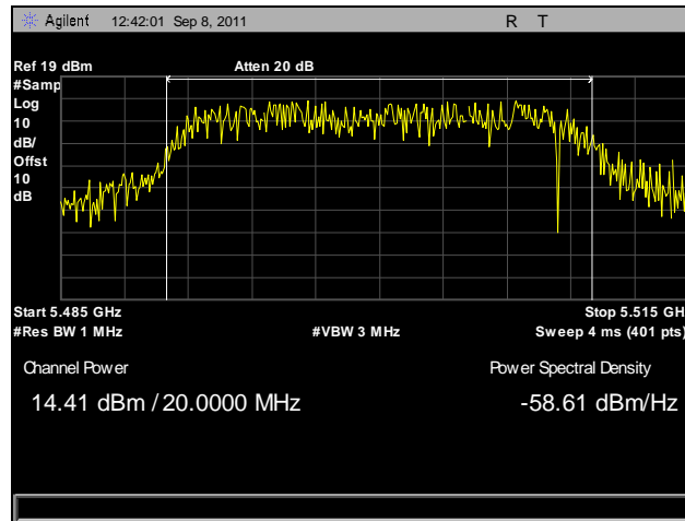
Plot 75. Conducted Output Power, 802.11n 20 MHz, Port A, 5500 MHz
