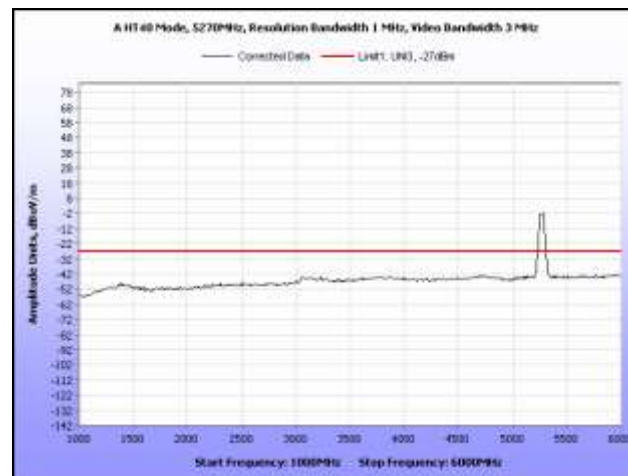
Plot 265. Radiated Spurious, 802.11n 40 MHz, 5270 MHz, 1 GHz – 6 GHz, Omni Antenna
