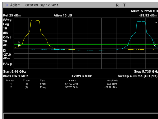
Plot 424. Frequency Stability, 802.11a, 5470 MHz – 5725 MHz @ 20°C, 120 V
