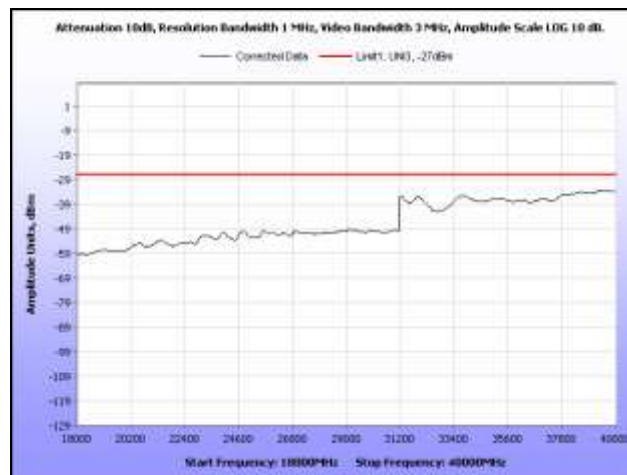
Plot 299. Radiated Spurious, 802.11a, 5320 MHz, 18 GHz – 40 GHz, Sector Antenna
