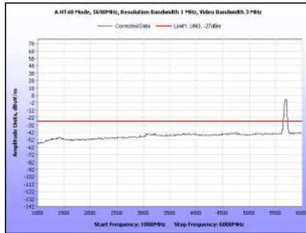
Plot 285. Radiated Spurious, 802.11n 40 MHz, 5690 MHz, 1 GHz – 6 GHz, Omni Antenna
