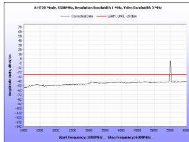
Plot 253. Radiated Spurious, 802.11n 20 MHz, 5500 MHz, 1 GHz – 6 GHz, Omni Antenna
