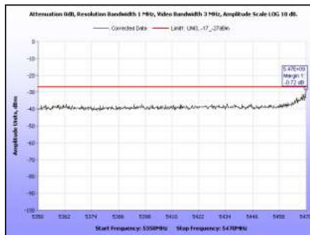
Plot 366. EIRP, 802.11n 20 MHz, 5500 MHz, Band Edge, Omni Antenna
