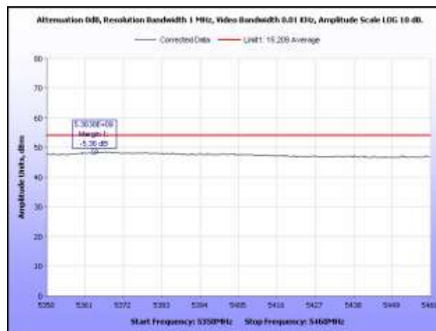
Plot 406. Restricted Band, 802.11n 40 MHz, 5510 MHz, Average, Sector Antenna
