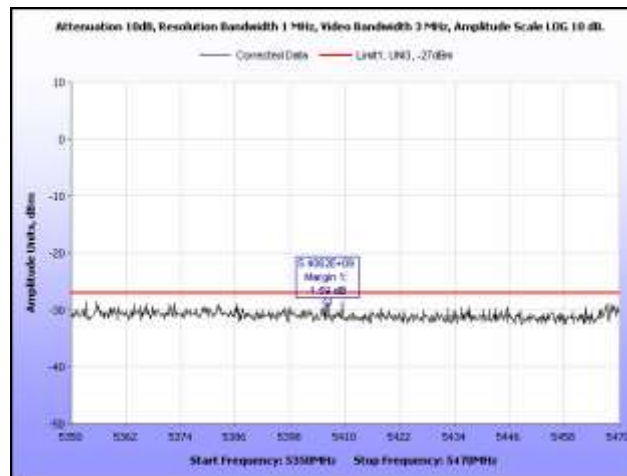
Plot 378. EIRP, 802.11n 20 MHz, 5500 MHz, Band Edge, Sector Antenna
