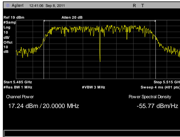
Plot 81. Conducted Output Power, 802.11n 20 MHz, Port B, 5500 MHz
