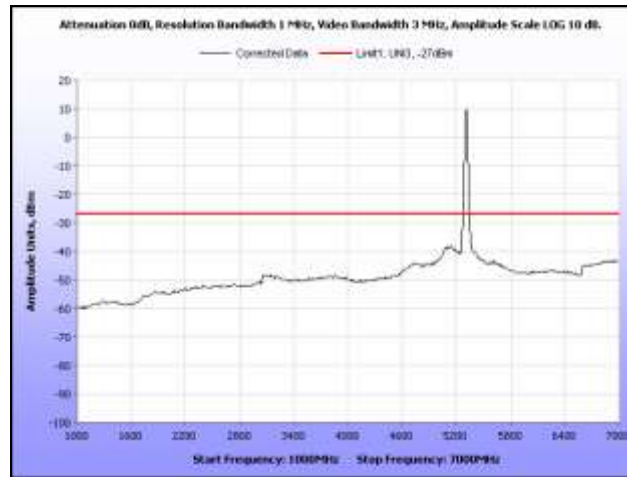
Plot 345. Radiated Spurious, 802.11n 40 MHz, 5310 MHz, 1 GHz – 7 GHz, Sector Antenna
