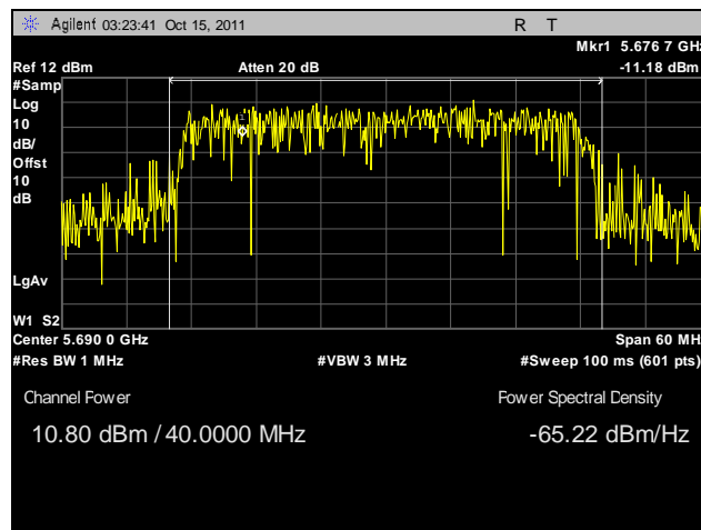
Plot 95. Conducted Output Power, 802.11n 40 MHz, Port B, 5690 MHz
