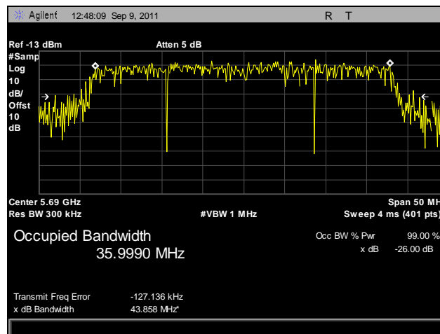
Plot 59. 99% Occupied Bandwidth, 802.11n 40 MHz, Port A, 5690 MHz
