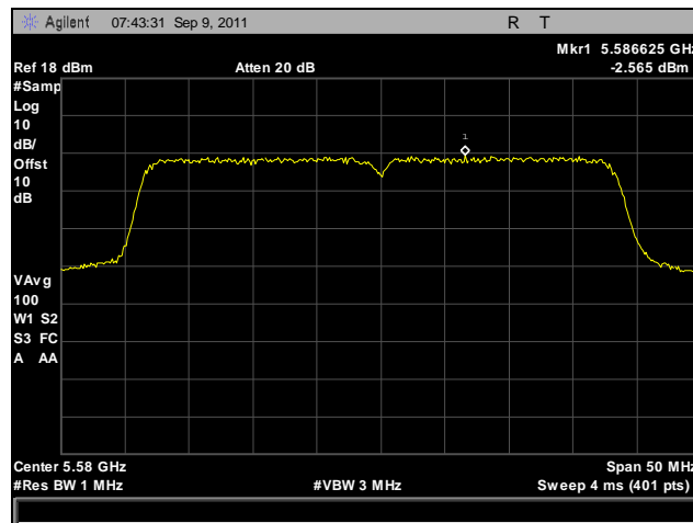
Plot 148. Peak Spectral Density, 802.11n 40 MHz, Port A, 5580 MHz
