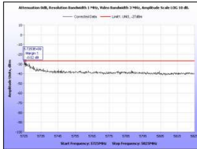
Plot 383. EIRP, 802.11n 40 MHz, 5690 MHz, Band Edge, Sector Antenna
