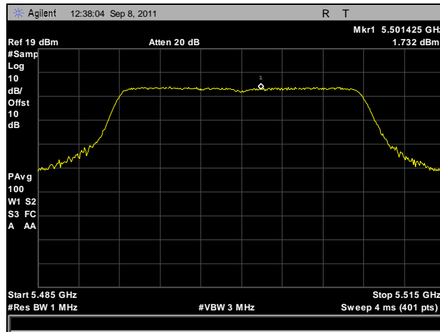
Plot 135. Peak Spectral Density, 802.11n 20 MHz, Port A, 5500 MHz
