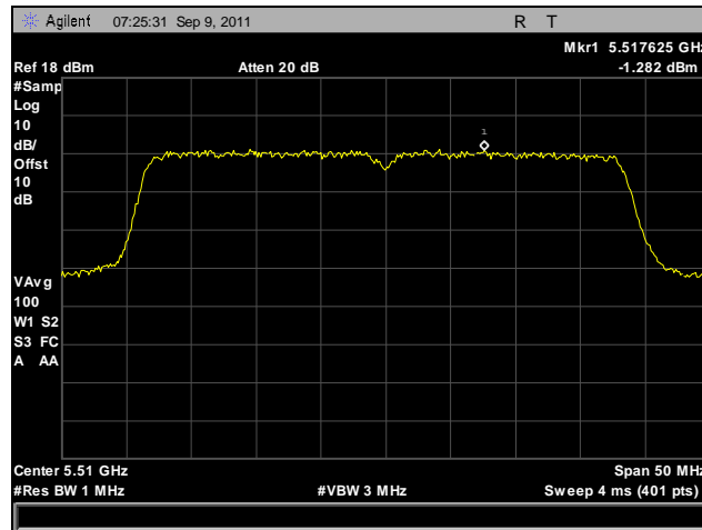
Plot 147. Peak Spectral Density, 802.11n 40 MHz, Port A, 5510 MHz
