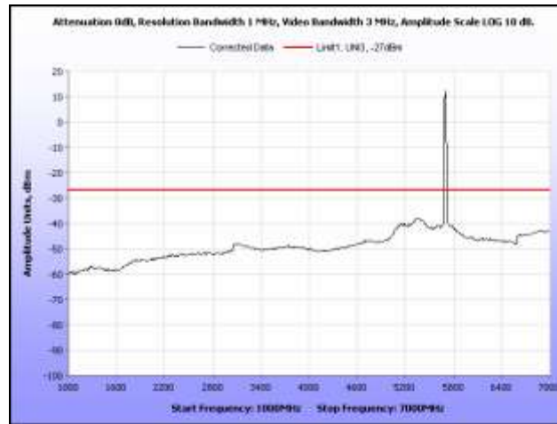
Plot 333. Radiated Spurious, 802.11n 20 MHz, 5700 MHz, 1 GHz – 7 GHz, Sector Antenna
