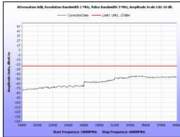
Plot 243. Radiated Spurious, 802.11n 20 MHz, 5260 MHz, 18 GHz – 40 GHz, Omni Antenna
