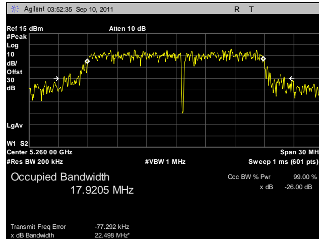
Plot 12. Occupied Bandwidth, 802.11n 20 MHz, Port A, 5260 MHz
