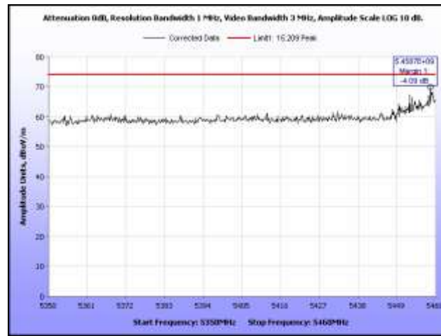
Plot 387. Restricted Band, 802.11a, 5500 MHz, Peak, Omni Antenna
