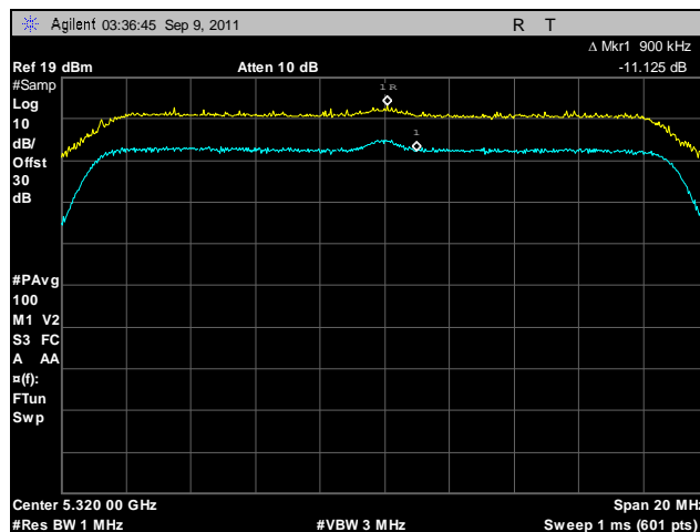
Plot 200. Peak Excursion, 802.11n 20 MHz, Port B, 5320 MHz
