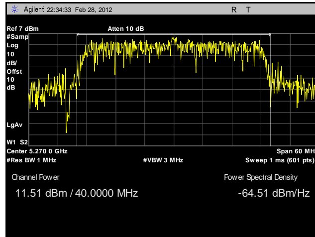
Plot 120. Conducted Output Power, 802.11n 40 MHz, Port B, 5270 MHz, Sector Antenna
