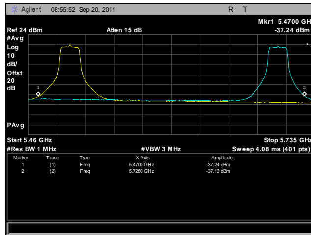
Plot 450. Frequency Stability, 802.11n 20 MHz, 5470 MHz – 5725 MHz @ 55°C, 120 V
