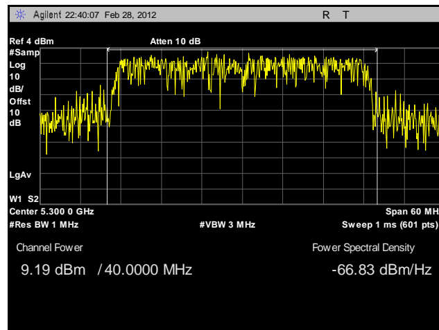
Plot 115. Conducted Output Power, 802.11n 40 MHz, Port A, 5300 MHz, Sector Antenna
