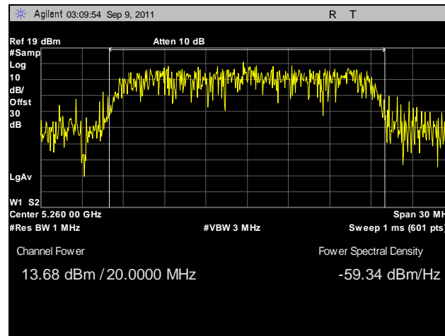
Plot 78. Conducted Output Power, 802.11n 20 MHz, Port B, 5260 MHz
