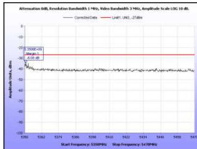
Plot 365. EIRP, 802.11n 20 MHz, 5320 MHz, Band Edge, Omni Antenna
