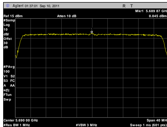
Plot 155. Peak Spectral Density, 802.11n 40 MHz, Port B, 5690 MHz
