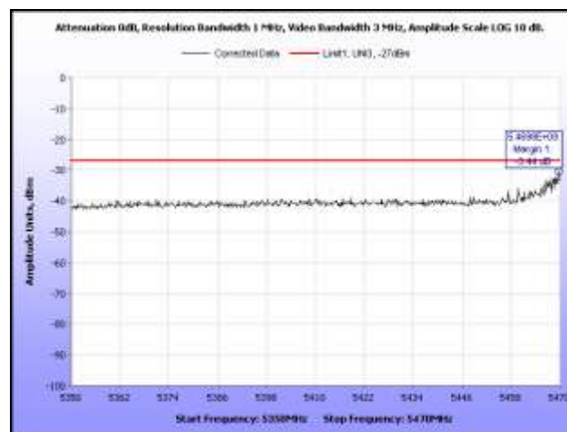
Plot 366. EIRP, 802.11n 20 MHz, 5500 MHz, Band Edge, Omni Antenna
