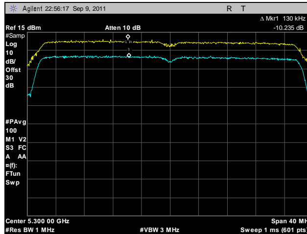
Plot 205. Peak Excursion, 802.11n 40 MHz, Port A, 5300 MHz
