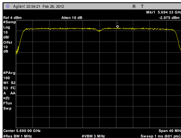
Plot 179. Peak Spectral Density, 802.11n 40 MHz, Port A, 5690 MHz, Sector Antenna
