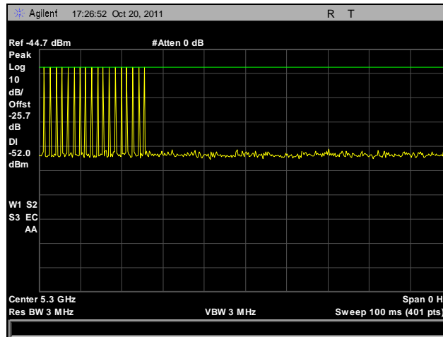
Plot 477. Radar Calibration, Bin 1
