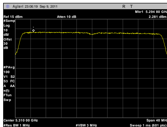
Plot 146. Peak Spectral Density, 802.11n 40 MHz, Port A, 5310 MHz
