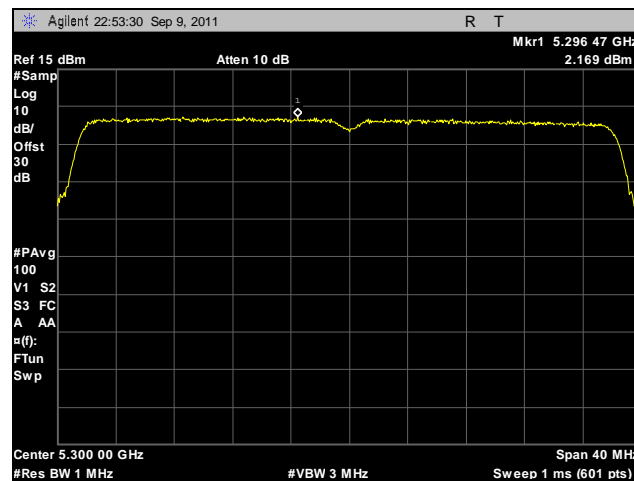
Plot 145. Peak Spectral Density, 802.11n 40 MHz, Port A, 5300 MHz
