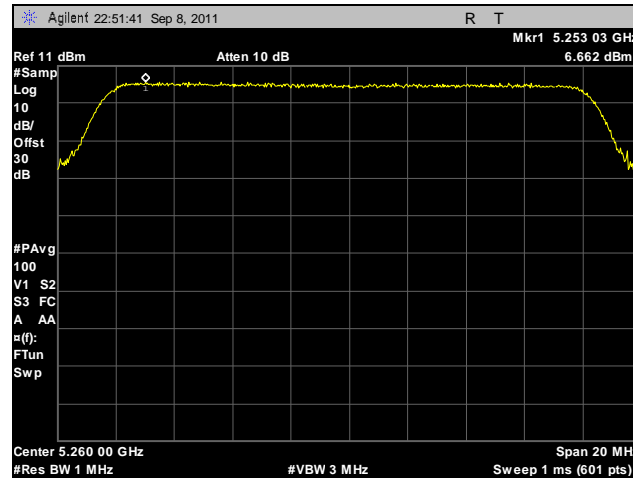
Plot 126. Peak Spectral Density, 802.11a, 5260 MHz
