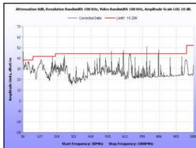
Plot 356. Radiated Spurious, 802.11n 40 MHz, 5690 MHz, 30 MHz – 1 GHz, Sector Antenna
