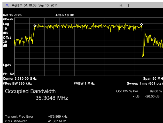
Plot 28. Occupied Bandwidth, 802.11n 40 MHz, Port A, 5580 MHz
