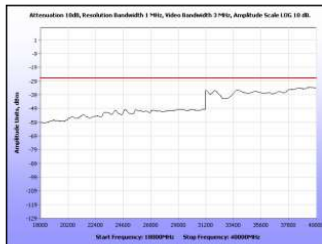
Plot 335. Radiated Spurious, 802.11n 20 MHz, 5700 MHz, 18 GHz – 40 GHz, Sector Antenna
