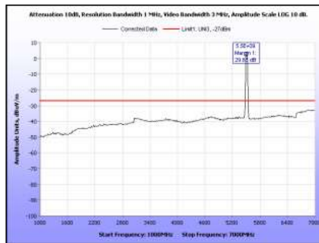
Plot 349. Radiated Spurious, 802.11n 40 MHz, 5510 MHz, 1 GHz – 7 GHz, Sector Antenna
