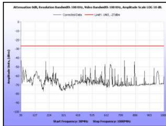
Plot 220. Radiated Spurious, 802.11a, 5300 MHz, 30 MHz – 1 GHz, Omni Antenna
