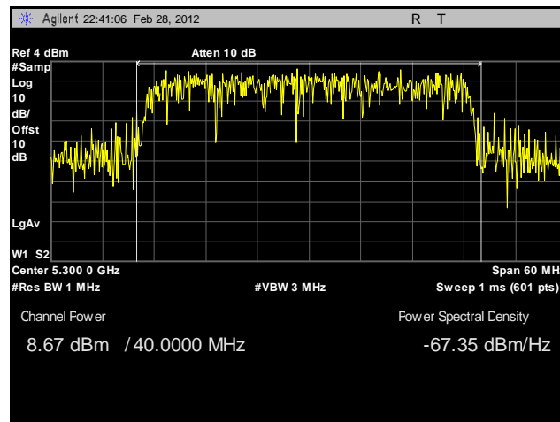
Plot 121. Conducted Output Power, 802.11n 40 MHz, Port B, 5300 MHz, Sector Antenna
