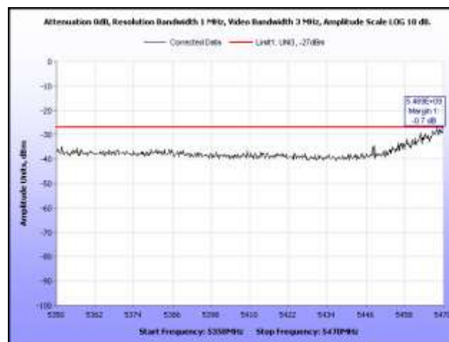
Plot 374. EIRP, 802.11a, 5500 MHz, Band Edge, Sector Antenna
