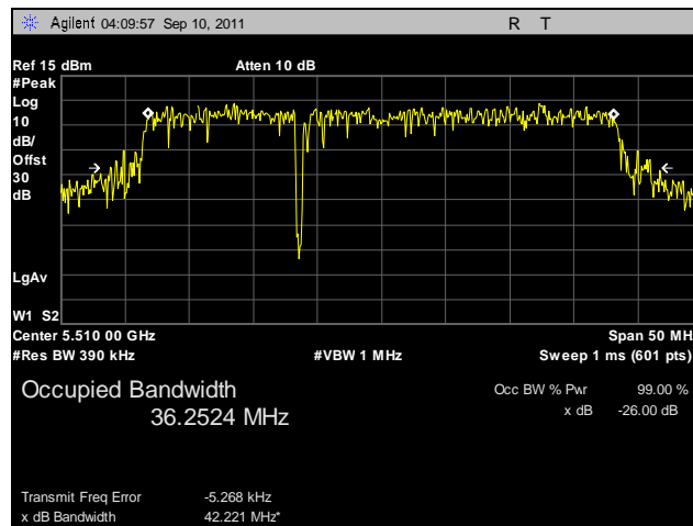
Plot 27. Occupied Bandwidth, 802.11n 40 MHz, Port A, 5510 MHz
