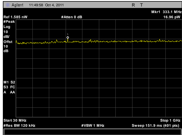
Plot 473. Receiver Spurious Emission, 5.8 GHz, 30 MHz – 1 GHz, Port A
