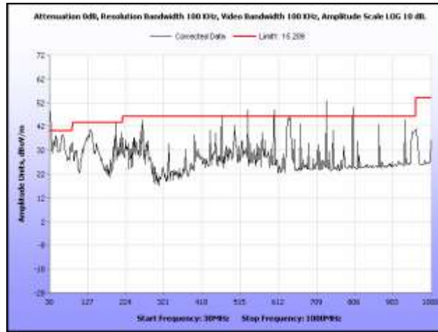
Plot 300. Radiated Spurious, 802.11a, 5500 MHz, 30 MHz – 1 GHz, Sector Antenna
