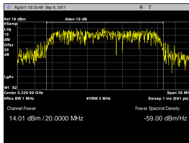
Plot 80. Conducted Output Power, 802.11n 20 MHz, Port B, 5320 MHz
