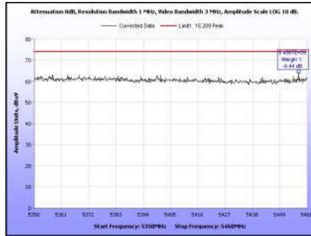
Plot 403. Restricted Band, 802.11n 20 MHz, 5500 MHz, Peak, Sector Antenna
