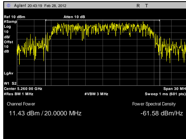
Plot 96. Conducted Output Power, 802.11a, 5260 MHz, Sector Antenna
