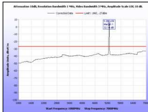
Plot 289. Radiated Spurious, 802.11a, 5260 MHz, 1 GHz – 7 GHz, Sector Antenna
