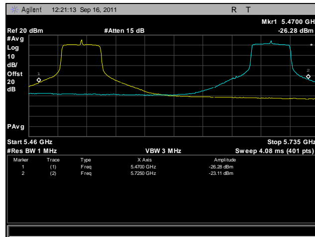
Plot 469. Frequency Stability, 802.11n 40 MHz, 5470 MHz – 5725 MHz @ 30°C, 120 V
