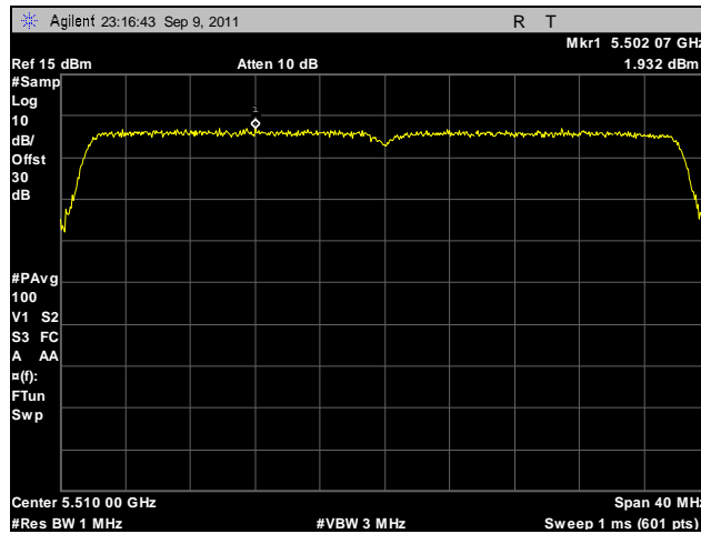
Plot 147. Peak Spectral Density, 802.11n 40 MHz, Port A, 5510 MHz
