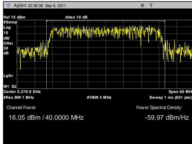
Plot 84. Conducted Output Power, 802.11n 40 MHz, Port A, 5270 MHz
