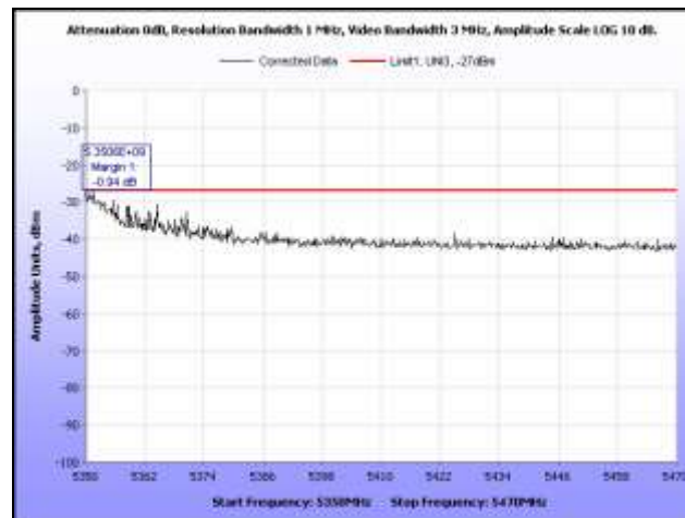
Plot 381. EIRP, 802.11n 40 MHz, 5310 MHz, Band Edge, Sector Antenna
