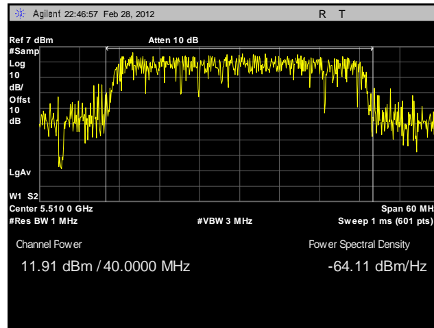
Plot 123. Conducted Output Power, 802.11n 40 MHz, Port B, 5510 MHz, Sector Antenna
