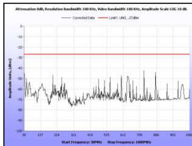
Plot 248. Radiated Spurious, 802.11n 20 MHz, 5320 MHz, 30 MHz – 1 GHz, Omni Antenna
