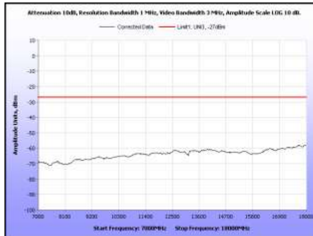
Plot 302. Radiated Spurious, 802.11a, 5500 MHz, 7 GHz – 18 GHz, Sector Antenna
