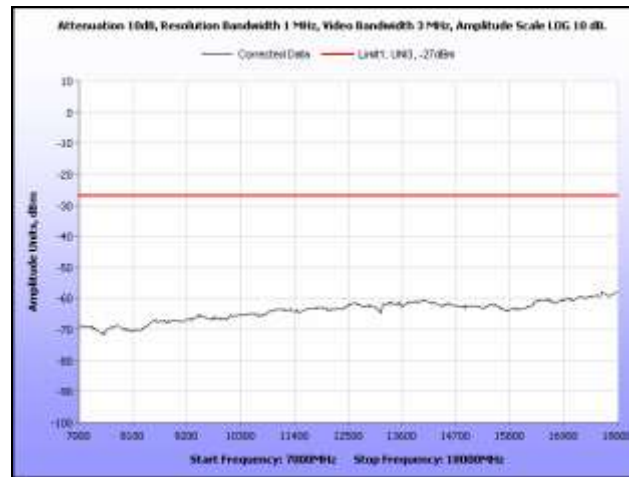
Plot 294. Radiated Spurious, 802.11a, 5300 MHz, 7 GHz – 18 GHz, Sector Antenna
