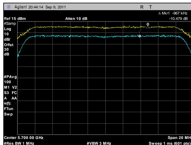
Plot 197. Peak Excursion, 802.11n 20 MHz, Port A, 5700 MHz
