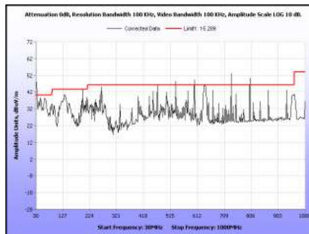
Plot 344. Radiated Spurious, 802.11n 40 MHz, 5310 MHz, 30 MHz – 1 GHz, Sector Antenna
