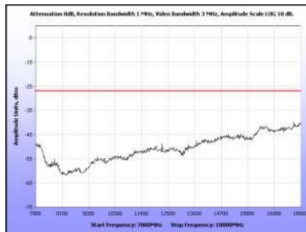
Plot 230. Radiated Spurious, 802.11a, 5500 MHz, 7 GHz – 18 GHz, Omni Antenna
