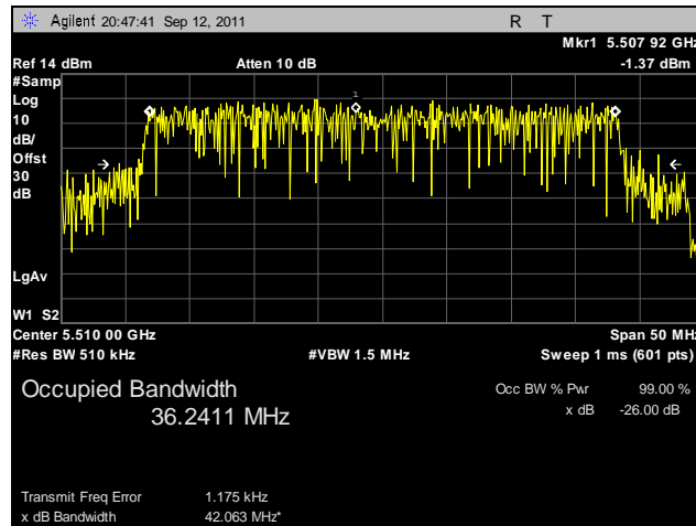
Plot 57. 99% Occupied Bandwidth, 802.11n 40 MHz, Port A, 5510 MHz
