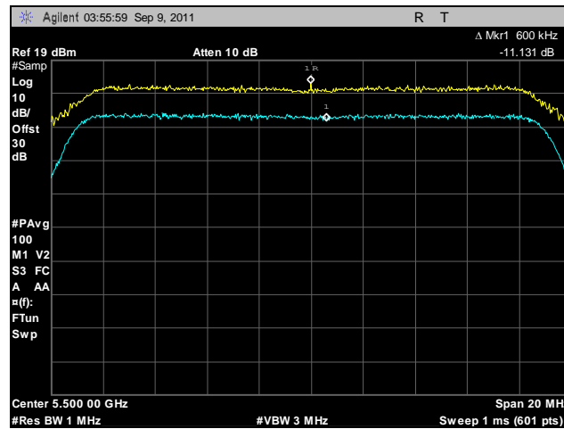
Plot 195. Peak Excursion, 802.11n 20 MHz, Port A, 5500 MHz
