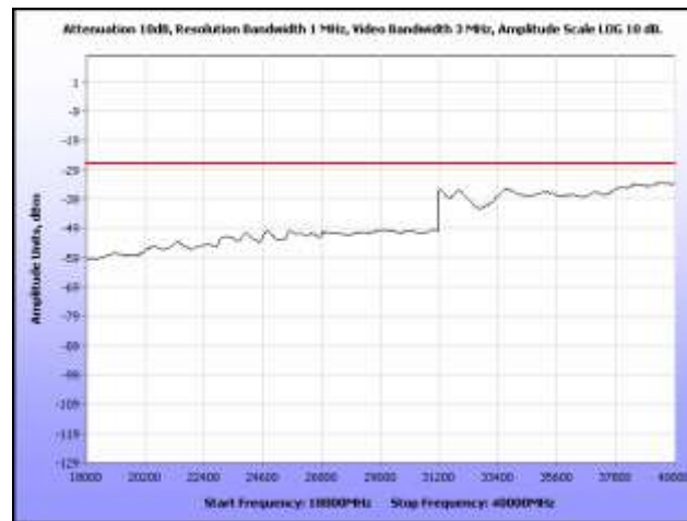
Plot 355. Radiated Spurious, 802.11n 40 MHz, 5580 MHz, 18 GHz – 40 GHz, Sector Antenna
