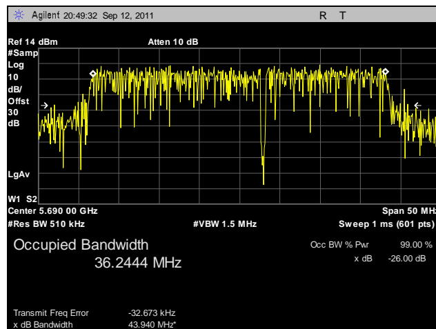
Plot 59. 99% Occupied Bandwidth, 802.11n 40 MHz, Port A, 5690 MHz
