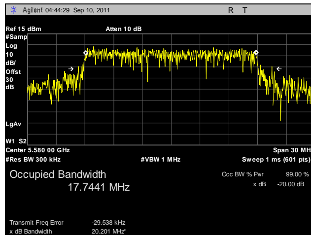
Plot 46. 99% Occupied Bandwidth, 802.11n 20 MHz, Port A, 5580 MHz
