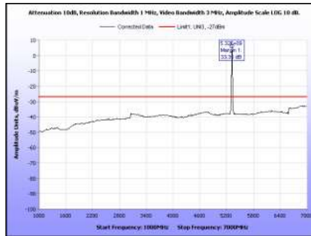
Plot 297. Radiated Spurious, 802.11a, 5320 MHz, 1 GHz – 7 GHz, Sector Antenna
