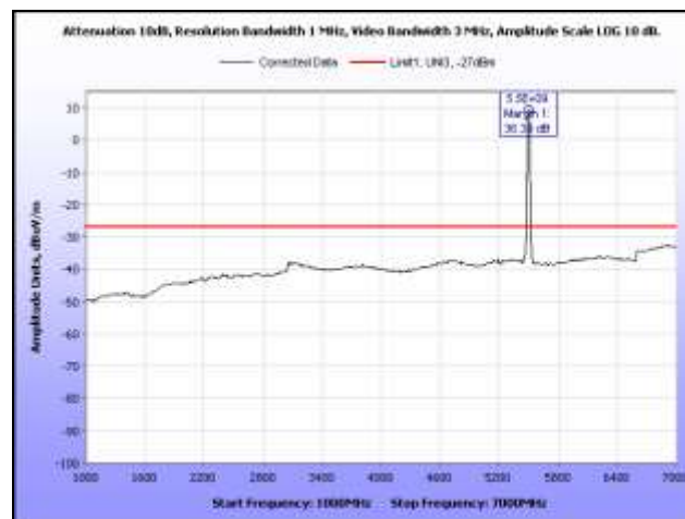
Plot 325. Radiated Spurious, 802.11n 20 MHz, 5500 MHz, 1 GHz – 7 GHz, Sector Antenna
