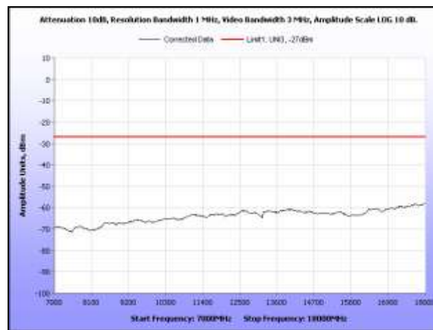
Plot 298. Radiated Spurious, 802.11a, 5320 MHz, 7 GHz – 18 GHz, Sector Antenna
