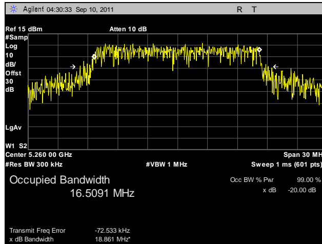
Plot 36. 99% Occupied Bandwidth, 802.11a, 5260 MHz
