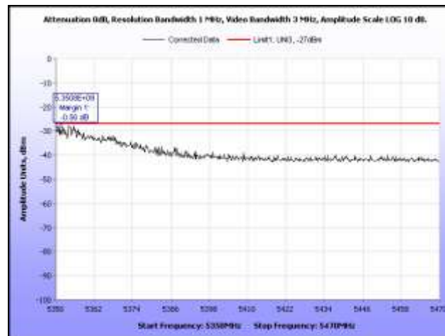
Plot 369. EIRP, 802.11n 40 MHz, 5310 MHz, Band Edge, Omni Antenna
