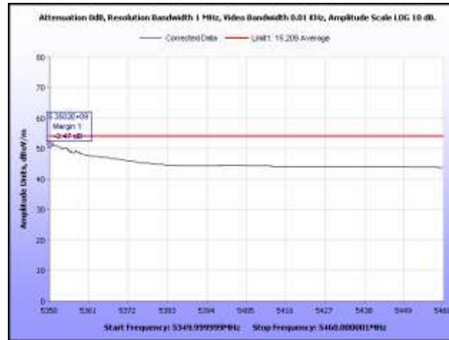
Plot 392. Restricted Band, 802.11n 40 MHz, 5310 MHz, Average, Omni Antenna
