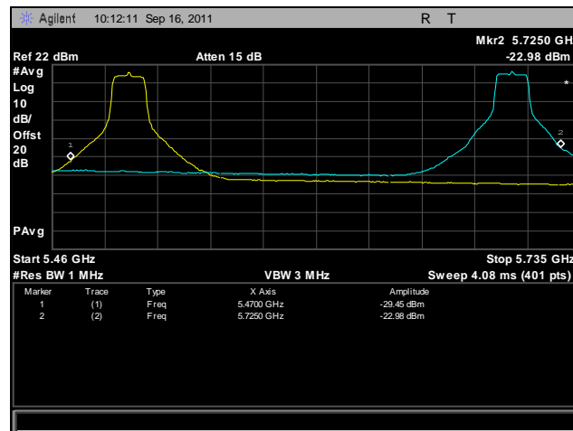
Plot 424. Frequency Stability, 802.11a, 5470 MHz – 5725 MHz @ 20°C, 132 V
