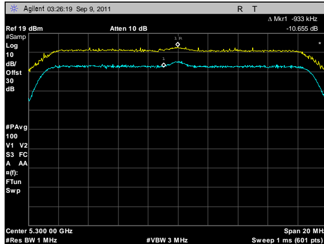
Plot 199. Peak Excursion, 802.11n 20 MHz, Port B, 5300 MHz
