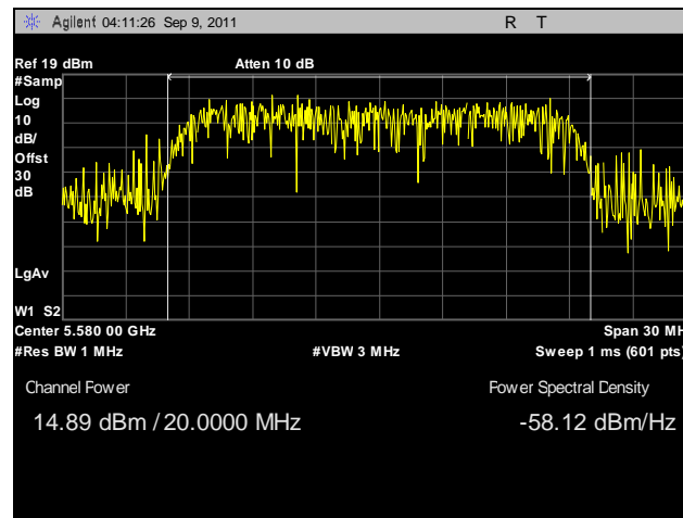
Plot 76. Conducted Output Power, 802.11n 20 MHz, Port A, 5580 MHz
