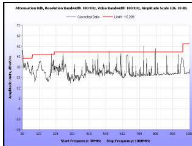
Plot 292. Radiated Spurious, 802.11a, 5300 MHz, 30 MHz – 1 GHz, Sector Antenna
