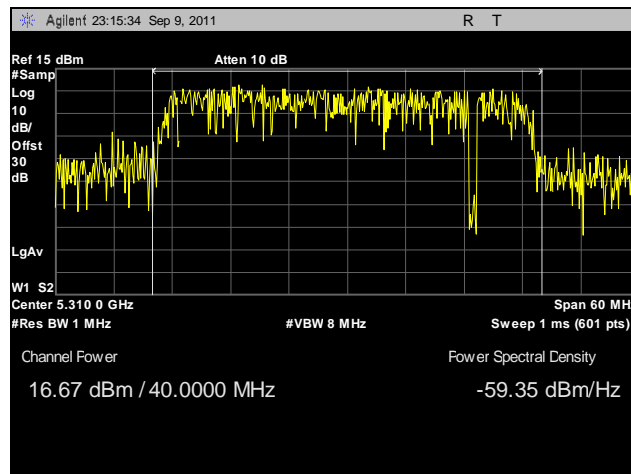
Plot 86. Conducted Output Power, 802.11n 40 MHz, Port A, 5310 MHz
