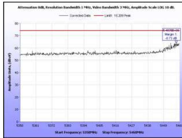
Plot 399. Restricted Band, 802.11a, 5500 MHz, Peak, Sector Antenna
