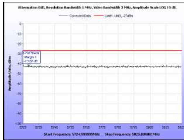
Plot 363. EIRP, 802.11a, 5700 MHz, Band Edge, Omni Antenna
