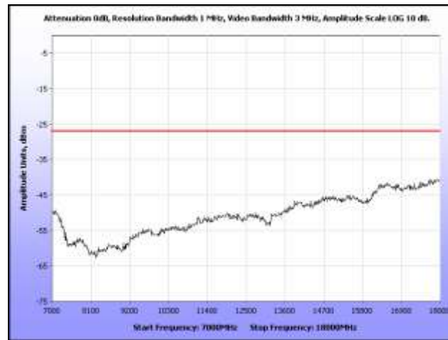
Plot 258. Radiated Spurious, 802.11n 20 MHz, 5580 MHz, 7 GHz – 18 GHz, Omni Antenna
