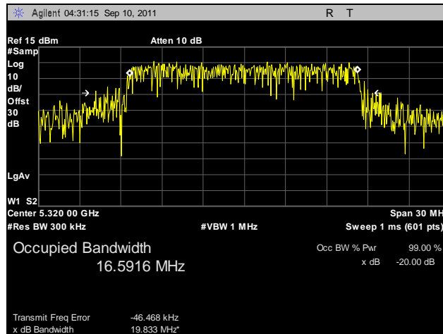
Plot 38. 99% Occupied Bandwidth, 802.11a, 5320 MHz
