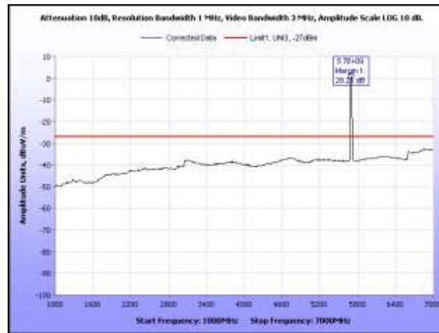
Plot 309. Radiated Spurious, 802.11a, 5700 MHz, 1 GHz – 7 GHz, Sector Antenna
