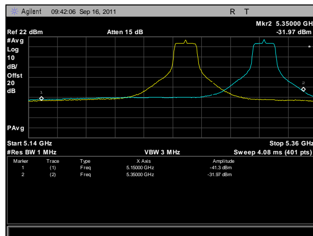
Plot 413. Frequency Stability, 802.11a, 5250 MHz – 5350 MHz @ 20°C, 132 V
