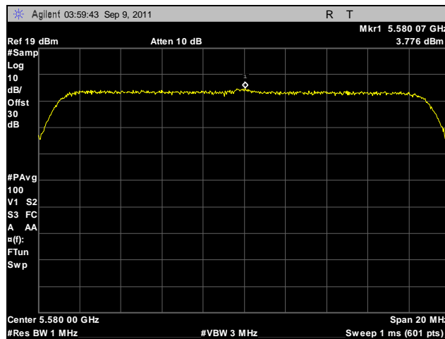
Plot 142. Peak Spectral Density, 802.11n 20 MHz, Port B, 5580 MHz
