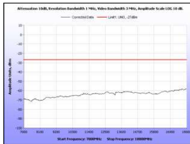
Plot 358. Radiated Spurious, 802.11n 40 MHz, 5690 MHz, 7 GHz – 18 GHz, Sector Antenna
