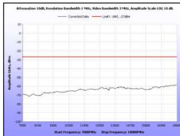
Plot 350. Radiated Spurious, 802.11n 40 MHz, 5510 MHz, 7 GHz – 18 GHz, Sector Antenna
