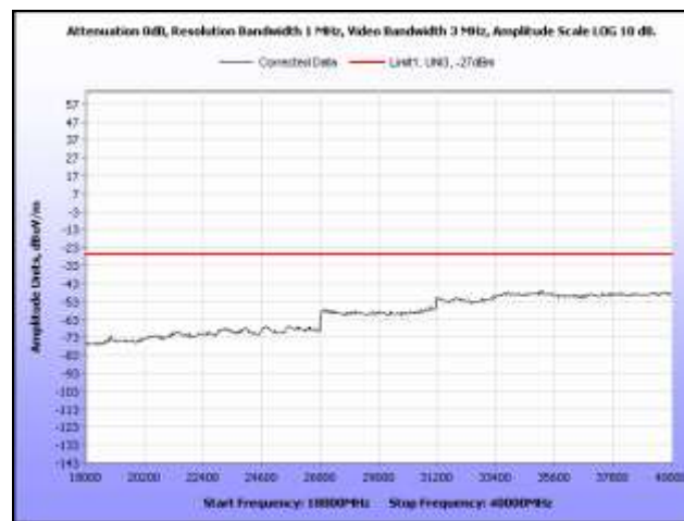
Plot 247. Radiated Spurious, 802.11n 20 MHz, 5300 MHz, 18 GHz – 40 GHz, Omni Antenna
