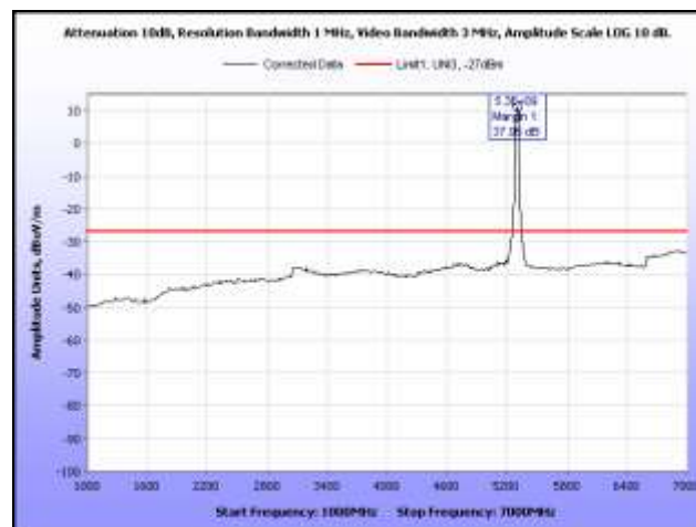
Plot 341. Radiated Spurious, 802.11n 40 MHz, 5300 MHz, 1 GHz – 7 GHz, Sector Antenna
