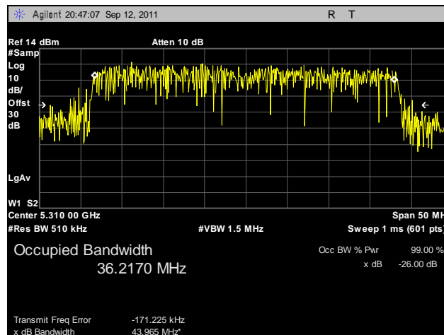
Plot 56. 99% Occupied Bandwidth, 802.11n 40 MHz, Port A, 5310 MHz
