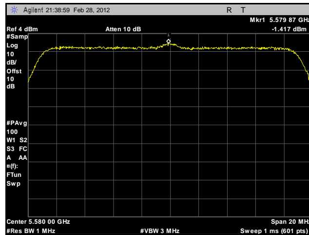
Plot 172. Peak Spectral Density, 802.11n 20 MHz, Port B, 5580 MHz, Sector Antenna
