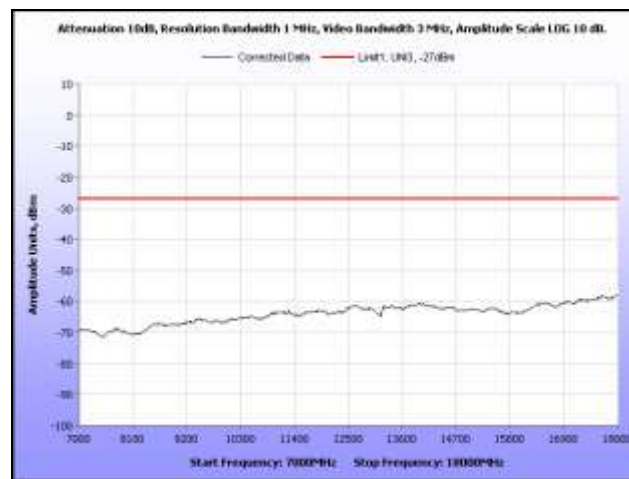
Plot 346. Radiated Spurious, 802.11n 40 MHz, 5310 MHz, 7 GHz – 18 GHz, Sector Antenna
