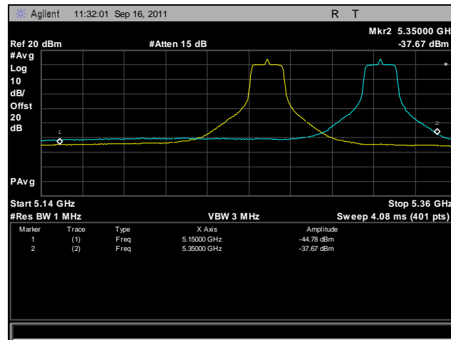
Plot 414. Frequency Stability, 802.11a, 5250 MHz – 5350 MHz @ 30°C, 120 V
