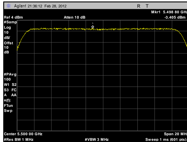
Plot 165. Peak Spectral Density, 802.11n 20 MHz, Port A, 5500 MHz, Sector Antenna
