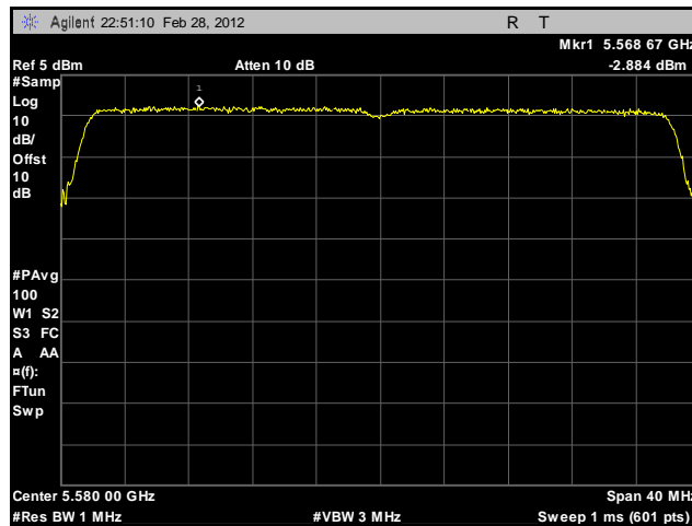
Plot 178. Peak Spectral Density, 802.11n 40 MHz, Port A, 5580 MHz, Sector Antenna
