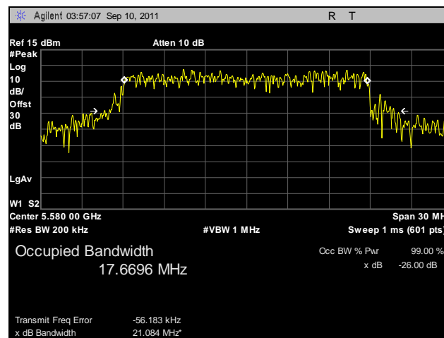
Plot 16. Occupied Bandwidth, 802.11n 20 MHz, Port A, 5580 MHz
