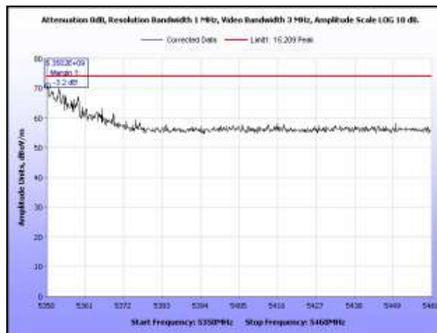
Plot 385. Restricted Band, 802.11a, 5320 MHz, Peak, Omni Antenna
