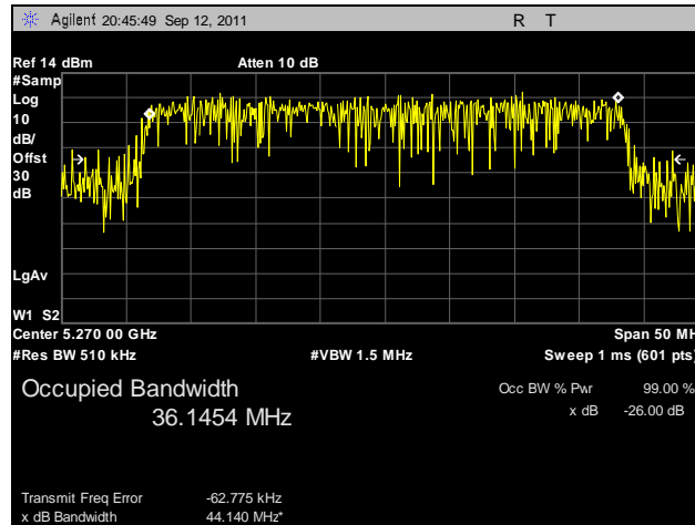
Plot 54. 99% Occupied Bandwidth, 802.11n 40 MHz, Port A, 5270 MHz
