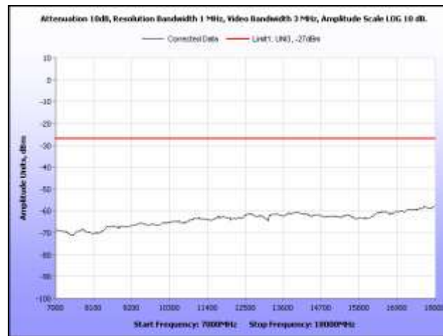
Plot 322. Radiated Spurious, 802.11n 20 MHz, 5320 MHz, 7 GHz – 18 GHz, Sector Antenna
