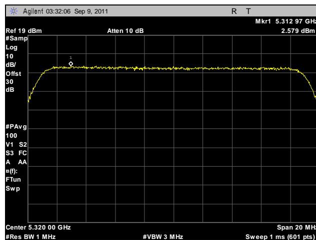
Plot 134. Peak Spectral Density, 802.11n 20 MHz, Port A, 5320 MHz
