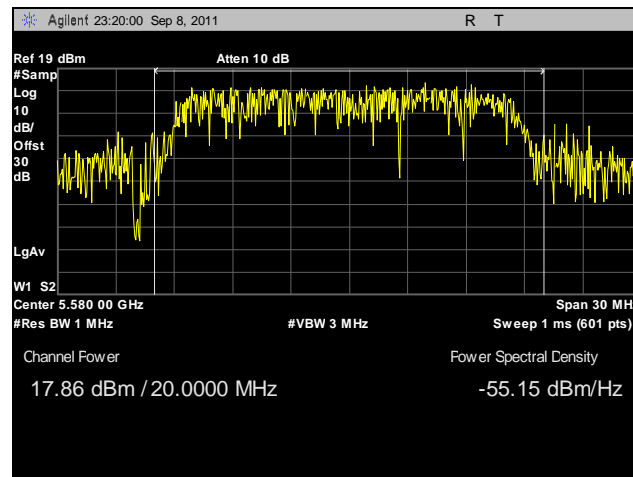
Plot 70. Conducted Output Power, 802.11a, 5580 MHz
