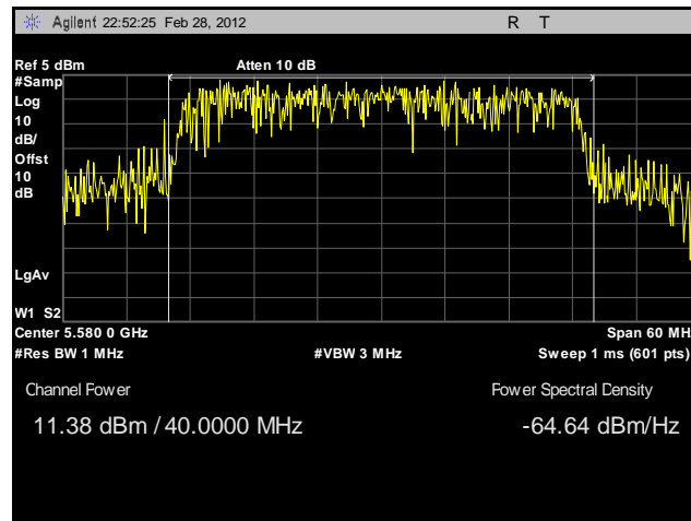
Plot 124. Conducted Output Power, 802.11n 40 MHz, Port B, 5580 MHz, Sector Antenna
