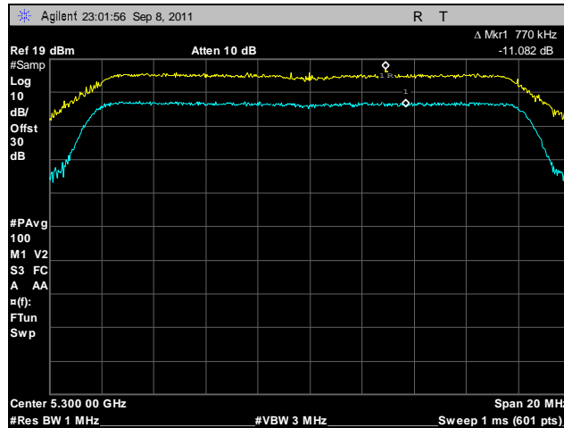
Plot 187. Peak Excursion, 802.11a, 5300 MHz
