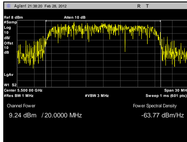
Plot 111. Conducted Output Power, 802.11n 20 MHz, Port B, 5500 MHz, Sector Antenna
