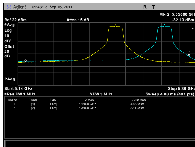
Plot 412. Frequency Stability, 802.11a, 5250 MHz – 5350 MHz @ 20°C, 120 V
