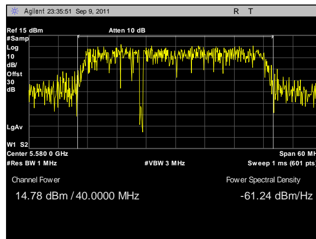
Plot 88. Conducted Output Power, 802.11n 40 MHz, Port A, 5580 MHz
