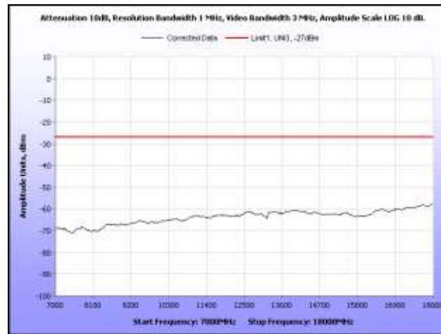
Plot 306. Radiated Spurious, 802.11a, 5580 MHz, 7 GHz – 18 GHz, Sector Antenna
