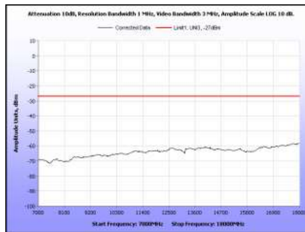
Plot 334. Radiated Spurious, 802.11n 20 MHz, 5700 MHz, 7 GHz – 18 GHz, Sector Antenna
