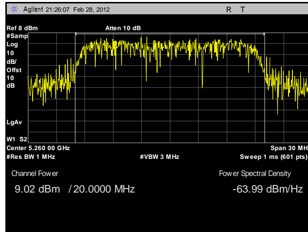
Plot 102. Conducted Output Power, 802.11n 20 MHz, Port A, 5260 MHz, Sector Antenna
