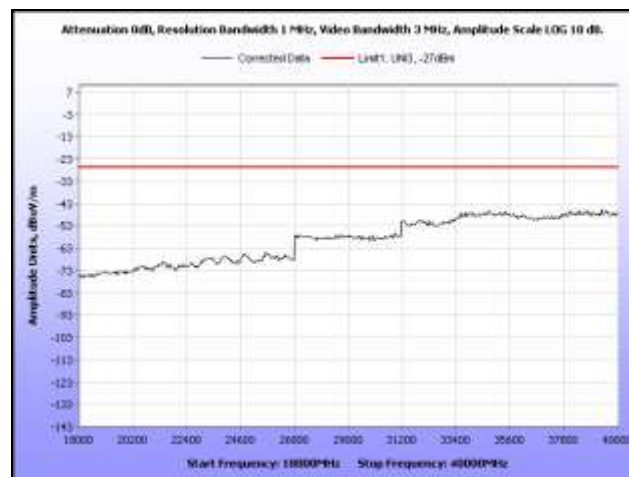
Plot 275. Radiated Spurious, 802.11n 40 MHz, 5310 MHz, 18 GHz – 40 GHz, Omni Antenna
