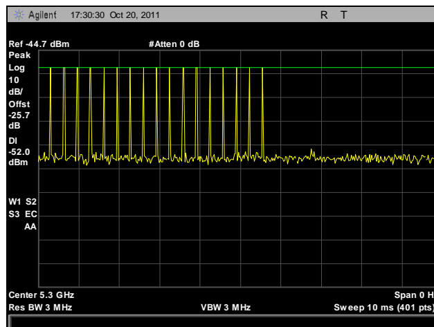
Plot 479. Radar Calibration, Bin 3
