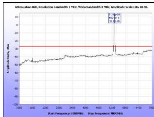
Plot 221. Radiated Spurious, 802.11a, 5300 MHz, 1 GHz – 7 GHz, Omni Antenna
