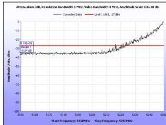
Plot 372. EIRP, 802.11a, 5260 MHz, Band Edge, Sector Antenna
