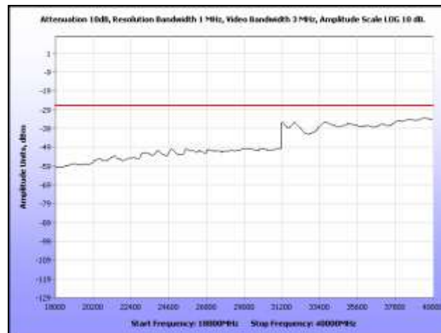
Plot 323. Radiated Spurious, 802.11n 20 MHz, 5320 MHz, 18 GHz – 40 GHz, Sector Antenna
