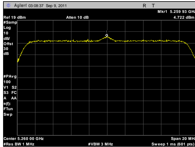
Plot 138. Peak Spectral Density, 802.11n 20 MHz, Port B, 5260 MHz
