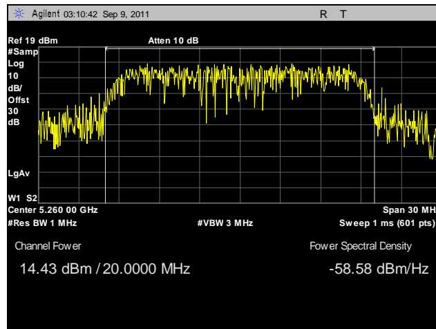
Plot 72. Conducted Output Power, 802.11n 20 MHz, Port A, 5260 MHz
