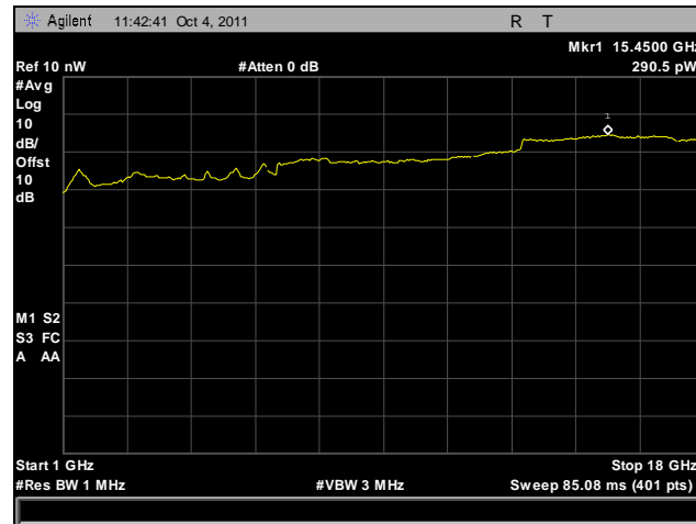
Plot 476. Receiver Spurious Emission, 5.8 GHz, 1 GHz – 18 GHz, Port B
