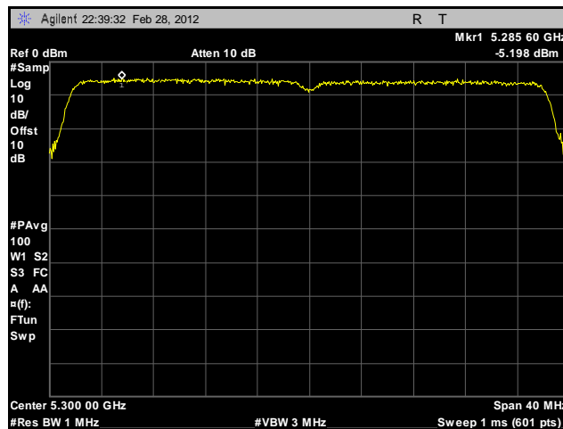
Plot 175. Peak Spectral Density, 802.11n 40 MHz, Port A, 5300 MHz, Sector Antenna
