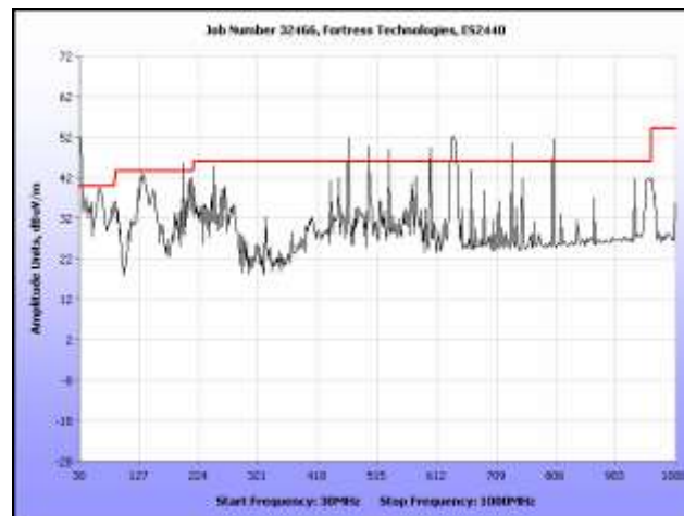
Plot 332. Radiated Spurious, 802.11n 20 MHz, 5700 MHz, 30 MHz – 1 GHz, Sector Antenna
