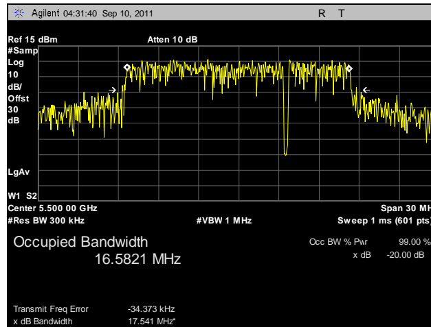
Plot 39. 99% Occupied Bandwidth, 802.11a, 5500 MHz
