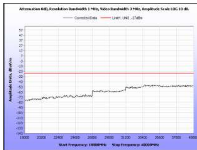
Plot 259. Radiated Spurious, 802.11n 20 MHz, 5580 MHz, 18 GHz – 40 GHz, Omni Antenna
