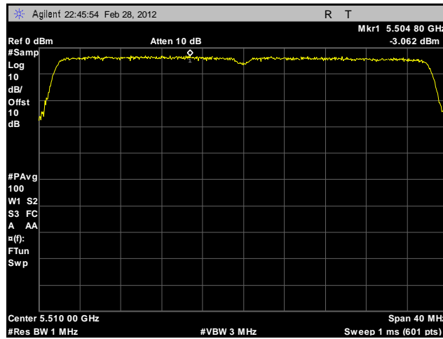
Plot 177. Peak Spectral Density, 802.11n 40 MHz, Port A, 5510 MHz, Sector Antenna
