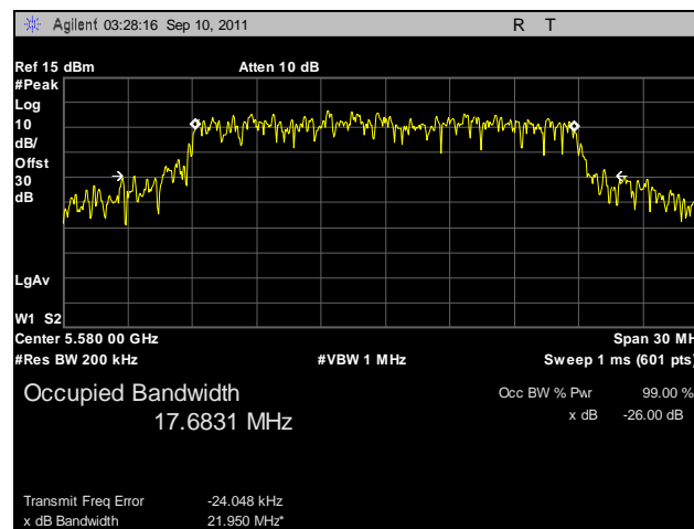
Plot 22. Occupied Bandwidth, 802.11n 20 MHz, Port B, 5580 MHz
