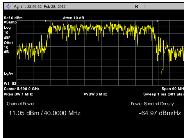
Plot 119. Conducted Output Power, 802.11n 40 MHz, Port A, 5690 MHz, Sector Antenna
