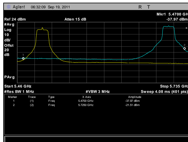
Plot 443. Frequency Stability, 802.11n 20 MHz, 5470 MHz – 5725 MHz @ 10°C, 120 V
