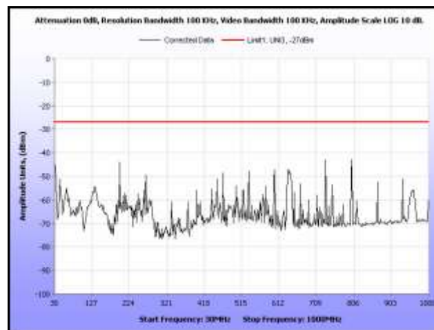
Plot 268. Radiated Spurious, 802.11n 40 MHz, 5300 MHz, 30 MHz – 1 GHz, Omni Antenna
