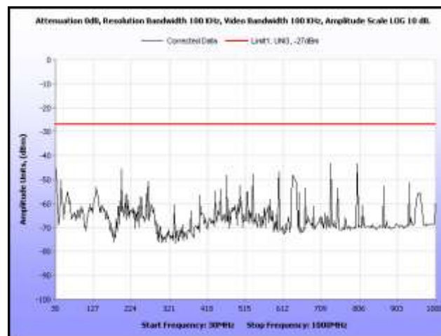
Plot 256. Radiated Spurious, 802.11n 20 MHz, 5580 MHz, 30 MHz – 1 GHz, Omni Antenna
