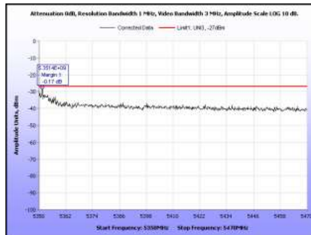
Plot 377. EIRP, 802.11n 20 MHz, 5320 MHz, Band Edge, Sector Antenna
