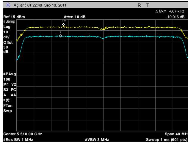
Plot 207. Peak Excursion, 802.11n 40 MHz, Port A, 5510 MHz
