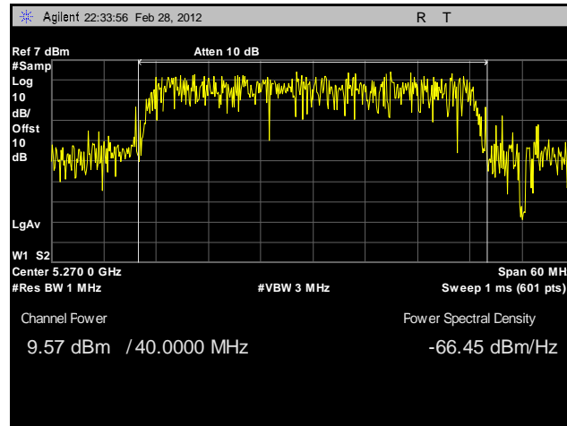
Plot 114. Conducted Output Power, 802.11n 40 MHz, Port A, 5270 MHz, Sector Antenna
