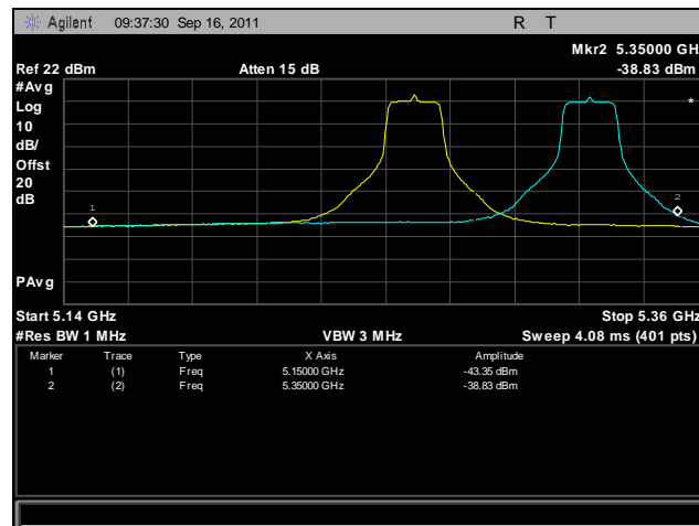
Plot 433. Frequency Stability, 802.11n 20 MHz, 5250 MHz – 5350 MHz @ 20°C, 108 V
