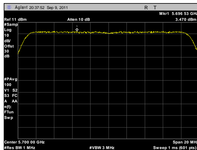
Plot 137. Peak Spectral Density, 802.11n 20 MHz, Port A, 5700 MHz
