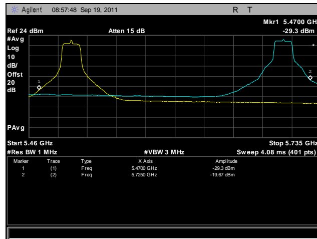
Plot 420. Frequency Stability, 802.11a, 5470 MHz – 5725 MHz @ 0°C, 120 V
