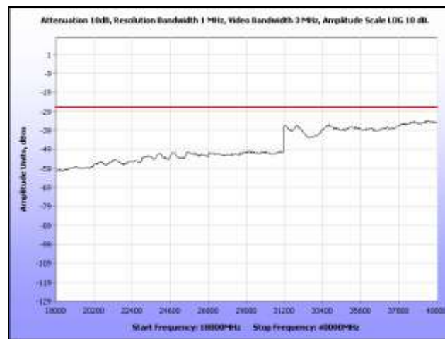
Plot 319. Radiated Spurious, 802.11n 20 MHz, 5300 MHz, 18 GHz – 40 GHz, Sector Antenna
