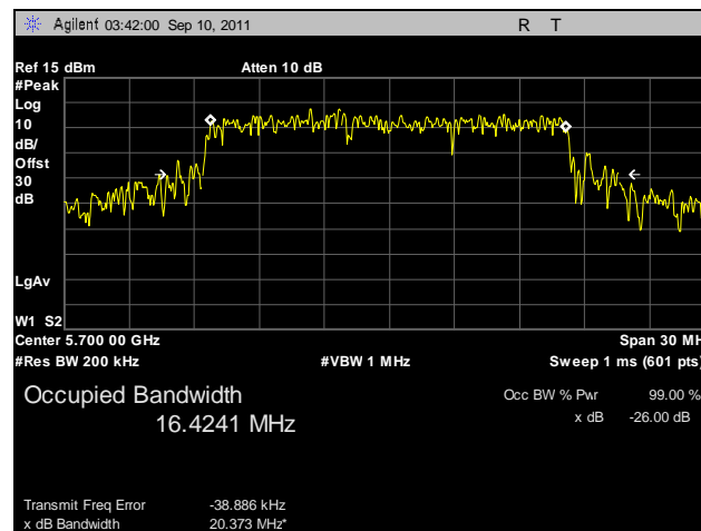
Plot 11. Occupied Bandwidth, 802.11a, 5700 MHz
