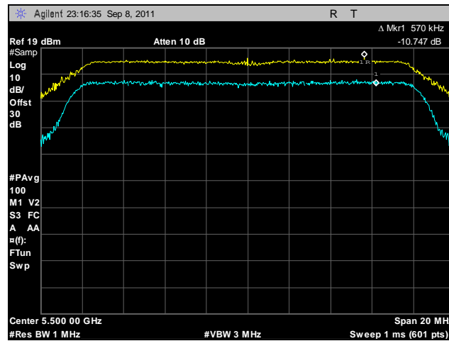
Plot 189. Peak Excursion, 802.11a, 5500 MHz
