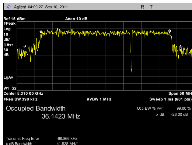
Plot 26. Occupied Bandwidth, 802.11n 40 MHz, Port A, 5310 MHz
