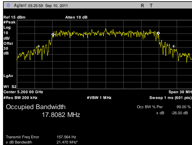
Plot 18. Occupied Bandwidth, 802.11n 20 MHz, Port B, 5260 MHz
