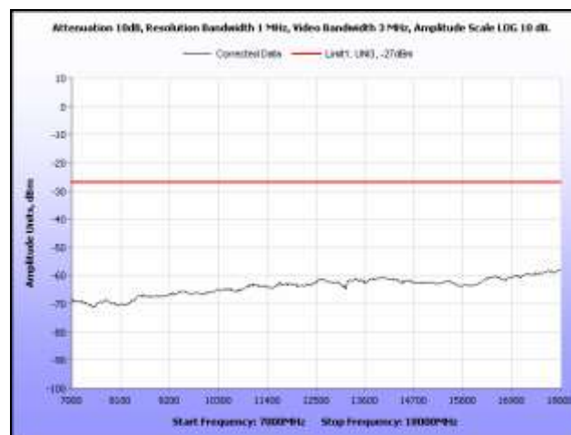
Plot 290. Radiated Spurious, 802.11a, 5260 MHz, 7 GHz – 18 GHz, Sector Antenna
