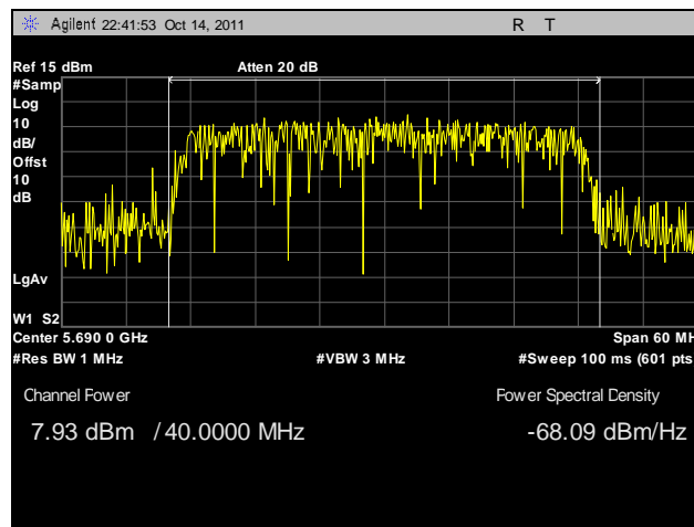
Plot 95. Conducted Output Power, 802.11n 40 MHz, Port B, 5690 MHz
