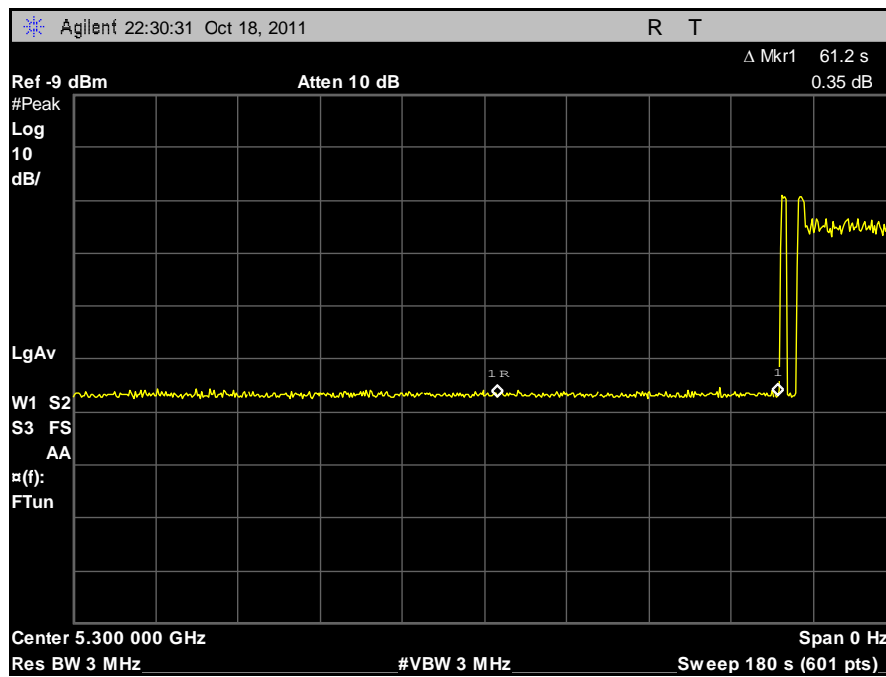
Plot 483. Initial Channel Availability Check Time
