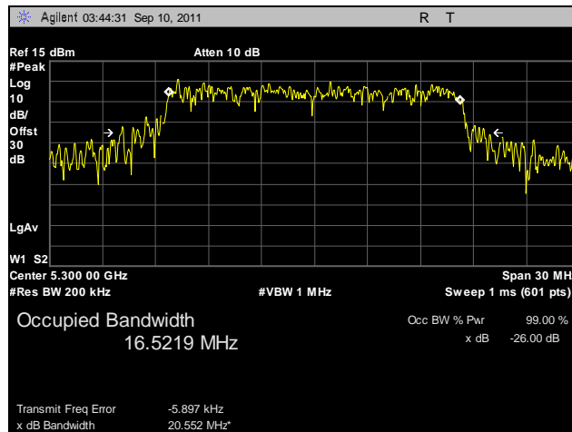
Plot 7. Occupied Bandwidth, 802.11a, 5300 MHz
