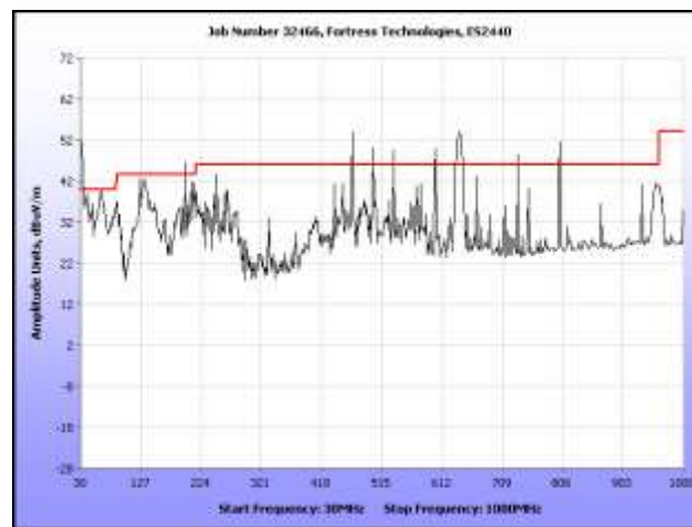
Plot 328. Radiated Spurious, 802.11n 20 MHz, 5580 MHz, 30 MHz – 1 GHz, Sector Antenna
