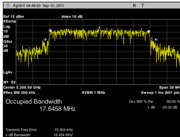
Plot 49. 99% Occupied Bandwidth, 802.11n 20 MHz, Port B, 5300 MHz
