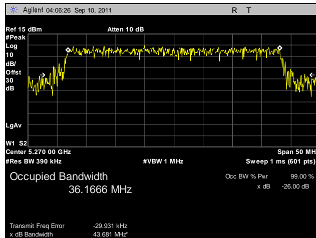
Plot 24. Occupied Bandwidth, 802.11n 40 MHz, Port A, 5270 MHz
