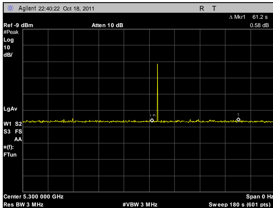
Plot 484. Radar Burst at the Beginning of CACT
