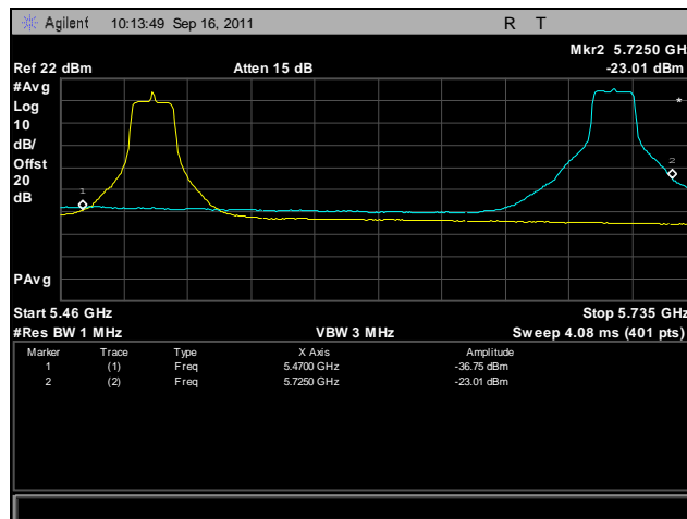
Plot 446. Frequency Stability, 802.11n 20 MHz, 5470 MHz – 5725 MHz @ 20°C, 132 V
