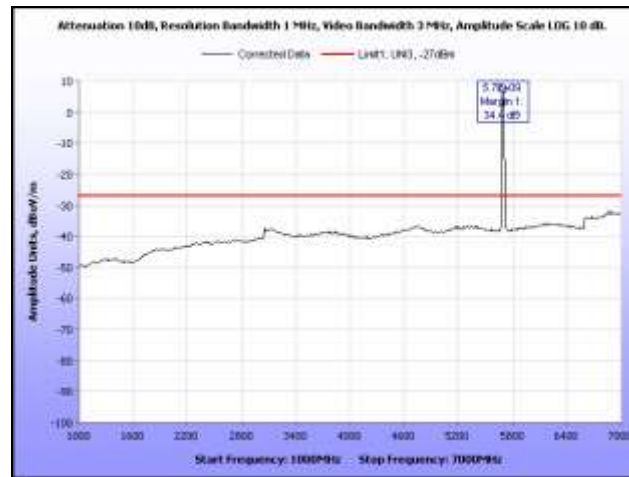
Plot 333. Radiated Spurious, 802.11n 20 MHz, 5700 MHz, 1 GHz – 7 GHz, Sector Antenna
