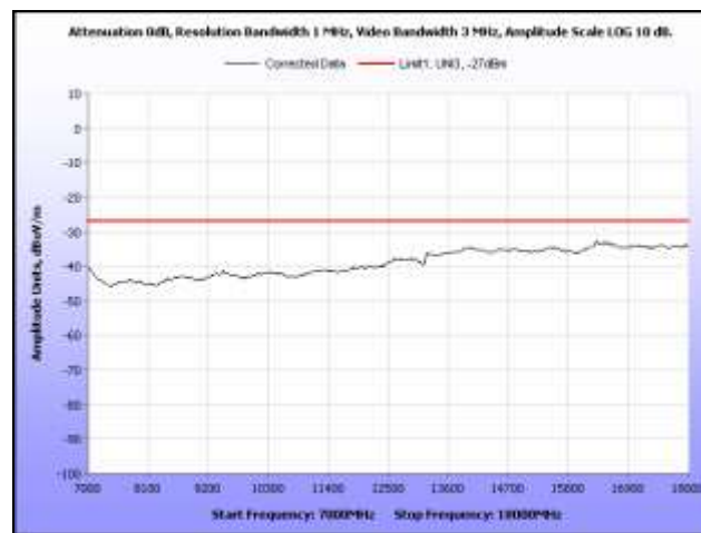
Plot 274. Radiated Spurious, 802.11n 40 MHz, 5310 MHz, 7 GHz – 18 GHz, Omni Antenna
