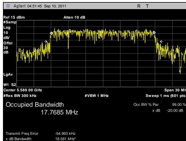
Plot 52. 99% Occupied Bandwidth, 802.11n 20 MHz, Port B, 5580 MHz
