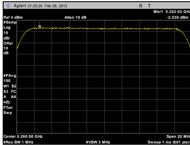
Plot 162. Peak Spectral Density, 802.11n 20 MHz, Port A, 5260 MHz, Sector Antenna
