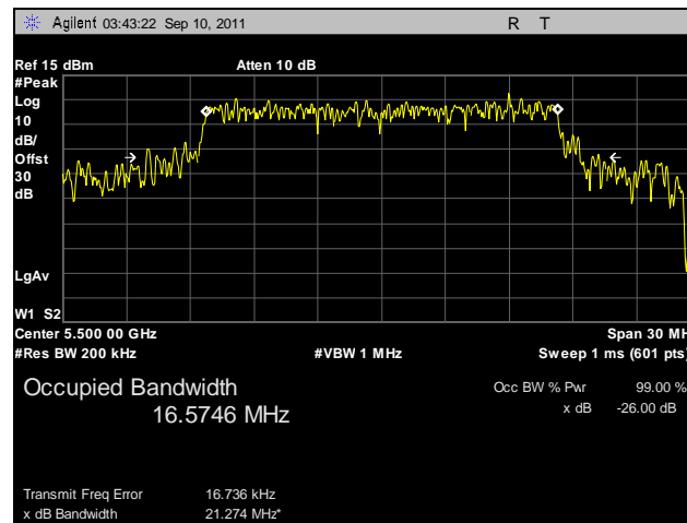
Plot 9. Occupied Bandwidth, 802.11a, 5500 MHz
