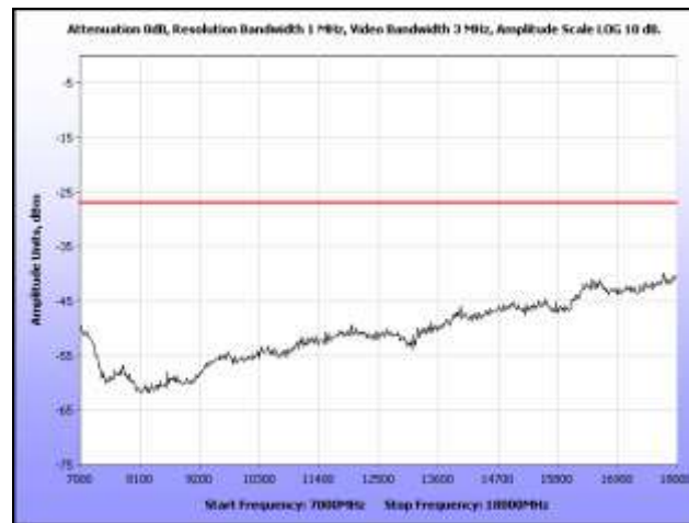
Plot 262. Radiated Spurious, 802.11n 20 MHz, 5700 MHz, 7 GHz – 18 GHz, Omni Antenna
