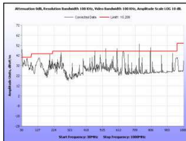
Plot 308. Radiated Spurious, 802.11a, 5700 MHz, 30 MHz – 1 GHz, Sector Antenna
