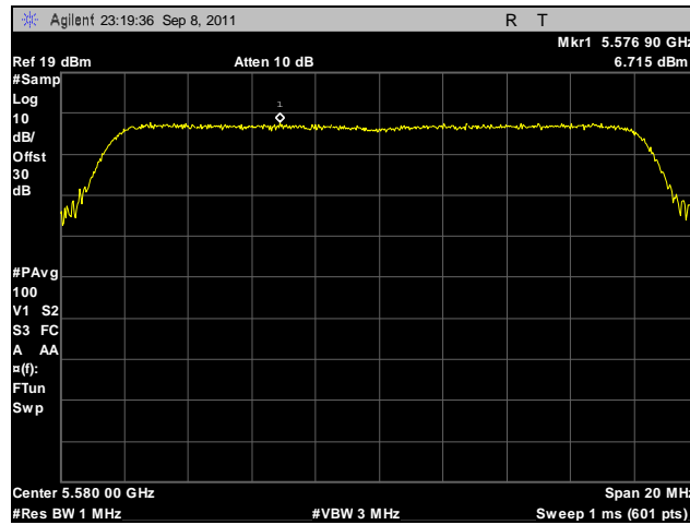
Plot 130. Peak Spectral Density, 802.11a, 5580 MHz
