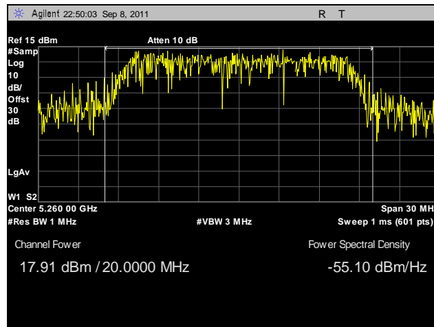
Plot 66. Conducted Output Power, 802.11a, 5260 MHz
