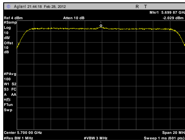
Plot 173. Peak Spectral Density, 802.11n 20 MHz, Port B, 5700 MHz, Sector Antenna
