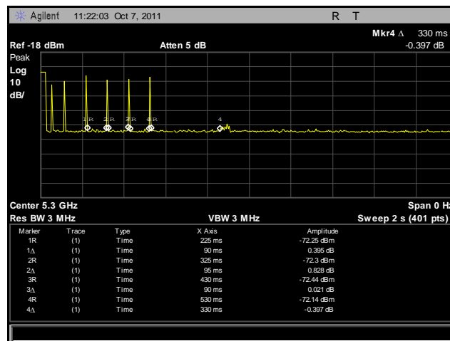
Plot 489. Channel Closing Transmission Time, 2
