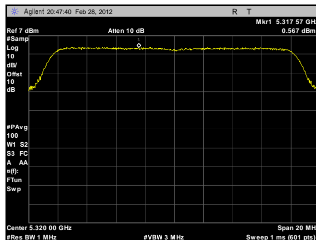
Plot 158. Peak Spectral Density, 802.11a, 5320 MHz, Sector Antenna
