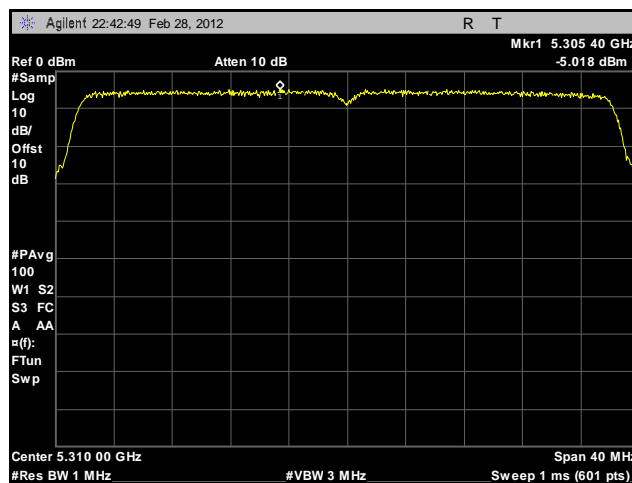
Plot 176. Peak Spectral Density, 802.11n 40 MHz, Port A, 5310 MHz, Sector Antenna
