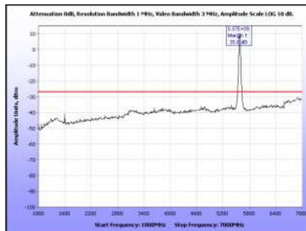
Plot 281. Radiated Spurious, 802.11n 40 MHz, 5580 MHz, 1 GHz – 7 GHz, Omni Antenna
