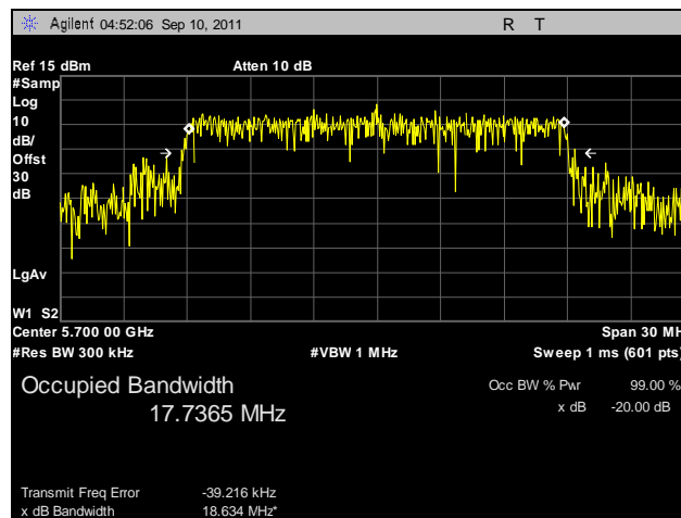
Plot 53. 99% Occupied Bandwidth, 802.11n 20 MHz, Port B, 5700 MHz
