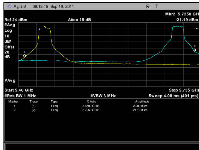
Plot 421. Frequency Stability, 802.11a, 5470 MHz – 5725 MHz @ 10°C, 120 V
