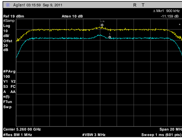
Plot 198. Peak Excursion, 802.11n 20 MHz, Port B, 5260 MHz
