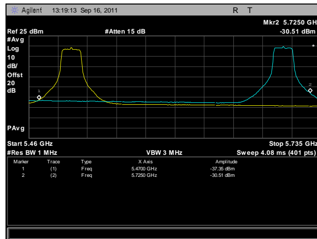
Plot 448. Frequency Stability, 802.11n 20 MHz, 5470 MHz – 5725 MHz @ 40°C, 120 V
