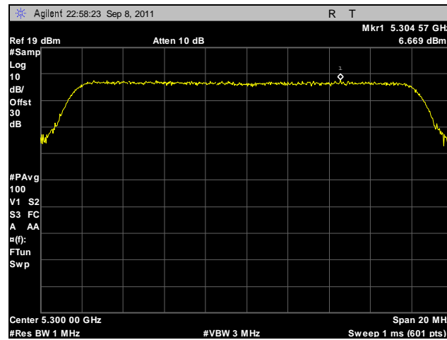
Plot 127. Peak Spectral Density, 802.11a, 5300 MHz
