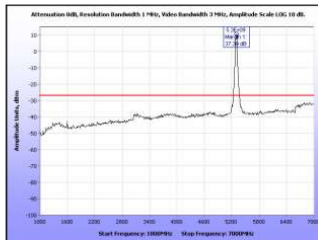
Plot 269. Radiated Spurious, 802.11n 40 MHz, 5300 MHz, 1 GHz – 7 GHz, Omni Antenna
