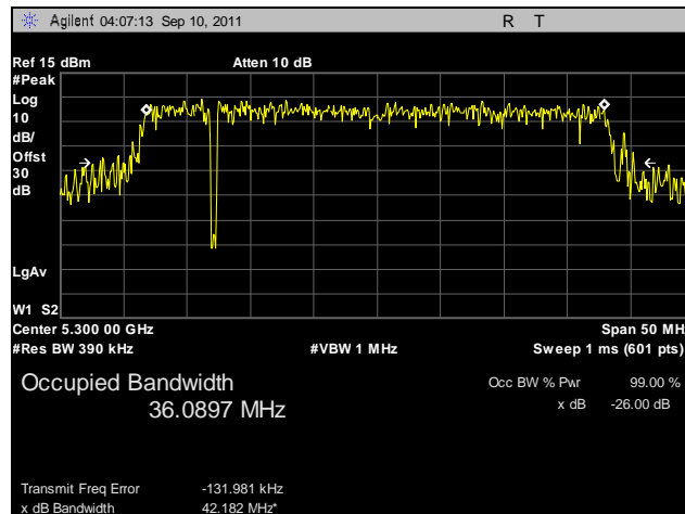
Plot 25. Occupied Bandwidth, 802.11n 40 MHz, Port A, 5300 MHz
