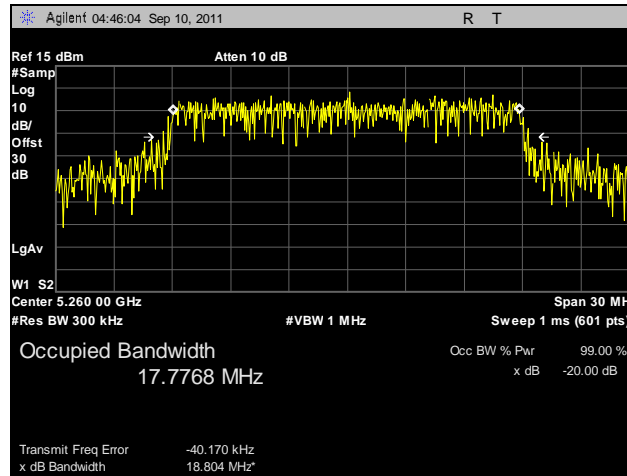
Plot 42. 99% Occupied Bandwidth, 802.11n 20 MHz, Port A, 5260 MHz
