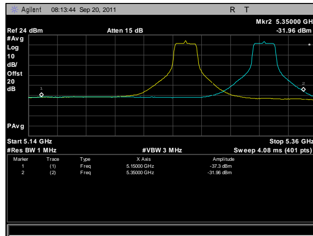
Plot 417. Frequency Stability, 802.11a, 5250 MHz – 5350 MHz @ 55°C, 120 V
