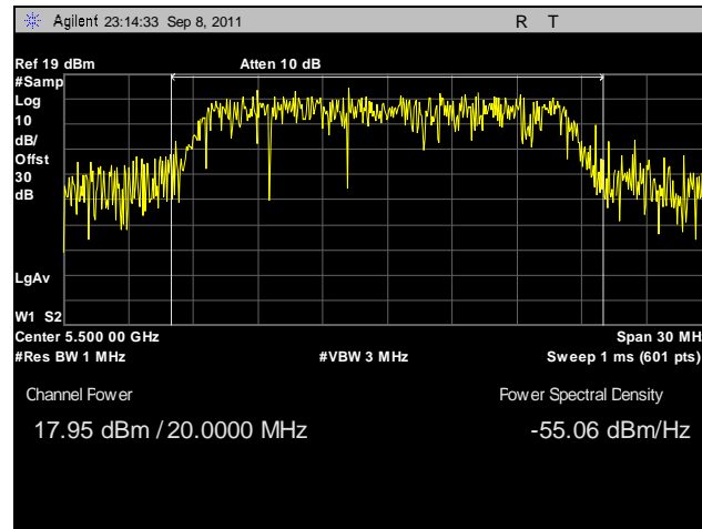
Plot 69. Conducted Output Power, 802.11a, 5500 MHz
