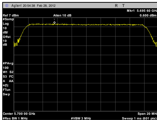
Plot 161. Peak Spectral Density, 802.11a, 5700 MHz, Sector Antenna
