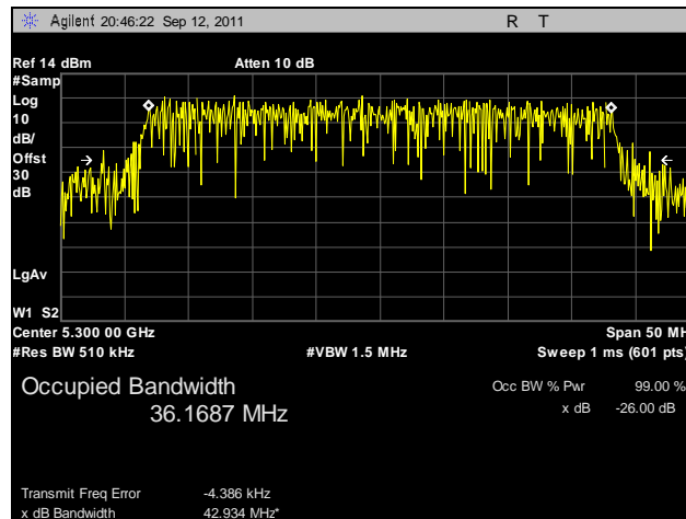
Plot 55. 99% Occupied Bandwidth, 802.11n 40 MHz, Port A, 5300 MHz
