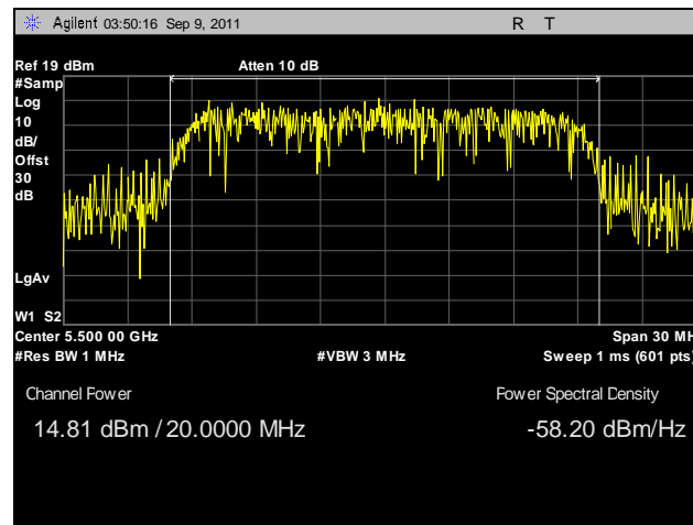
Plot 81. Conducted Output Power, 802.11n 20 MHz, Port B, 5500 MHz
