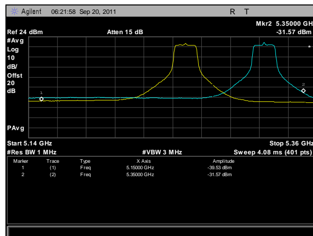
Plot 416. Frequency Stability, 802.11a, 5250 MHz – 5350 MHz @ 50°C, 120 V
