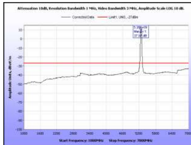
Plot 337. Radiated Spurious, 802.11n 40 MHz, 5270 MHz, 1 GHz – 7 GHz, Sector Antenna
