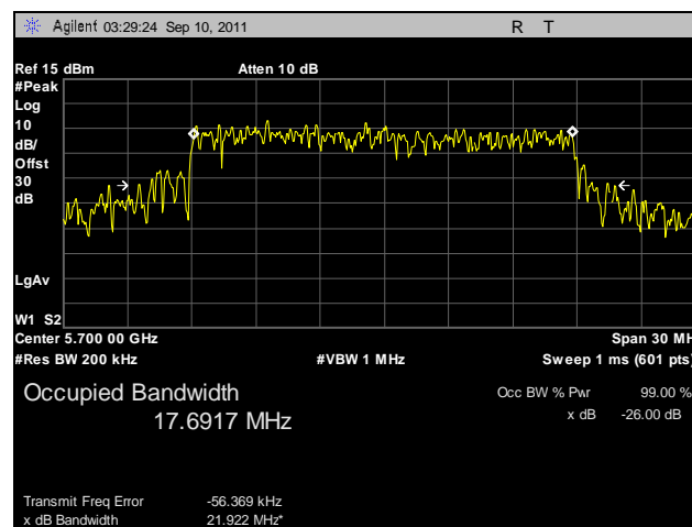
Plot 23. Occupied Bandwidth, 802.11n 20 MHz, Port B, 5700 MHz
