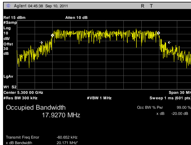
Plot 43. 99% Occupied Bandwidth, 802.11n 20 MHz, Port A, 5300 MHz
