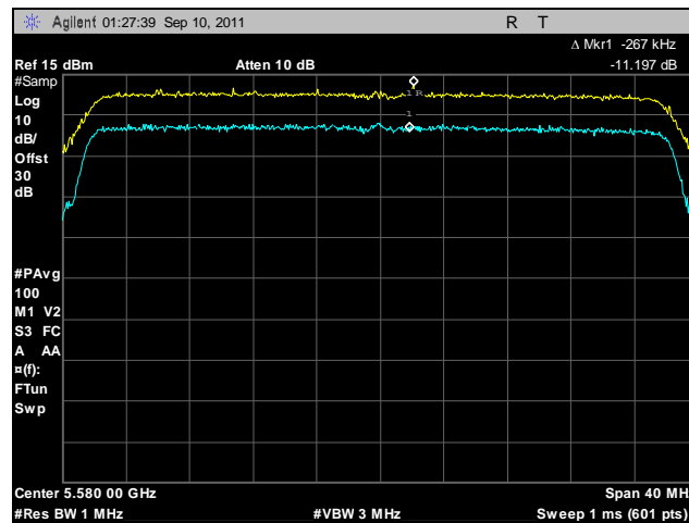
Plot 214. Peak Excursion, 802.11n 40 MHz, Port B, 5580 MHz
