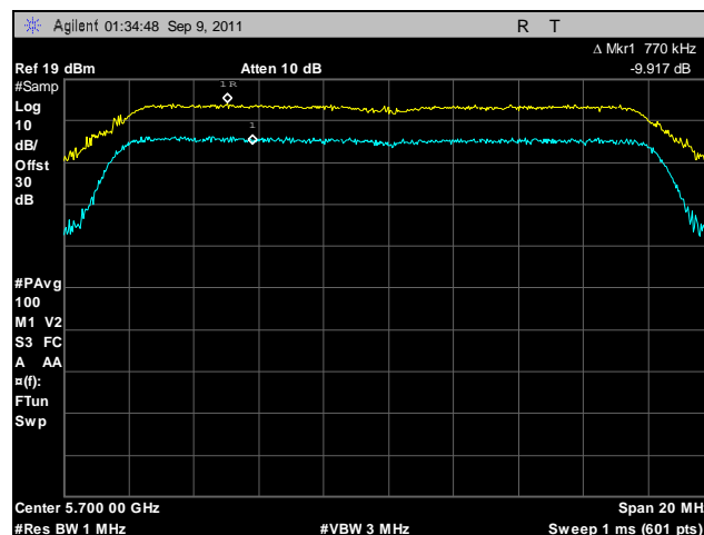
Plot 191. Peak Excursion, 802.11a, 5700 MHz
