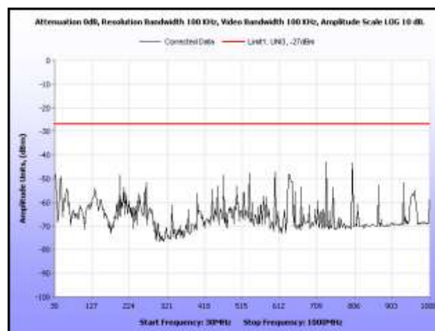
Plot 284. Radiated Spurious, 802.11n 40 MHz, 5690 MHz, 30 MHz – 1 GHz, Omni Antenna
