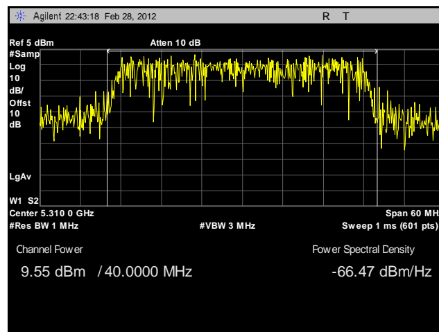
Plot 116. Conducted Output Power, 802.11n 40 MHz, Port A, 5310 MHz, Sector Antenna
