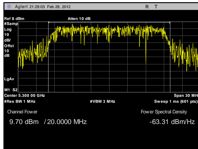
Plot 103. Conducted Output Power, 802.11n 20 MHz, Port A, 5300 MHz, Sector Antenna
