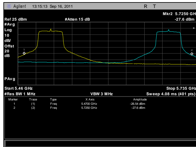
Plot 470. Frequency Stability, 802.11n 40 MHz, 5470 MHz – 5725 MHz @ 40°C, 120 V
