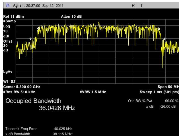
Plot 61. 99% Occupied Bandwidth, 802.11n 40 MHz, Port B, 5300 MHz
