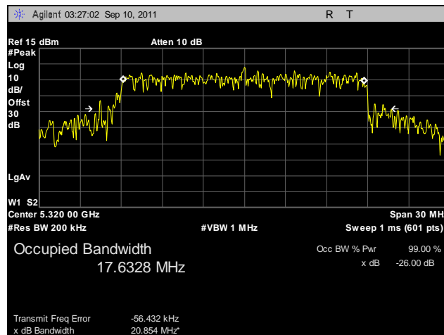
Plot 20. Occupied Bandwidth, 802.11n 20 MHz, Port B, 5320 MHz
