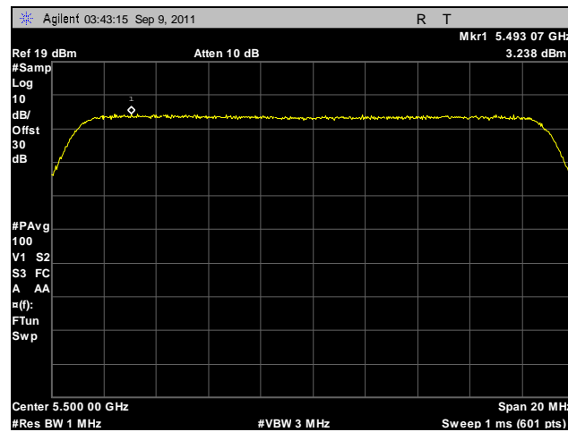
Plot 135. Peak Spectral Density, 802.11n 20 MHz, Port A, 5500 MHz
