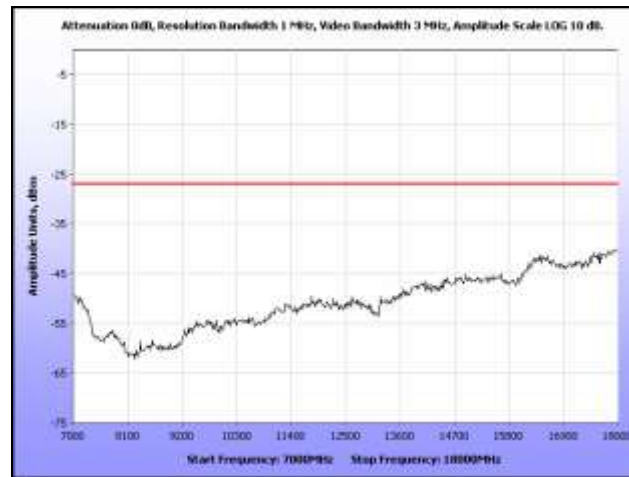
Plot 270. Radiated Spurious, 802.11n 40 MHz, 5300 MHz, 7 GHz – 18 GHz, Omni Antenna
