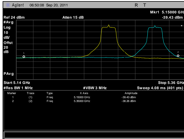
Plot 438. Frequency Stability, 802.11n 20 MHz, 5250 MHz – 5350 MHz @ 50°C, 120 V
