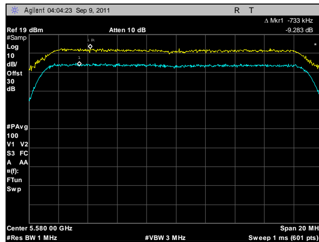
Plot 196. Peak Excursion, 802.11n 20 MHz, Port A, 5580 MHz
