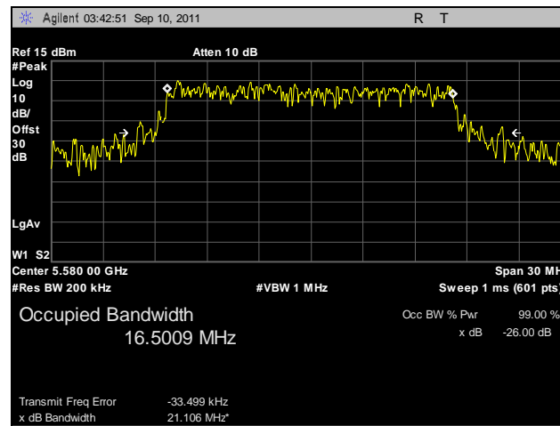
Plot 10. Occupied Bandwidth, 802.11a, 5580 MHz
