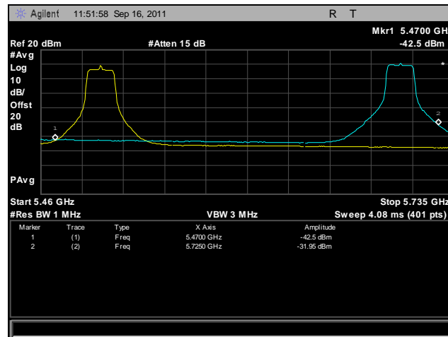
Plot 447. Frequency Stability, 802.11n 20 MHz, 5470 MHz – 5725 MHz @ 30°C, 120 V
