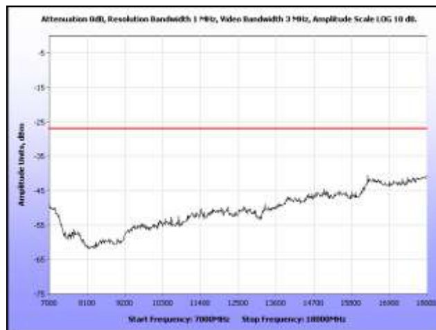
Plot 266. Radiated Spurious, 802.11n 40 MHz, 5270 MHz, 7 GHz – 18 GHz, Omni Antenna
