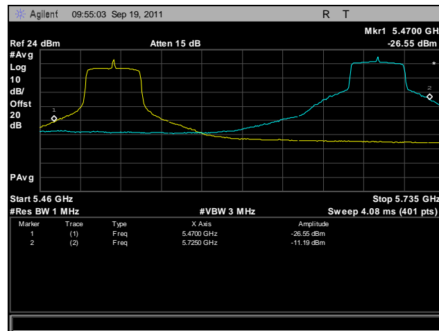
Plot 464. Frequency Stability, 802.11n 40 MHz, 5470 MHz – 5725 MHz @ 0°C, 120 V
