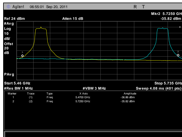
Plot 449. Frequency Stability, 802.11n 20 MHz, 5470 MHz – 5725 MHz @ 50°C, 120 V
