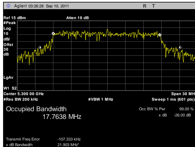
Plot 19. Occupied Bandwidth, 802.11n 20 MHz, Port B, 5300 MHz
