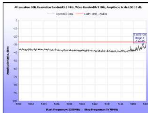
Plot 378. EIRP, 802.11n 20 MHz, 5500 MHz, Band Edge, Sector Antenna
