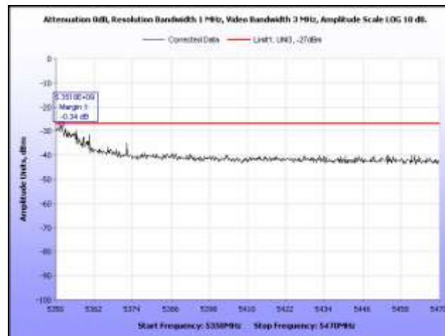
Plot 373. EIRP, 802.11a, 5320 MHz, Band Edge, Sector Antenna
