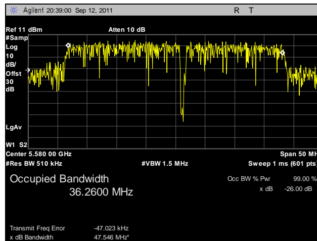
Plot 64. 99% Occupied Bandwidth, 802.11n 40 MHz, Port B, 5580 MHz
