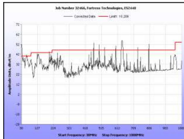
Plot 296. Radiated Spurious, 802.11a, 5320 MHz, 30 MHz – 1 GHz, Sector Antenna
