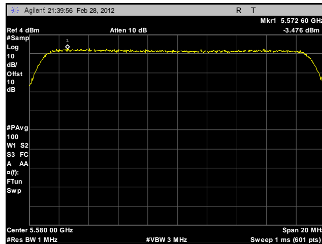
Plot 166. Peak Spectral Density, 802.11n 20 MHz, Port A, 5580 MHz, Sector Antenna
