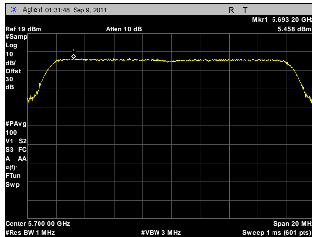
Plot 131. Peak Spectral Density, 802.11a, 5700 MHz
