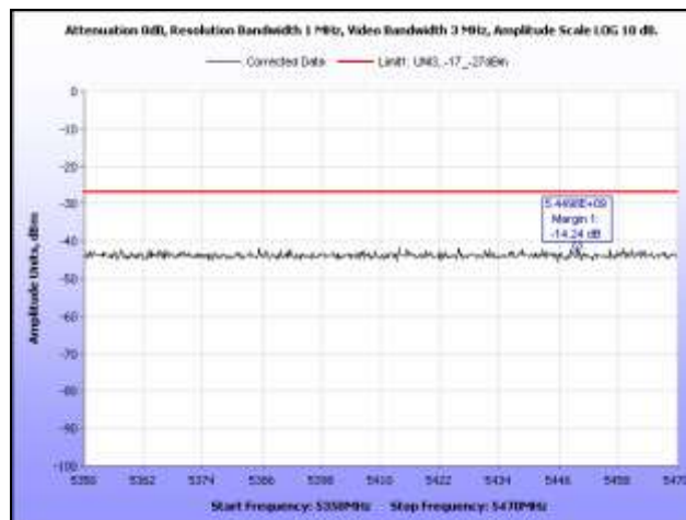
Plot 362. EIRP, 802.11a, 5500 MHz, Band Edge, Omni Antenna
