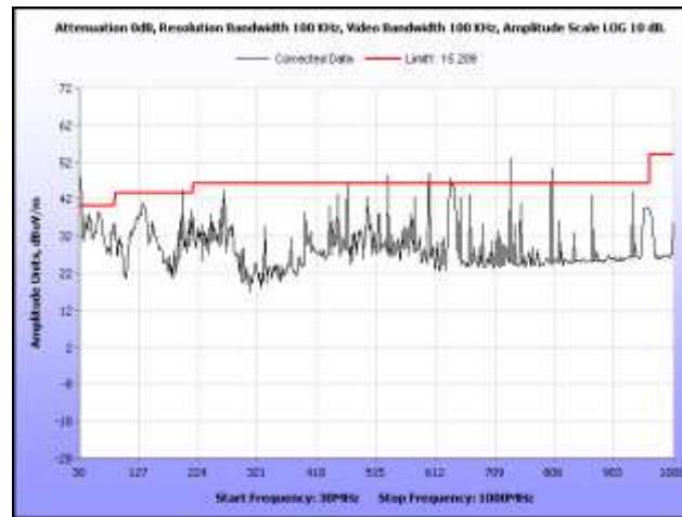
Plot 348. Radiated Spurious, 802.11n 40 MHz, 5510 MHz, 30 MHz – 1 GHz, Sector Antenna
