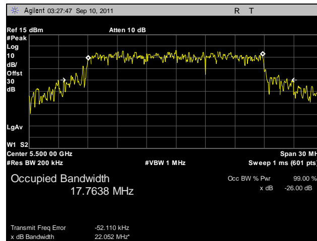
Plot 21. Occupied Bandwidth, 802.11n 20 MHz, Port B, 5500 MHz
