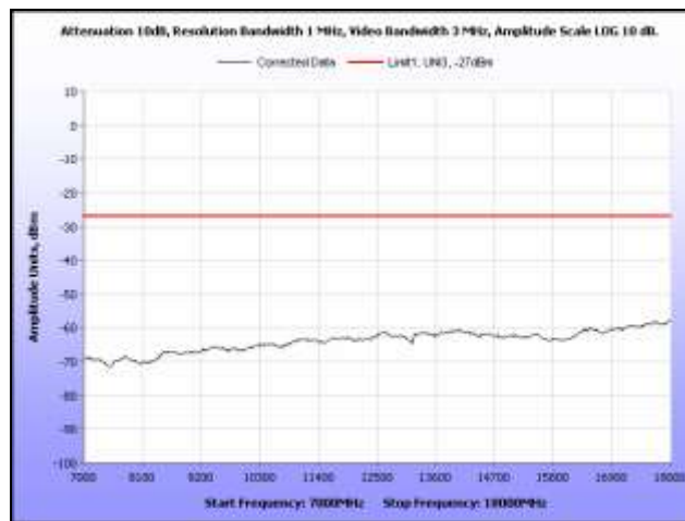
Plot 314. Radiated Spurious, 802.11n 20 MHz, 5260 MHz, 7 GHz – 18 GHz, Sector Antenna
