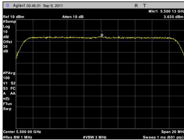
Plot 141. Peak Spectral Density, 802.11n 20 MHz, Port B, 5500 MHz
