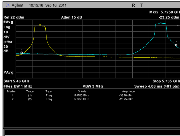
Plot 445. Frequency Stability, 802.11n 20 MHz, 5470 MHz – 5725 MHz @ 20°C, 120 V
