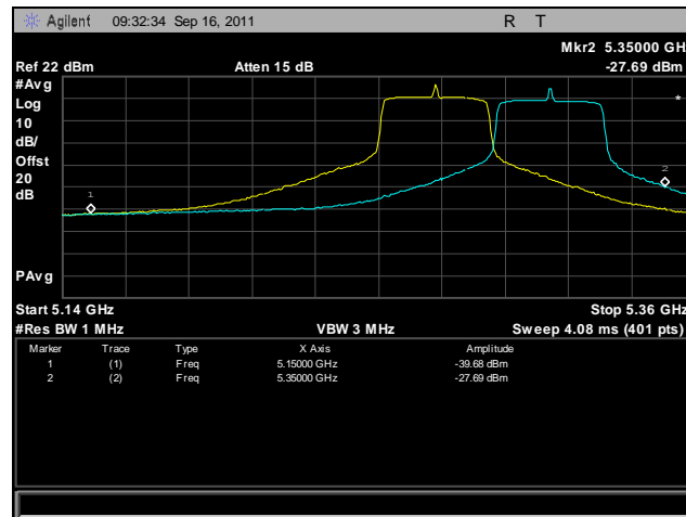
Plot 457. Frequency Stability, 802.11n 40 MHz, 5250 MHz – 5350 MHz @ 20°C, 132 V
