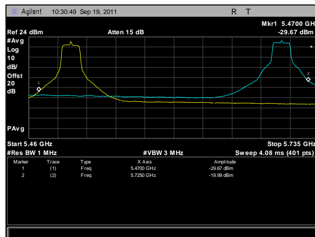
Plot 419. Frequency Stability, 802.11a, 5470 MHz – 5725 MHz @ -10°C, 120 V
