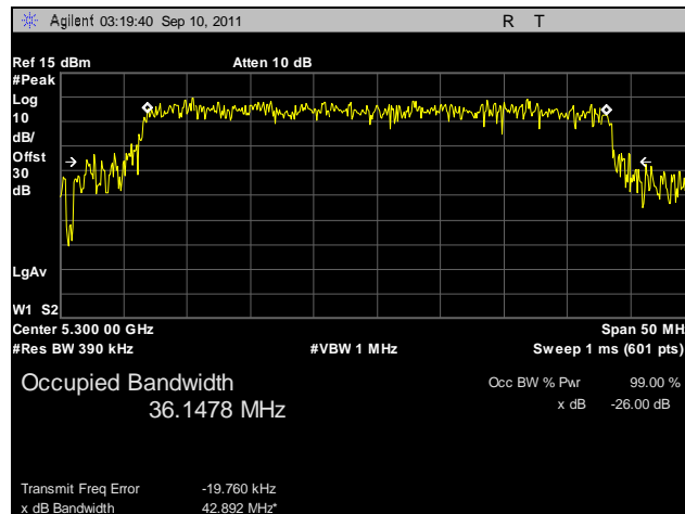
Plot 31. Occupied Bandwidth, 802.11n 40 MHz, Port B, 5300 MHz
