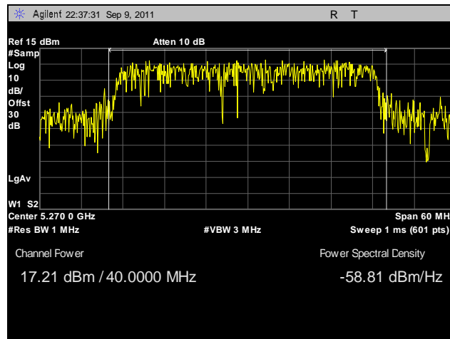
Plot 90. Conducted Output Power, 802.11n 40 MHz, Port B, 5270 MHz
