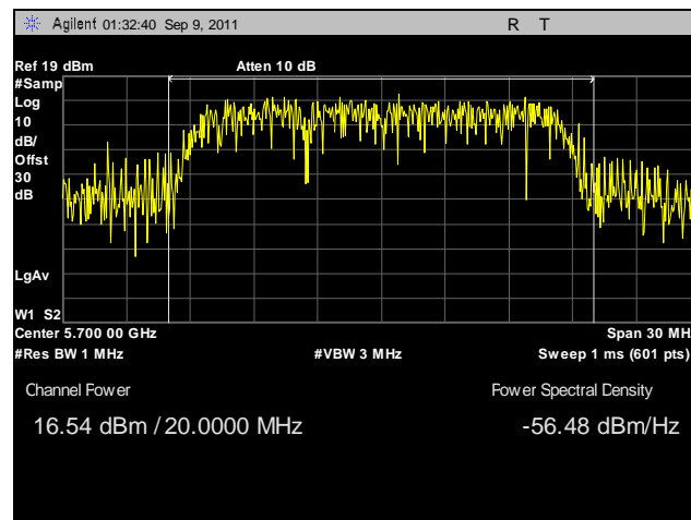
Plot 71. Conducted Output Power, 802.11a, 5700 MHz
