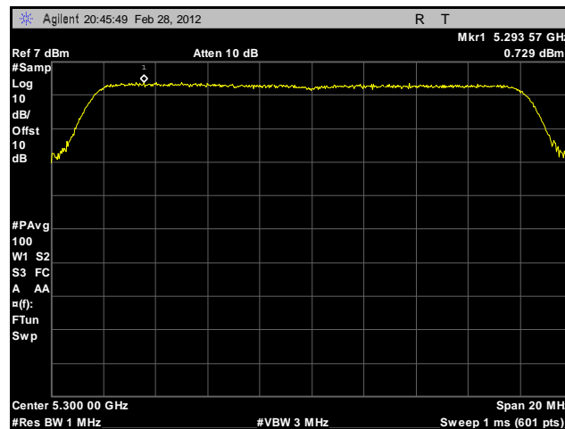
Plot 157. Peak Spectral Density, 802.11a, 5300 MHz, Sector Antenna
