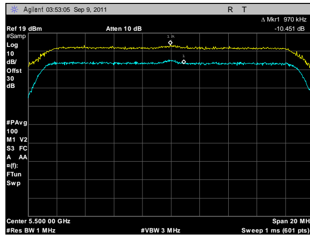
Plot 201. Peak Excursion, 802.11n 20 MHz, Port B, 5500 MHz
