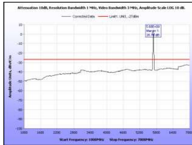
Plot 357. Radiated Spurious, 802.11n 40 MHz, 5690 MHz, 1 GHz – 7 GHz, Sector Antenna
