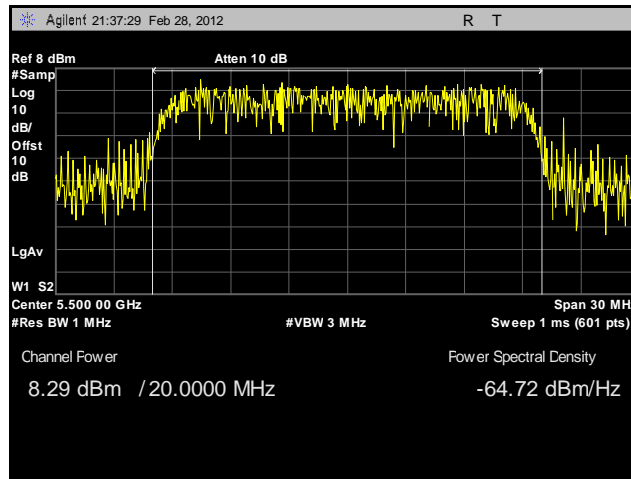
Plot 105. Conducted Output Power, 802.11n 20 MHz, Port A, 5500 MHz, Sector Antenna
