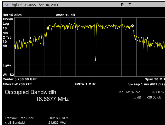
Plot 6. Occupied Bandwidth, 802.11a, 5260 MHz
