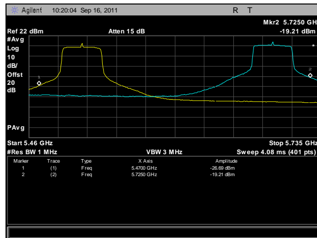
Plot 467. Frequency Stability, 802.11n 40 MHz, 5470 MHz – 5725 MHz @ 20°C, 120 V
