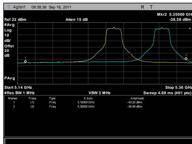
Plot 434. Frequency Stability, 802.11n 20 MHz, 5250 MHz – 5350 MHz @ 20°C, 120 V
