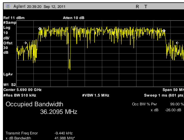
Plot 65. 99% Occupied Bandwidth, 802.11n 40 MHz, Port B, 5690 MHz
