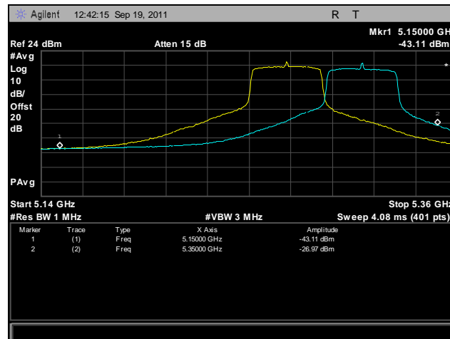
Plot 451. Frequency Stability, 802.11n 40 MHz, 5250 MHz – 5350 MHz @ -20°C, 120 V
