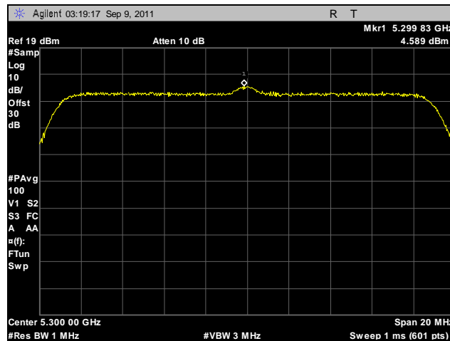
Plot 139. Peak Spectral Density, 802.11n 20 MHz, Port B, 5300 MHz
