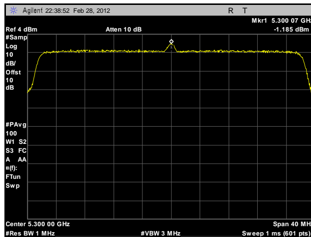
Plot 181. Peak Spectral Density, 802.11n 40 MHz, Port B, 5300 MHz, Sector Antenna
