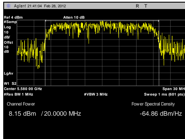
Plot 112. Conducted Output Power, 802.11n 20 MHz, Port B, 5580 MHz, Sector Antenna
