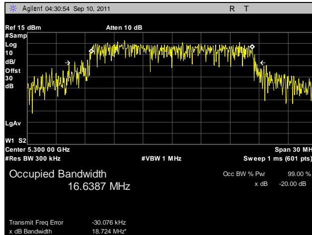
Plot 37. 99% Occupied Bandwidth, 802.11a, 5300 MHz
