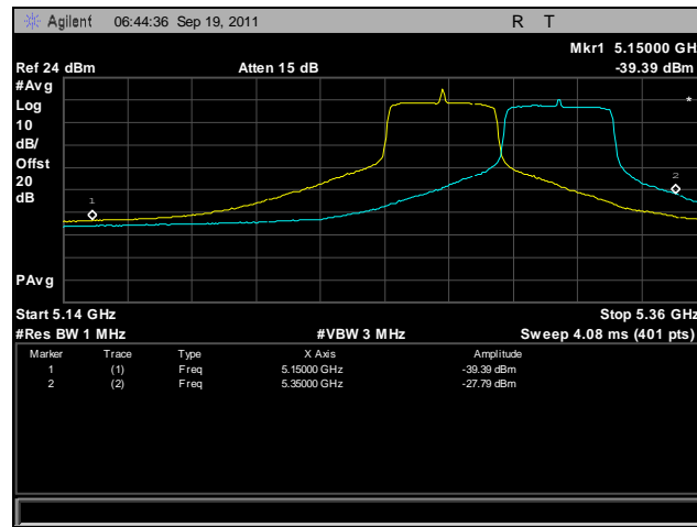
Plot 454. Frequency Stability, 802.11n 40 MHz, 5250 MHz – 5350 MHz @ 10°C, 120 V
