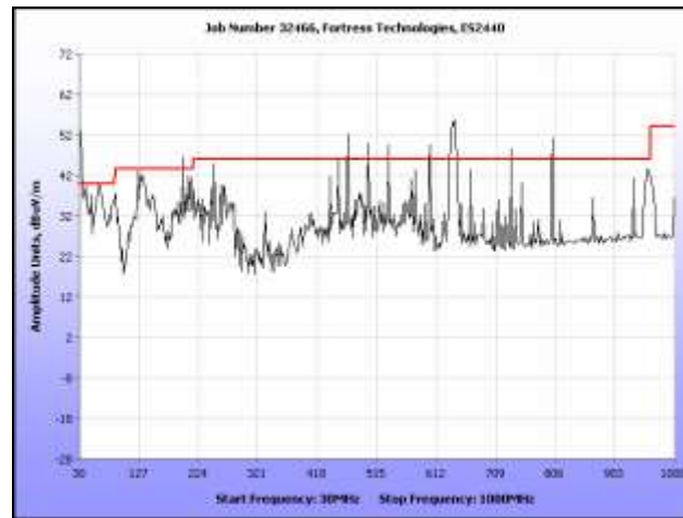
Plot 324. Radiated Spurious, 802.11n 20 MHz, 5500 MHz, 30 MHz – 1 GHz, Sector Antenna
