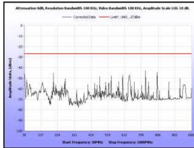
Plot 252. Radiated Spurious, 802.11n 20 MHz, 5500 MHz, 30 MHz – 1 GHz, Omni Antenna
