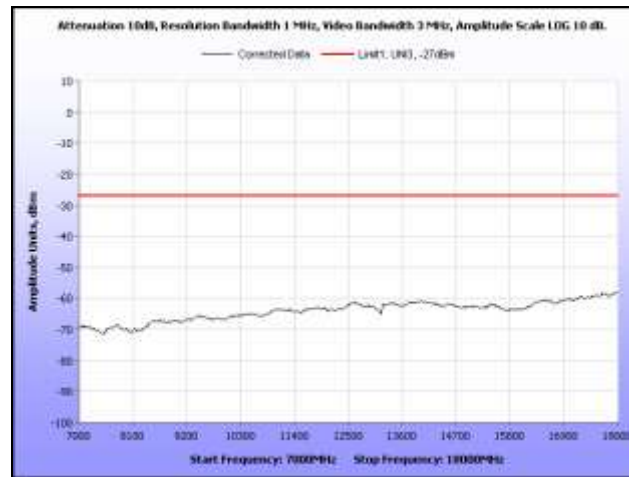
Plot 342. Radiated Spurious, 802.11n 40 MHz, 5300 MHz, 7 GHz – 18 GHz, Sector Antenna
