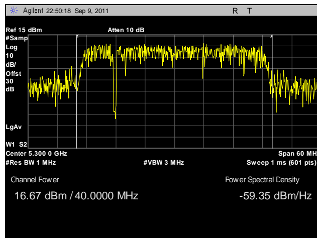
Plot 91. Conducted Output Power, 802.11n 40 MHz, Port B, 5300 MHz
