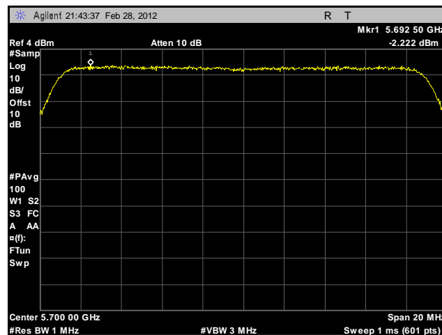
Plot 167. Peak Spectral Density, 802.11n 20 MHz, Port A, 5700 MHz, Sector Antenna
