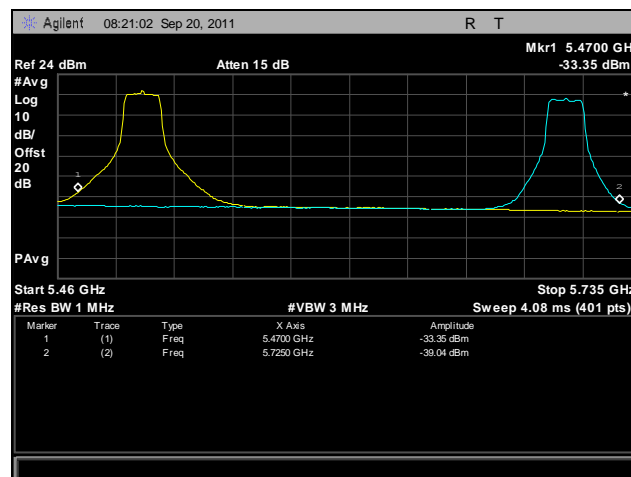
Plot 428. Frequency Stability, 802.11a, 5470 MHz – 5725 MHz @ 55°C, 120 V
