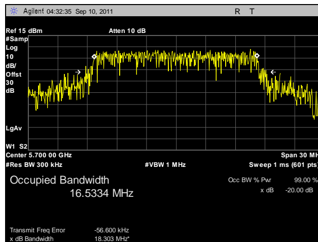
Plot 41. 99% Occupied Bandwidth, 802.11a, 5700 MHz
