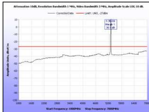
Plot 293. Radiated Spurious, 802.11a, 5300 MHz, 1 GHz – 7 GHz, Sector Antenna
