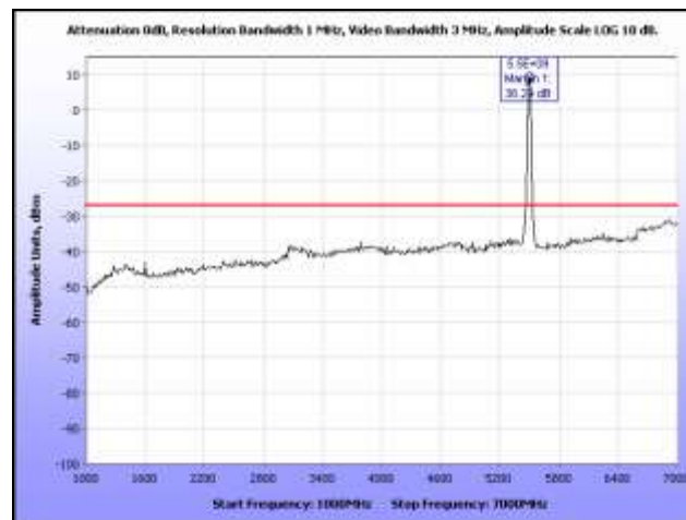
Plot 253. Radiated Spurious, 802.11n 20 MHz, 5500 MHz, 1 GHz – 7 GHz, Omni Antenna
