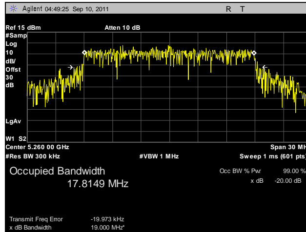
Plot 48. 99% Occupied Bandwidth, 802.11n 20 MHz, Port B, 5260 MHz
