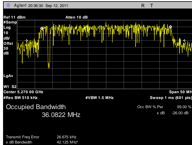
Plot 60. 99% Occupied Bandwidth, 802.11n 40 MHz, Port B, 5270 MHz
