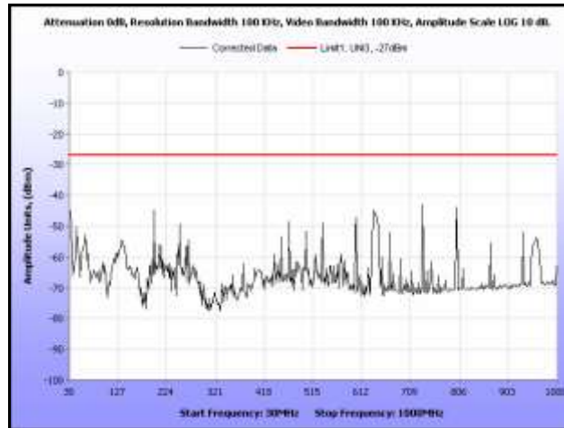
Plot 216. Radiated Spurious, 802.11a, 5260 MHz, 30 MHz – 1 GHz, Omni Antenna
