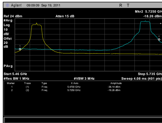
Plot 442. Frequency Stability, 802.11n 20 MHz, 5470 MHz – 5725 MHz @ 0°C, 120 V
