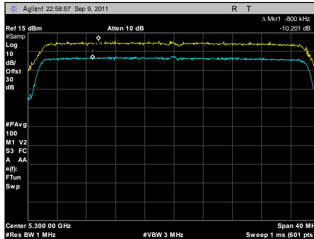
Plot 211. Peak Excursion, 802.11n 40 MHz, Port B, 5300 MHz
