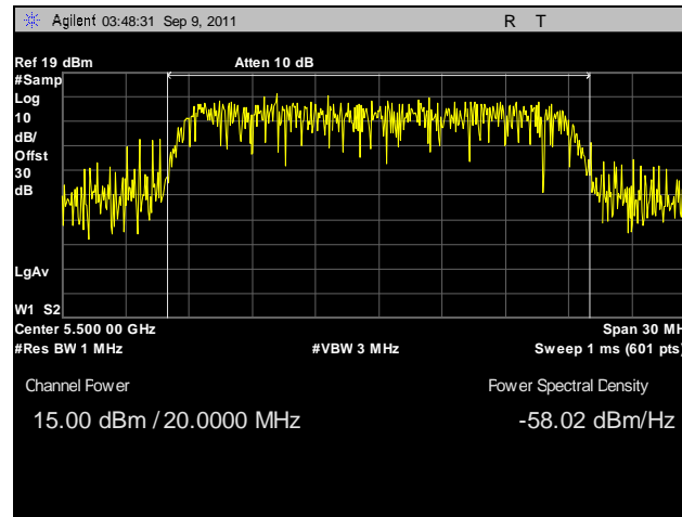
Plot 75. Conducted Output Power, 802.11n 20 MHz, Port A, 5500 MHz
