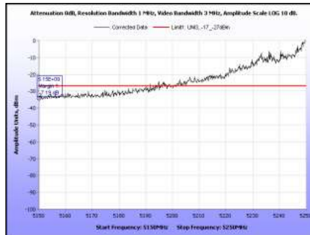
Plot 380. EIRP, 802.11n 40 MHz, 5270 MHz, Band Edge, Sector Antenna
