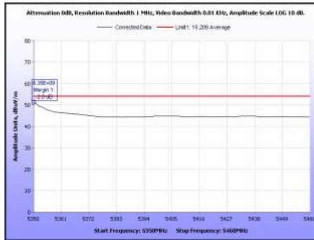
Plot 384. Restricted Band, 802.11a, 5320 MHz, Average, Omni Antenna
