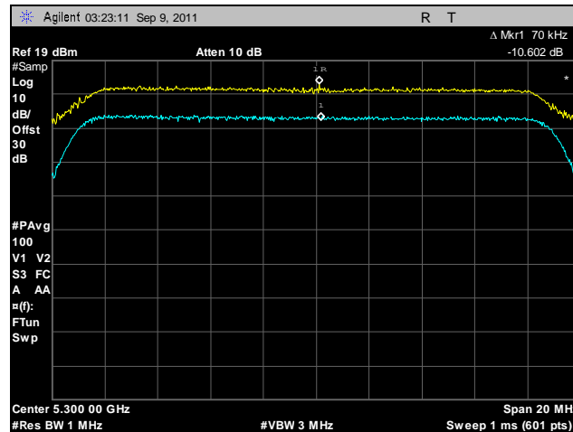
Plot 193. Peak Excursion, 802.11n 20 MHz, Port A, 5300 MHz
