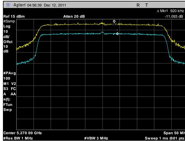
Plot 210. Peak Excursion, 802.11n 40 MHz, Port B, 5270 MHz
