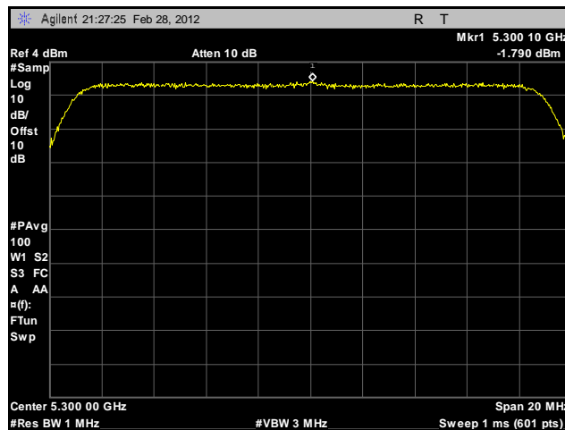
Plot 169. Peak Spectral Density, 802.11n 20 MHz, Port B, 5300 MHz, Sector Antenna
