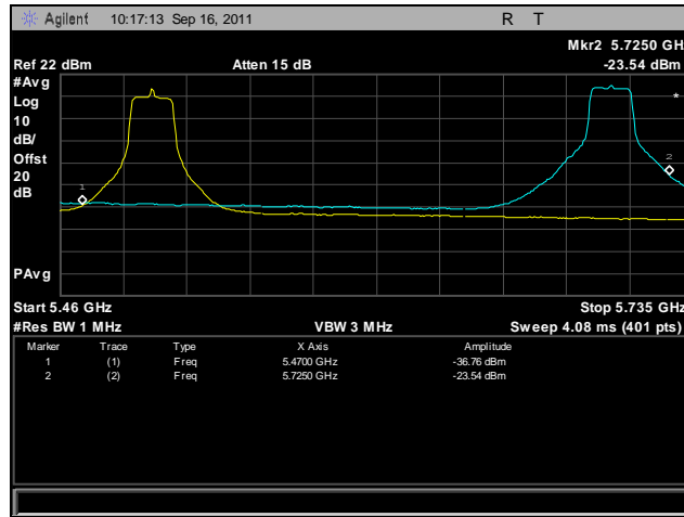
Plot 444. Frequency Stability, 802.11n 20 MHz, 5470 MHz – 5725 MHz @ 20°C, 108 V
