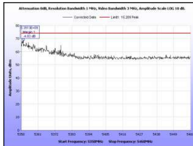
Plot 405. Restricted Band, 802.11n 40 MHz, 5310 MHz, Peak, Sector Antenna
