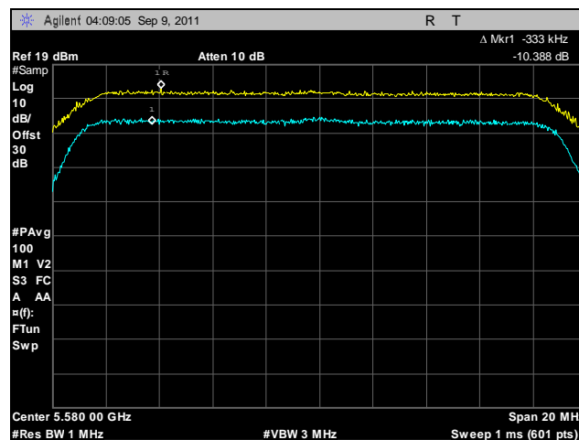
Plot 202. Peak Excursion, 802.11n 20 MHz, Port B, 5580 MHz
