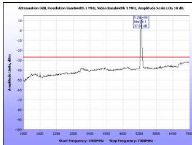
Plot 217. Radiated Spurious, 802.11a, 5260 MHz, 1 GHz – 7 GHz, Omni Antenna
