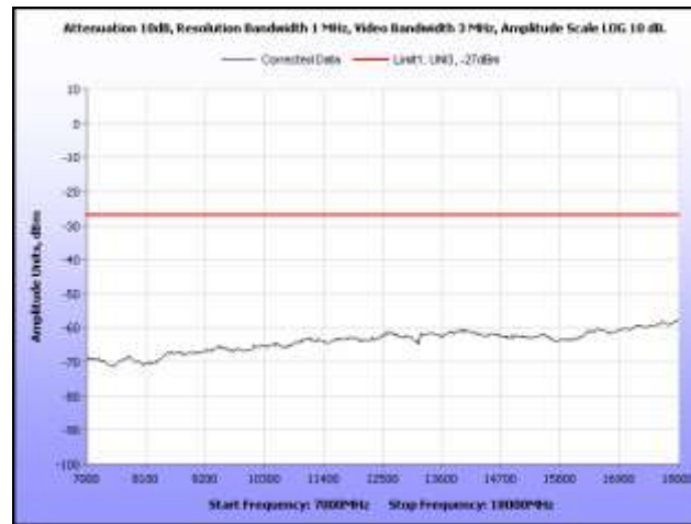
Plot 330. Radiated Spurious, 802.11n 20 MHz, 5580 MHz, 7 GHz – 18 GHz, Sector Antenna
