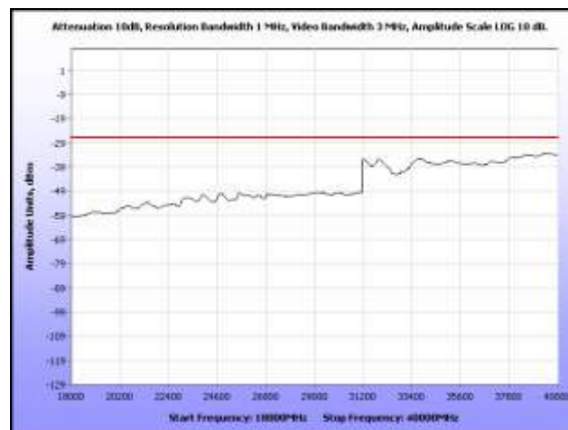
Plot 347. Radiated Spurious, 802.11n 40 MHz, 5310 MHz, 18 GHz – 40 GHz, Sector Antenna
