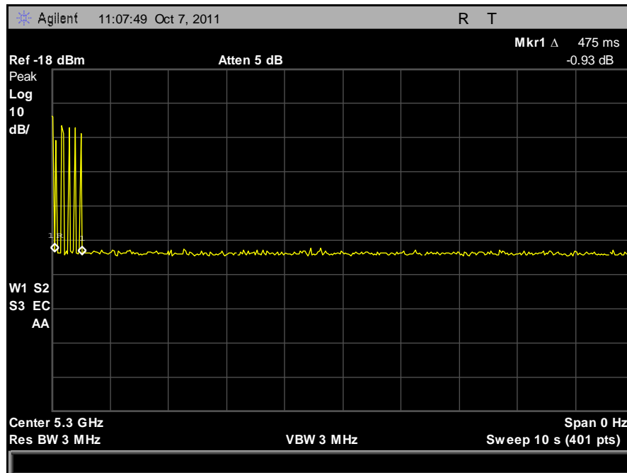
Plot 486. Channel Move Time
