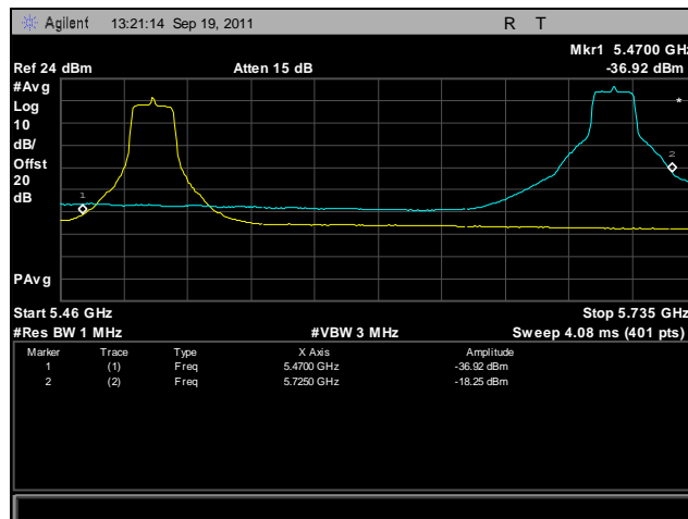
Plot 440. Frequency Stability, 802.11n 20 MHz, 5470 MHz – 5725 MHz @ -20°C, 120 V
