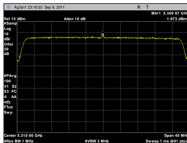
Plot 152. Peak Spectral Density, 802.11n 40 MHz, Port B, 5310 MHz
