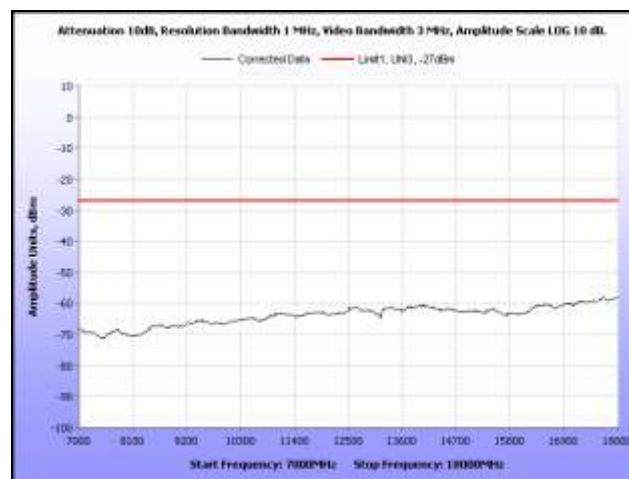
Plot 338. Radiated Spurious, 802.11n 40 MHz, 5270 MHz, 7 GHz – 18 GHz, Sector Antenna
