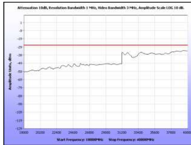
Plot 339. Radiated Spurious, 802.11n 40 MHz, 5270 MHz, 18 GHz – 40 GHz, Sector Antenna
