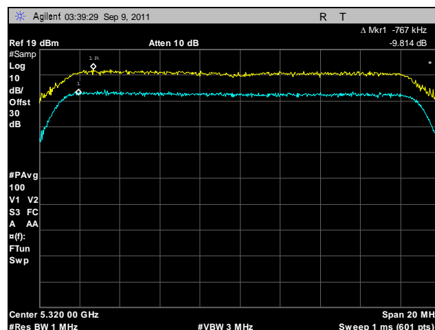
Plot 194. Peak Excursion, 802.11n 20 MHz, Port A, 5320 MHz
