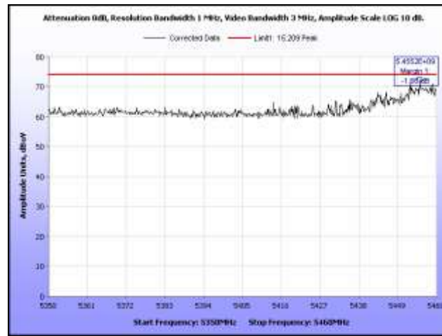
Plot 407. Restricted Band, 802.11n 40 MHz, 5510 MHz, Peak, Sector Antenna
