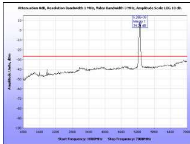
Plot 265. Radiated Spurious, 802.11n 40 MHz, 5270 MHz, 1 GHz – 7 GHz, Omni Antenna
