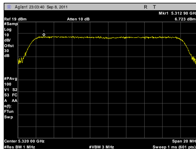
Plot 128. Peak Spectral Density, 802.11a, 5320 MHz
