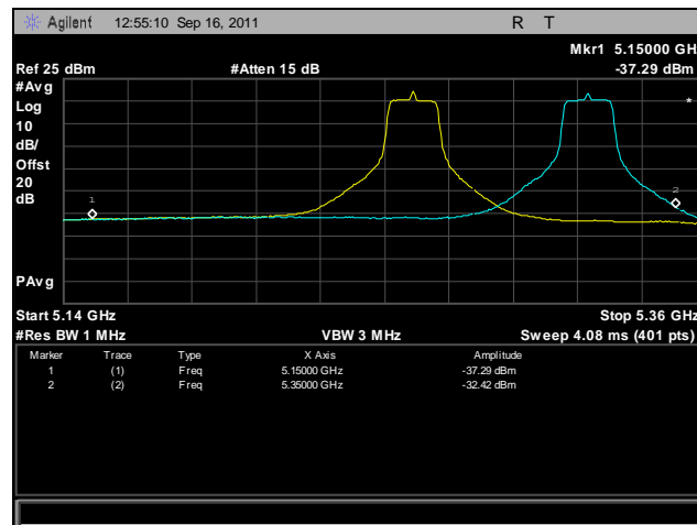
Plot 415. Frequency Stability, 802.11a, 5250 MHz – 5350 MHz @ 40°C, 120 V
