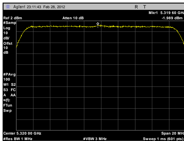
Plot 170. Peak Spectral Density, 802.11n 20 MHz, Port B, 5320 MHz, Sector Antenna
