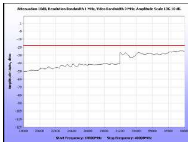
Plot 359. Radiated Spurious, 802.11n 40 MHz, 5690 MHz, 18 GHz – 40 GHz, Sector Antenna
