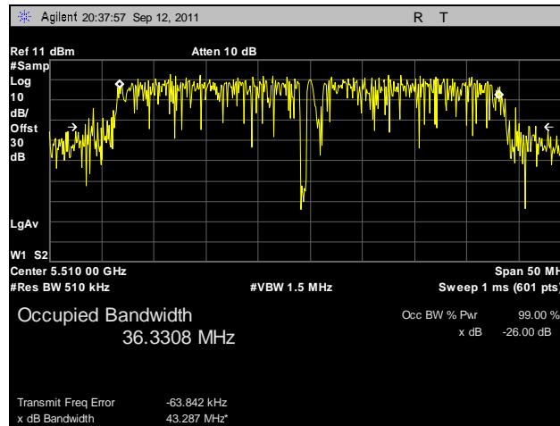
Plot 63. 99% Occupied Bandwidth, 802.11n 40 MHz, Port B, 5510 MHz
