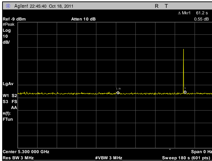
Plot 485. Radar Burst at the End of CACT
