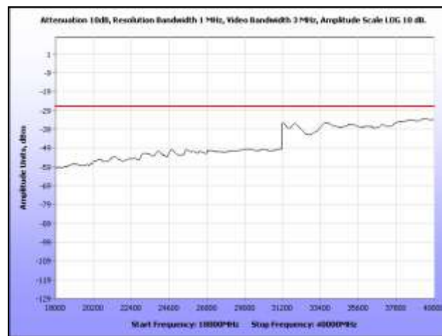
Plot 343. Radiated Spurious, 802.11n 40 MHz, 5300 MHz, 18 GHz – 40 GHz, Sector Antenna
