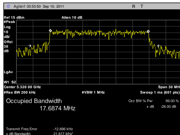
Plot 14. Occupied Bandwidth, 802.11n 20 MHz, Port A, 5320 MHz
