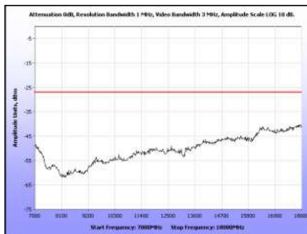
Plot 218. Radiated Spurious, 802.11a, 5260 MHz, 7 GHz – 18 GHz, Omni Antenna
