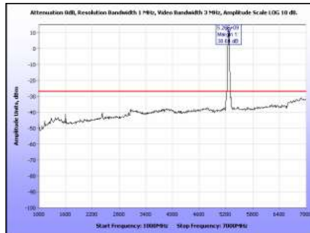
Plot 241. Radiated Spurious, 802.11n 20 MHz, 5260 MHz, 1 GHz – 7 GHz, Omni Antenna
