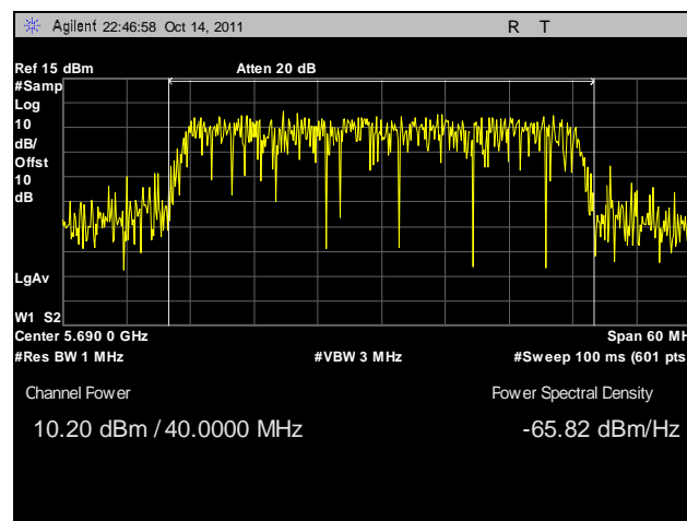
Plot 89. Conducted Output Power, 802.11n 40 MHz, Port A, 5690 MHz
