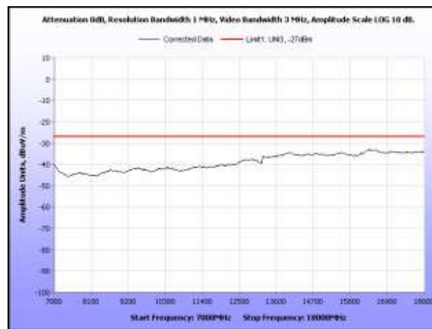
Plot 286. Radiated Spurious, 802.11n 40 MHz, 5690 MHz, 7 GHz – 18 GHz, Omni Antenna
