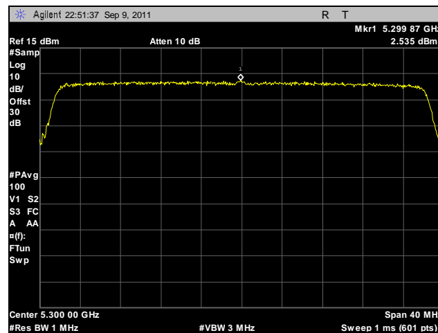
Plot 151. Peak Spectral Density, 802.11n 40 MHz, Port B, 5300 MHz
