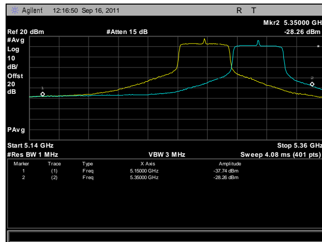
Plot 458. Frequency Stability, 802.11n 40 MHz, 5250 MHz – 5350 MHz @ 30°C, 120 V
