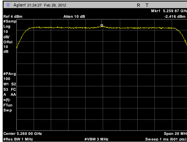
Plot 168. Peak Spectral Density, 802.11n 20 MHz, Port B, 5260 MHz, Sector Antenna
