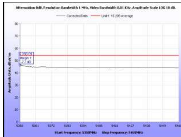
Plot 388. Restricted Band, 802.11n 20 MHz, 5320 MHz, Average, Omni Antenna
