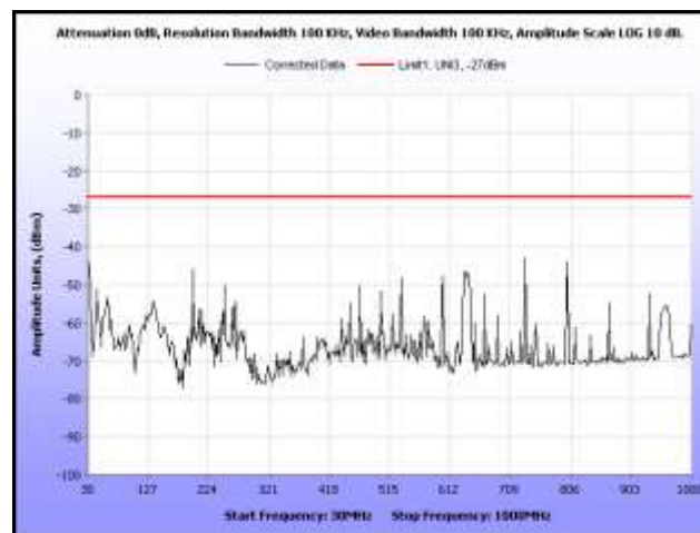
Plot 244. Radiated Spurious, 802.11n 20 MHz, 5300 MHz, 30 MHz – 1 GHz, Omni Antenna
