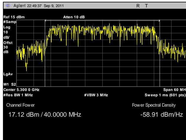
Plot 85. Conducted Output Power, 802.11n 40 MHz, Port A, 5300 MHz
