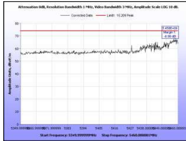
Plot 395. Restricted Band, 802.11n 40 MHz, 5510 MHz, Peak, Omni Antenna
