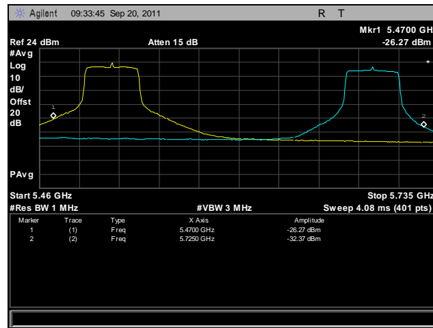
Plot 472. Frequency Stability, 802.11n 40 MHz, 5470 MHz – 5725 MHz @ 55°C, 120 V
