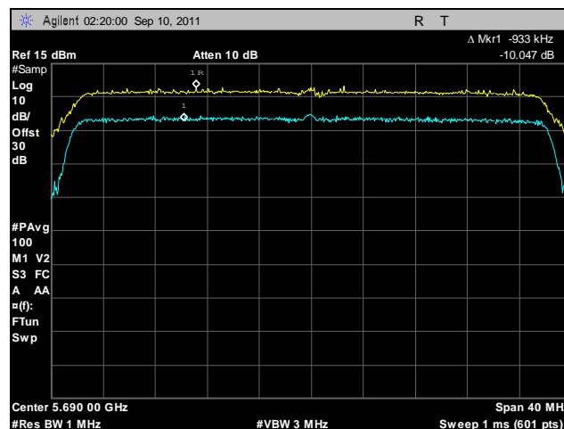
Plot 215. Peak Excursion, 802.11n 40 MHz, Port B, 5690 MHz
