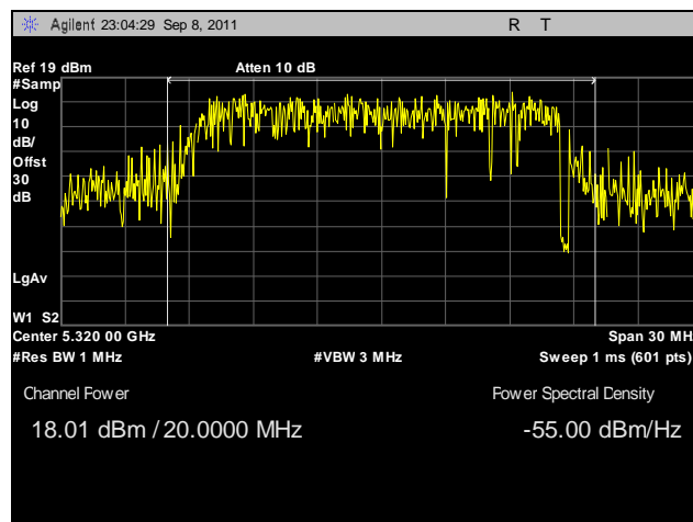
Plot 68. Conducted Output Power, 802.11a, 5320 MHz
