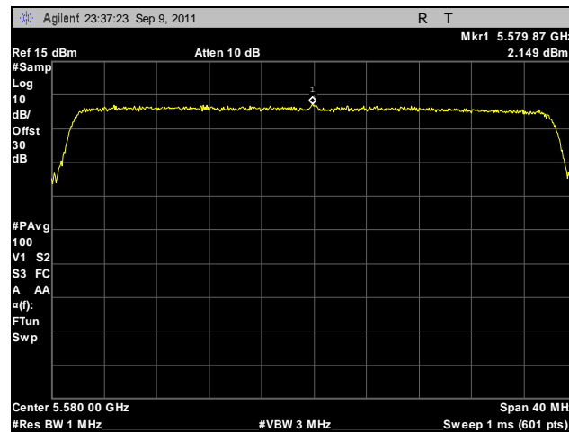
Plot 154. Peak Spectral Density, 802.11n 40 MHz, Port B, 5580 MHz
