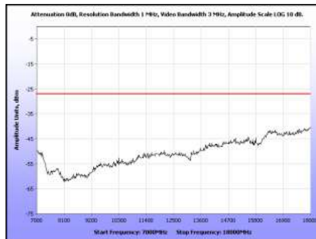
Plot 242. Radiated Spurious, 802.11n 20 MHz, 5260 MHz, 7 GHz – 18 GHz, Omni Antenna
