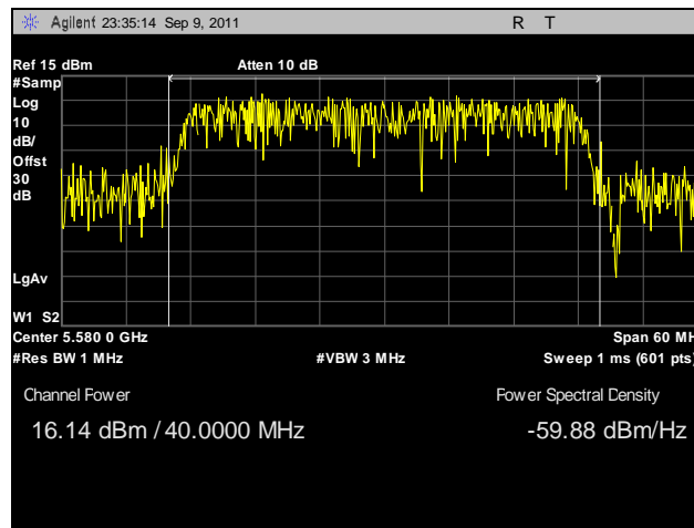
Plot 94. Conducted Output Power, 802.11n 40 MHz, Port B, 5580 MHz
