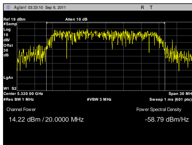
Plot 74. Conducted Output Power, 802.11n 20 MHz, Port A, 5320 MHz
