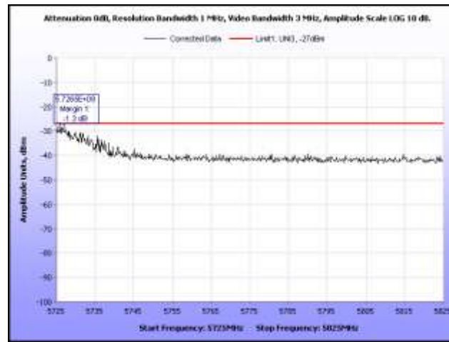
Plot 367. EIRP, 802.11n 20 MHz, 5700 MHz, Band Edge, Omni Antenna
