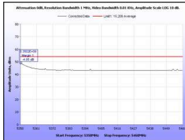
Plot 396. Restricted Band, 802.11a, 5320 MHz, Average, Sector Antenna
