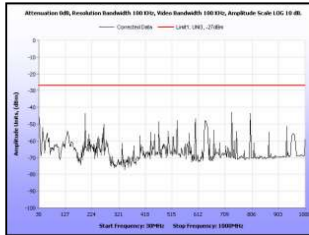
Plot 228. Radiated Spurious, 802.11a, 5500 MHz, 30 MHz – 1 GHz, Omni Antenna
