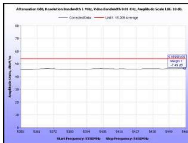
Plot 390. Restricted Band, 802.11n 20 MHz, 5500 MHz, Average, Omni Antenna
