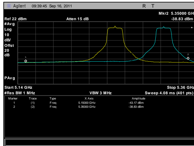
Plot 435. Frequency Stability, 802.11n 20 MHz, 5250 MHz – 5350 MHz @ 20°C, 132 V
