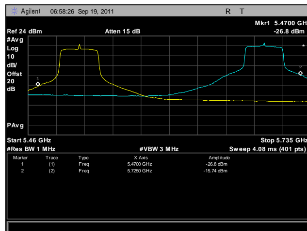
Plot 465. Frequency Stability, 802.11n 40 MHz, 5470 MHz – 5725 MHz @ 10°C, 120 V
