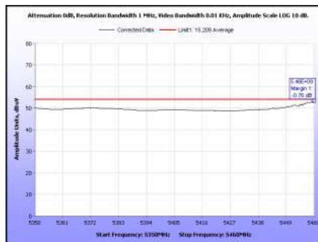
Plot 406. Restricted Band, 802.11n 40 MHz, 5510 MHz, Average, Sector Antenna
