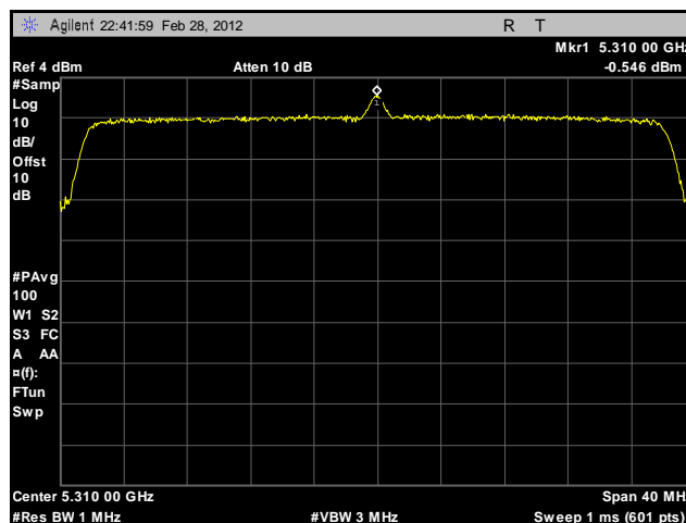
Plot 182. Peak Spectral Density, 802.11n 40 MHz, Port B, 5310 MHz, Sector Antenna
