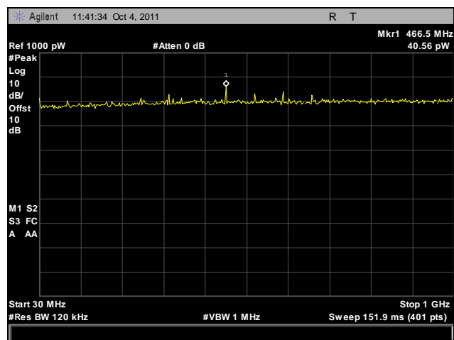
Plot 475. Receiver Spurious Emission, 5.8 GHz, 30 MHz – 1 GHz, Port B
