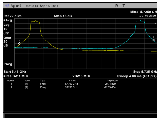
Plot 422. Frequency Stability, 802.11a, 5470 MHz – 5725 MHz @ 20°C, 108 V
