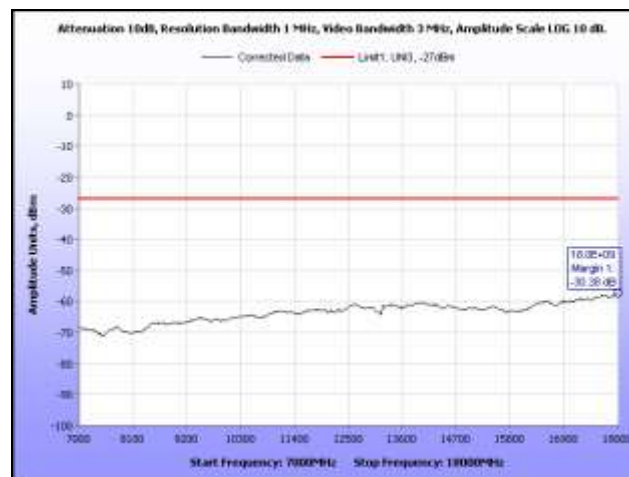
Plot 310. Radiated Spurious, 802.11a, 5700 MHz, 7 GHz – 18 GHz, Sector Antenna
