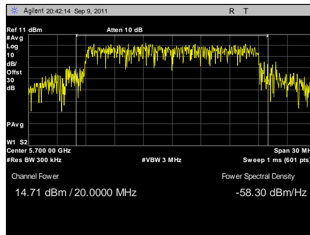
Plot 77. Conducted Output Power, 802.11n 20 MHz, Port A, 5700 MHz
