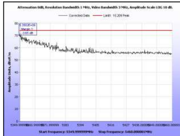
Plot 393. Restricted Band, 802.11n 40 MHz, 5310 MHz, Peak, Omni Antenna
