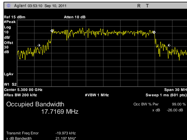
Plot 13. Occupied Bandwidth, 802.11n 20 MHz, Port A, 5300 MHz
