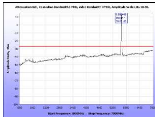
Plot 233. Radiated Spurious, 802.11a, 5580 MHz, 1 GHz – 7 GHz, Omni Antenna
