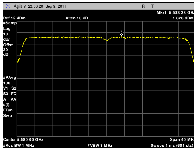
Plot 148. Peak Spectral Density, 802.11n 40 MHz, Port A, 5580 MHz
