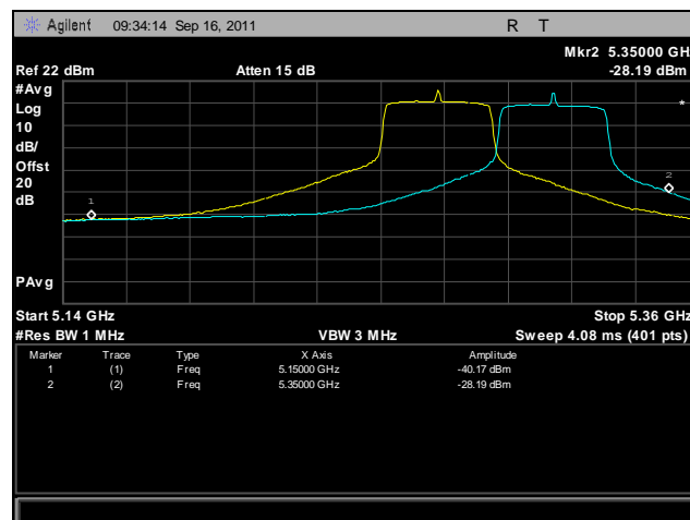
Plot 456. Frequency Stability, 802.11n 40 MHz, 5250 MHz – 5350 MHz @ 20°C, 120 V
