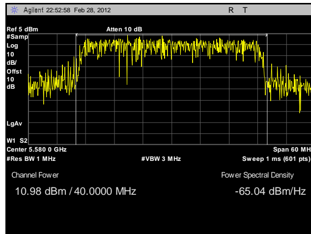
Plot 118. Conducted Output Power, 802.11n 40 MHz, Port A, 5580 MHz, Sector Antenna
