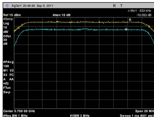
Plot 203. Peak Excursion, 802.11n 20 MHz, Port B, 5700 MHz
