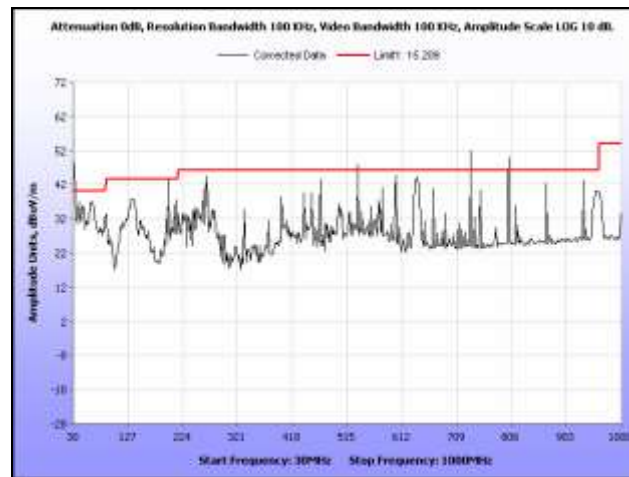
Plot 304. Radiated Spurious, 802.11a, 5580 MHz, 30 MHz – 1 GHz, Sector Antenna
