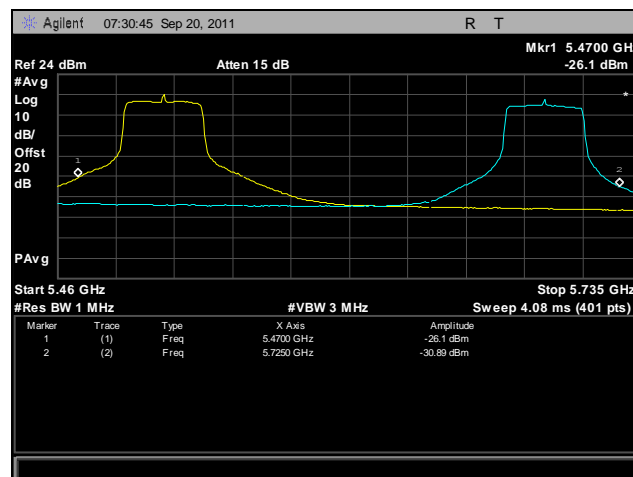
Plot 471. Frequency Stability, 802.11n 40 MHz, 5470 MHz – 5725 MHz @ 50°C, 120 V
