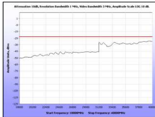
Plot 331. Radiated Spurious, 802.11n 20 MHz, 5580 MHz, 18 GHz – 40 GHz, Sector Antenna
