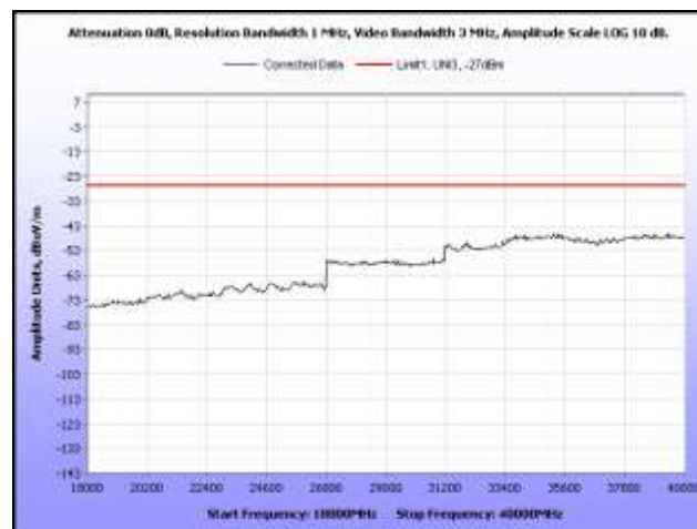
Plot 287. Radiated Spurious, 802.11n 40 MHz, 5690 MHz, 18 GHz – 40 GHz, Omni Antenna
