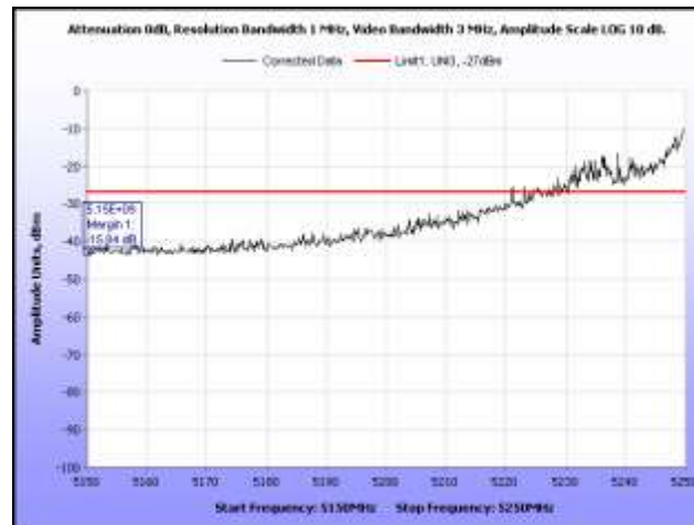
Plot 368. EIRP, 802.11n 40 MHz, 5270 MHz, Band Edge, Omni Antenna
