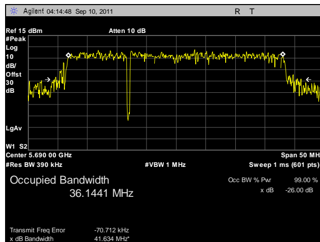
Plot 29. Occupied Bandwidth, 802.11n 40 MHz, Port A, 5690 MHz
