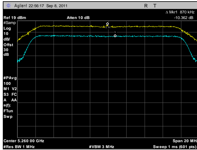
Plot 186. Peak Excursion, 802.11a, 5260 MHz
