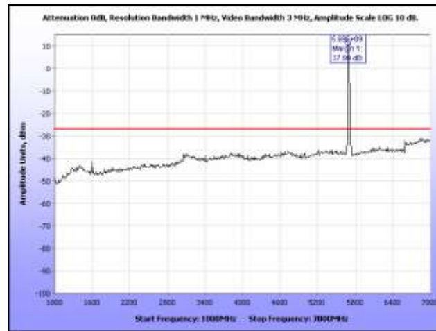
Plot 237. Radiated Spurious, 802.11a, 5700 MHz, 1 GHz – 7 GHz, Omni Antenna
