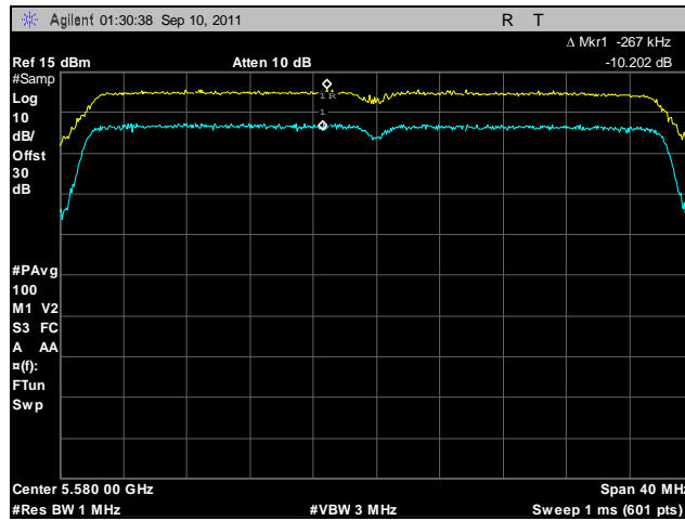
Plot 208. Peak Excursion, 802.11n 40 MHz, Port A, 5580 MHz
