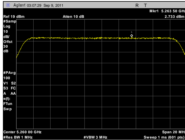
Plot 132. Peak Spectral Density, 802.11n 20 MHz, Port A, 5260 MHz
