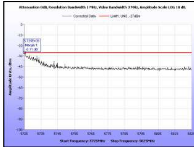
Plot 379. EIRP, 802.11n 20 MHz, 5700 MHz, Band Edge, Sector Antenna
