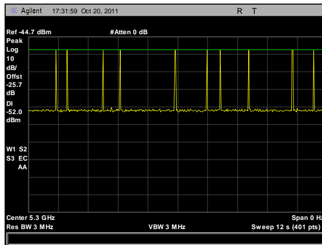
Plot 481. Radar Calibration, Bin 5
