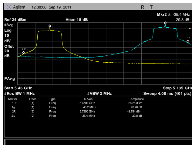
Plot 462. Frequency Stability, 802.11n 40 MHz, 5470 MHz – 5725 MHz @ -20°C, 120 V
