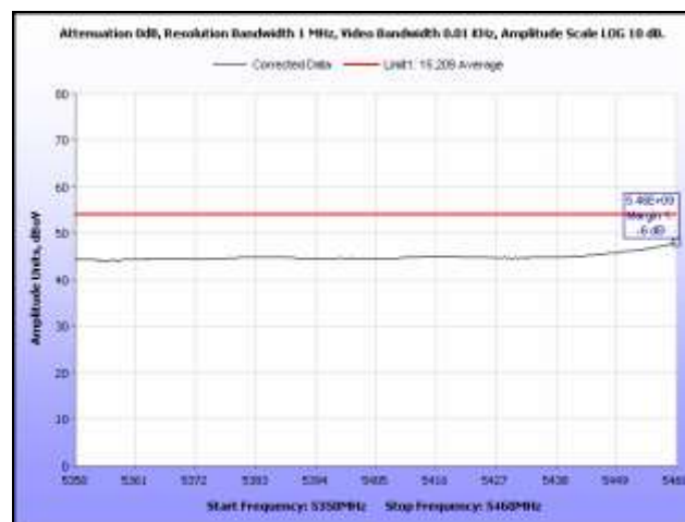
Plot 398. Restricted Band, 802.11a, 5500 MHz, Average, Sector Antenna
