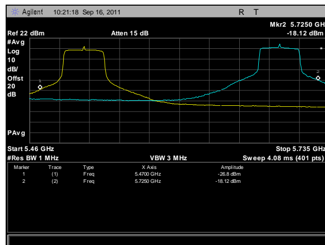
Plot 468. Frequency Stability, 802.11n 40 MHz, 5470 MHz – 5725 MHz @ 20°C, 132 V
