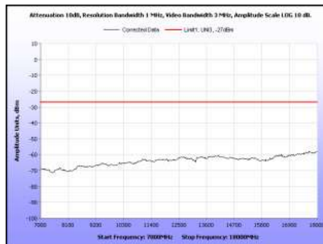
Plot 326. Radiated Spurious, 802.11n 20 MHz, 5500 MHz, 7 GHz – 18 GHz, Sector Antenna
