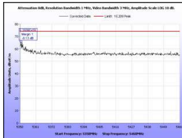
Plot 389. Restricted Band, 802.11n 20 MHz, 5320 MHz, Peak, Omni Antenna
