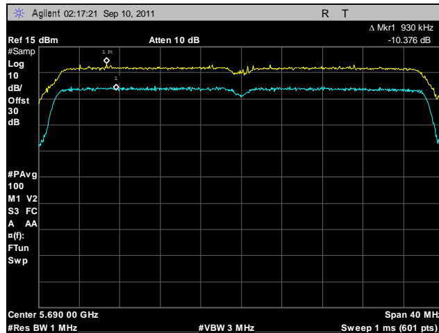
Plot 209. Peak Excursion, 802.11n 40 MHz, Port A, 5690 MHz
