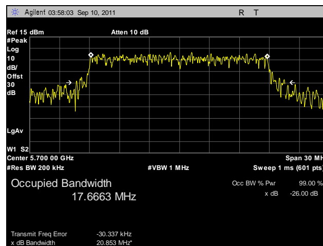
Plot 17. Occupied Bandwidth, 802.11n 20 MHz, Port A, 5700 MHz
