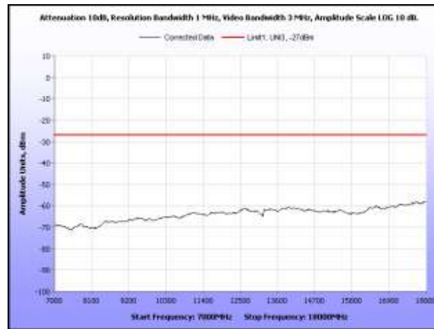
Plot 354. Radiated Spurious, 802.11n 40 MHz, 5580 MHz, 7 GHz – 18 GHz, Sector Antenna
