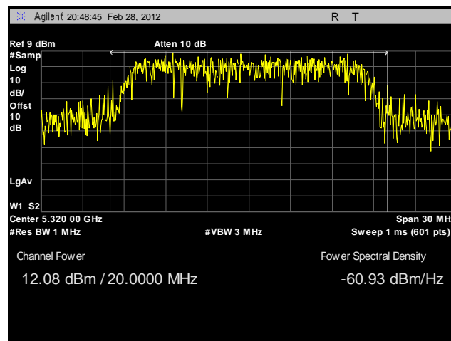
Plot 98. Conducted Output Power, 802.11a, 5320 MHz, Sector Antenna
