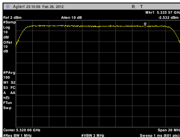
Plot 164. Peak Spectral Density, 802.11n 20 MHz, Port A, 5320 MHz, Sector Antenna
