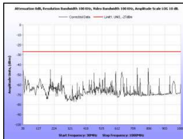
Plot 260. Radiated Spurious, 802.11n 20 MHz, 5700 MHz, 30 MHz – 1 GHz, Omni Antenna
