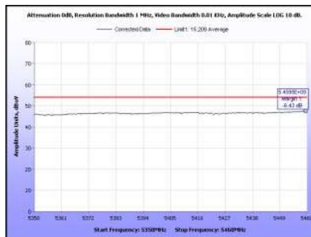
Plot 402. Restricted Band, 802.11n 20 MHz, 5500 MHz, Average, Sector Antenna
