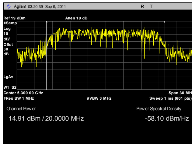
Plot 73. Conducted Output Power, 802.11n 20 MHz, Port A, 5300 MHz
