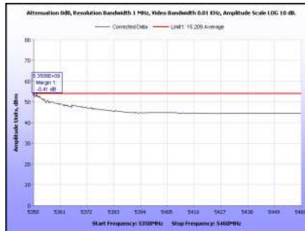
Plot 404. Restricted Band, 802.11n 40 MHz, 5310 MHz, Average, Sector Antenna
