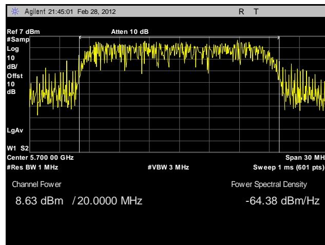
Plot 113. Conducted Output Power, 802.11n 20 MHz, Port B, 5700 MHz, Sector Antenna
