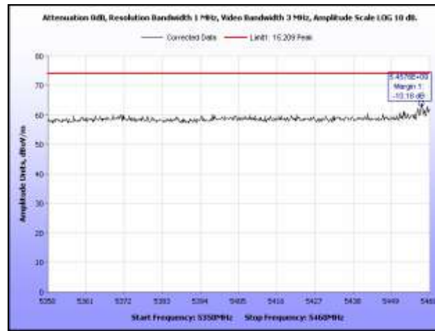
Plot 391. Restricted Band, 802.11n 20 MHz, 5500 MHz, Peak, Omni Antenna
