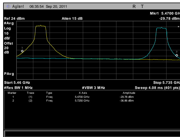
Plot 427. Frequency Stability, 802.11a, 5470 MHz – 5725 MHz @ 50°C, 120 V
