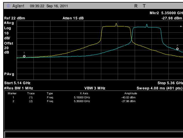
Plot 455. Frequency Stability, 802.11n 40 MHz, 5250 MHz – 5350 MHz @ 20°C, 108 V
