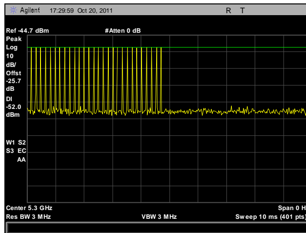
Plot 478. Radar Calibration, Bin 2
