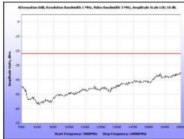
Plot 282. Radiated Spurious, 802.11n 40 MHz, 5580 MHz, 7 GHz – 18 GHz, Omni Antenna
