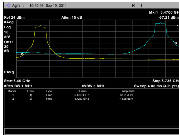
Plot 441. Frequency Stability, 802.11n 20 MHz, 5470 MHz – 5725 MHz @ -10°C, 120 V
