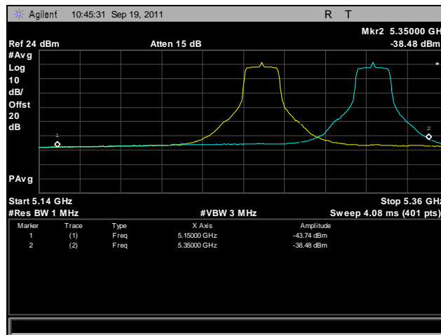
Plot 430. Frequency Stability, 802.11n 20 MHz, 5250 MHz – 5350 MHz @ -10°C, 120 V
