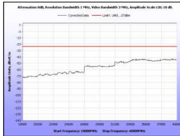
Plot 267. Radiated Spurious, 802.11n 40 MHz, 5270 MHz, 18 GHz – 40 GHz, Omni Antenna
