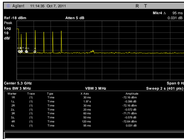
Plot 488. Channel Closing Transmission Time, 1
