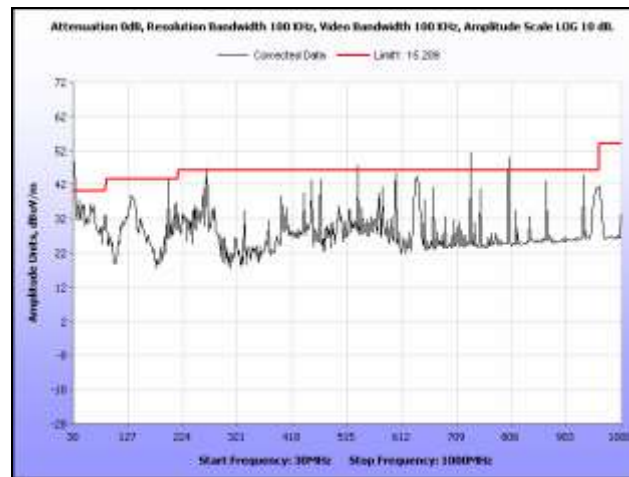
Plot 316. Radiated Spurious, 802.11n 20 MHz, 5300 MHz, 30 MHz – 1 GHz, Sector Antenna
