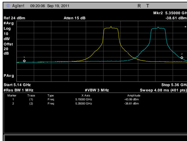
Plot 431. Frequency Stability, 802.11n 20 MHz, 5250 MHz – 5350 MHz @ 0°C, 120 V
