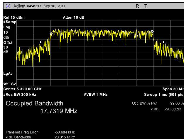
Plot 44. 99% Occupied Bandwidth, 802.11n 20 MHz, Port A, 5320 MHz
