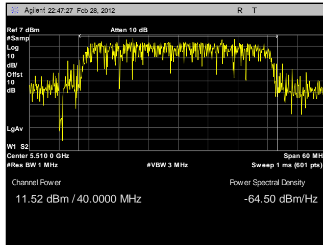
Plot 117. Conducted Output Power, 802.11n 40 MHz, Port A, 5510 MHz, Sector Antenna
