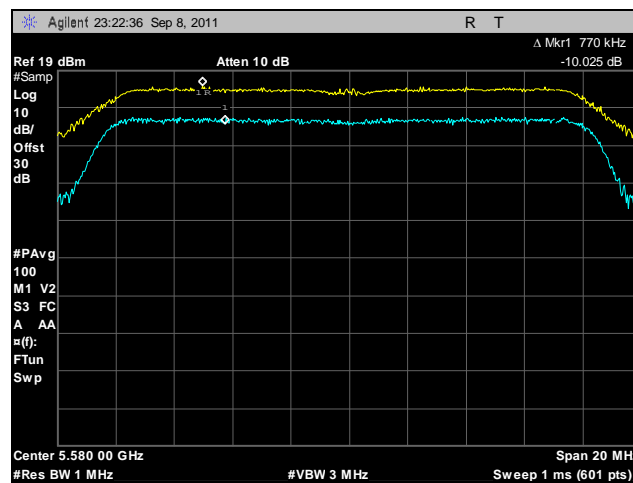
Plot 190. Peak Excursion, 802.11a, 5580 MHz
