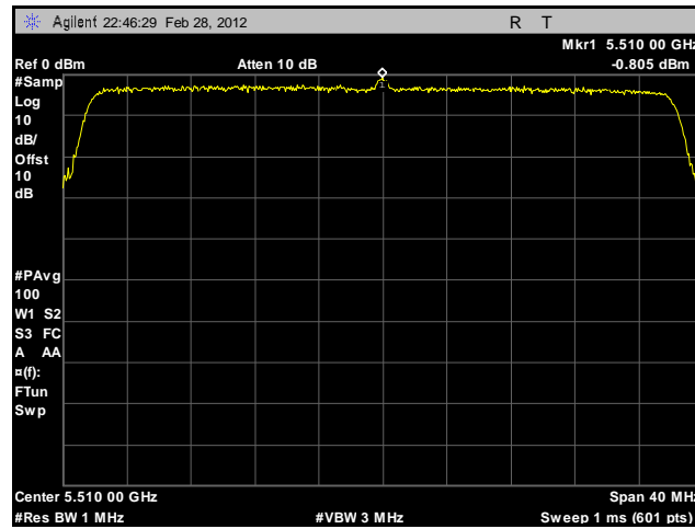
Plot 183. Peak Spectral Density, 802.11n 40 MHz, Port B, 5510 MHz, Sector Antenna
