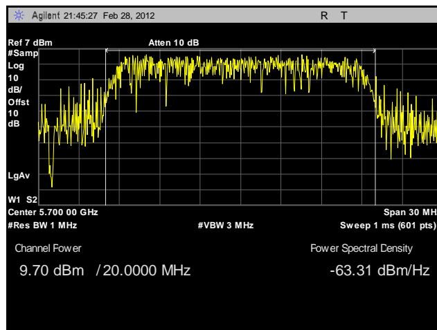
Plot 107. Conducted Output Power, 802.11n 20 MHz, Port A, 5700 MHz, Sector Antenna
