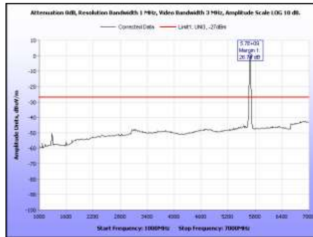
Plot 285. Radiated Spurious, 802.11n 40 MHz, 5690 MHz, 1 GHz – 7 GHz, Omni Antenna
