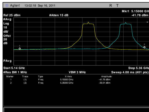
Plot 437. Frequency Stability, 802.11n 20 MHz, 5250 MHz – 5350 MHz @ 40°C, 120 V
