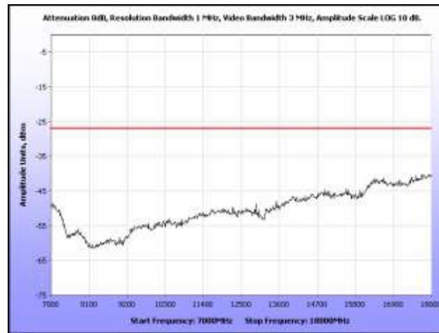
Plot 234. Radiated Spurious, 802.11a, 5580 MHz, 7 GHz – 18 GHz, Omni Antenna
