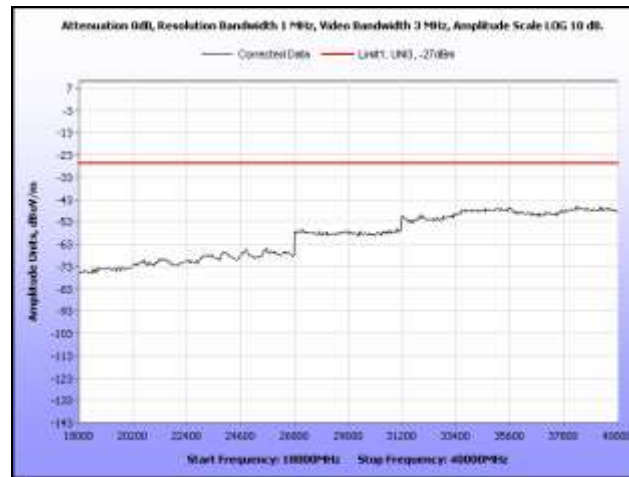
Plot 279. Radiated Spurious, 802.11n 40 MHz, 5510 MHz, 18 MHz – 40 GHz, Omni Antenna
