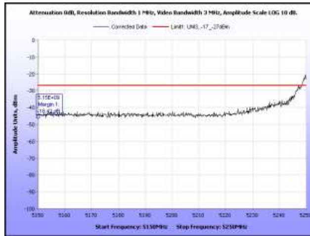
Plot 360. EIRP, 802.11a, 5260 MHz, Band Edge, Omni Antenna
