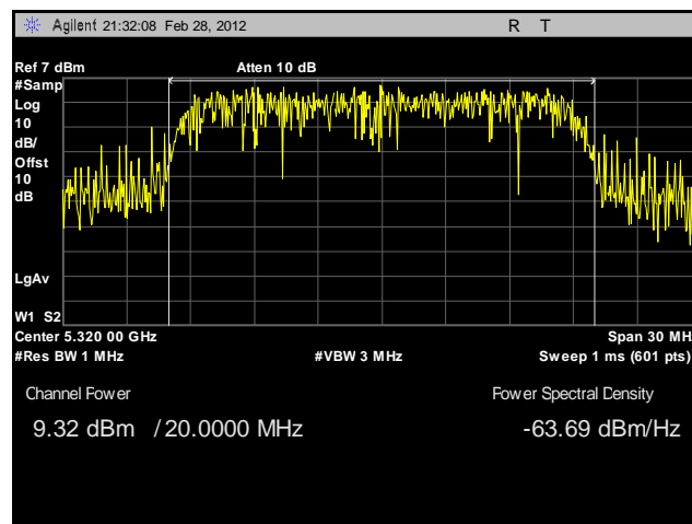
Plot 110. Conducted Output Power, 802.11n 20 MHz, Port B, 5320 MHz, Sector Antenna
