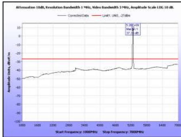
Plot 313. Radiated Spurious, 802.11n 20 MHz, 5260 MHz, 1 GHz – 7 GHz, Sector Antenna
