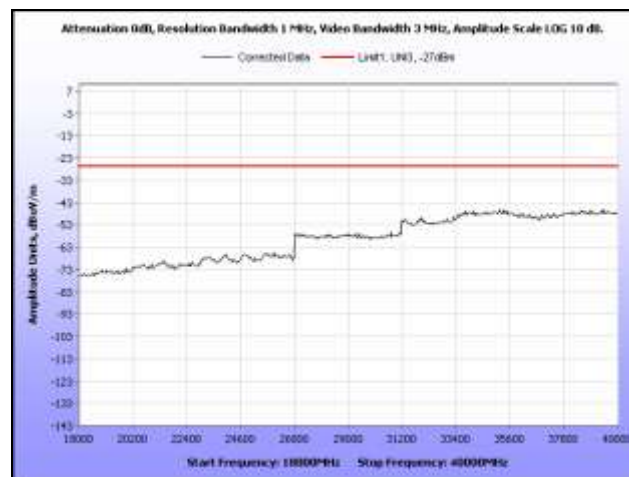
Plot 283. Radiated Spurious, 802.11n 40 MHz, 5580 MHz, 18 GHz – 40 GHz, Omni Antenna
