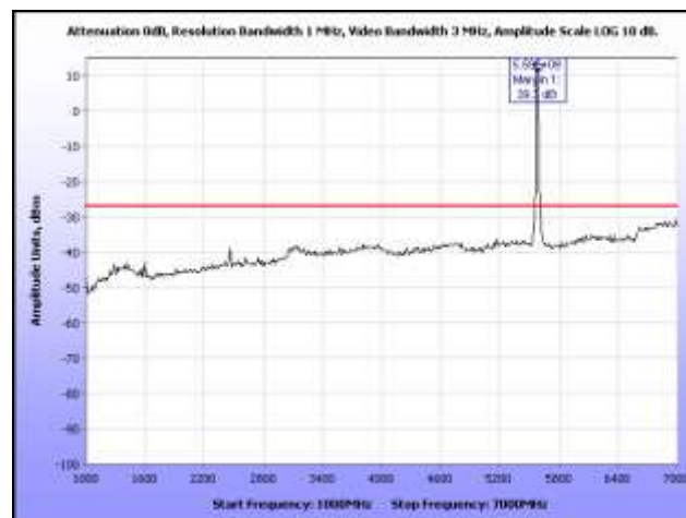
Plot 257. Radiated Spurious, 802.11n 20 MHz, 5580 MHz, 1 GHz – 7 GHz, Omni Antenna
