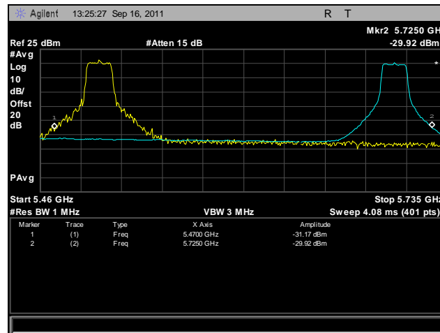
Plot 426. Frequency Stability, 802.11a, 5470 MHz – 5725 MHz @ 40°C, 120 V
