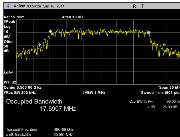
Plot 15. Occupied Bandwidth, 802.11n 20 MHz, Port A, 5500 MHz
