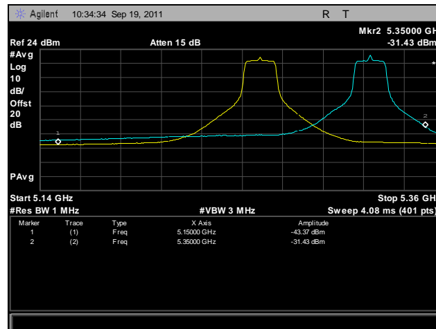
Plot 408. Frequency Stability, 802.11a, 5250 MHz – 5350 MHz @ -10°C, 120 V
