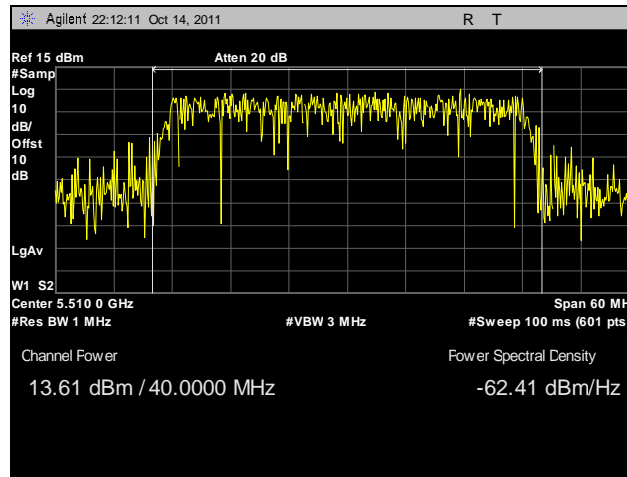
Plot 93. Conducted Output Power, 802.11n 40 MHz, Port B, 5510 MHz
