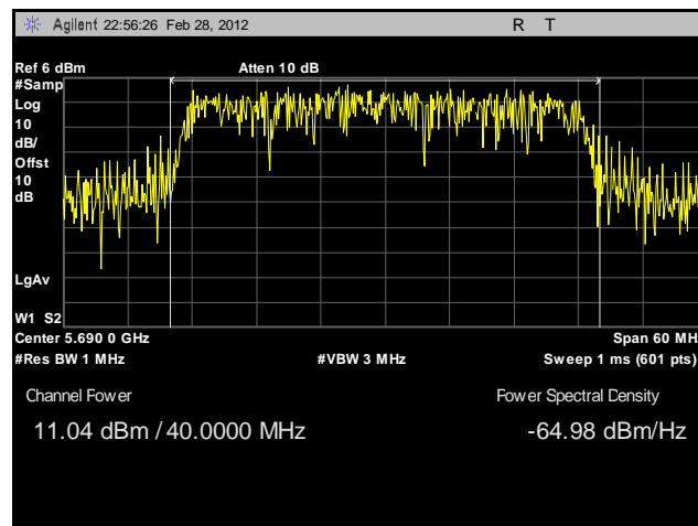
Plot 125. Conducted Output Power, 802.11n 40 MHz, Port B, 5690 MHz, Sector Antenna
