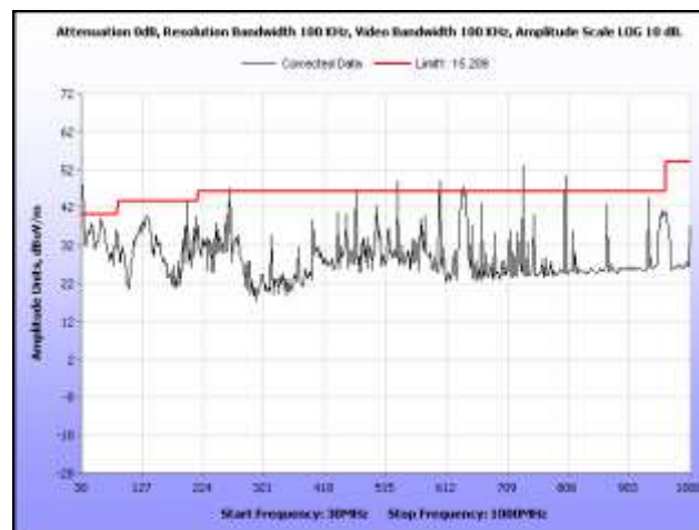
Plot 352. Radiated Spurious, 802.11n 40 MHz, 5580 MHz, 30 MHz – 1 GHz, Sector Antenna
