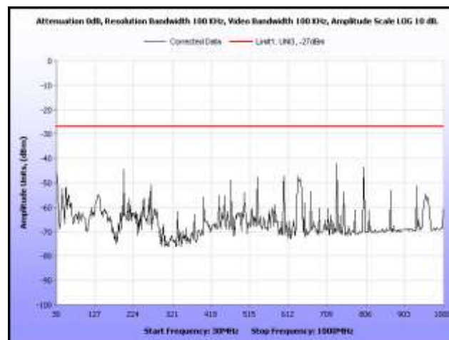
Plot 236. Radiated Spurious, 802.11a, 5700 MHz, 30 MHz – 1 GHz, Omni Antenna
