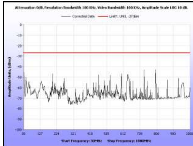
Plot 264. Radiated Spurious, 802.11n 40 MHz, 5270 MHz, 30 MHz – 1 GHz, Omni Antenna
