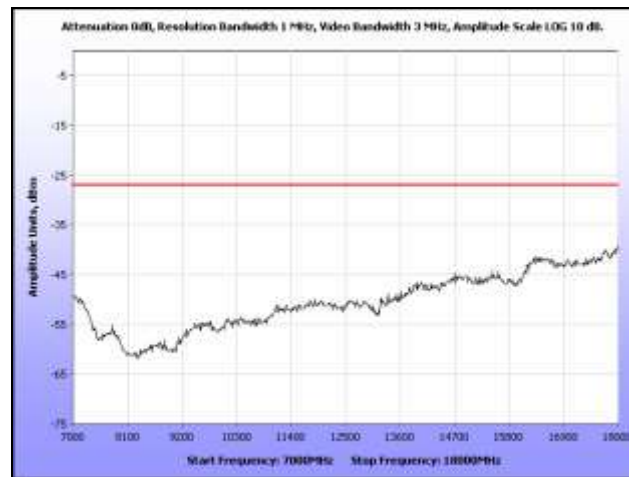
Plot 226. Radiated Spurious, 802.11a, 5320 MHz, 7 GHz – 18 GHz, Omni Antenna
