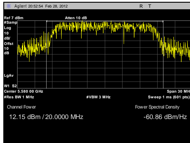
Plot 100. Conducted Output Power, 802.11a, 5580 MHz, Sector Antenna
