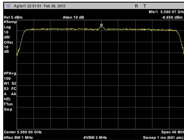
Plot 184. Peak Spectral Density, 802.11n 40 MHz, Port B, 5580 MHz, Sector Antenna
