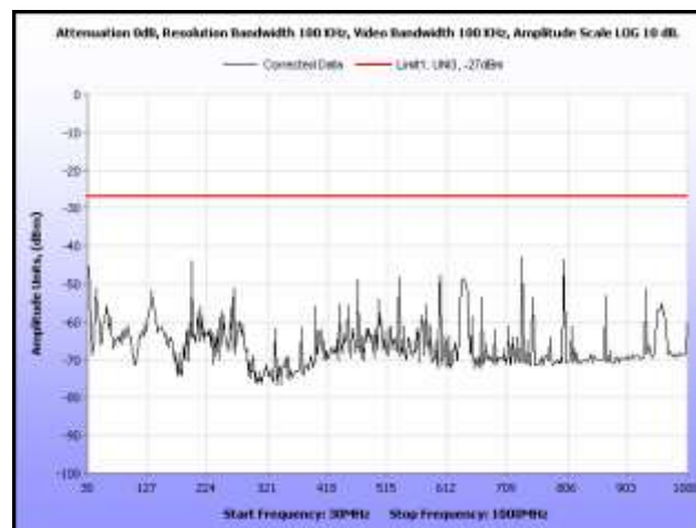
Plot 272. Radiated Spurious, 802.11n 40 MHz, 5310 MHz, 30 MHz – 1 GHz, Omni Antenna
