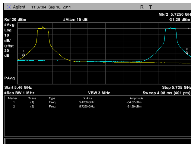
Plot 425. Frequency Stability, 802.11a, 5470 MHz – 5725 MHz @ 30°C, 120 V
