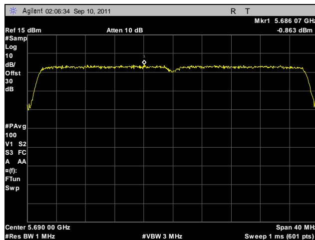
Plot 149. Peak Spectral Density, 802.11n 40 MHz, Port A, 5690 MHz
