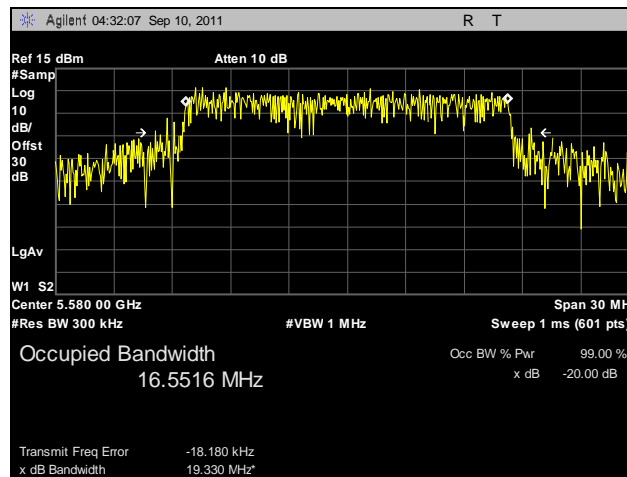
Plot 40. 99% Occupied Bandwidth, 802.11a, 5580 MHz
