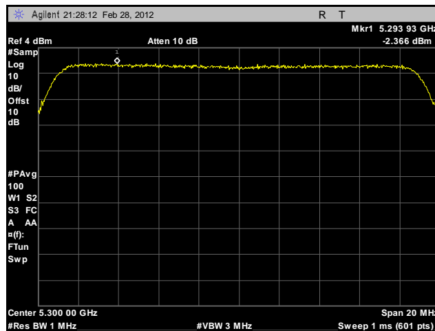
Plot 163. Peak Spectral Density, 802.11n 20 MHz, Port A, 5300 MHz, Sector Antenna
