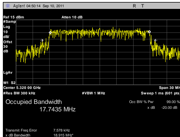
Plot 50. 99% Occupied Bandwidth, 802.11n 20 MHz, Port B, 5320 MHz
