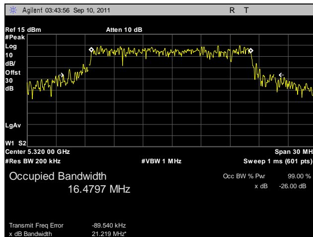
Plot 8. Occupied Bandwidth, 802.11a, 5320 MHz
