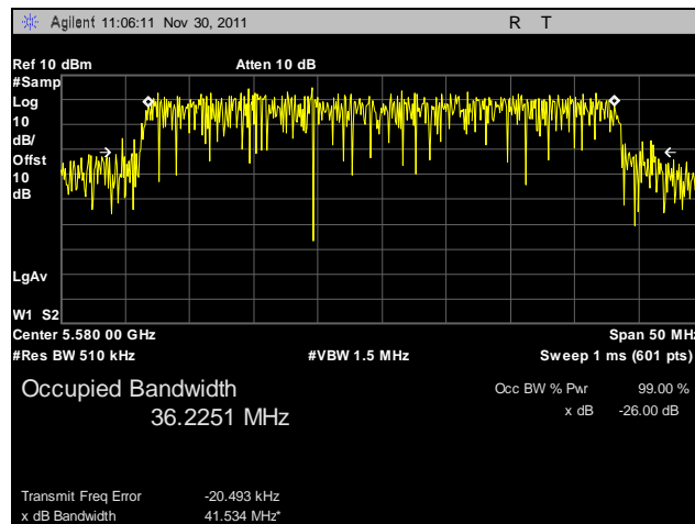
Plot 58. 99% Occupied Bandwidth, 802.11n 40 MHz, Port A, 5580 MHz
