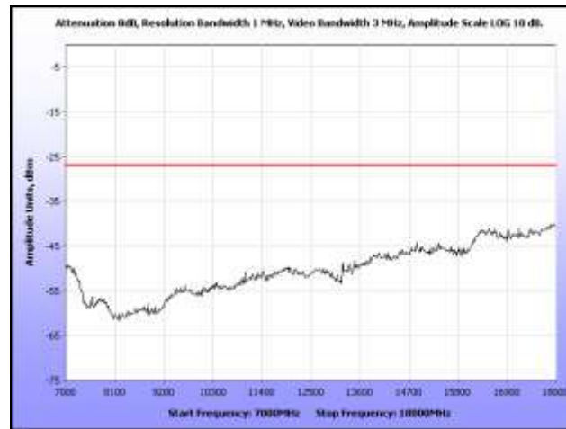
Plot 246. Radiated Spurious, 802.11n 20 MHz, 5300 MHz, 7 GHz – 18 GHz, Omni Antenna
