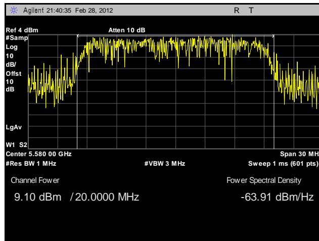
Plot 106. Conducted Output Power, 802.11n 20 MHz, Port A, 5580 MHz, Sector Antenna
