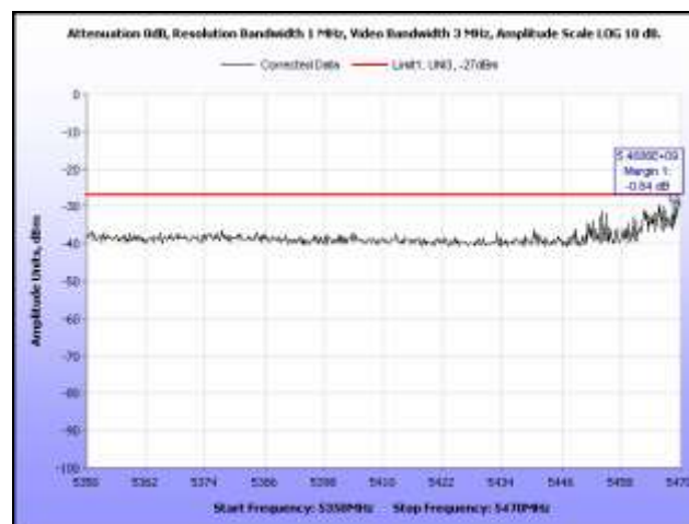
Plot 382. EIRP, 802.11n 40 MHz, 5510 MHz, Band Edge, Sector Antenna
