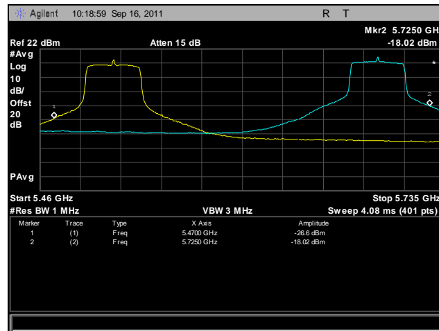
Plot 466. Frequency Stability, 802.11n 40 MHz, 5470 MHz – 5725 MHz @ 20°C, 108 V
