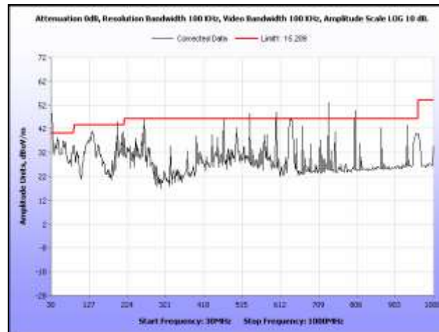
Plot 288. Radiated Spurious, 802.11a, 5260 MHz, 30 MHz – 1 GHz, Sector Antenna
