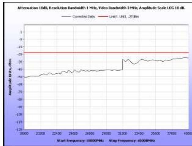
Plot 315. Radiated Spurious, 802.11n 20 MHz, 5260 MHz, 18 GHz – 40 GHz, Sector Antenna
