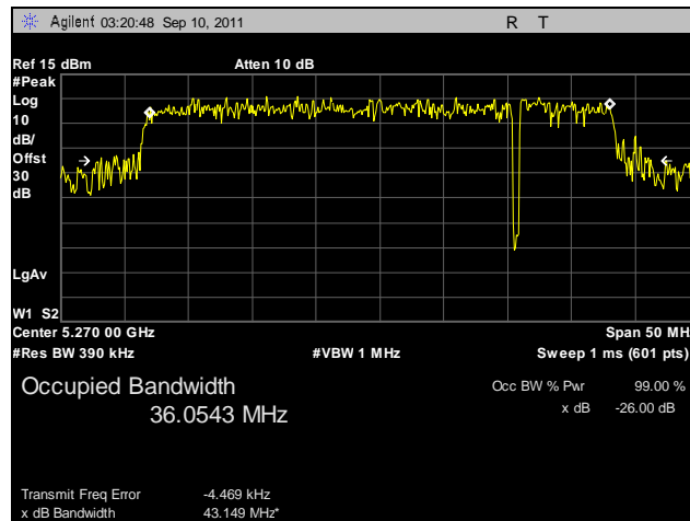
Plot 30. Occupied Bandwidth, 802.11n 40 MHz, Port B, 5270 MHz
