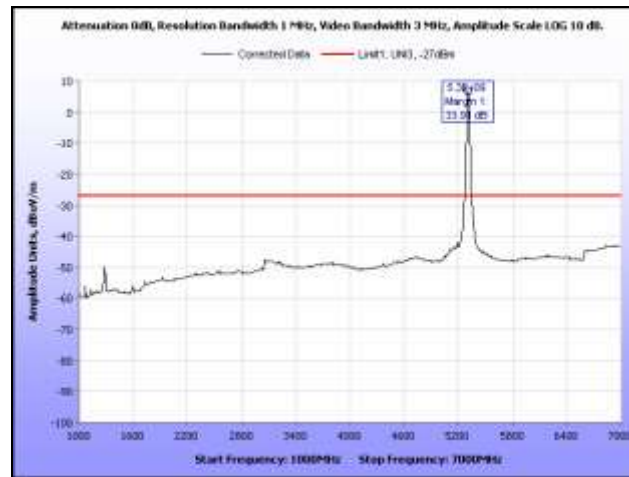
Plot 273. Radiated Spurious, 802.11n 40 MHz, 5310 MHz, 1 GHz – 7 GHz, Omni Antenna
