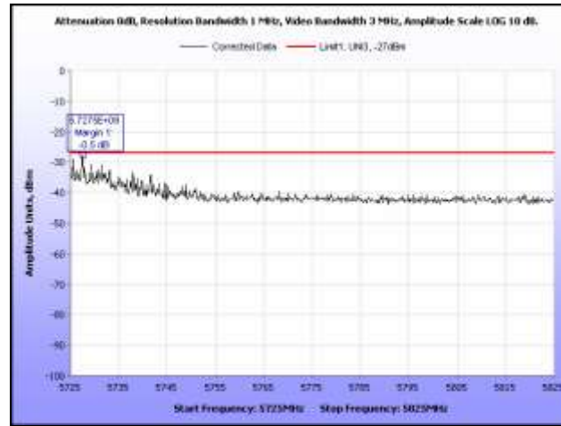
Plot 371. EIRP, 802.11n 40 MHz, 5690 MHz, Band Edge, Omni Antenna
