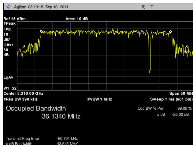
Plot 32. Occupied Bandwidth, 802.11n 40 MHz, Port B, 5310 MHz
