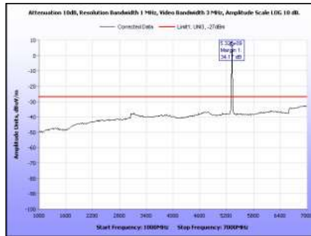
Plot 321. Radiated Spurious, 802.11n 20 MHz, 5320 MHz, 1 GHz – 7 GHz, Sector Antenna
