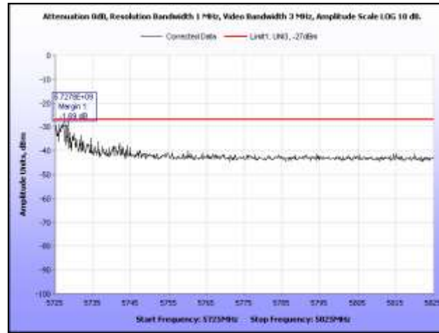
Plot 383. EIRP, 802.11n 40 MHz, 5690 MHz, Band Edge, Sector Antenna
