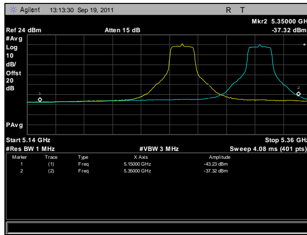
Plot 429. Frequency Stability, 802.11n 20 MHz, 5250 MHz – 5350 MHz @ -20°C, 120 V
