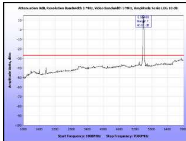
Plot 229. Radiated Spurious, 802.11a, 5500 MHz, 1 GHz – 7 GHz, Omni Antenna
