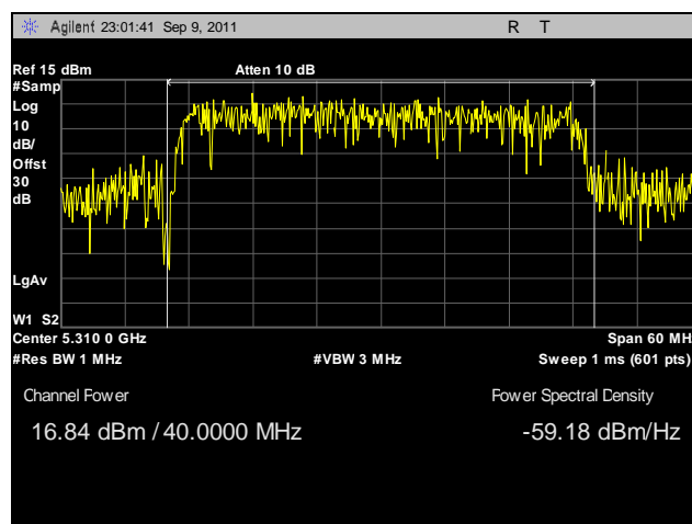
Plot 92. Conducted Output Power, 802.11n 40 MHz, Port B, 5310 MHz
