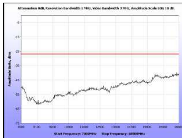
Plot 254. Radiated Spurious, 802.11n 20 MHz, 5500 MHz, 7 GHz – 18 GHz, Omni Antenna
