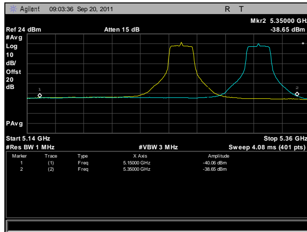
Plot 439. Frequency Stability, 802.11n 20 MHz, 5250 MHz – 5350 MHz @ 55°C, 120 V
