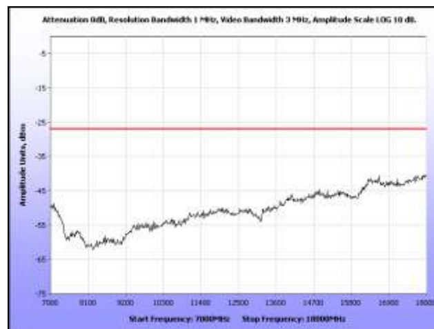
Plot 278. Radiated Spurious, 802.11n 40 MHz, 5510 MHz, 7 GHz – 18 GHz, Omni Antenna
