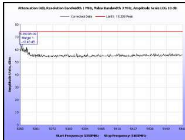
Plot 401. Restricted Band, 802.11n 20 MHz, 5320 MHz, Peak, Sector Antenna
