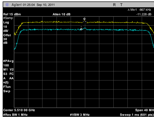
Plot 213. Peak Excursion, 802.11n 40 MHz, Port B, 5510 MHz
