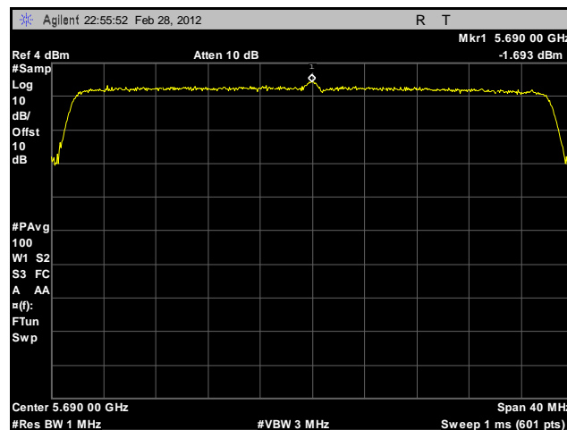
Plot 185. Peak Spectral Density, 802.11n 40 MHz, Port B, 5690 MHz, Sector Antenna
