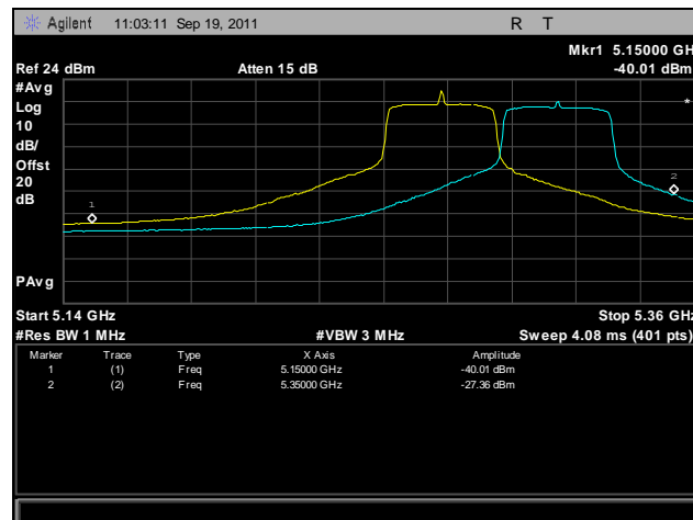
Plot 452. Frequency Stability, 802.11n 40 MHz, 5250 MHz – 5350 MHz @ -10°C, 120 V
