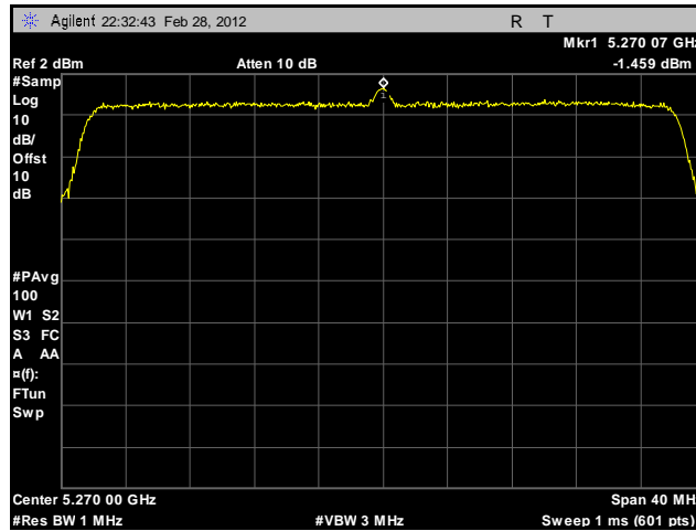
Plot 180. Peak Spectral Density, 802.11n 40 MHz, Port B, 5270 MHz, Sector Antenna
