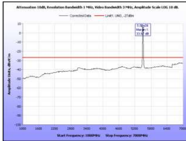
Plot 301. Radiated Spurious, 802.11a, 5500 MHz, 1 GHz – 7 GHz, Sector Antenna
