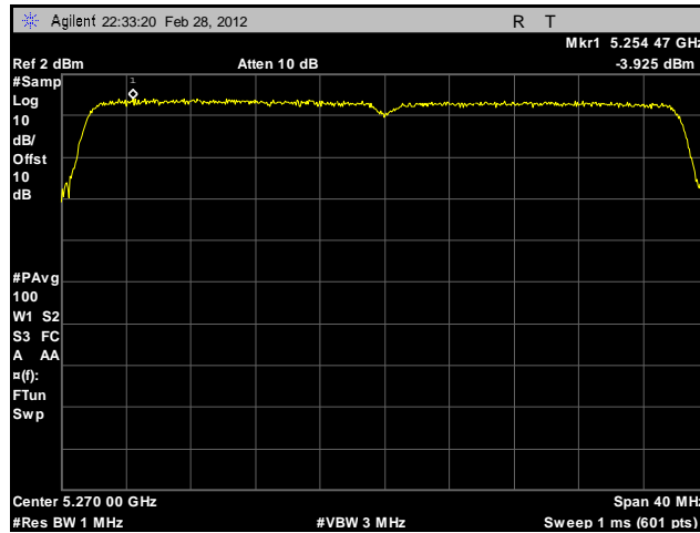
Plot 174. Peak Spectral Density, 802.11n 40 MHz, Port A, 5270 MHz, Sector Antenna
