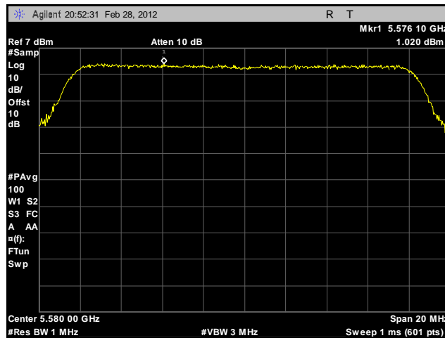
Plot 160. Peak Spectral Density, 802.11a, 5580 MHz, Sector Antenna
