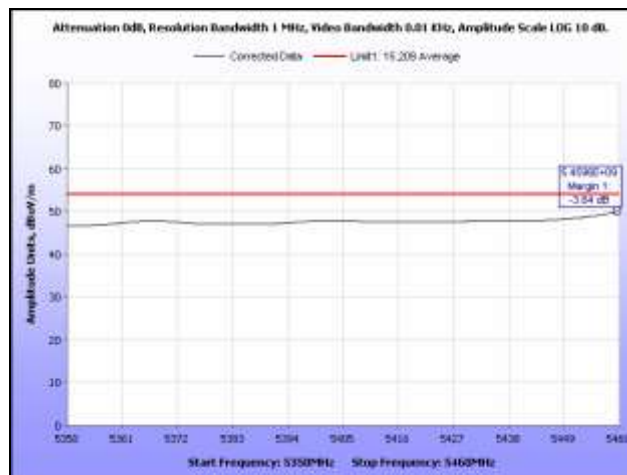
Plot 386. Restricted Band, 802.11a, 5500 MHz, Average, Omni Antenna
