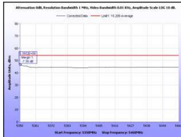
Plot 400. Restricted Band, 802.11n 20 MHz, 5320 MHz, Average, Sector Antenna
