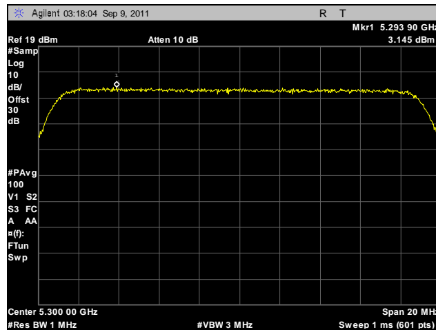
Plot 133. Peak Spectral Density, 802.11n 20 MHz, Port A, 5300 MHz
