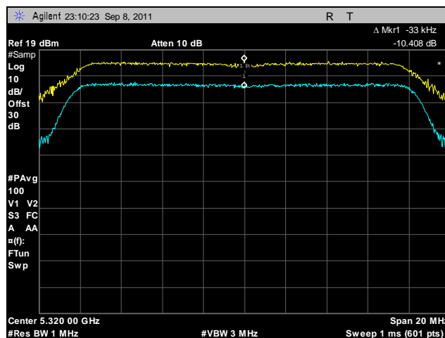
Plot 188. Peak Excursion, 802.11a, 5320 MHz
