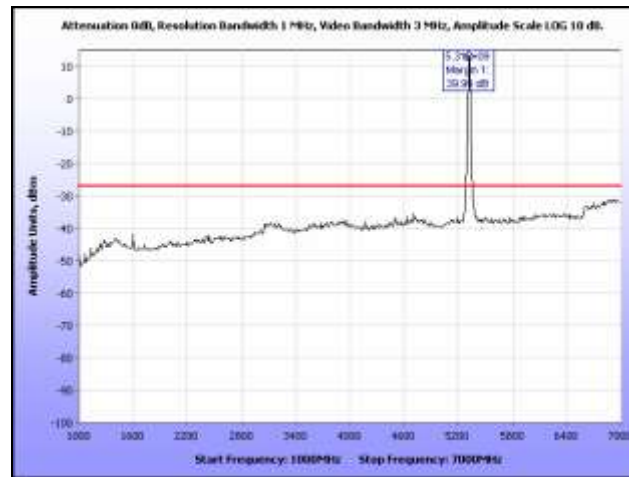
Plot 225. Radiated Spurious, 802.11a, 5320 MHz, 1 GHz – 7 GHz, Omni Antenna
