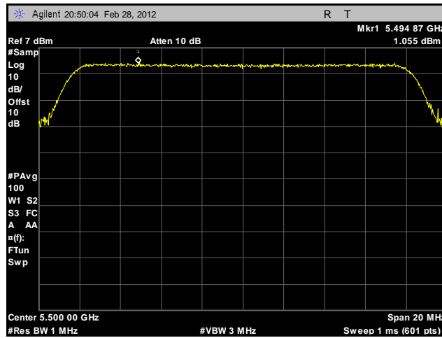
Plot 159. Peak Spectral Density, 802.11a, 5500 MHz, Sector Antenna
