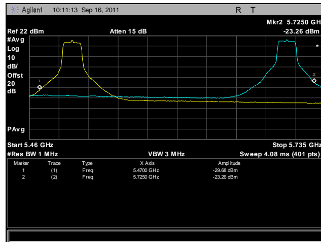
Plot 423. Frequency Stability, 802.11a, 5470 MHz – 5725 MHz @ 20°C, 120 V
