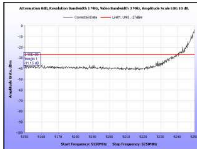
Plot 376. EIRP, 802.11n 20 MHz, 5260 MHz, Band Edge, Sector Antenna
