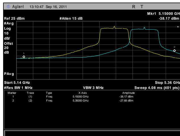
Plot 459. Frequency Stability, 802.11n 40 MHz, 5250 MHz – 5350 MHz @ 40°C, 120 V
