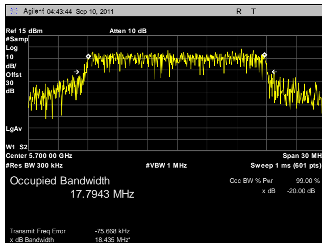
Plot 47. 99% Occupied Bandwidth, 802.11n 20 MHz, Port A, 5700 MHz
