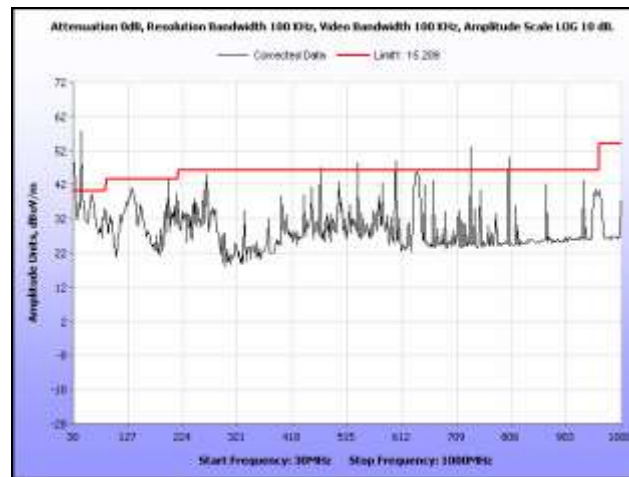
Plot 340. Radiated Spurious, 802.11n 40 MHz, 5300 MHz, 30 MHz – 1 GHz, Sector Antenna
