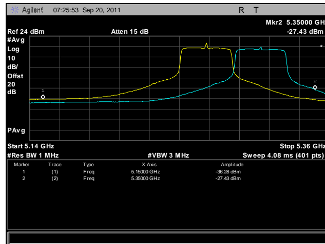
Plot 460. Frequency Stability, 802.11n 40 MHz, 5250 MHz – 5350 MHz @ 50°C, 120 V
