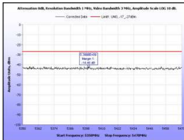
Plot 361. EIRP, 802.11a, 5320 MHz, Band Edge, Omni Antenna
