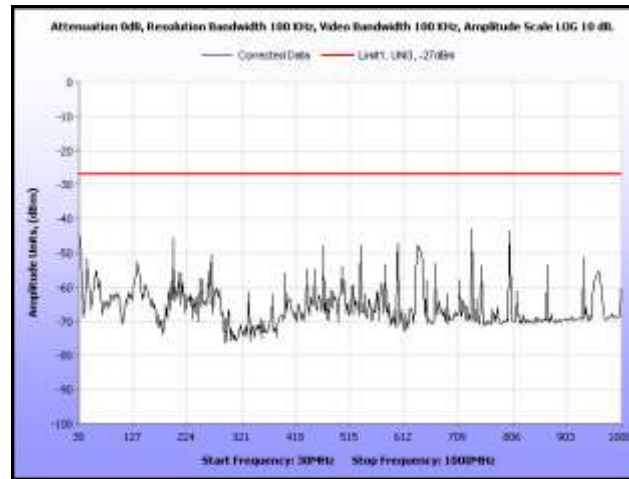
Plot 276. Radiated Spurious, 802.11n 40 MHz, 5510 MHz, 30 MHz – 1 GHz, Omni Antenna
