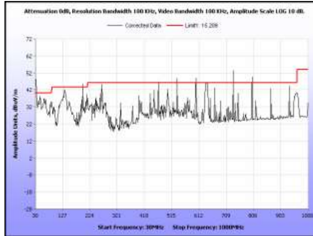
Plot 312. Radiated Spurious, 802.11n 20 MHz, 5260 MHz, 30 MHz – 1 GHz, Sector Antenna
