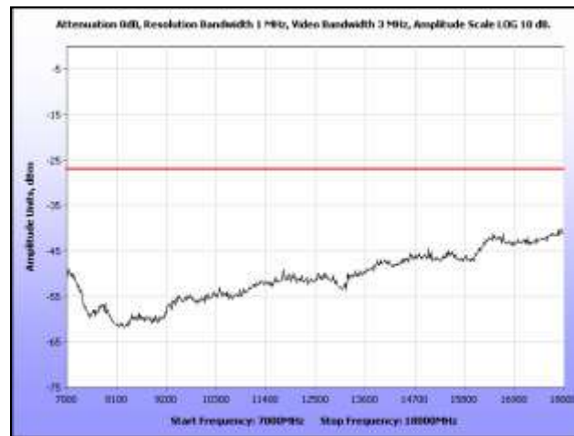
Plot 250. Radiated Spurious, 802.11n 20 MHz, 5320 MHz, 7 GHz – 18 GHz, Omni Antenna
