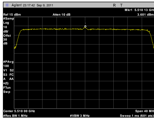
Plot 153. Peak Spectral Density, 802.11n 40 MHz, Port B, 5510 MHz
