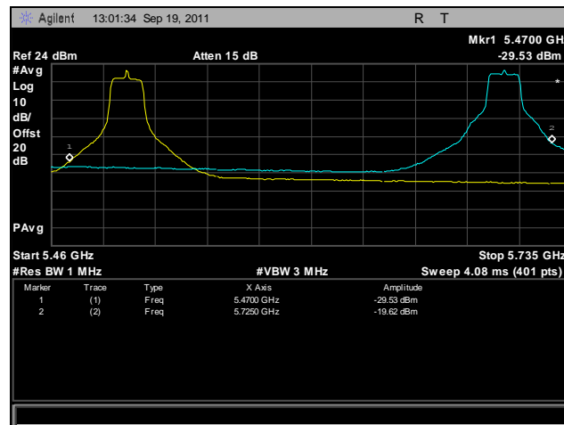
Plot 418. Frequency Stability, 802.11a, 5470 MHz – 5725 MHz @ -20°C, 120 V
