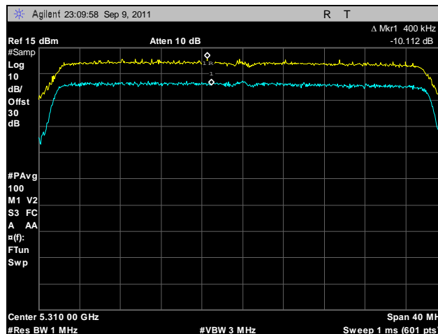
Plot 212. Peak Excursion, 802.11n 40 MHz, Port B, 5310 MHz
