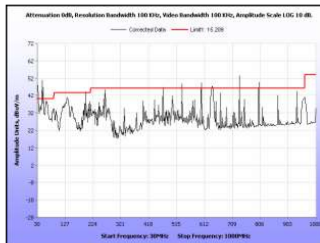
Plot 320. Radiated Spurious, 802.11n 20 MHz, 5320 MHz, 30 MHz – 1 GHz, Sector Antenna
