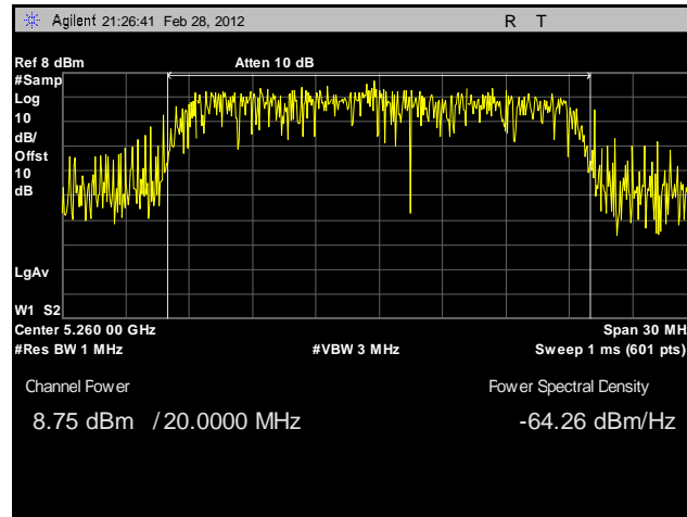
Plot 108. Conducted Output Power, 802.11n 20 MHz, Port B, 5260 MHz, Sector Antenna
