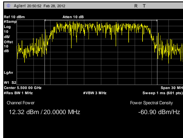
Plot 99. Conducted Output Power, 802.11a, 5500 MHz, Sector Antenna
