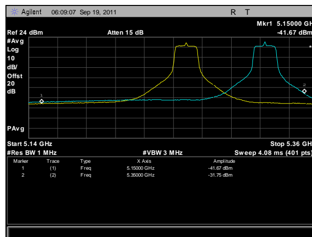
Plot 410. Frequency Stability, 802.11a, 5250 MHz – 5350 MHz @ 10°C, 120 V
