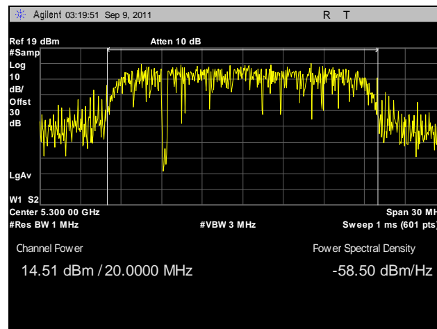
Plot 79. Conducted Output Power, 802.11n 20 MHz, Port B, 5300 MHz
