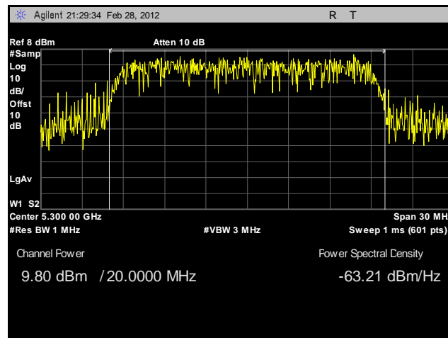
Plot 109. Conducted Output Power, 802.11n 20 MHz, Port B, 5300 MHz, Sector Antenna
