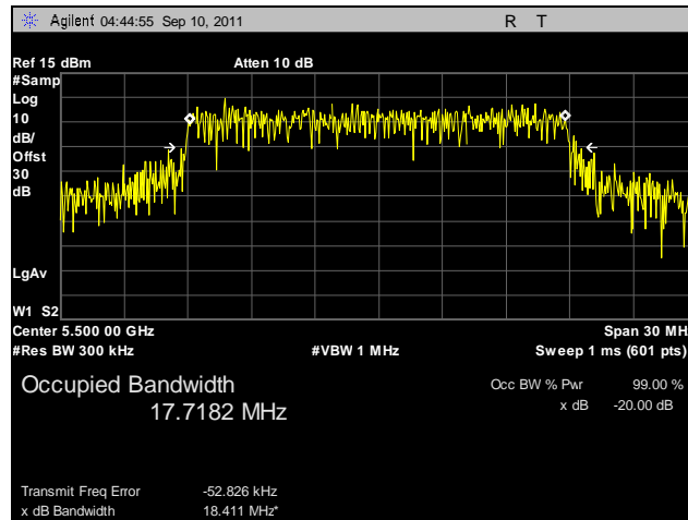
Plot 45. 99% Occupied Bandwidth, 802.11n 20 MHz, Port A, 5500 MHz
