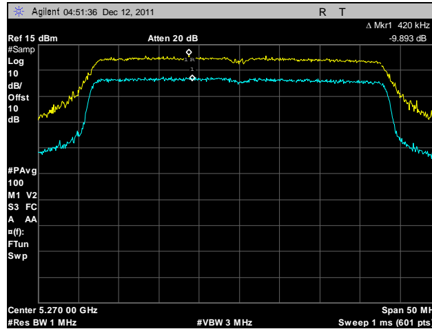
Plot 204. Peak Excursion, 802.11n 40 MHz, Port A, 5270 MHz
