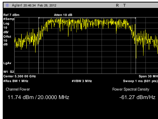
Plot 97. Conducted Output Power, 802.11a, 5300 MHz, Sector Antenna
