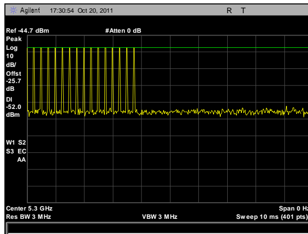
Plot 480. Radar Calibration, Bin 4
