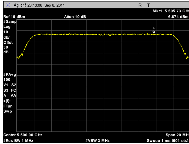
Plot 129. Peak Spectral Density, 802.11a, 5500 MHz
