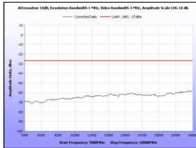
Plot 318. Radiated Spurious, 802.11n 20 MHz, 5300 MHz, 7 GHz – 18 GHz, Sector Antenna
