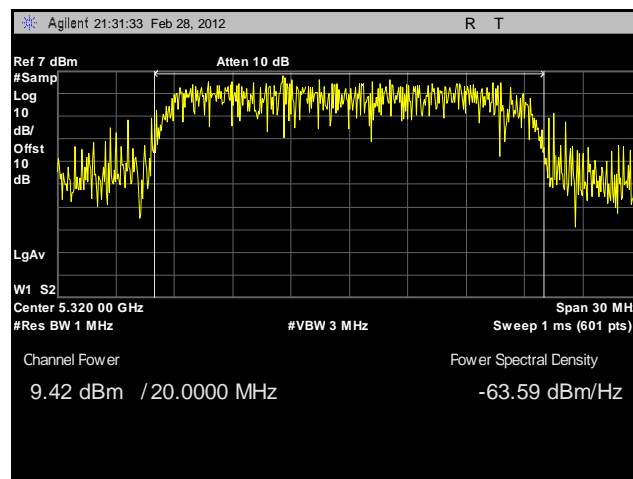
Plot 104. Conducted Output Power, 802.11n 20 MHz, Port A, 5320 MHz, Sector Antenna
