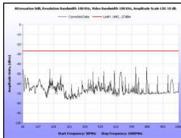
Plot 280. Radiated Spurious, 802.11n 40 MHz, 5580 MHz, 30 MHz – 1 GHz, Omni Antenna
