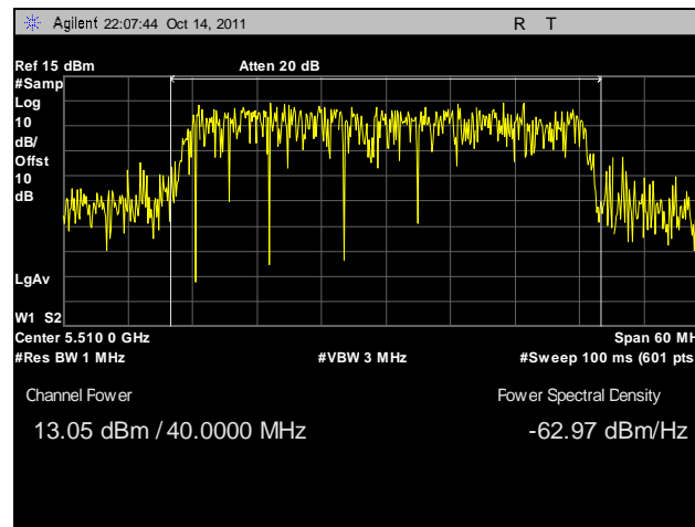
Plot 87. Conducted Output Power, 802.11n 40 MHz, Port A, 5510 MHz
