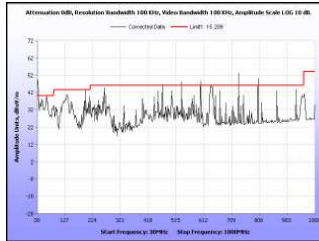
Plot 336. Radiated Spurious, 802.11n 40 MHz, 5270 MHz, 30 MHz – 1 GHz, Sector Antenna
