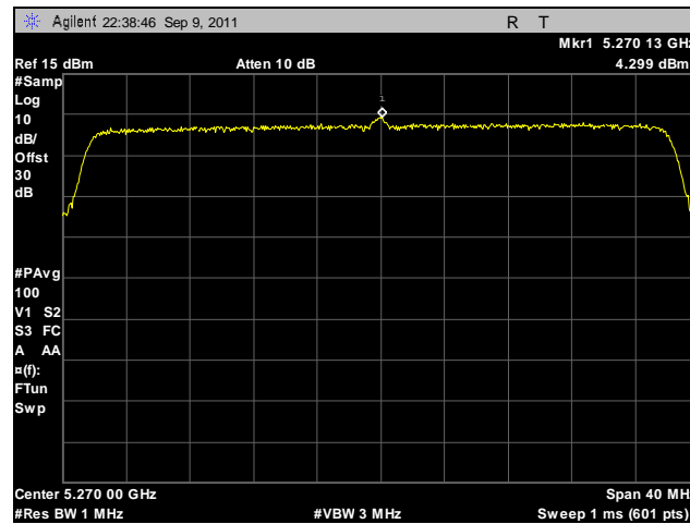
Plot 150. Peak Spectral Density, 802.11n 40 MHz, Port B, 5270 MHz
