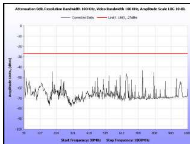
Plot 224. Radiated Spurious, 802.11a, 5320 MHz, 30 MHz – 1 GHz, Omni Antenna
