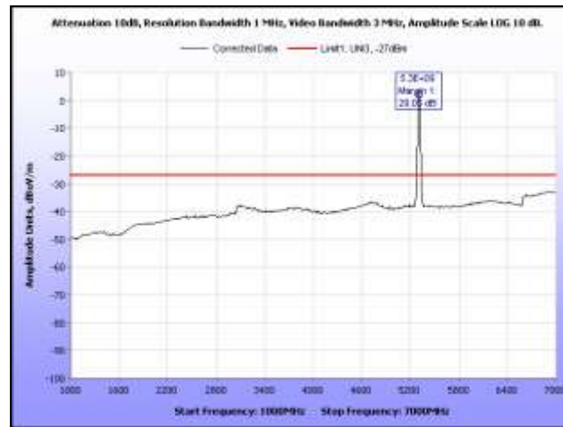
Plot 345. Radiated Spurious, 802.11n 40 MHz, 5310 MHz, 1 GHz – 7 GHz, Sector Antenna
