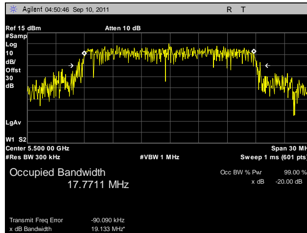
Plot 51. 99% Occupied Bandwidth, 802.11n 20 MHz, Port B, 5500 MHz
