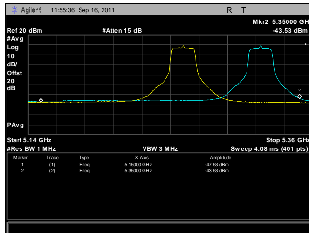
Plot 436. Frequency Stability, 802.11n 20 MHz, 5250 MHz – 5350 MHz @ 30°C, 120 V
