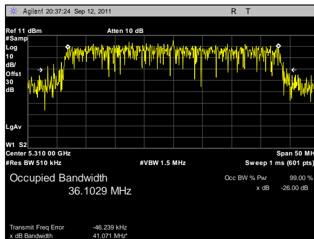
Plot 62. 99% Occupied Bandwidth, 802.11n 40 MHz, Port B, 5310 MHz
