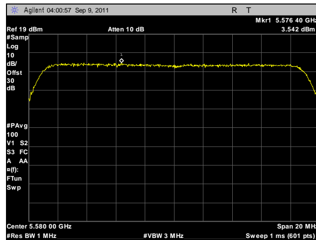
Plot 136. Peak Spectral Density, 802.11n 20 MHz, Port A, 5580 MHz
