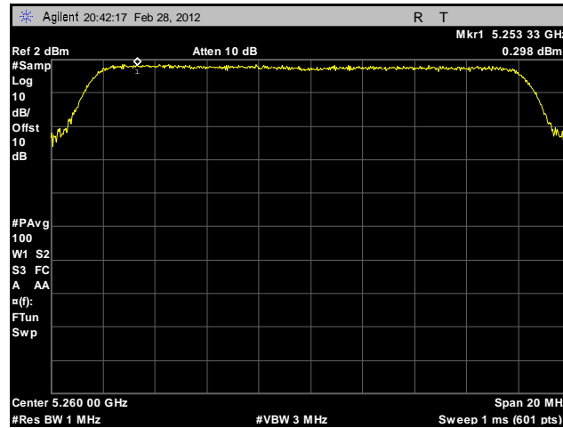
Plot 156. Peak Spectral Density, 802.11a, 5260 MHz, Sector Antenna
