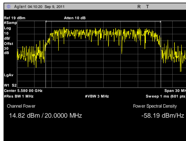
Plot 82. Conducted Output Power, 802.11n 20 MHz, Port B, 5580 MHz
