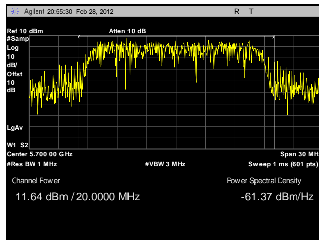
Plot 101. Conducted Output Power, 802.11a, 5700 MHz, Sector Antenna
