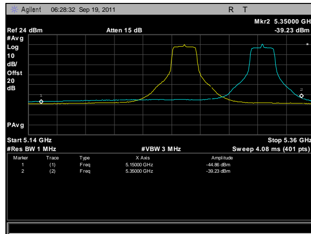
Plot 432. Frequency Stability, 802.11n 20 MHz, 5250 MHz – 5350 MHz @ 10°C, 120 V
