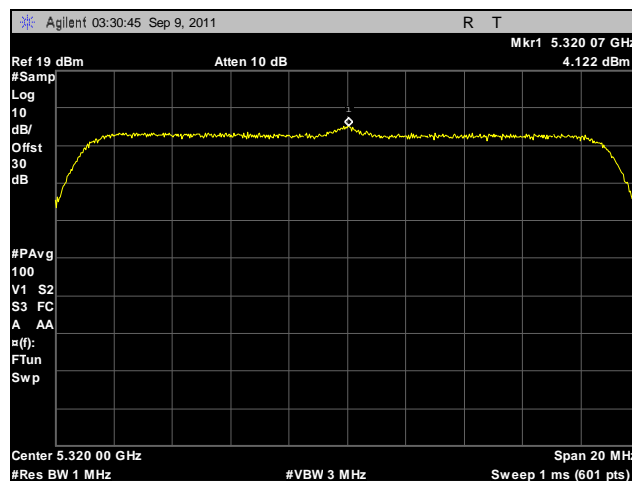
Plot 140. Peak Spectral Density, 802.11n 20 MHz, Port B, 5320 MHz
