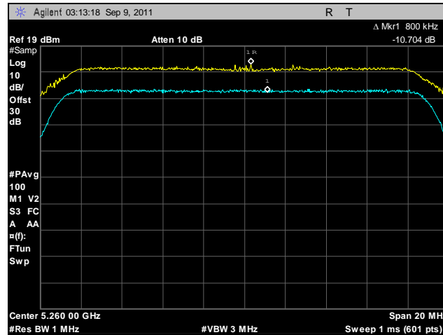
Plot 192. Peak Excursion, 802.11n 20 MHz, Port A, 5260 MHz
