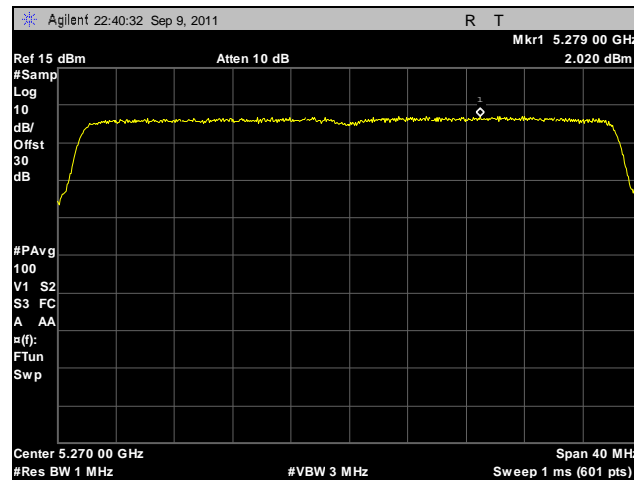
Plot 144. Peak Spectral Density, 802.11n 40 MHz, Port A, 5270 MHz
