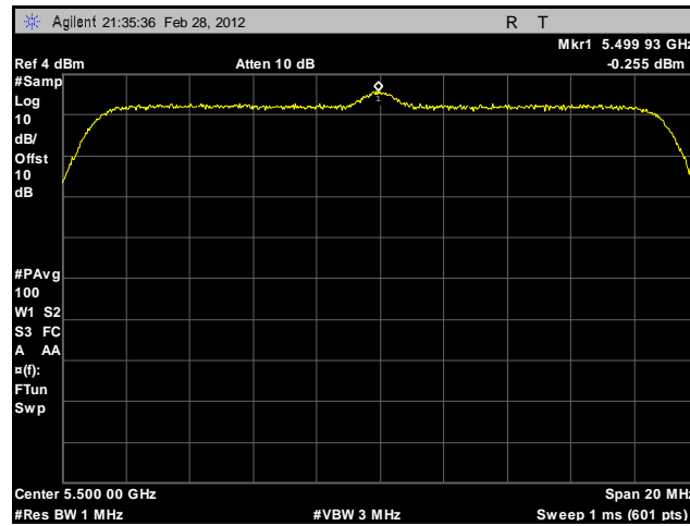
Plot 171. Peak Spectral Density, 802.11n 20 MHz, Port B, 5500 MHz, Sector Antenna
