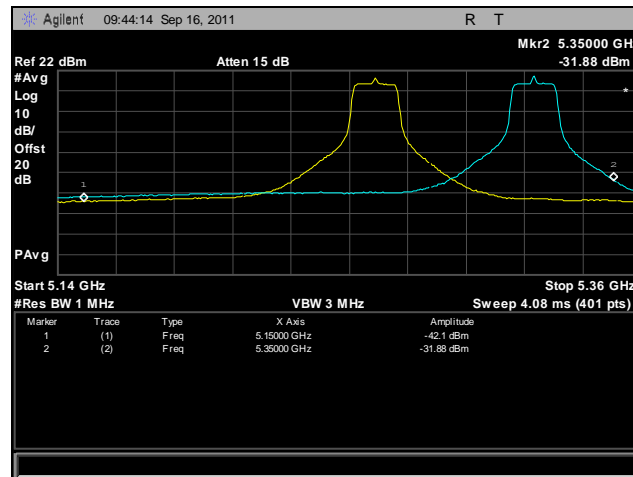
Plot 411. Frequency Stability, 802.11a, 5250 MHz – 5350 MHz @ 20°C, 108 V
