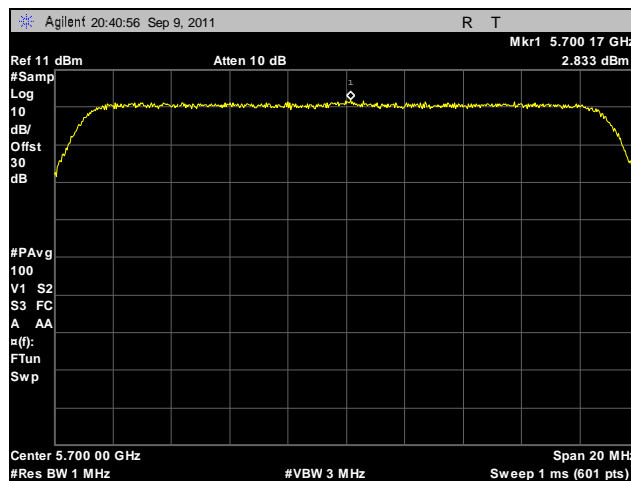
Plot 143. Peak Spectral Density, 802.11n 20 MHz, Port B, 5700 MHz
