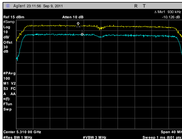
Plot 206. Peak Excursion, 802.11n 40 MHz, Port A, 5310 MHz
