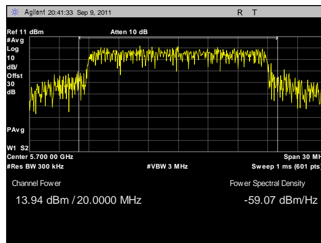
Plot 83. Conducted Output Power, 802.11n 20 MHz, Port B, 5700 MHz
