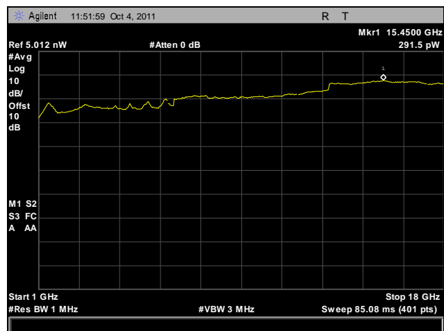
Plot 474. Receiver Spurious Emission, 5.8 GHz, 1 GHz – 18 GHz, Port A
