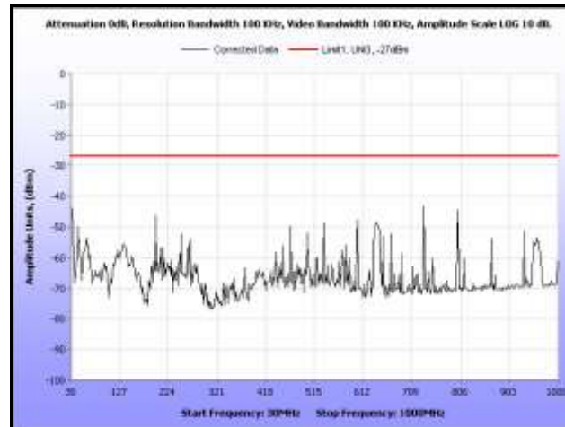
Plot 240. Radiated Spurious, 802.11n 20 MHz, 5260 MHz, 30 MHz – 1 GHz, Omni Antenna
