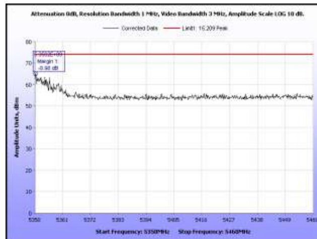
Plot 397. Restricted Band, 802.11a, 5320 MHz, Peak, Sector Antenna
