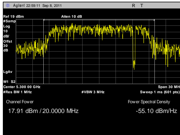
Plot 67. Conducted Output Power, 802.11a, 5300 MHz
