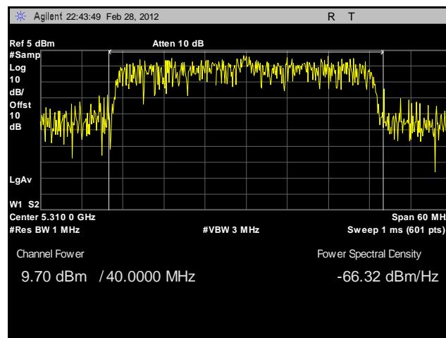
Plot 122. Conducted Output Power, 802.11n 40 MHz, Port B, 5310 MHz, Sector Antenna
