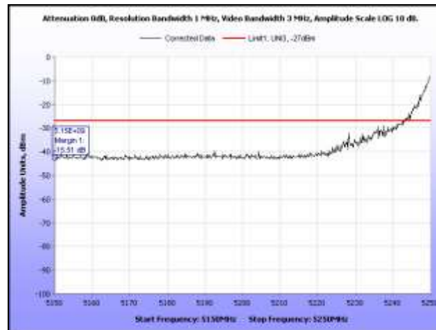
Plot 364. EIRP, 802.11n 20 MHz, 5260 MHz, Band Edge, Omni Antenna
