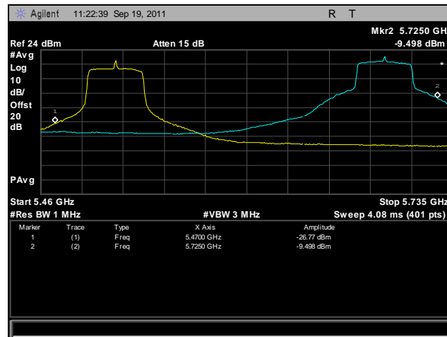
Plot 463. Frequency Stability, 802.11n 40 MHz, 5470 MHz – 5725 MHz @ -10°C, 120 V
