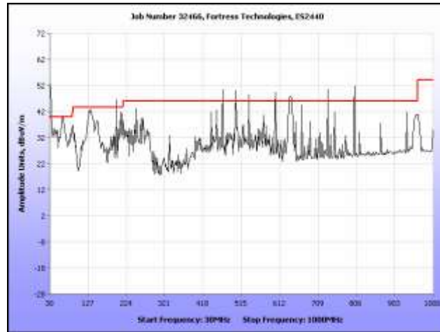
Plot 355. Radiated Spurs, Mid Channel, 5.8 GHz, 802.11n 40 MHz, 30 MHz – 1 GHz, Sector
