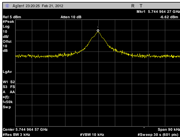
Plot 635. Peak Power Spectral Density, Low Channel, 5.8 GHz, 802.11n 20 MHz, Port B, Sector Antenna
