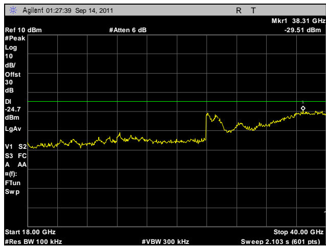
Plot 497. Conducted Spurious Emissions, High Channel, 5.8 GHz, 802.11n 40 MHz, Port B, 18 GHz – 40 GHz
