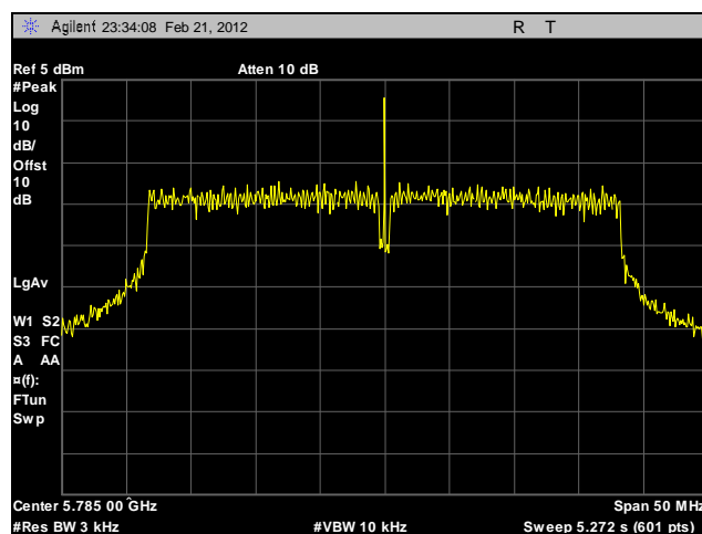
Plot 642. Peak Power Spectral Density, Mid Channel, 5.8 GHz, 802.11n 40 MHz, Port A, Sector Antenna, Determination
