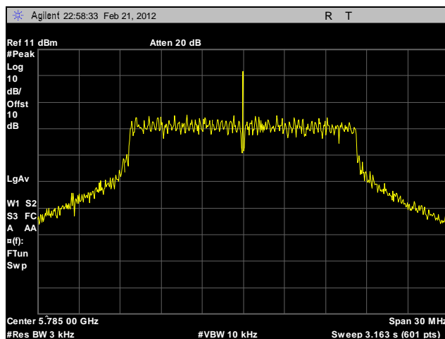
Plot 624. Peak Power Spectral Density, Mid Channel, 5.8 GHz, 802.11a, Port A, Sector Antenna, Determination
