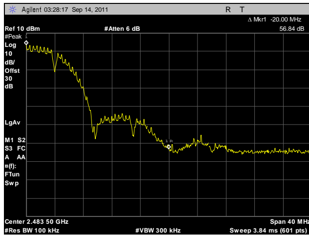
Plot 499. Conducted Band Edge, High, Channel, 2.4 GHz, 802.11b, Port A
