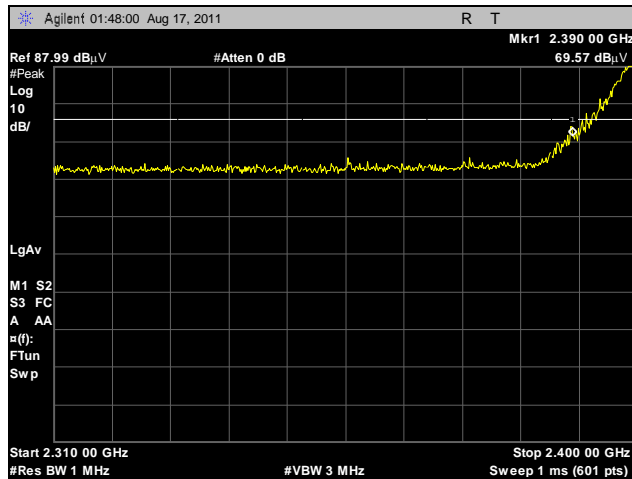
Plot 392. Radiated Restricted Band Edge, Low Channel, 2.4 GHz, 802.11g HT20, Peak, Sector
