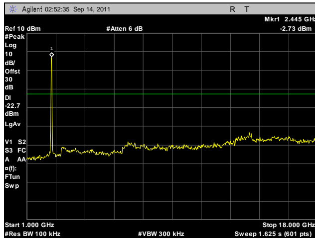
Plot 445. Conducted Spurious Emissions, Mid Channel, 2.4 GHz, 802.11g HT40, Port B, 1 GHz – 18 GHz
