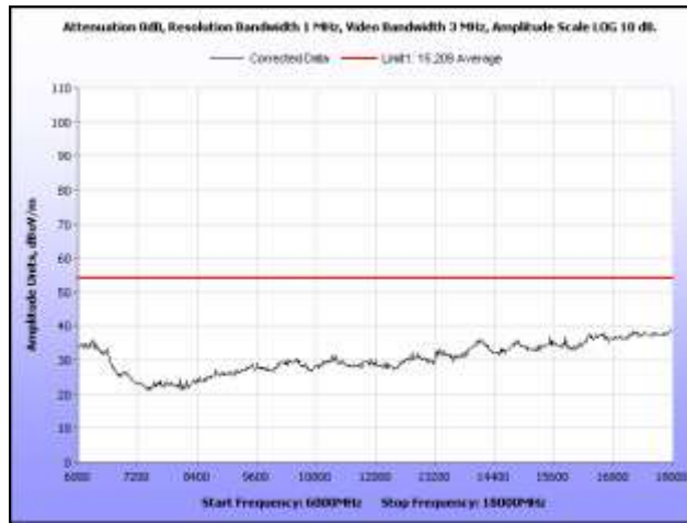
Plot 352. Radiated Spurs, Low Channel, 5.8 GHz, 802.11n 40 MHz, 6 GHz – 18 GHz, Peak under Avg., Sector
