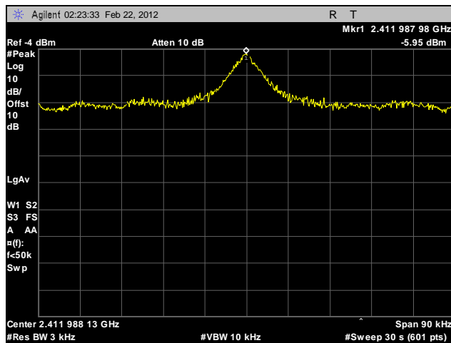
Plot 593. Peak Power Spectral Density, Low Channel, 2.4 GHz, 802.11g, Port A, Sector Antenna
