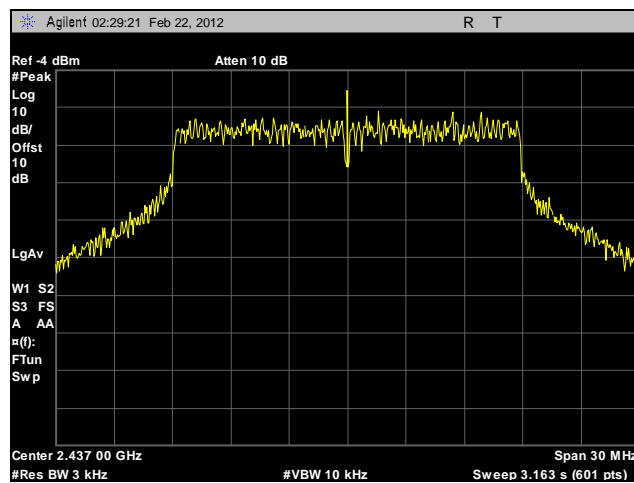
Plot 606. Peak Power Spectral Density, Mid Channel, 2.4 GHz, 802.11g HT20, Port B, Sector Antenna, Determination
