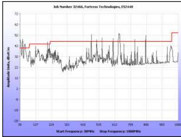
Plot 295. Radiated Spurs, Low Channel, 5.8 GHz, 802.11n 40 MHz, 30 MHz – 1 GHz, Omni
