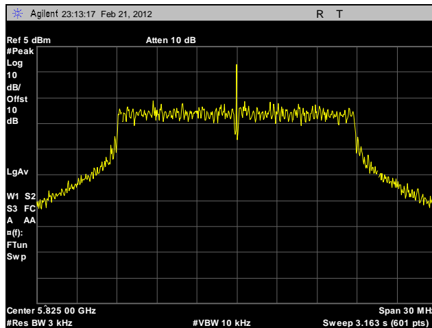
Plot 632. Peak Power Spectral Density, High Channel, 5.8 GHz, 802.11n 20 MHz, Port A, Sector Antenna, Determination
