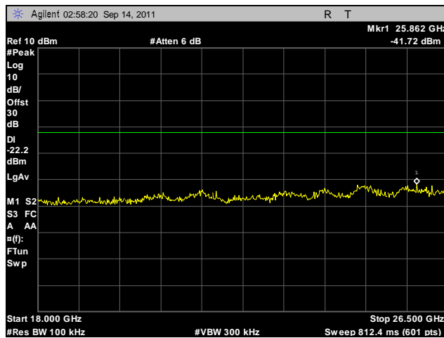
Plot 434. Conducted Spurious Emissions, High Channel, 2.4 GHz, 802.11g HT20, Port B, 18 GHz – 26.5 GHz
