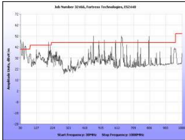
Plot 301. Radiated Spurs, Mid Channel, 5.8 GHz, 802.11n 40 MHz, 30 MHz – 1 GHz, Omni
