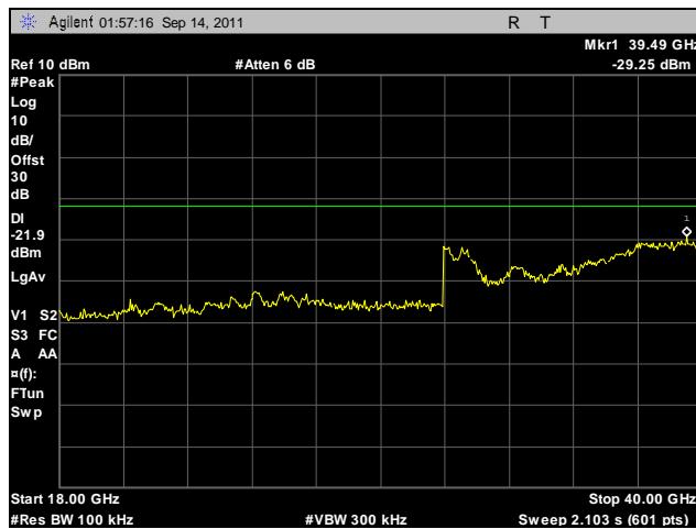
Plot 470. Conducted Spurious Emissions, Mid Channel, 5.8 GHz, 802.11n 20 MHz, Port A, 18 GHz – 40 GHz
