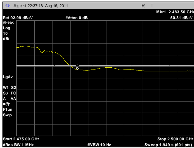
Plot 369. Radiated Restricted Band Edge, High Channel, 2.4 GHz, 802.11b, Average, Omni
