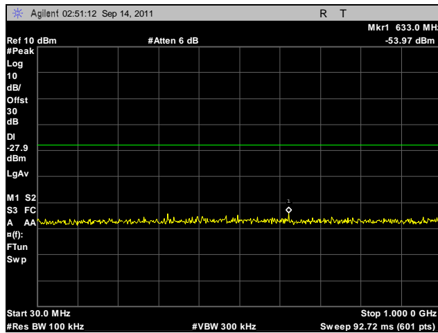
Plot 438. Conducted Spurious Emissions, Low Channel, 2.4 GHz, 802.11g HT40, Port B, 30 MHz – 1 GHz
