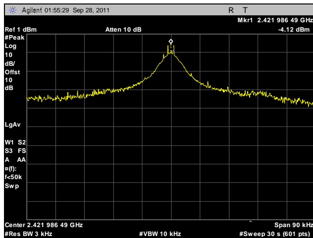
Plot 551. Peak Power Spectral Density, Low Channel, 2.4 GHz, 802.11g HT40, Port B
