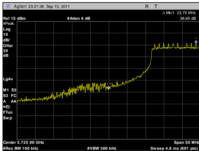
Plot 518. Conducted Band Edge, Low Channel, 5.8 GHz, 802.11n 40 MHz, Port B
