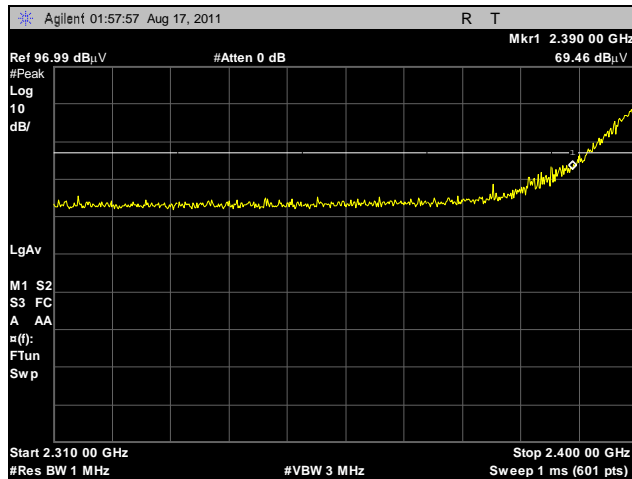
Plot 396. Radiated Restricted Band Edge, Low Channel, 2.4 GHz, 802.11g HT40, Peak, Sector
