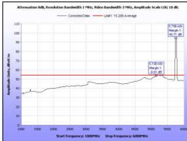
Plot 350. Radiated Spurs, Low Channel, 5.8 GHz, 802.11n 40 MHz, 1 GHz – 6 GHz, Average, Sector
