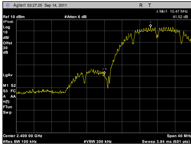
Plot 498. Conducted Band Edge, Low Channel, 2.4 GHz, 802.11b, Port A
