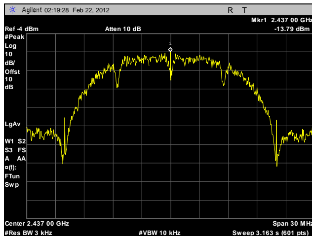
Plot 588. Peak Power Spectral Density, Mid Channel, 2.4 GHz, 802.11b, Port A, Sector Antenna, Determination
