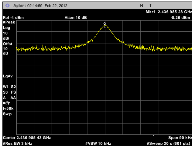
Plot 601. Peak Power Spectral Density, Mid Channel, 2.4 GHz 802.11g HT20, Port A, Sector Antenna
