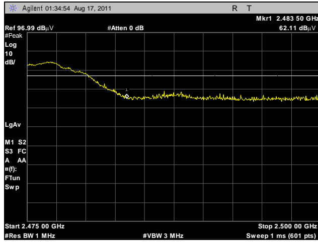
Plot 386. Radiated Restricted Band Edge, High Channel, 2.4 GHz, 802.11b, Peak, Sector
