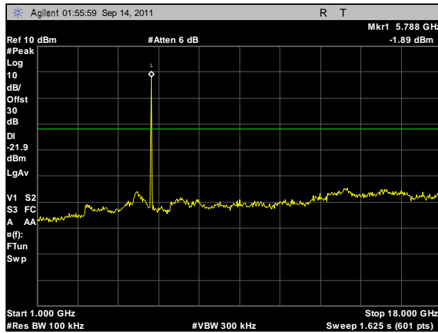
Plot 469. Conducted Spurious Emissions, Mid Channel, 5.8 GHz, 802.11n 20 MHz, Port A, 1 GHz – 18 GHz
