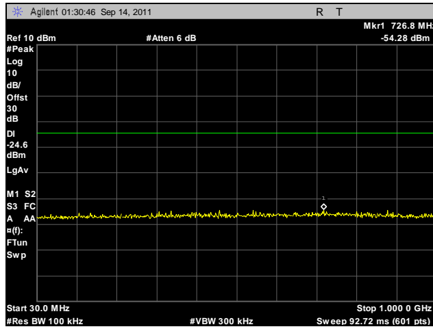
Plot 492. Conducted Spurious Emissions, High Channel, 5.8 GHz, 802.11n 40 MHz, Port A, 30 MHz – 1 GHz
