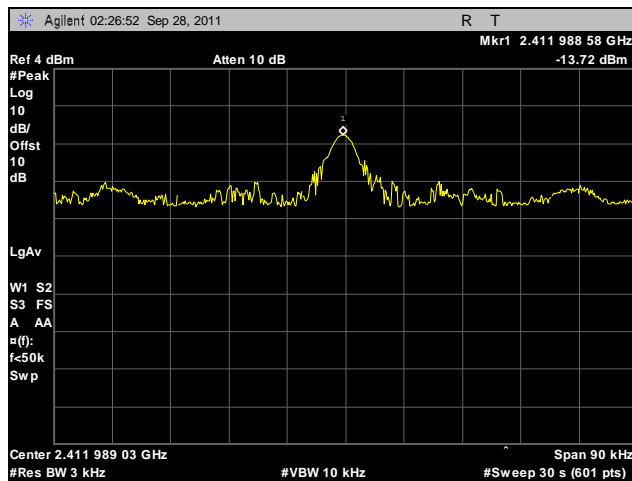
Plot 521. Peak Power Spectral Density, Low Channel, 2.4 GHz, 802.11b, Port A
