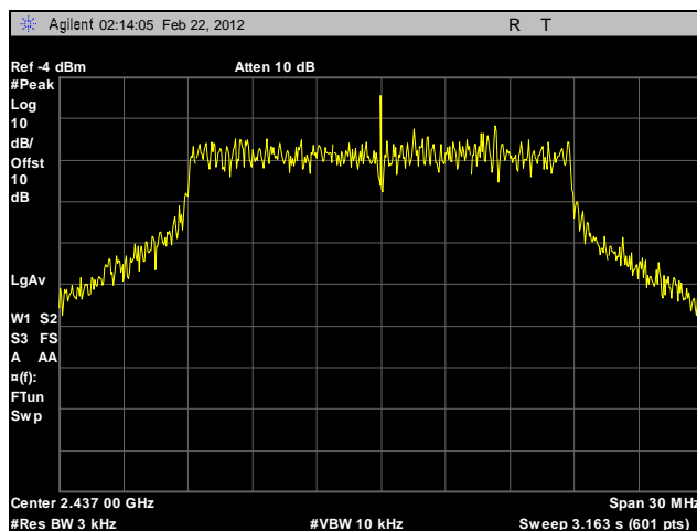
Plot 600. Peak Power Spectral Density, Mid Channel, 2.4 GHz, 802.11g HT20, Port A, Sector Antenna, Determination
