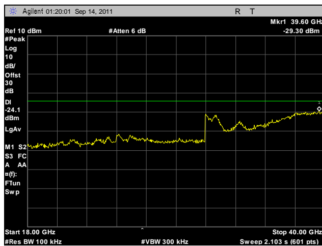
Plot 491. Conducted Spurious Emissions, Mid Channel, 5.8 GHz, 802.11n 40 MHz, Port B, 18 GHz – 40 GHz
