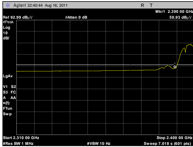
Plot 367. Radiated Restricted Band Edge, Low Channel, 2.4 GHz, 802.11b, Average, Omni
