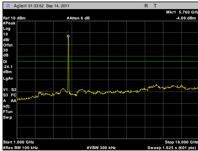
Plot 487. Conducted Spurious Emissions, Mid Channel, 5.8 GHz, 802.11n 40 MHz, Port A, 1 GHz – 18 GHz
