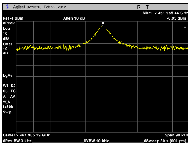
Plot 603. Peak Power Spectral Density, High Channel, 2.4 GHz, 802.11g HT20, Port A, Sector Antenna
