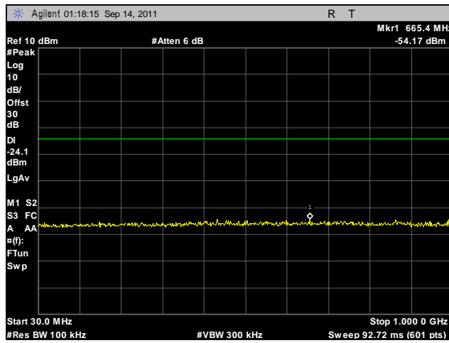
Plot 489. Conducted Spurious Emissions, Mid Channel, 5.8 GHz, 802.11n 40 MHz, Port B, 30 MHz – 1 GHz
