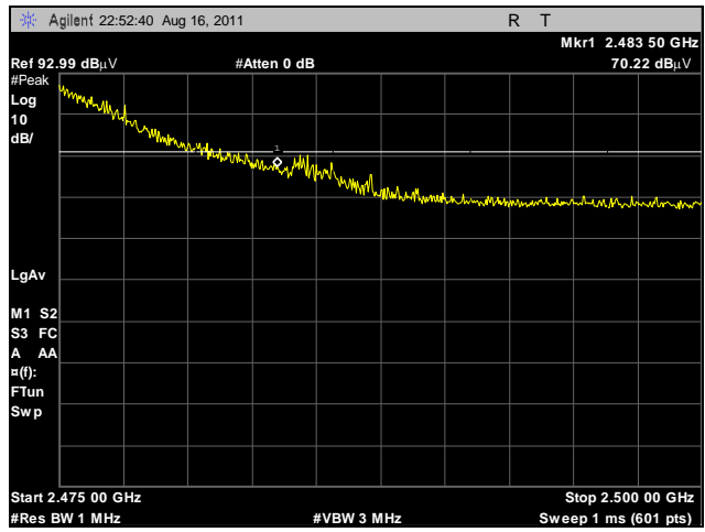
Plot 378. Radiated Restricted Band Edge, High Channel, 2.4 GHz, 802.11g HT20, Peak, Omni
