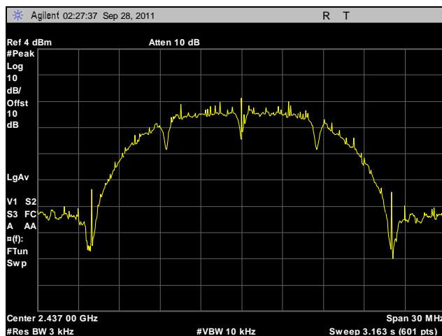
Plot 522. Peak Power Spectral Density, Mid Channel, 2.4 GHz, 802.11b, Port A, Determination
