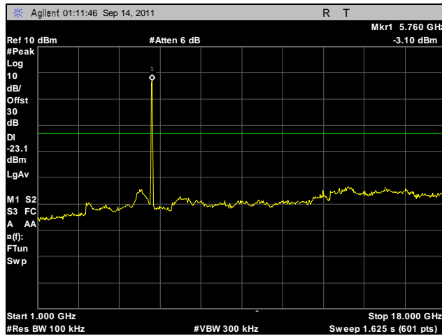
Plot 484. Conducted Spurious Emissions, Low Channel, 5.8 GHz, 802.11n 40 MHz, Port B, 1 GHz – 18 GHz
