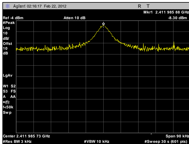
Plot 599. Peak Power Spectral Density, Low Channel, 2.4 GHz, 802.11g HT20, Port A, Sector Antenna
