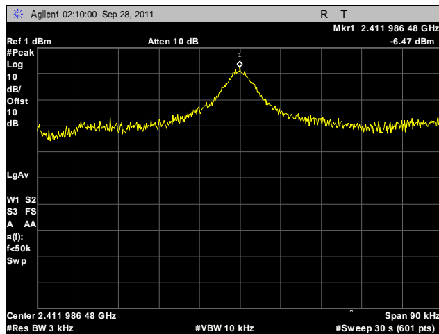
Plot 533. Peak Power Spectral Density, Low Channel, 2.4 GHz, 802.11g HT20, Port A
