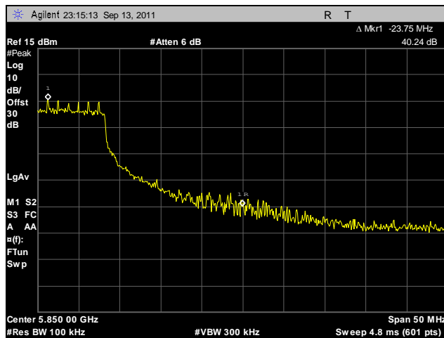
Plot 517. Conducted Band Edge, High, Channel, 5.8 GHz, 802.11n 40 MHz, Port A
