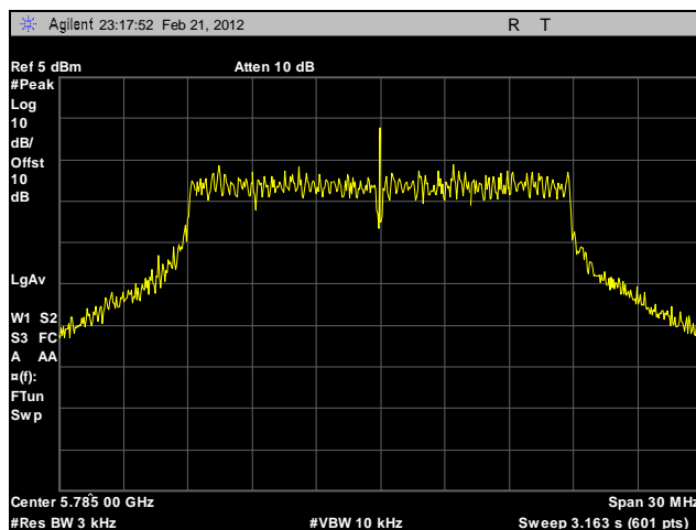
Plot 636. Peak Power Spectral Density, Mid Channel, 5.8 GHz, 802.11n 20 MHz, Port B, Sector Antenna, Determination
