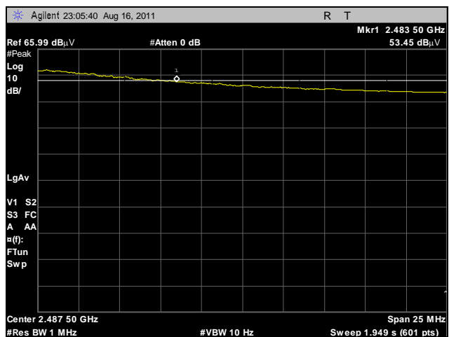
Plot 381. Radiated Restricted Band Edge, High Channel, 2.4 GHz, 802.11g HT40, Average, Omni
