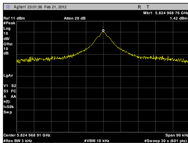
Plot 627. Peak Power Spectral Density, High Channel, 5.8 GHz, 802.11a, Port A, Sector Antenna
