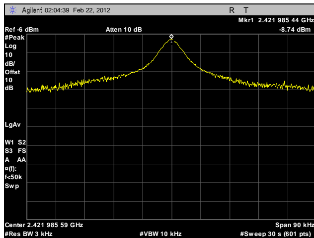
Plot 611. Peak Power Spectral Density, Low Channel, 2.4 GHz, 802.11g HT40, Port A, Sector Antenna
