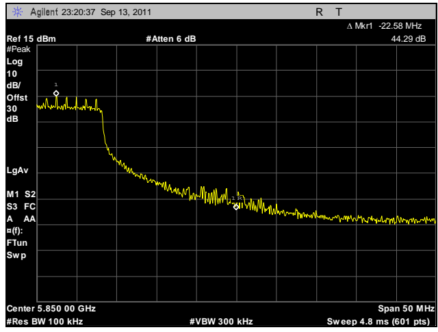
Plot 519. Conducted Band Edge, High, Channel, 5.8 GHz, 802.11n 40 MHz, Port B
