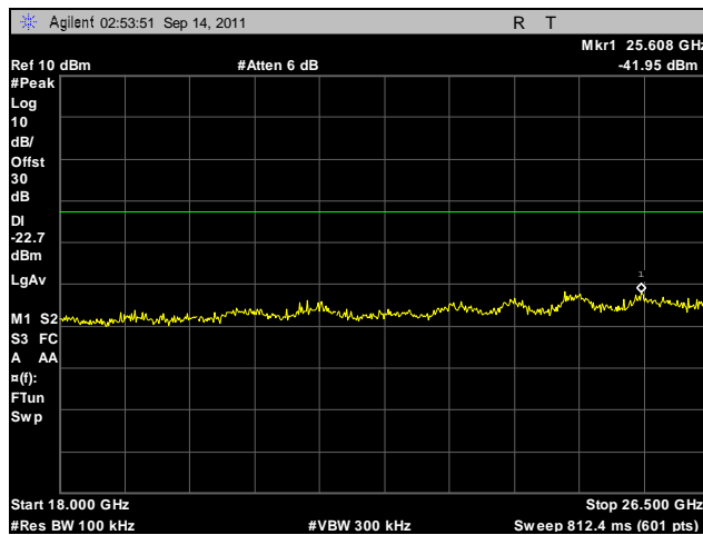
Plot 446. Conducted Spurious Emissions, Mid Channel, 2.4 GHz, 802.11g HT40, Port B, 18 GHz – 26.5 GHz
