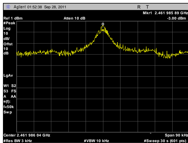
Plot 543. Peak Power Spectral Density, High Channel, 2.4 GHz, 802.11g HT20, Port B
