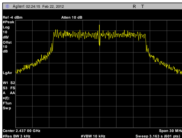
Plot 594. Peak Power Spectral Density, Mid Channel, 2.4 GHz, 802.11g, Port A, Sector Antenna, Determination
