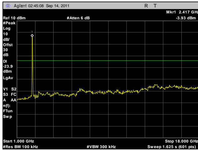
Plot 442. Conducted Spurious Emissions, Mid Channel, 2.4 GHz, 802.11g HT40, Port A, 1 GHz – 18 GHz
