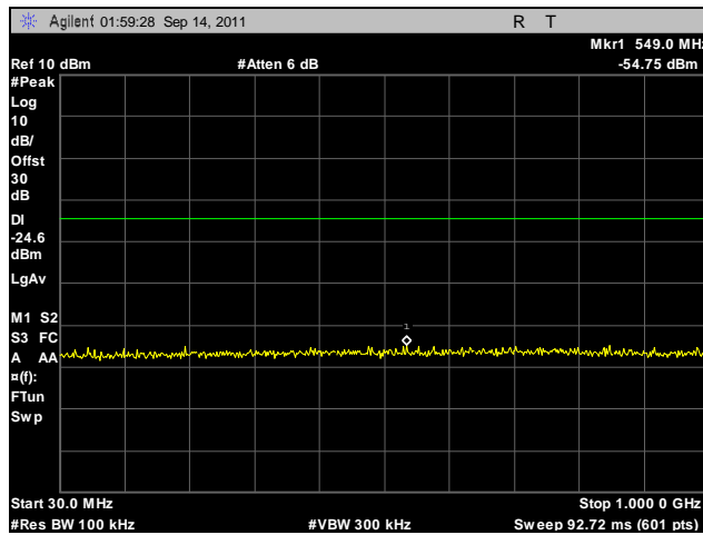
Plot 474. Conducted Spurious Emissions, High Channel, 5.8 GHz, 802.11n 20 MHz, Port A, 30 MHz – 1 GHz
