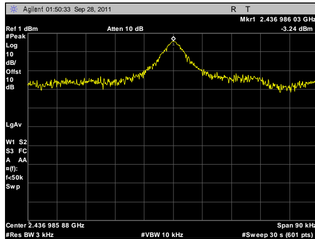
Plot 541. Peak Power Spectral Density, Mid Channel, 2.4 GHz 802.11g HT20, Port B
