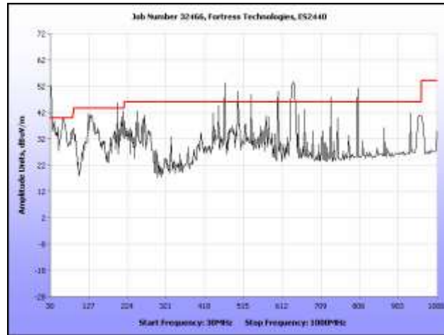
Plot 361. Radiated Spurs, High Channel, 5.8 GHz, 802.11n 40 MHz, 30 MHz – 1 GHz, Sector
