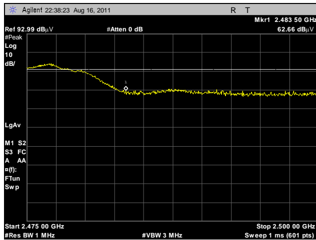
Plot 370. Radiated Restricted Band Edge, High Channel, 2.4 GHz, 802.11b, Peak, Omni
