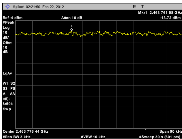
Plot 591. Peak Power Spectral Density, High Channel, 2.4 GHz, 802.11b, Port A, Sector Antenna
