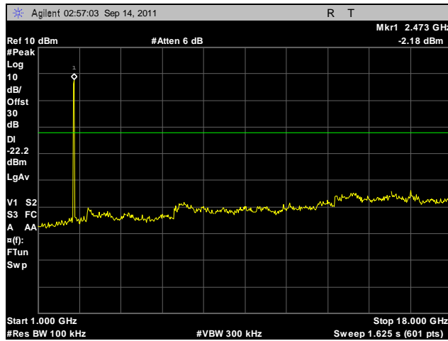
Plot 433. Conducted Spurious Emissions, High Channel, 2.4 GHz, 802.11g HT20, Port B, 1 GHz – 18 GHz
