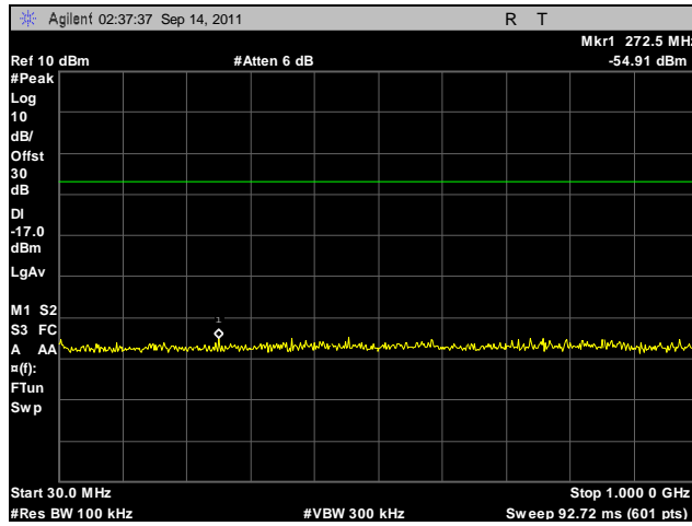
Plot 423. Conducted Spurious Emissions, Mid Channel, 2.4 GHz, 802.11g HT20, Port A, 30 MHz – 1 GHz
