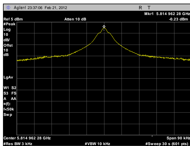
Plot 645. Peak Power Spectral Density, High Channel, 5.8 GHz, 802.11n 40 MHz, Port A, Sector Antenna
