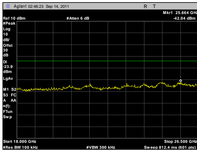
Plot 443. Conducted Spurious Emissions, Mid Channel, 2.4 GHz, 802.11g HT40, Port A, 18 GHz – 26.5 GHz
