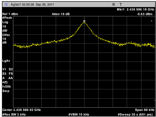
Plot 547. Peak Power Spectral Density, Mid Channel, 2.4 GHz 802.11g HT40, Port A
