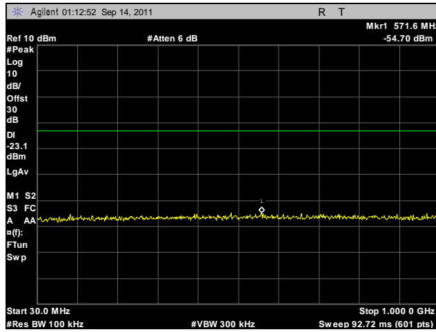
Plot 483. Conducted Spurious Emissions, Low Channel, 5.8 GHz, 802.11n 40 MHz, Port B, 30 MHz – 1 GHz
