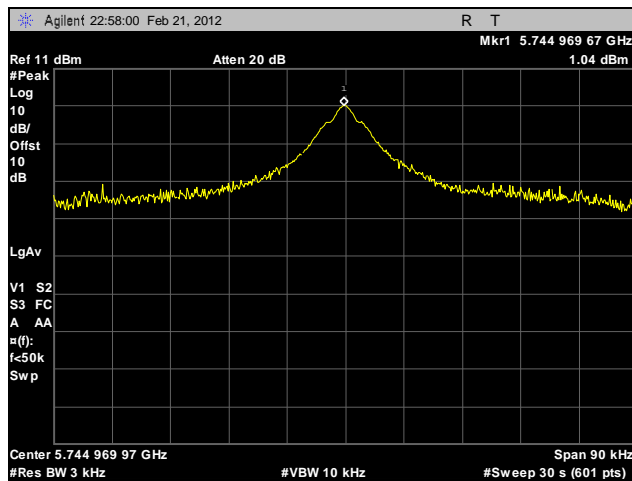
Plot 623. Peak Power Spectral Density, Low Channel, 5.8 GHz, 802.11a, Port A, Sector Antenna
