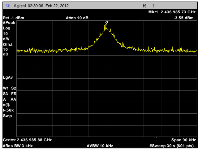
Plot 607. Peak Power Spectral Density, Mid Channel, 2.4 GHz 802.11g HT20, Port B, Sector Antenna
