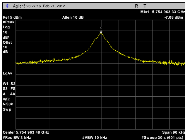
Plot 647. Peak Power Spectral Density, Low Channel, 5.8 GHz, 802.11n 40 MHz, Port B, Sector Antenna
