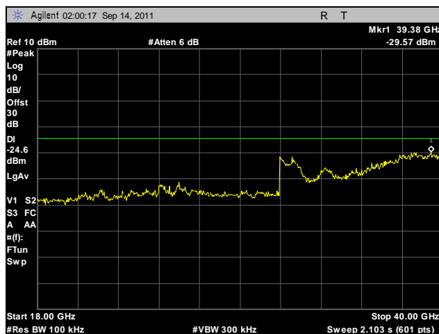
Plot 476. Conducted Spurious Emissions, High Channel, 5.8 GHz, 802.11n 20 MHz, Port A, 18 GHz – 40 GHz
