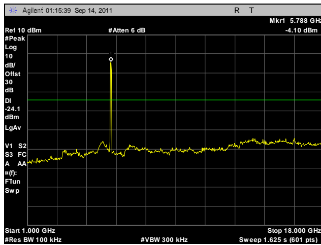
Plot 490. Conducted Spurious Emissions, Mid Channel, 5.8 GHz, 802.11n 40 MHz, Port B, 1 GHz – 18 GHz
