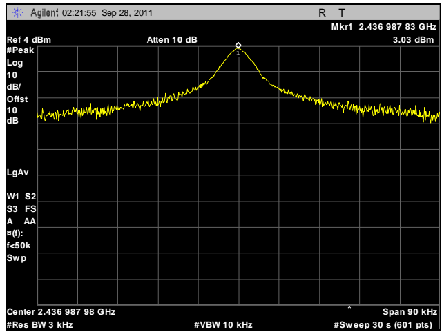
Plot 529. Peak Power Spectral Density, Mid Channel, 2.4 GHz, 802.11g, Port A
