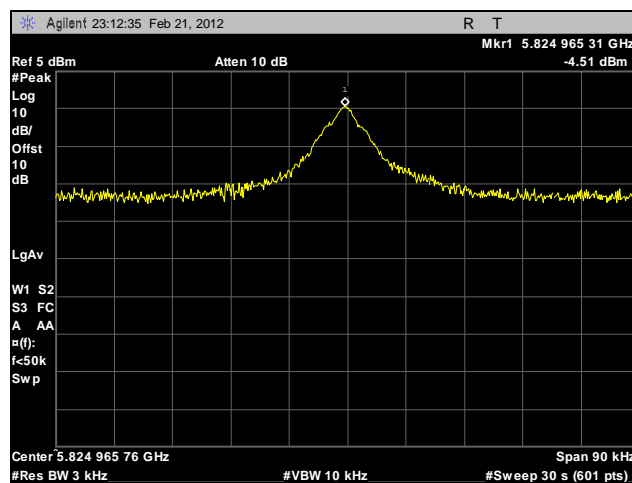
Plot 639. Peak Power Spectral Density, High Channel, 5.8 GHz, 802.11n 20 MHz, Port B, Sector Antenna
