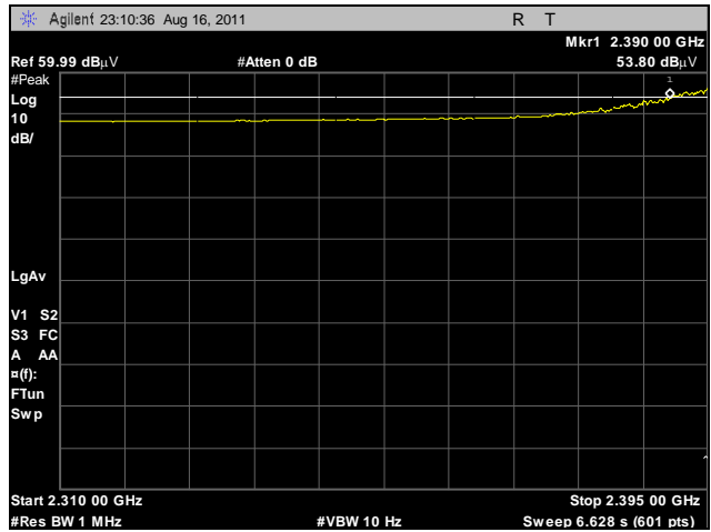
Plot 379. Radiated Restricted Band Edge, Low Channel, 2.4 GHz, 802.11g HT40, Average, Omni
