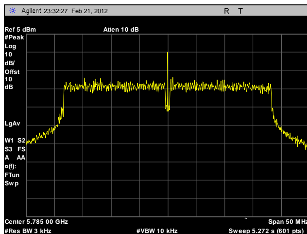
Plot 648. Peak Power Spectral Density, Mid Channel, 5.8 GHz, 802.11n 40 MHz, Port B, Sector Antenna, Determination
