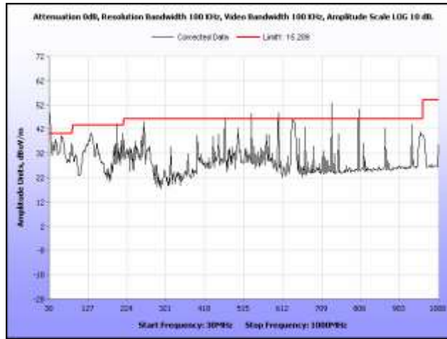
Plot 325. Radiated Spurs, High Channel, 5.8 GHz, 802.11a, 30 MHz – 1 GHz, Sector Note: Emissions which exceed the limit are digital emissions.
