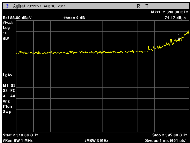
Plot 380. Radiated Restricted Band Edge, Low Channel, 2.4 GHz, 802.11g HT40, Peak, Omni
