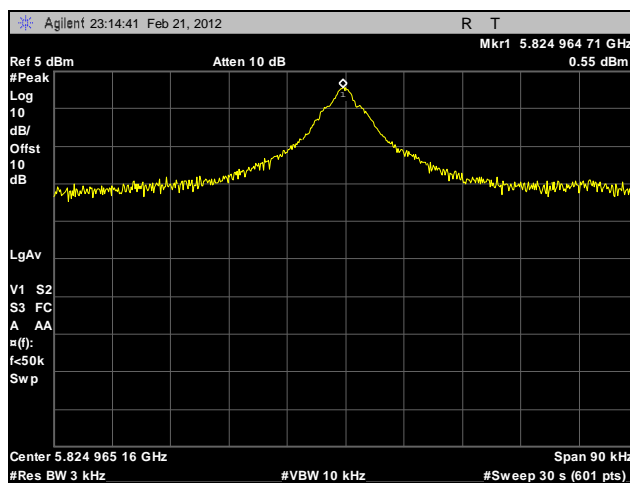
Plot 633. Peak Power Spectral Density, High Channel, 5.8 GHz, 802.11n 20 MHz, Port A, Sector Antenna
