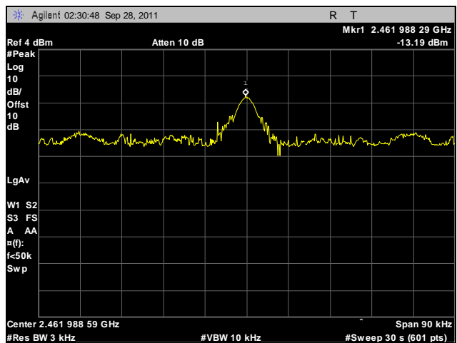
Plot 525. Peak Power Spectral Density, High Channel, 2.4 GHz, 802.11b, Port A
