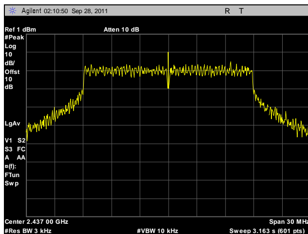
Plot 534. Peak Power Spectral Density, Mid Channel, 2.4 GHz, 802.11g HT20, Port A, Determination
