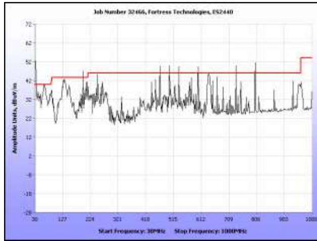
Plot 349. Radiated Spurs, Low Channel, 5.8 GHz, 802.11n 40 MHz, 30 MHz – 1 GHz, Sector Note: Emissions which exceed the limit are digital emissions.
