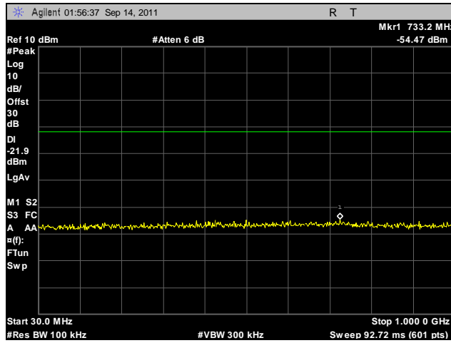
Plot 468. Conducted Spurious Emissions, Mid Channel, 5.8 GHz, 802.11n 20 MHz, Port A, 30 MHz – 1 GHz
