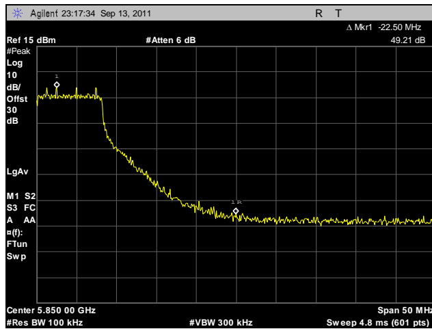
Plot 511. Conducted Band Edge, High, Channel, 5.8 GHz, 802.11a, Port A
