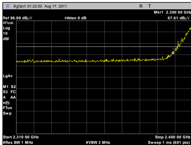
Plot 388. Radiated Restricted Band Edge, Low Channel, 2.4 GHz, 802.11g, Peak, Sector
