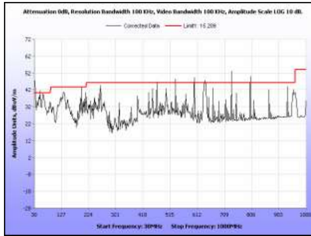
Plot 313. Radiated Spurs, Low Channel, 5.8 GHz, 802.11a, 30 MHz – 1 GHz, Sector Note: Emissions which exceed the limit are digital emissions.
