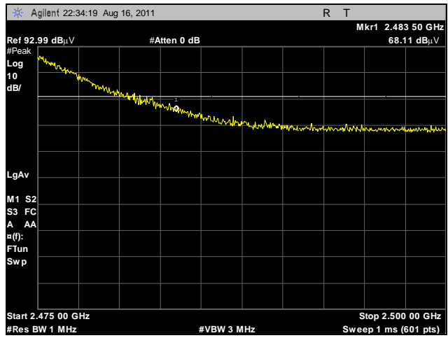
Plot 374. Radiated Restricted Band Edge, High Channel, 2.4 GHz, 802.11g, Peak, Omni
