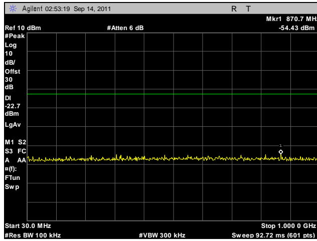
Plot 444. Conducted Spurious Emissions, Mid Channel, 2.4 GHz, 802.11g HT40, Port B, 30 MHz – 1 GHz
