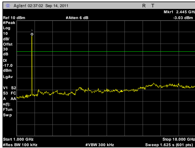
Plot 424. Conducted Spurious Emissions, Mid Channel, 2.4 GHz, 802.11g HT20, Port A, 1 GHz – 18 GHz
