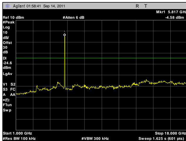
Plot 475. Conducted Spurious Emissions, High Channel, 5.8 GHz, 802.11n 20 MHz, Port A, 1 GHz – 18 GHz
