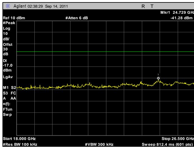
Plot 425. Conducted Spurious Emissions, Mid Channel, 2.4 GHz, 802.11g HT20, Port A, 18 GHz – 26.5 GHz
