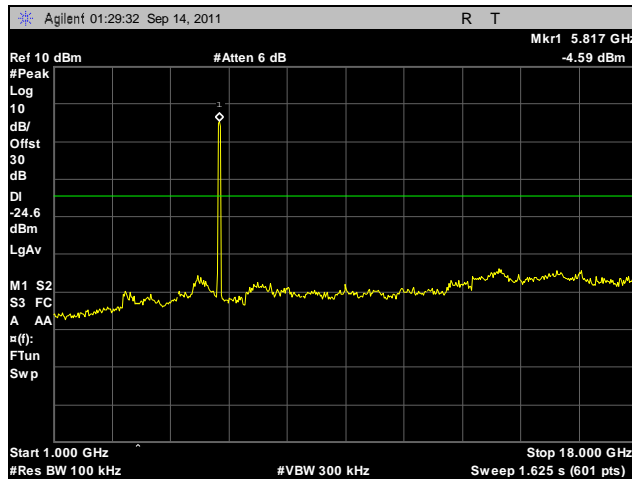
Plot 493. Conducted Spurious Emissions, High Channel, 5.8 GHz, 802.11n 40 MHz, Port A, 1 GHz – 18 GHz
