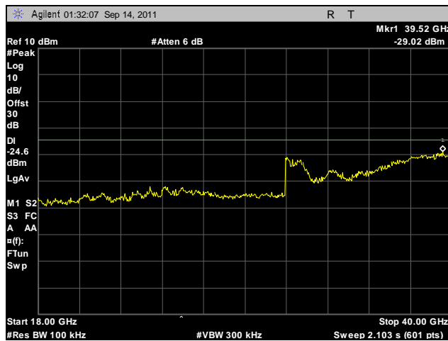
Plot 494. Conducted Spurious Emissions, High Channel, 5.8 GHz, 802.11n 40 MHz, Port A, 18 GHz – 40 GHz
