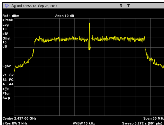
Plot 552. Peak Power Spectral Density, Mid Channel, 2.4 GHz, 802.11g HT40, Port B, Determination
