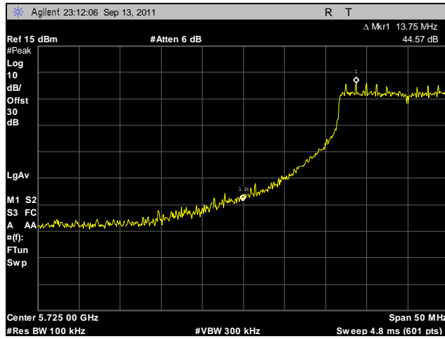
Plot 510. Conducted Band Edge, Low Channel, 5.8 GHz, 802.11a, Port A
