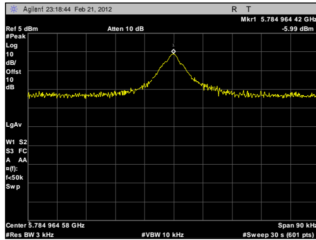
Plot 637. Peak Power Spectral Density, Mid Channel, 5.8 GHz, 802.11n 20 MHz, Port B, Sector Antenna
