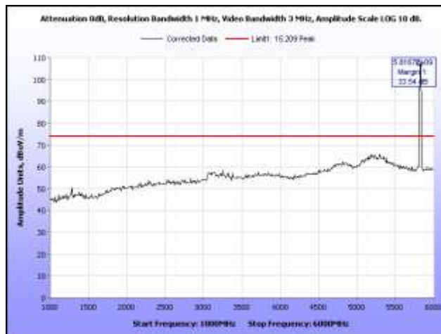
Plot 345. Radiated Spurs, High Channel, 5.8 GHz, 802.11n 20 MHz, 1 GHz – 6 GHz, Peak, Sector
