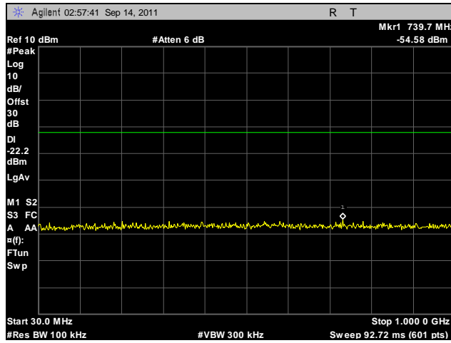
Plot 432. Conducted Spurious Emissions, High Channel, 2.4 GHz, 802.11g HT20, Port B, 30 MHz – 1 GHz
