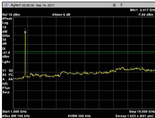
Plot 439. Conducted Spurious Emissions, Low Channel, 2.4 GHz, 802.11g HT40, Port B, 1 GHz – 18 GHz
