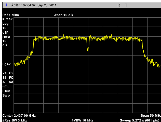
Plot 546. Peak Power Spectral Density, Mid Channel, 2.4 GHz, 802.11g HT40, Port A, Determination
