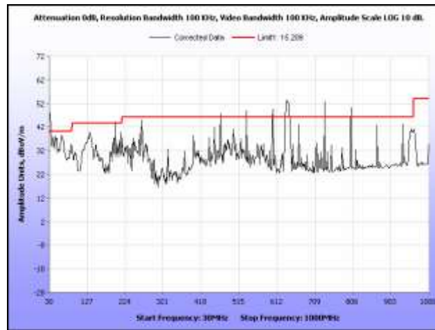
Plot 331. Radiated Spurs, Low Channel, 5.8 GHz, 802.11n 20 MHz, 30 MHz – 1 GHz, Sector Note: Emissions which exceed the limit are digital emissions.
