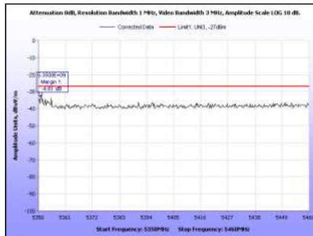
Plot 53. Radiated Spurious Emissions, 5320 MHz, HT20, 5.35 GHz – 5.46 GHz
