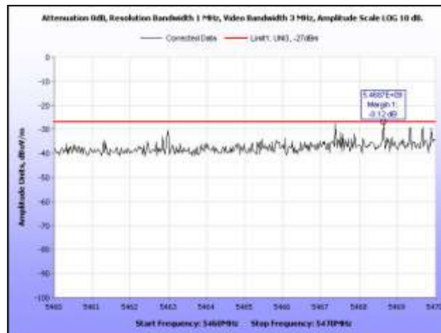
Plot 65. Radiated Spurious Emissions, 5500 MHz, HT20, 5.46 GHz – 5.47 GHz
