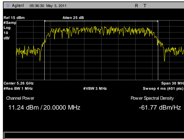
Plot 15. RF Power Output, 5260 MHz, HT20
