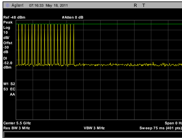
Plot 100. Radar Type 1 Calibration, 5500 MHz
