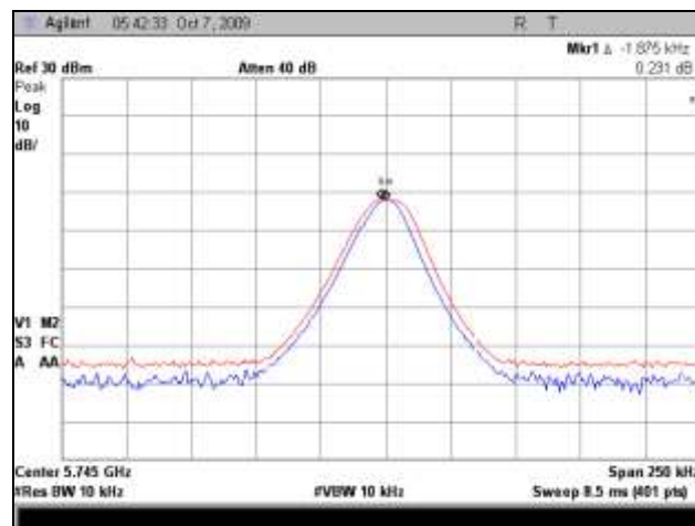
Plot 95. Frequency Stability, Battery Drain Test
