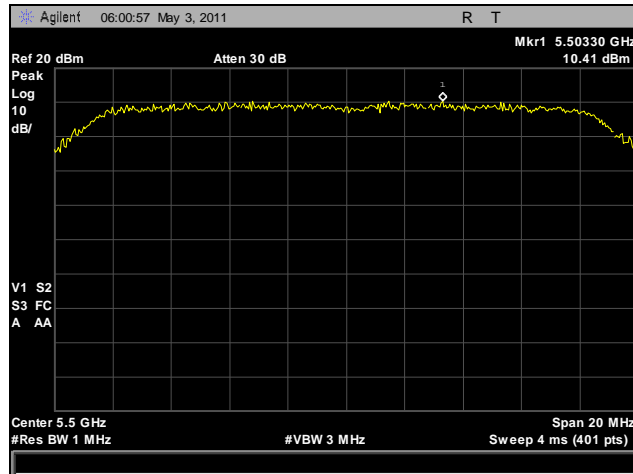
Plot 24. Power Spectral Density, 5500 MHz, HT20
