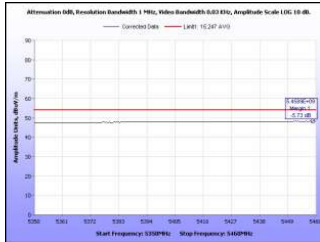
Plot 45. Radiated Spurious Emissions, 5300 MHz, HT20, 5.35 GHz – 5.46 GHz, Average
