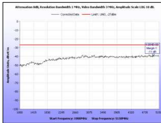
Plot 52. Radiated Spurious Emissions, 5320 MHz, HT20, 1 GHz – 5.15 GHz
