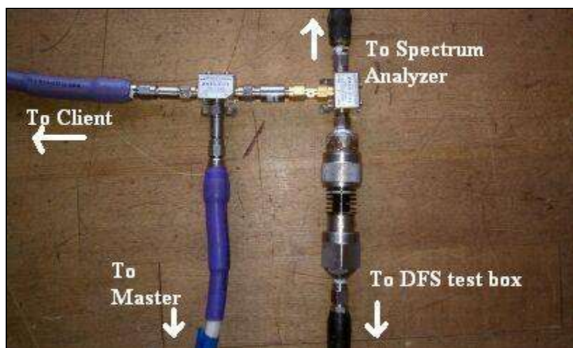
Photograph 5. DFS Cable Setup
