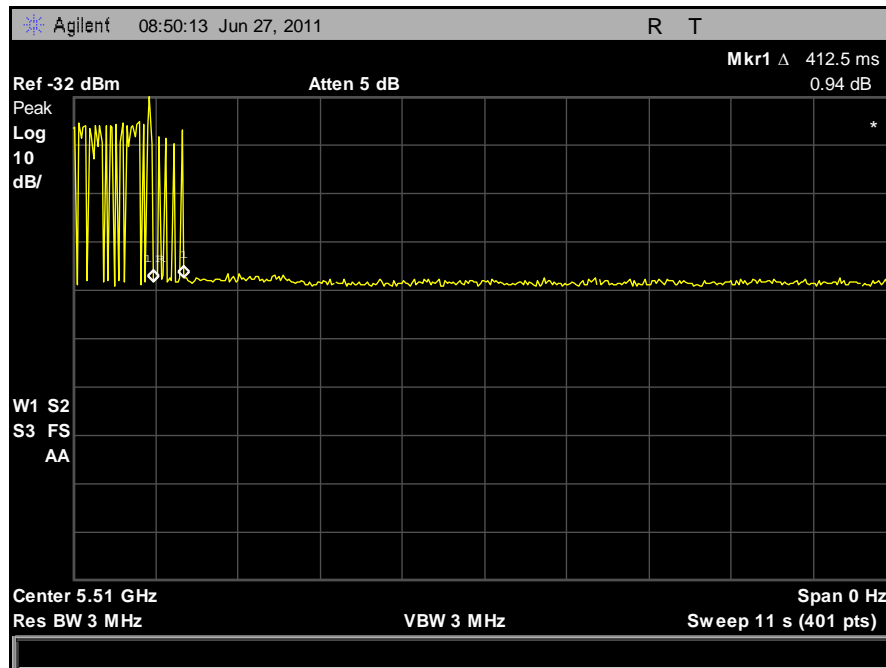
Plot 109. Channel Move Time
