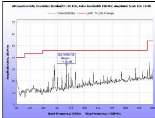
Plot 33. Radiated Spurious Emissions, 5260 MHz, HT20, 30 MHz – 1 GHz
