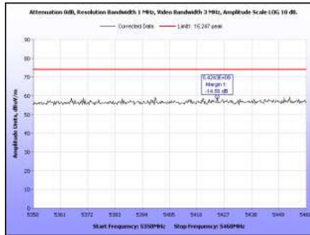
Plot 37. Radiated Spurious Emissions, 5260 MHz, HT20, 5.35 GHz – 5.46 GHz, Peak
