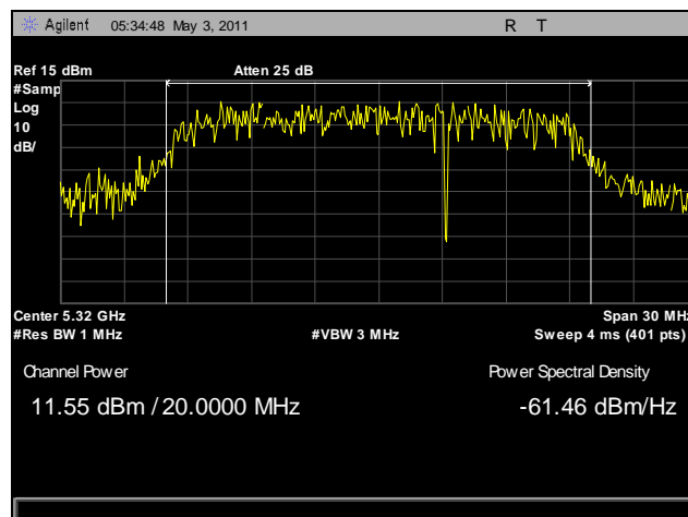
Plot 17. RF Power Output, 5320 MHz, HT20
