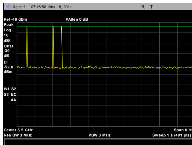
Plot 105. Radar Type 6 Calibration, 5500 MHz
