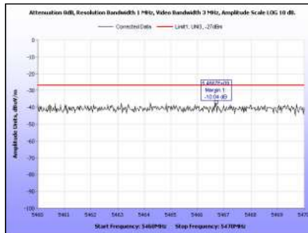
Plot 56. Radiated Spurious Emissions, 5320 MHz, HT20, 5.46 GHz – 5.47 GHz
