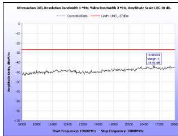
Plot 85. Radiated Spurious Emissions, 5700 MHz, HT20, 10 GHz – 18 GHz
