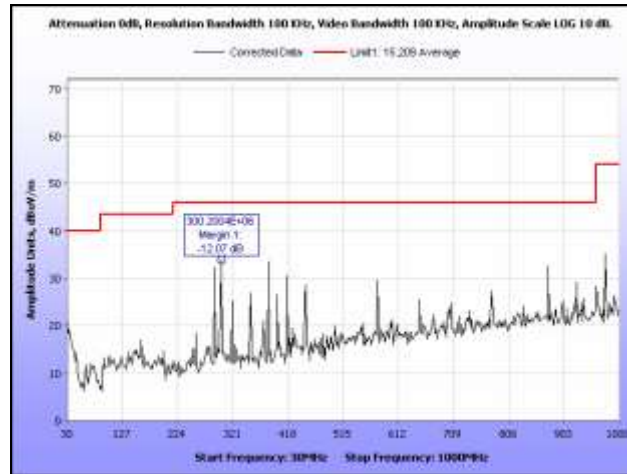
Plot 42. Radiated Spurious Emissions, 5300 MHz, HT20, 30 MHz – 1 GHz
