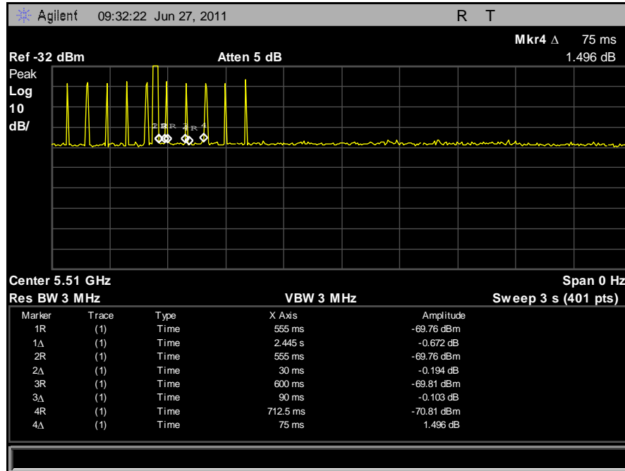
Plot 110. Channel Closing Transmission Time, 1
