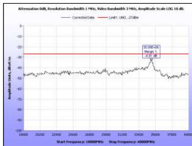
Plot 59. Radiated Spurious Emissions, 5320 MHz, HT20, 18 GHz – 40 GHz
