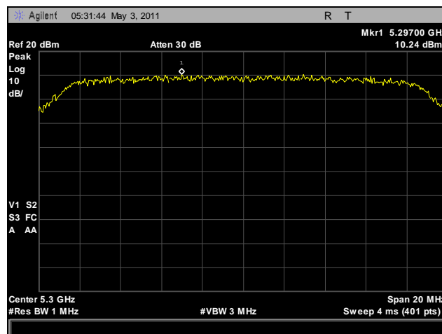
Plot 22. Power Spectral Density, 5300 MHz, HT20
