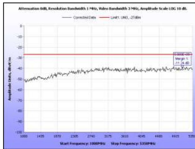
Plot 70. Radiated Spurious Emissions, 5580 MHz, HT20, 1 GHz – 5.35 GHz
