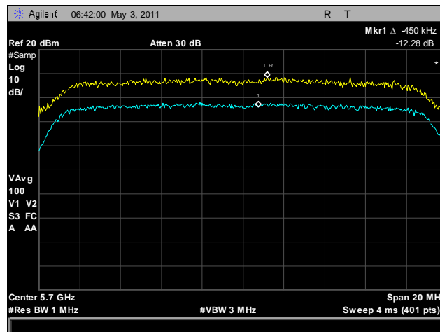
Plot 32. Peak Excursion Ratio, 5700 MHz, HT20
