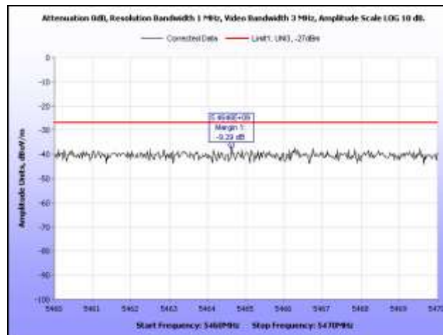
Plot 74. Radiated Spurious Emissions, 5580 MHz, HT20, 5.46 GHz – 5.47 GHz
