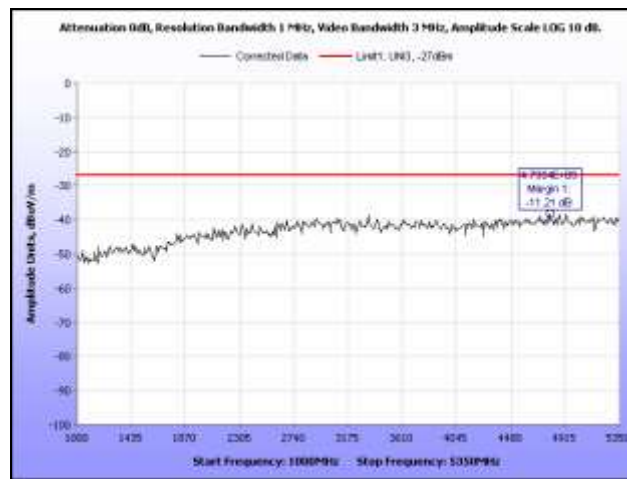
Plot 61. Radiated Spurious Emissions, 5500 MHz, HT20, 1 GHz – 5.35 GHz
