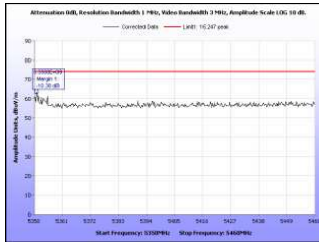
Plot 55. Radiated Spurious Emissions, 5320 MHz, HT20, 5.35 GHz – 5.46 GHz, Peak
