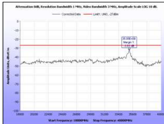
Plot 50. Radiated Spurious Emissions, 5300 MHz, HT20, 18 GHz – 40 GHz
