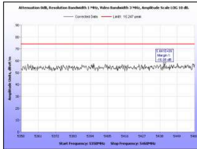
Plot 64. Radiated Spurious Emissions, 5500 MHz, HT20, 5.35 GHz – 5.46 GHz, Peak
