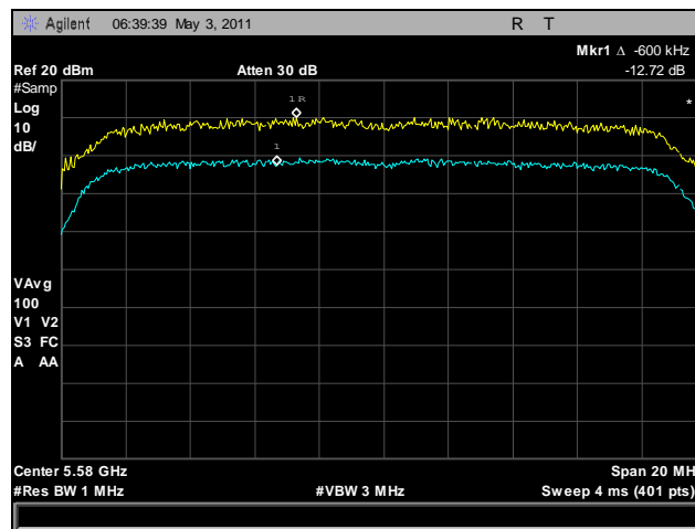
Plot 31. Peak Excursion Ratio, 5580 MHz, HT20
