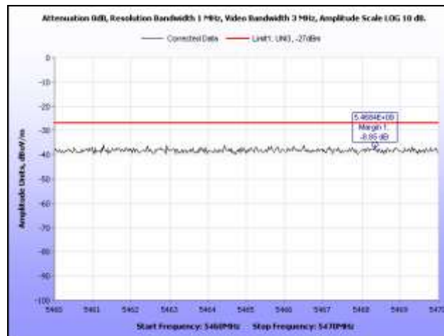
Plot 47. Radiated Spurious Emissions, 5300 MHz, HT20, 5.46 GHz – 5.47 GHz
