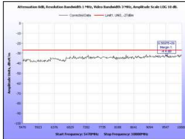
Plot 57. Radiated Spurious Emissions, 5320 MHz, HT20, 5.47 GHz – 10 GHz
