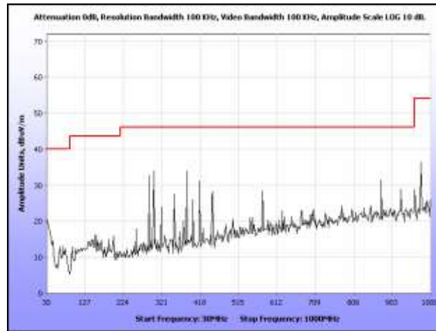
Plot 96. Receiver Spurious Emission, 5300 MHz, HT20, 30 MHz – 1 GHz
