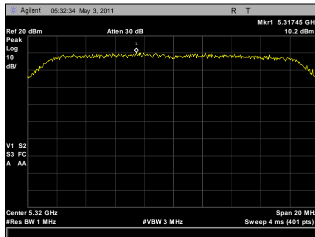
Plot 23. Power Spectral Density, 5320 MHz, HT20
