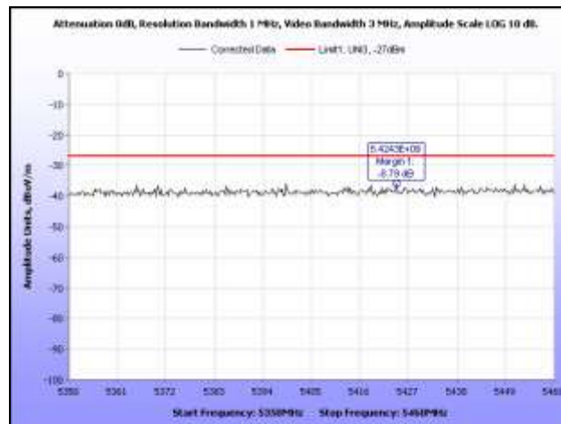
Plot 35. Radiated Spurious Emissions, 5260 MHz, HT20, 5.35 GHz – 5.46 GHz
