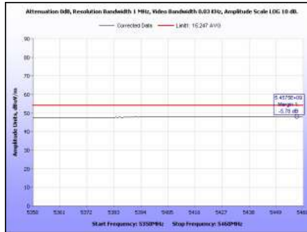
Plot 36. Radiated Spurious Emissions, 5260 MHz, HT20, 5.35 GHz – 5.46 GHz, Average
