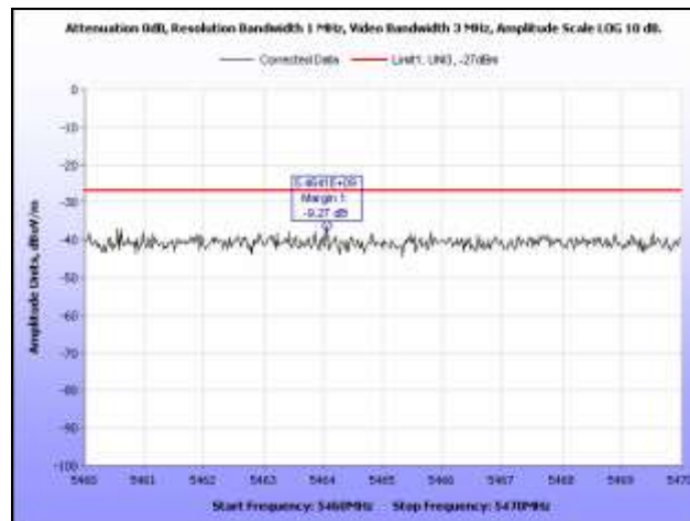
Plot 38. Radiated Spurious Emissions, 5260 MHz, HT20, 5.46 GHz – 5.47 GHz
