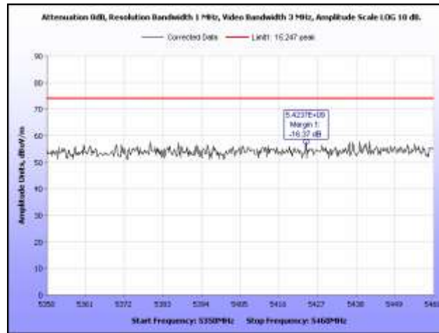
Plot 46. Radiated Spurious Emissions, 5300 MHz, HT20, 5.35 GHz – 5.46 GHz, Peak
