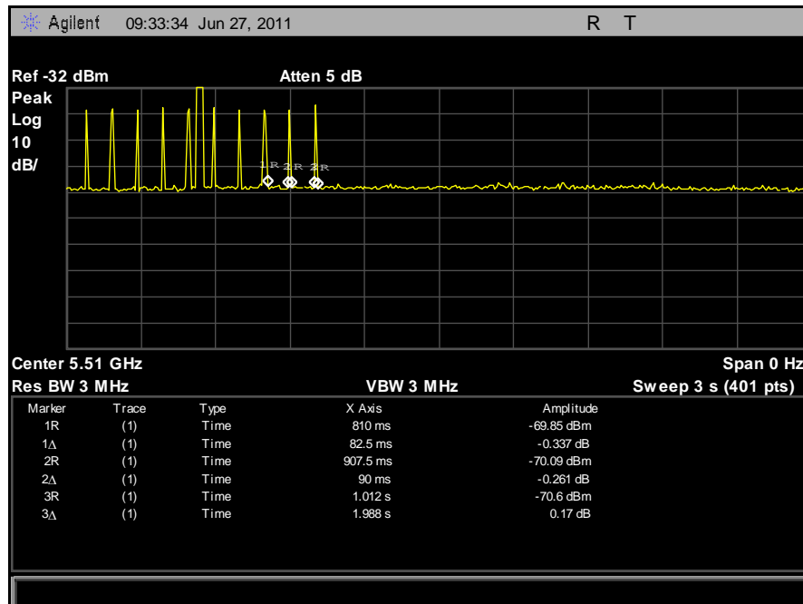
Plot 111. Channel Closing Transmission Time, 2
