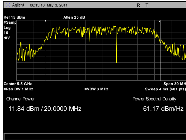
Plot 18. RF Power Output, 5500 MHz, HT20
