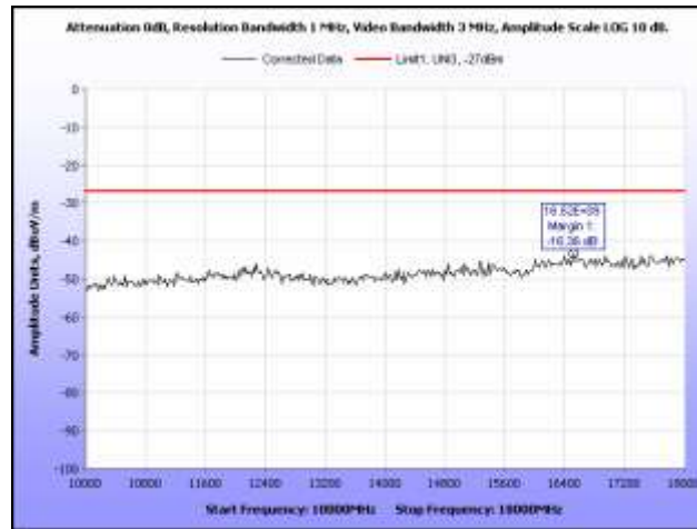
Plot 40. Radiated Spurious Emissions, 5260 MHz, HT20, 10 GHz – 18 GHz
