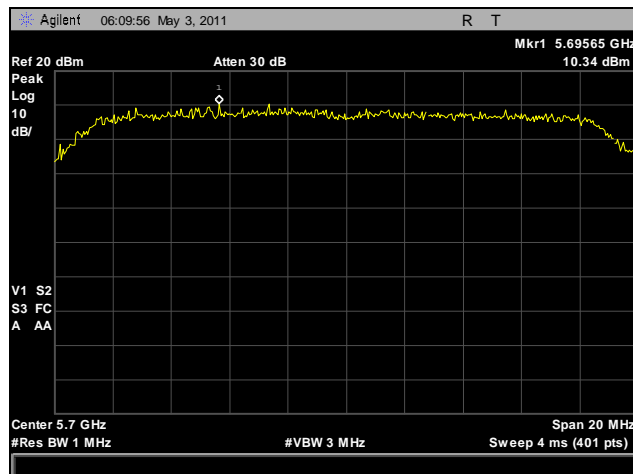
Plot 26. Power Spectral Density, 5700 MHz, HT20
