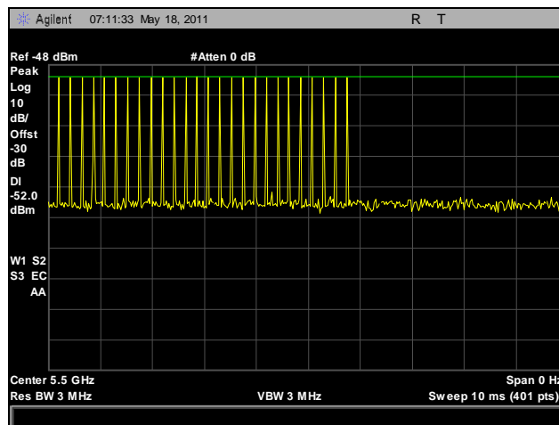
Plot 101. Radar Type 2 Calibration, 5500 MHz
