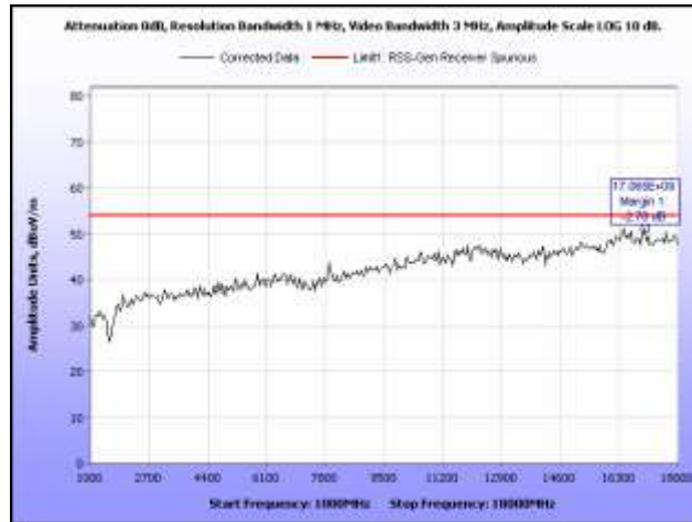
Plot 99. Receiver Spurious Emission, 5580 MHz, HT20, 1 GHz – 18 GHz
