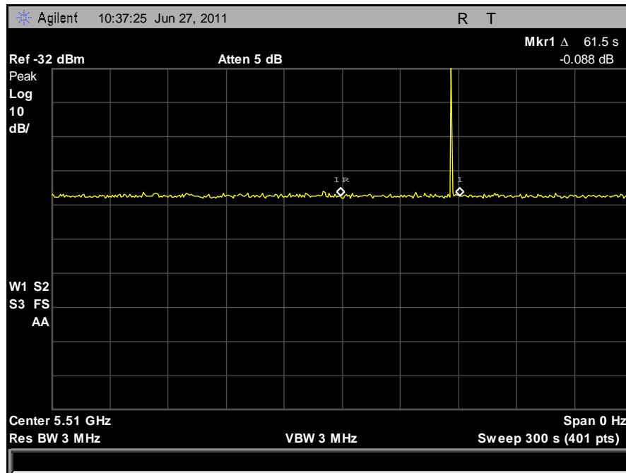
Plot 108. Radar Burst at the End of CACT
