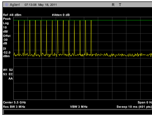
Plot 103. Radar Type 4 Calibration, 5500 MHz
