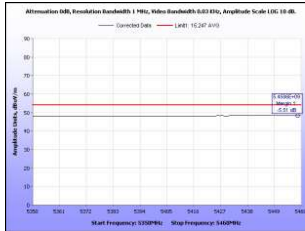
Plot 72. Radiated Spurious Emissions, 5580 MHz, HT20, 5.35 GHz – 5.46 GHz, Average
