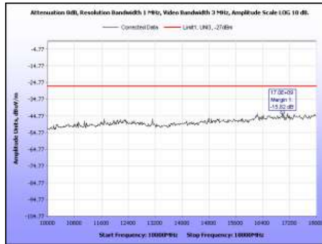
Plot 76. Radiated Spurious Emissions, 5580 MHz, HT20, 10 GHz – 18 GHz
