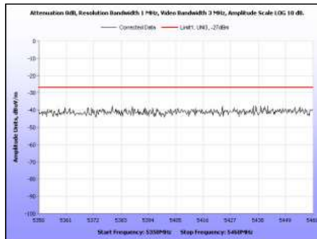
Plot 44. Radiated Spurious Emissions, 5300 MHz, HT20, 5.35 GHz – 5.46 GHz
