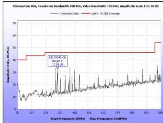
Plot 51. Radiated Spurious Emissions, 5320 MHz, HT20, 30 MHz – 1 GHz
