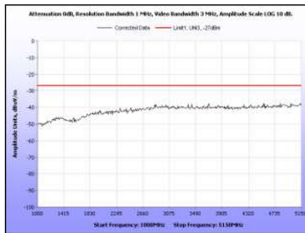
Plot 34. Radiated Spurious Emissions, 5260 MHz, HT20, 1 GHz – 5.15 GHz
