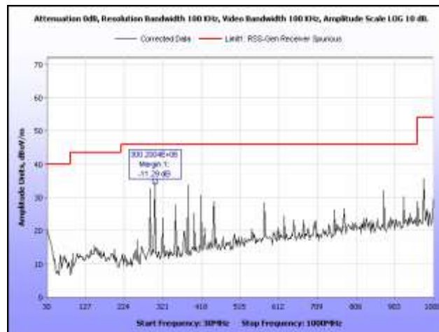
Plot 98. Receiver Spurious Emission, 5580 MHz, HT20, 30 MHz – 1 GHz
