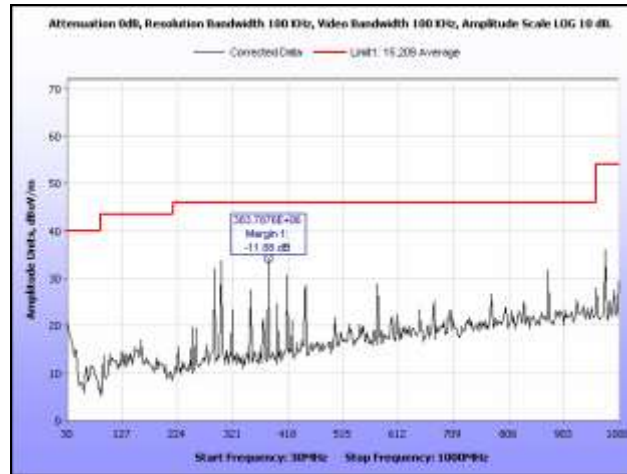
Plot 60. Radiated Spurious Emissions, 5500 MHz, HT20, 30 MHz – 1 GHz
