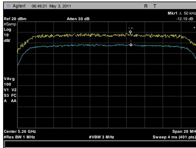
Plot 27. Peak Excursion Ratio, 5260 MHz, HT20
