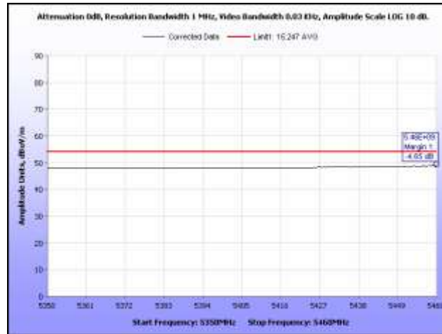
Plot 63. Radiated Spurious Emissions, 5500 MHz, HT20, 5.35 GHz – 5.46 GHz, Average
