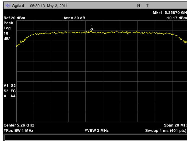
Plot 21. Power Spectral Density, 5260 MHz, HT20
