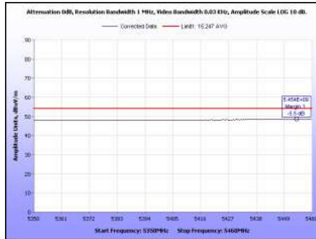
Plot 81. Radiated Spurious Emissions, 5700 MHz, HT20, 5.35 GHz – 5.46 GHz, Average
