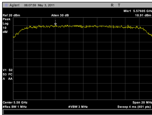
Plot 25. Power Spectral Density, 5580 MHz, HT20
