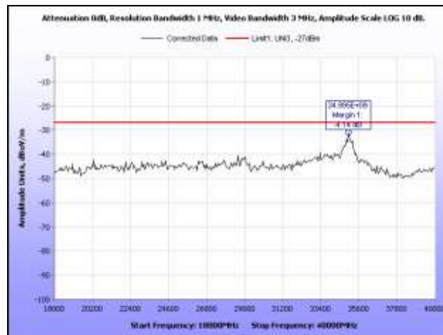
Plot 86. Radiated Spurious Emissions, 5700 MHz, HT20, 18 GHz – 40 GHz
