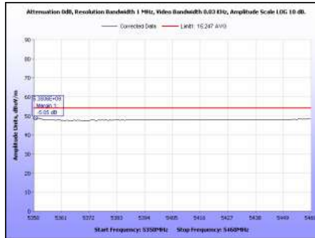
Plot 54. Radiated Spurious Emissions, 5320 MHz, HT20, 5.35 GHz – 5.46 GHz, Average
