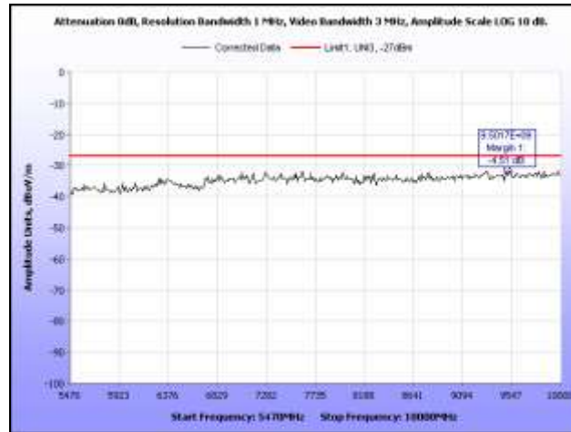
Plot 39. Radiated Spurious Emissions, 5260 MHz, HT20, 5.47 GHz – 10 GHz
