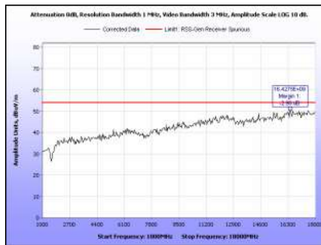
Plot 97. Receiver Spurious Emission, 5300 MHz, HT20, 1 GHz – 18 GHz
