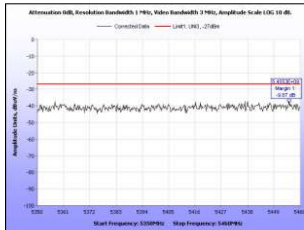
Plot 71. Radiated Spurious Emissions, 5580 MHz, HT20, 5.35 GHz – 5.46 GHz
