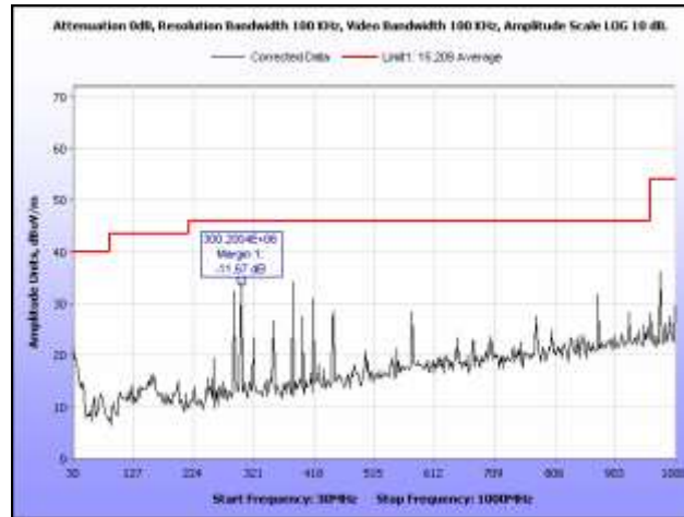
Plot 69. Radiated Spurious Emissions, 5580 MHz, HT20, 30 MHz – 1 GHz
