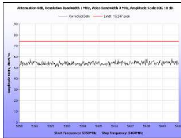
Plot 73. Radiated Spurious Emissions, 5580 MHz, HT20, 5.35 GHz – 5.46 GHz, Peak
