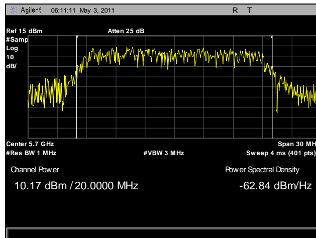
Plot 20. RF Power Output, 5700 MHz, HT20
