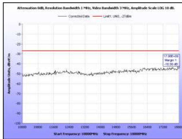
Plot 58. Radiated Spurious Emissions, 5320 MHz, HT20, 10 GHz – 18 GHz
