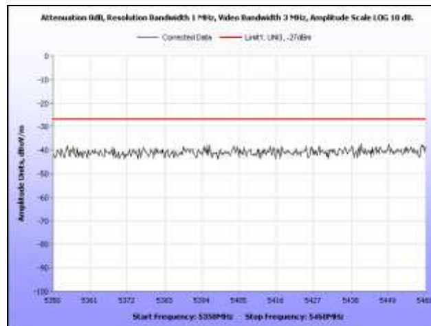
Plot 62. Radiated Spurious Emissions, 5500 MHz, HT20, 5.35 GHz – 5.46 GHz
