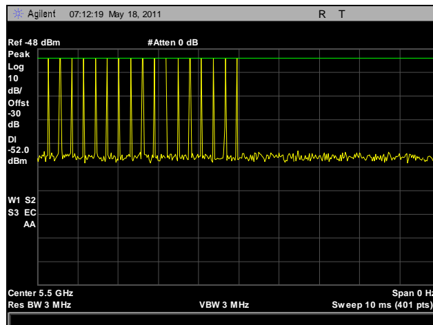
Plot 102. Radar Type 3 Calibration, 5500 MHz
