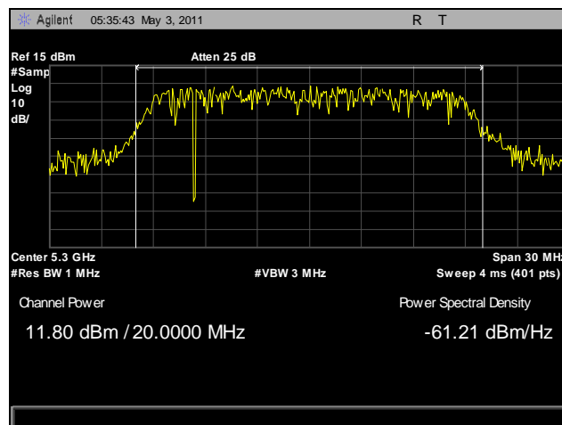
Plot 16. RF Power Output, 5300 MHz, HT20
