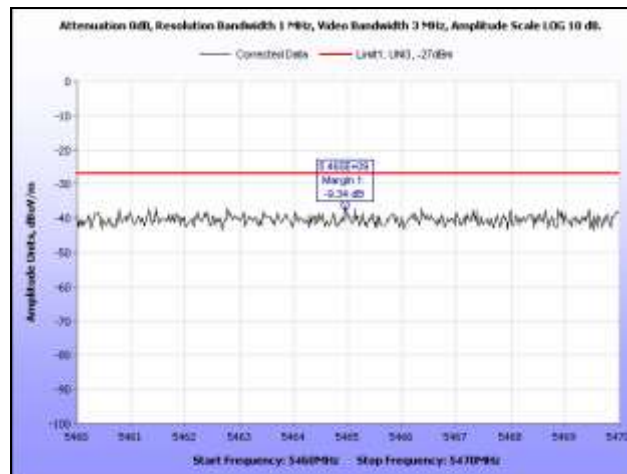
Plot 83. Radiated Spurious Emissions, 5700 MHz, HT20, 5.46 GHz – 5.47 GHz
