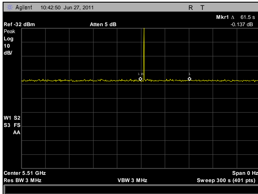
Plot 107. Radar Burst at the Beginning of CACT
