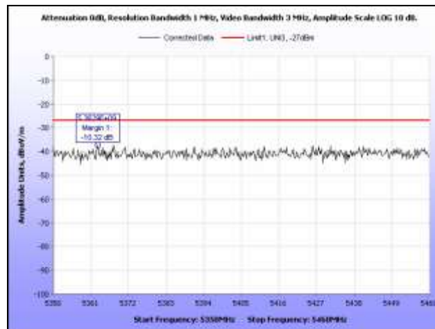
Plot 80. Radiated Spurious Emissions, 5700 MHz, HT20, 5.35 GHz – 5.46 GHz
