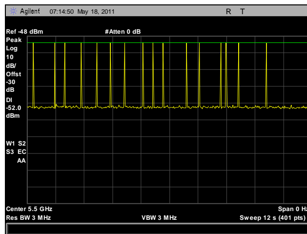
Plot 104. Radar Type 5 Calibration, 5500 MHz
