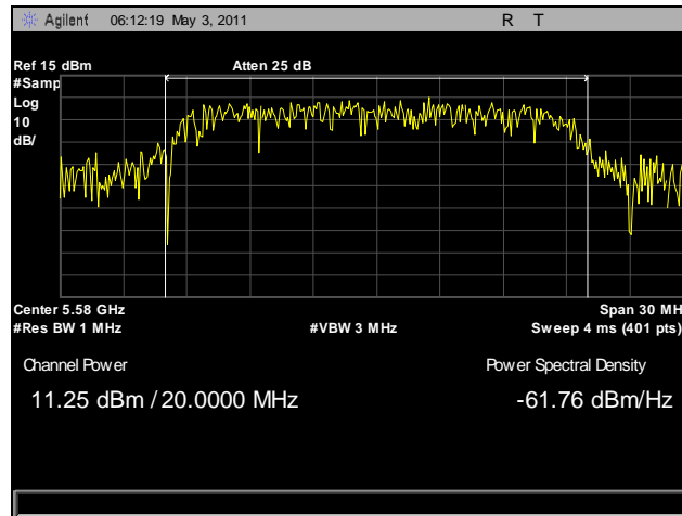
Plot 19. RF Power Output, 5580 MHz, HT20
