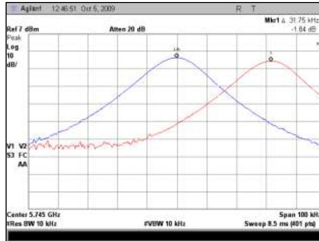
Plot 93. Frequency Stability, 50°C
