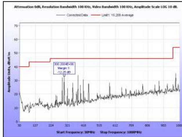
Plot 78. Radiated Spurious Emissions, 5700 MHz, HT20, 30 MHz – 1 GHz
