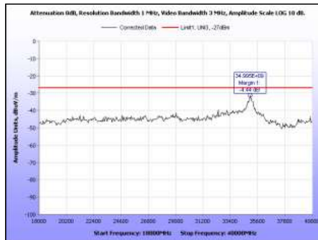
Plot 77. Radiated Spurious Emissions, 5580 MHz, HT20, 18 GHz – 40 GHz
