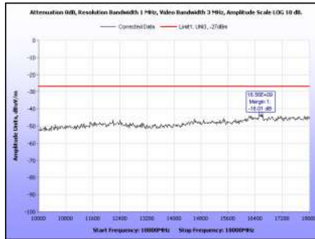
Plot 67. Radiated Spurious Emissions, 5500 MHz, HT20, 10 GHz – 18 GHz
