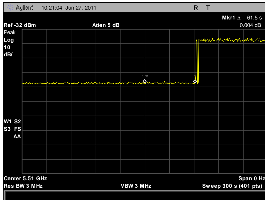
Plot 106. Initial Channel Availability Check Time
