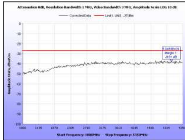
Plot 79. Radiated Spurious Emissions, 5700 MHz, HT20, 1 GHz – 5.35 GHz
