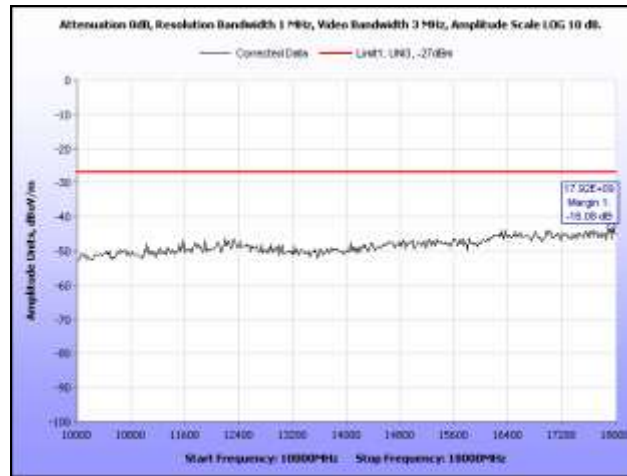
Plot 49. Radiated Spurious Emissions, 5300 MHz, HT20, 10 GHz – 18 GHz
