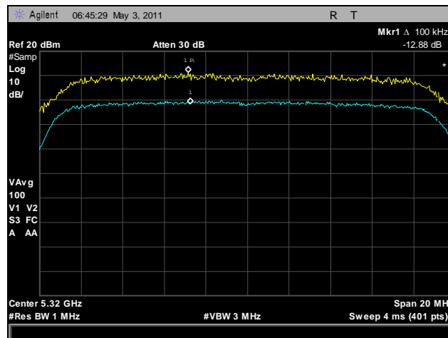
Plot 29. Peak Excursion Ratio, 5320 MHz, HT20
