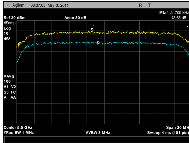
Plot 30. Peak Excursion Ratio, 5500 MHz, HT20
