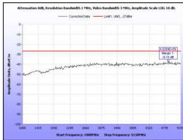
Plot 43. Radiated Spurious Emissions, 5300 MHz, HT20, 1 GHz – 5.15 GHz
