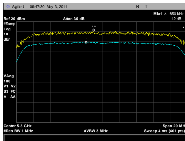
Plot 28. Peak Excursion Ratio, 5300 MHz, HT20
