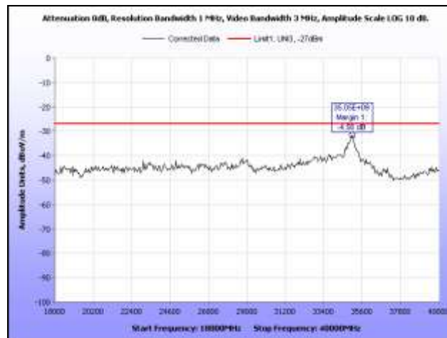
Plot 68. Radiated Spurious Emissions, 5580 MHz, HT20, 18 GHz – 40 GHz
