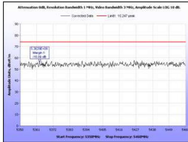
Plot 82. Radiated Spurious Emissions, 5700 MHz, HT20, 5.35 GHz – 5.46 GHz, Peak
