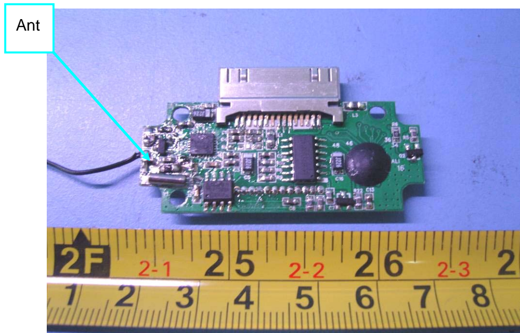
PCB - Front View
