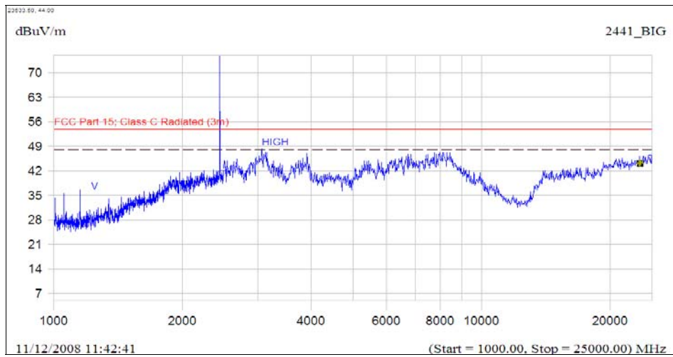
(Plot B.5 Antenna Vertical, 1GHz to 25GHz)
