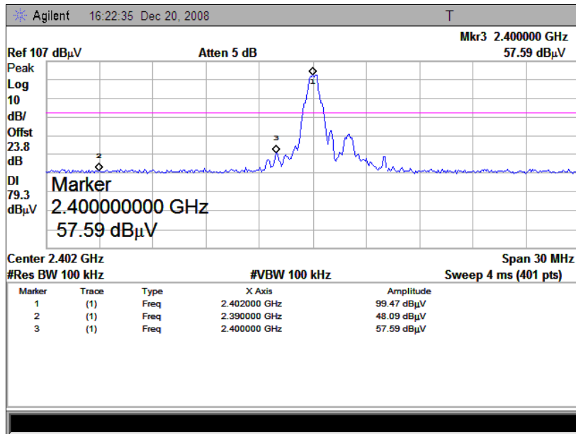
(Plot A1: Channel = 0 2402MHz)
