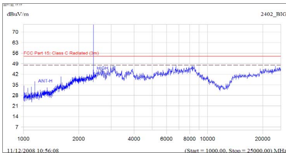
(Plot A.3: Antenna Horizontal, 1GHz to 25GHz)
