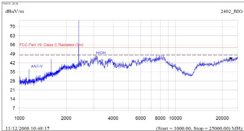
(Plot A.5: Antenna Vertical, 1GHz to 25GHz)
