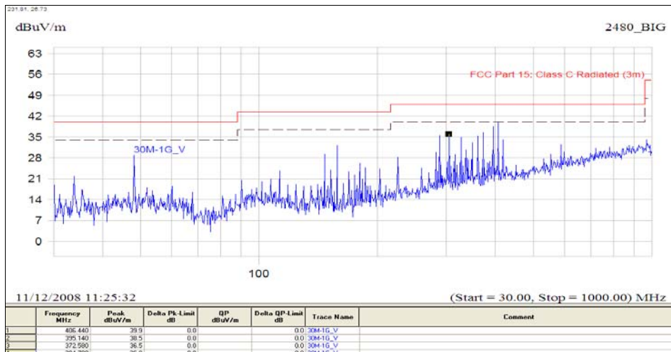
(Plot C.4: Antenna Vertical, 30MHz to 1GHz)
