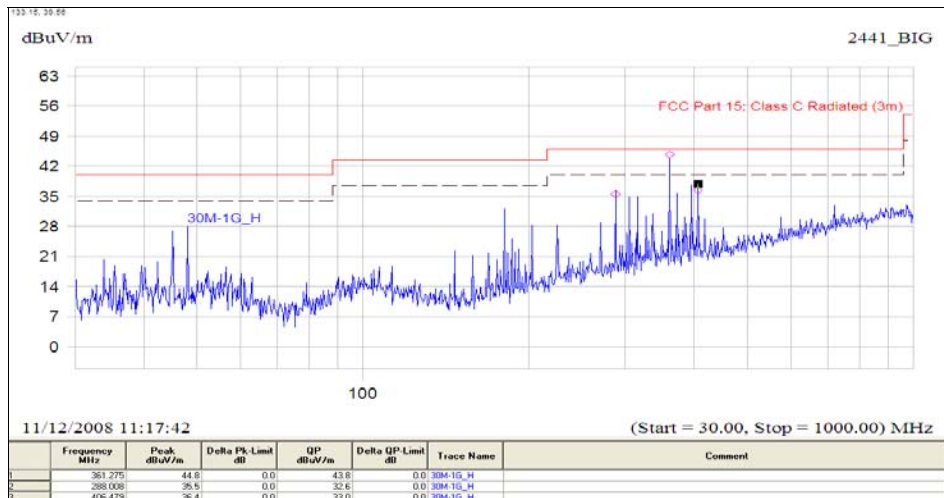
(Plot B.2: Antenna Horizontal, 30MHz to 1GHz)
