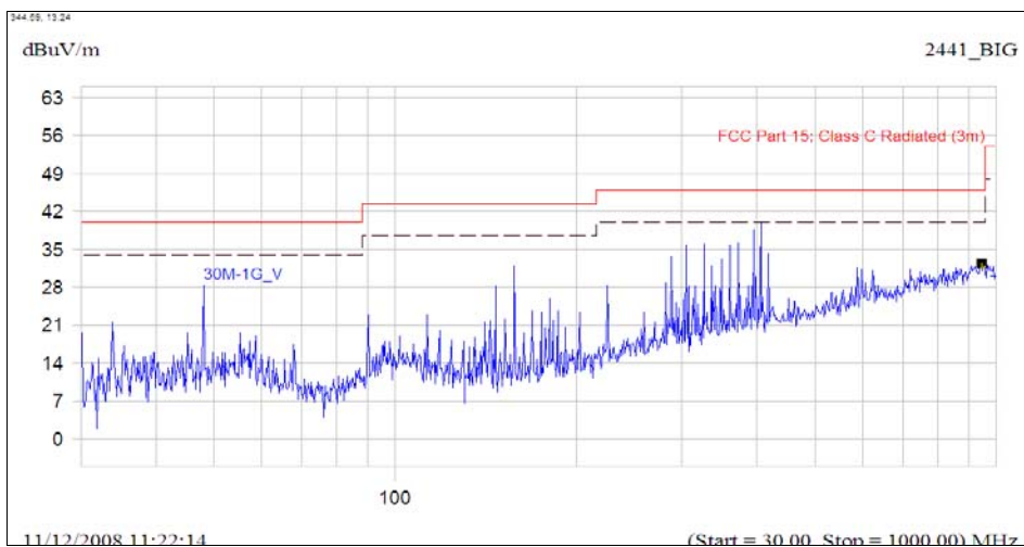
(Plot B.4: Antenna Vertical, 30MHz to 1GHz)
