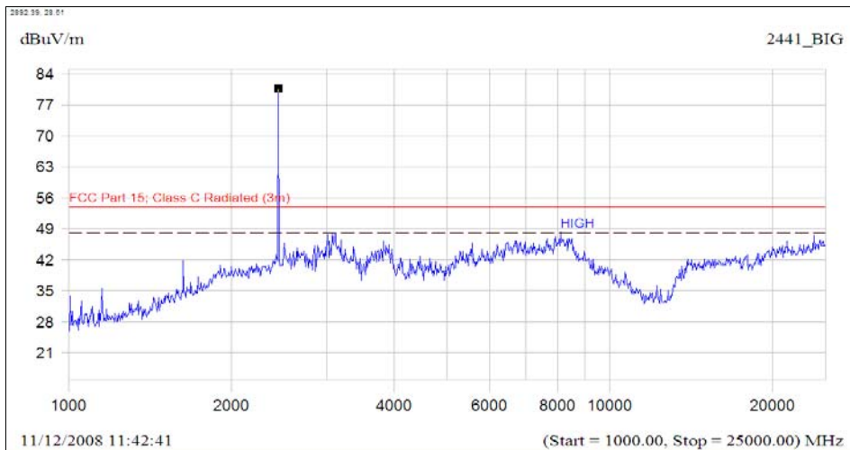
(Plot B.3: Antenna Horizontal, 1GHz to 25GHz)
