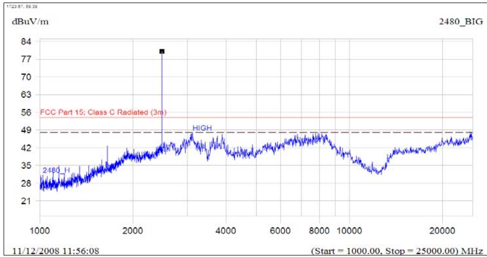
(Plot C.3: Antenna Horizontal, 1GHz to 25GHz)
