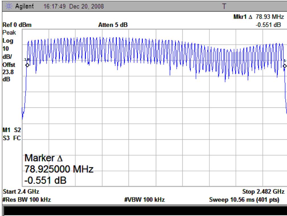
(Plot A.1: 2402MHz to 2480MHz)
