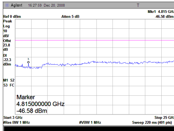
(Plot A.2: Channel = 0, 3GHz to 25GHz)
