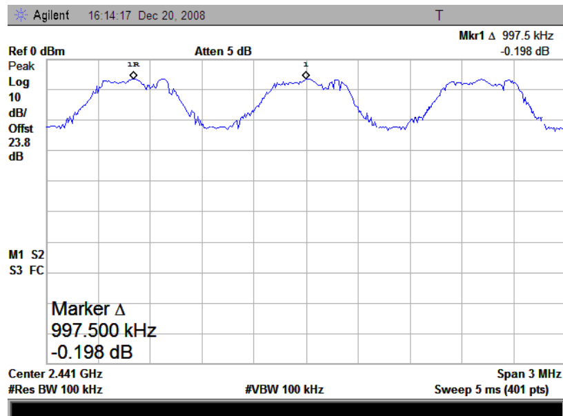
(Plot A: Carried Frequency Separation)
