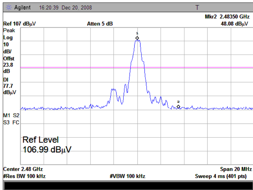
(Plot B1: Channel = 78 2480MHz)
