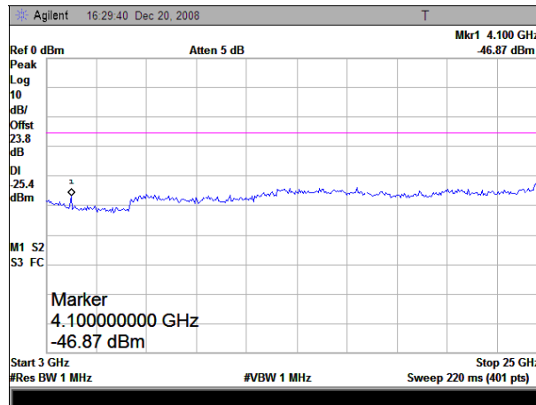
(Plot B.2: Channel = 39, 3GHz to 25GHz)
