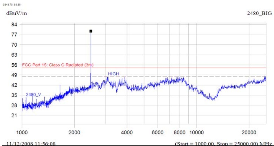
(Plot C.5 : Antenna Vertical, 1GHz to 25GHz)
