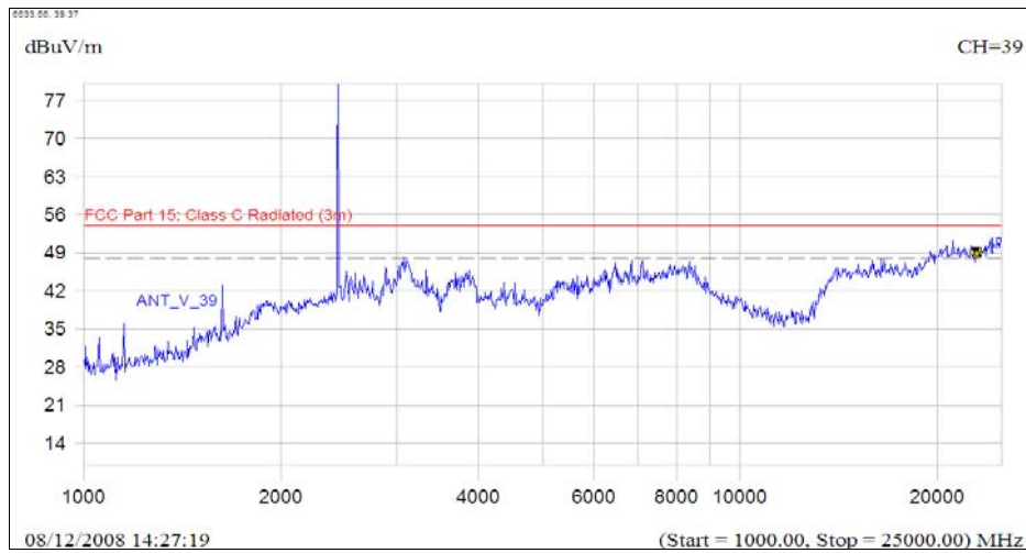
(Plot B.5 Antenna Vertical, 1GHz to 25GHz)
