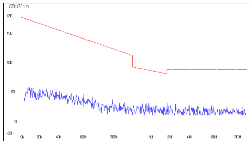
(Plot B.1: 9kHz to 30MHz)
