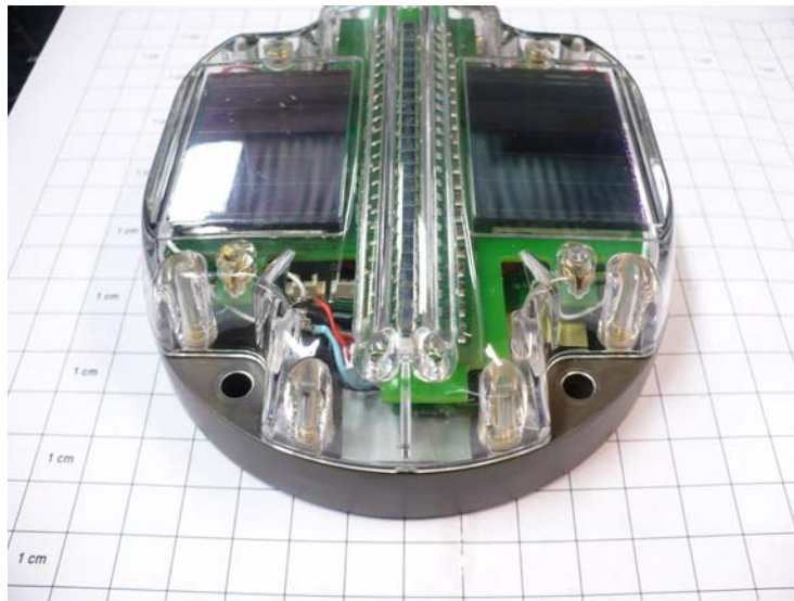
FRONT WIEV
