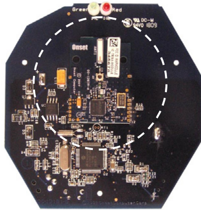
91-ZW-EM260 Soldered onto ZW PCB in location shown
