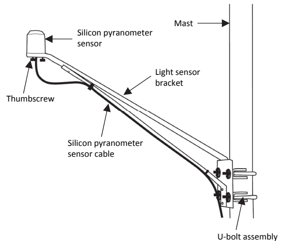
Silicon Pyranometer Sensor Bracket Mounting
