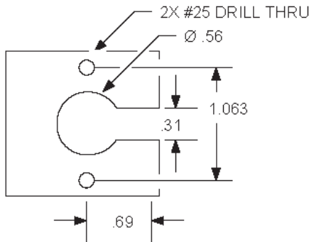
Recommended Mounting Plate Dimensions
