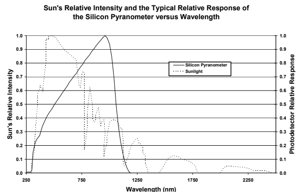
Plot A: Silicon Pyranometer Sensor Response Curve
