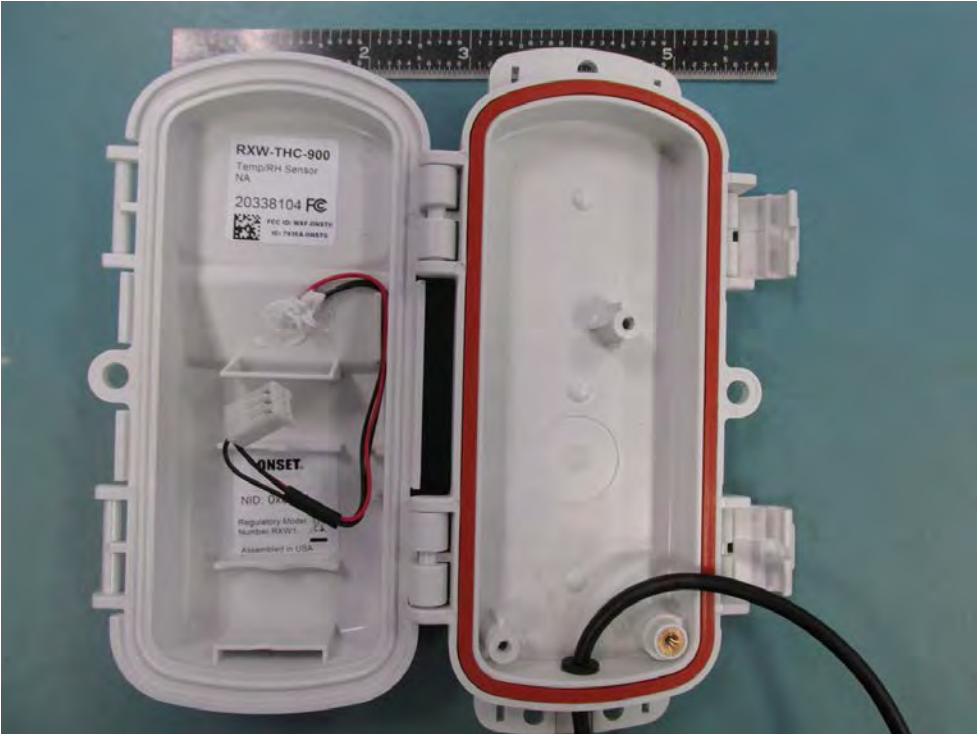
RXW-THC-900 Inner Housing
