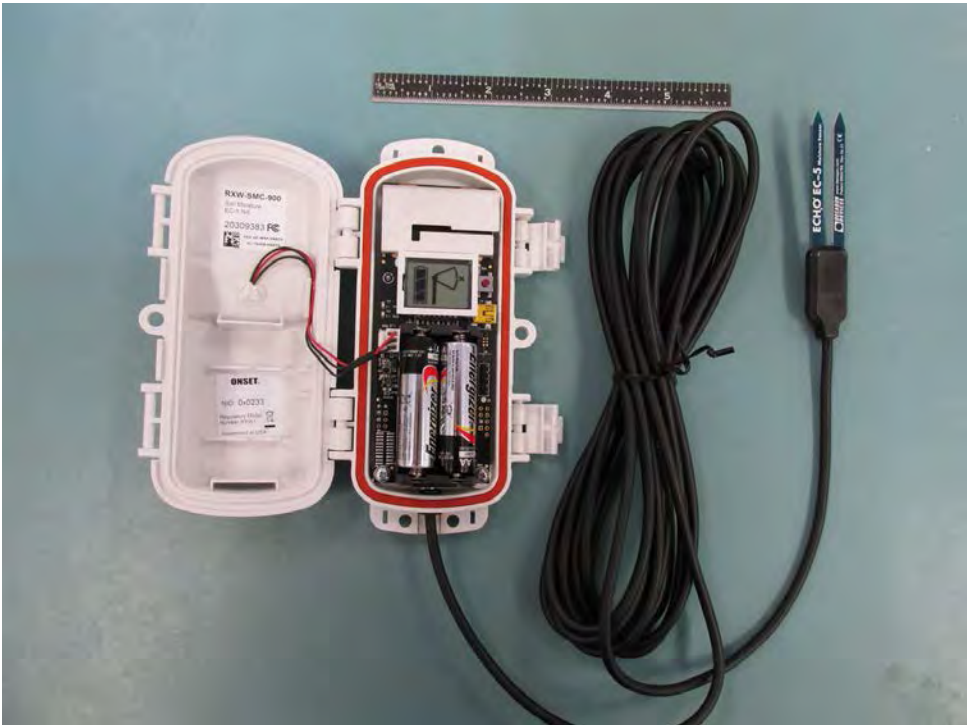
RXW-SMC-900 Product Case Open
