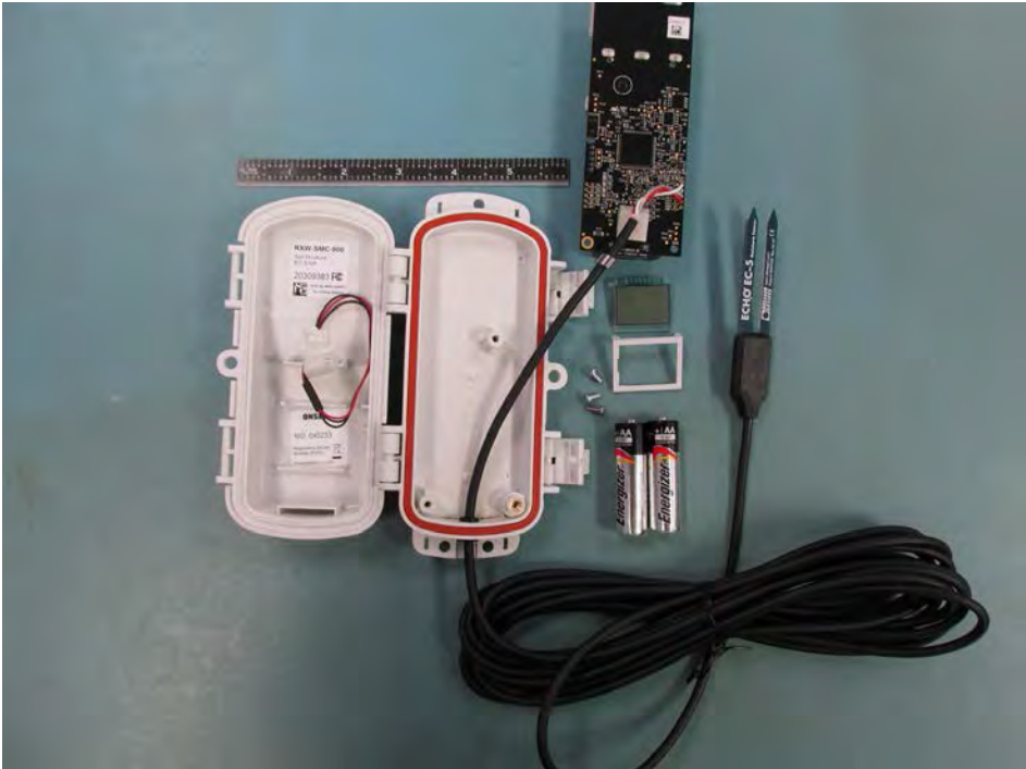
RXW-SMC-900 Exploded View with Sensor
