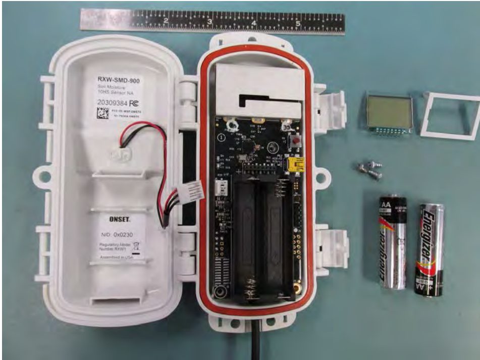
RXW-SMD-900 LCD Removed
