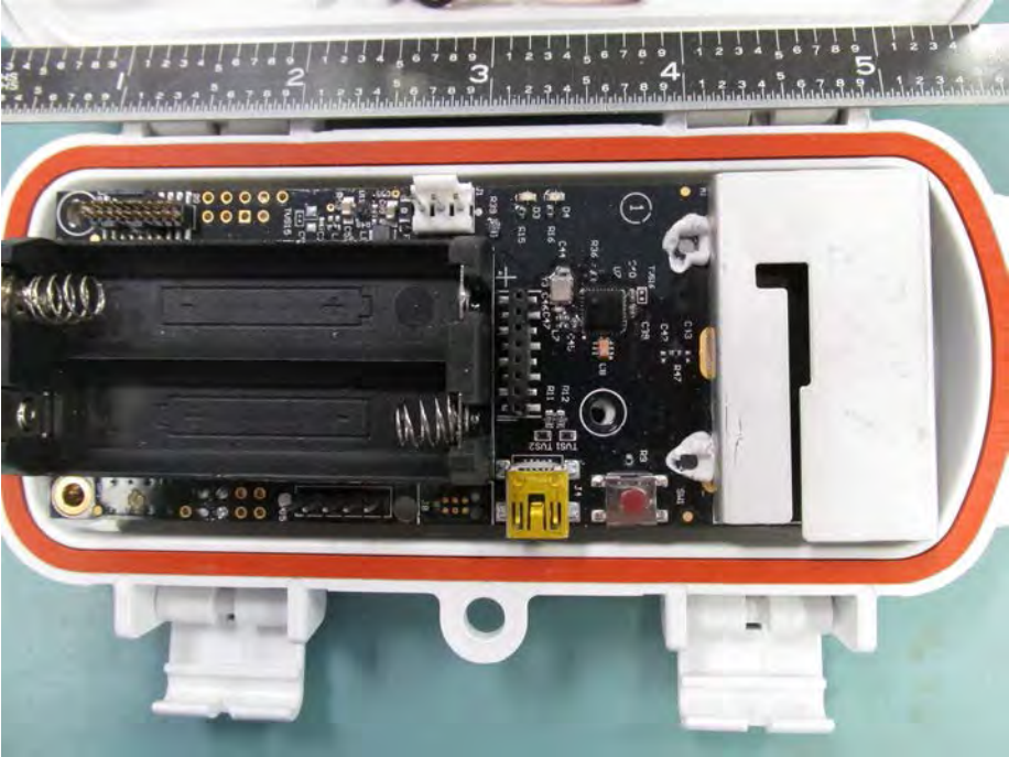
RXW-LIB-900 PCB Front
