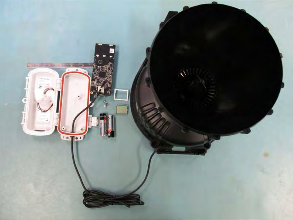
RXW-RGE-900 Exploded View with Sensor
