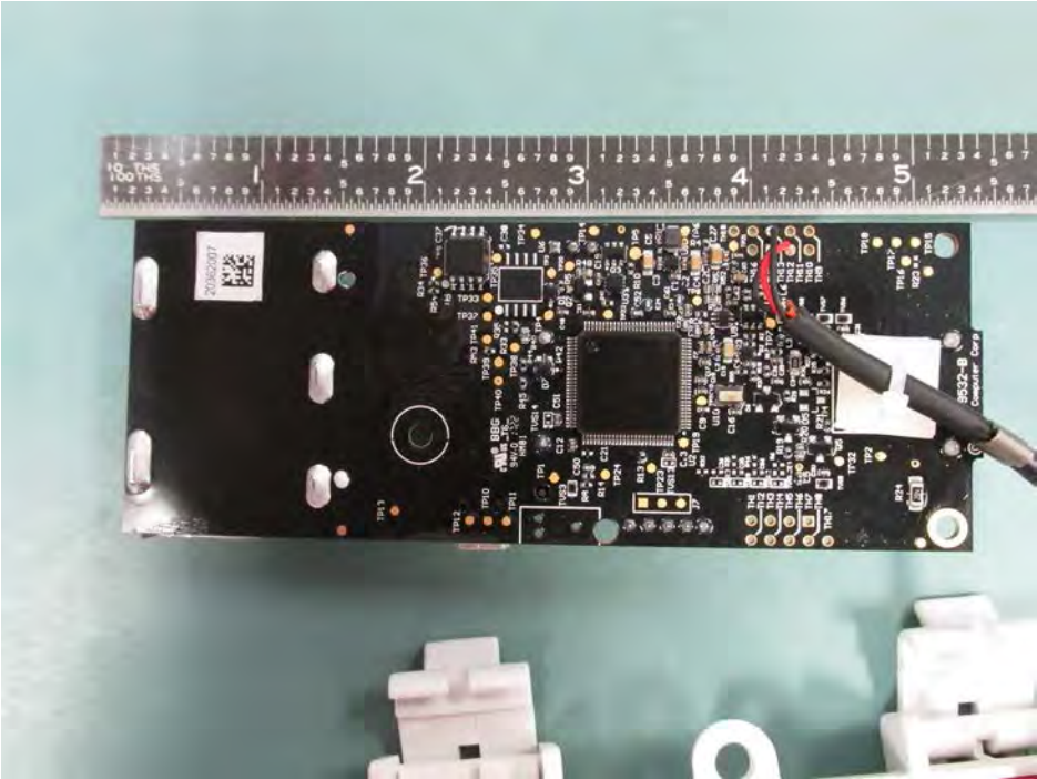
RXW-RGF-900 PCB Back
