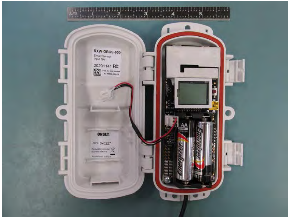
RXW-OBUS-900 Housing Open
