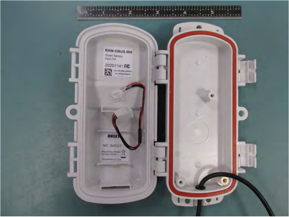
RXW-OBUS-900 Inner Housing
