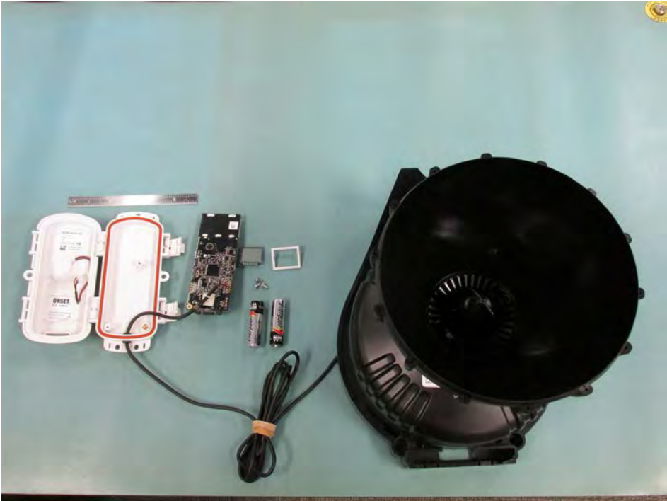
RXW-RGF-900 Exploded View with Sensor
