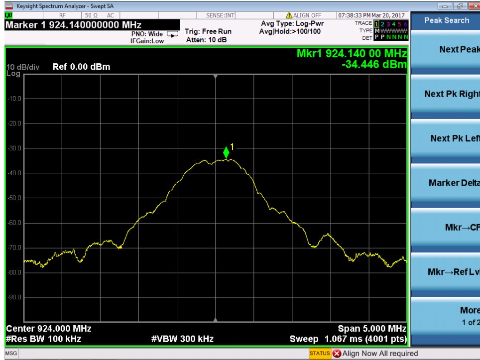
High Channel - Conducted Spurious Reference
