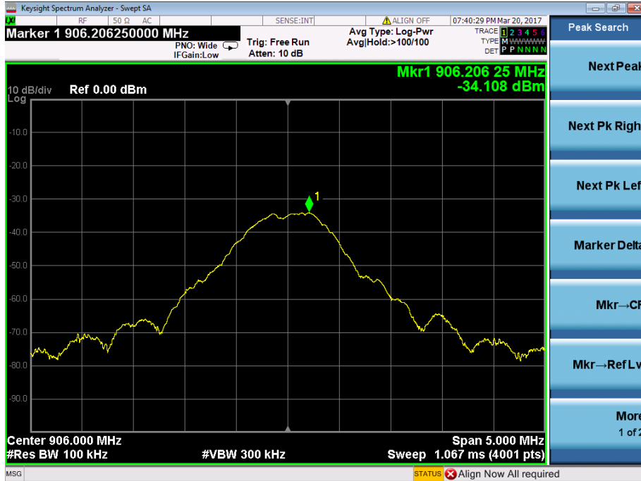
Low Channel - Conducted Spurious Reference
