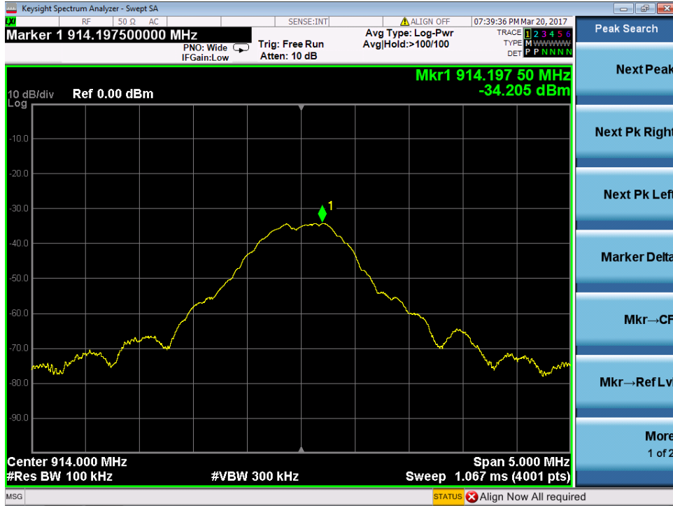
Middle Channel - Conducted Spurious Reference
