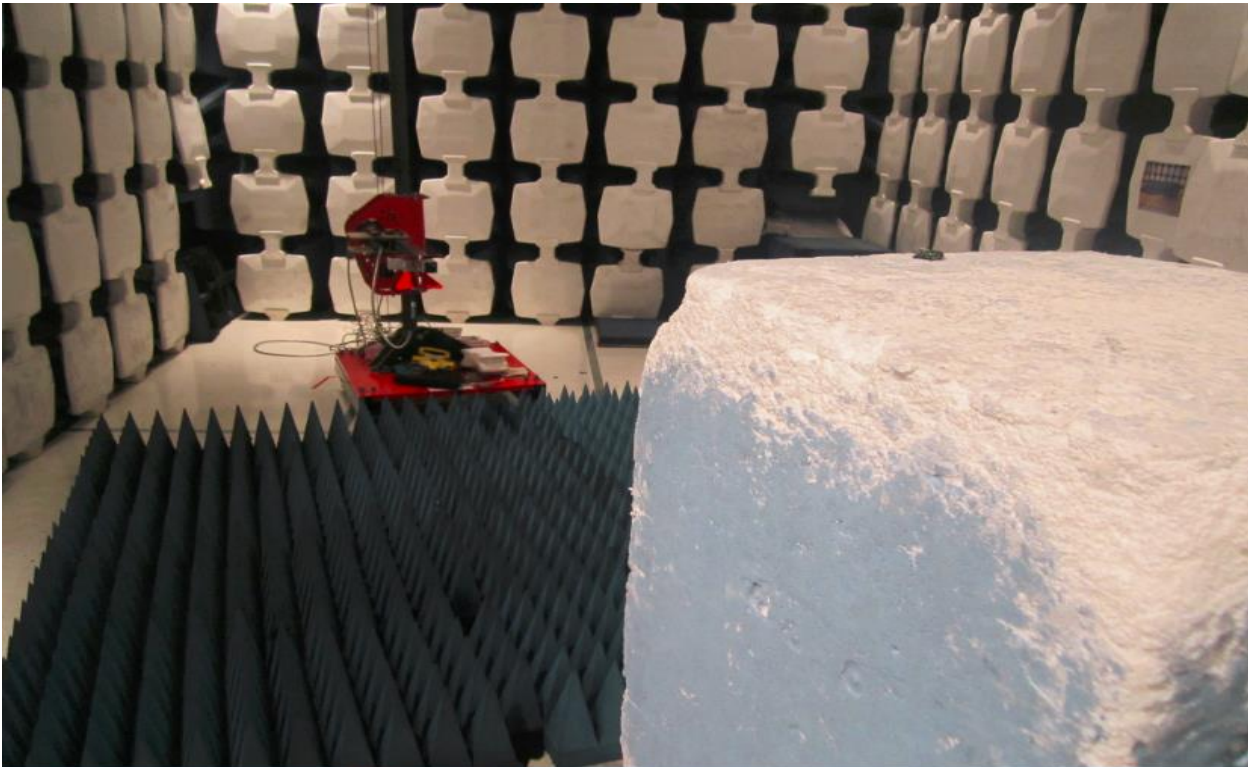
1-6GHz
