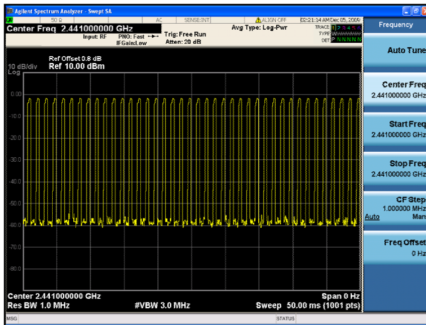
Channel 39 (2441MHz)-(3DH1)
