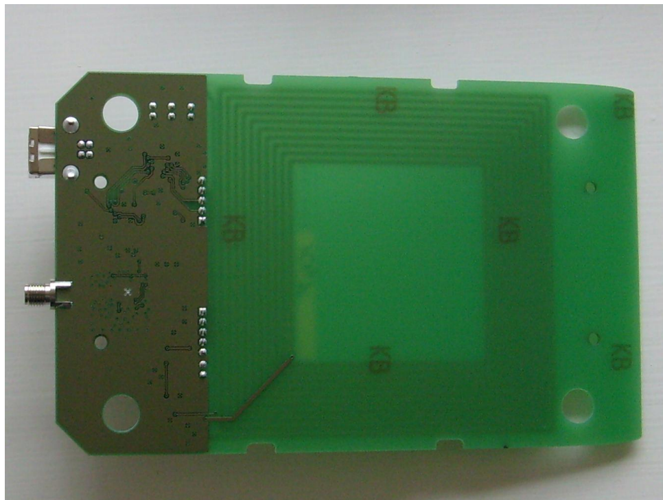
Internal Photograph of IceReader (Bottom Side)
