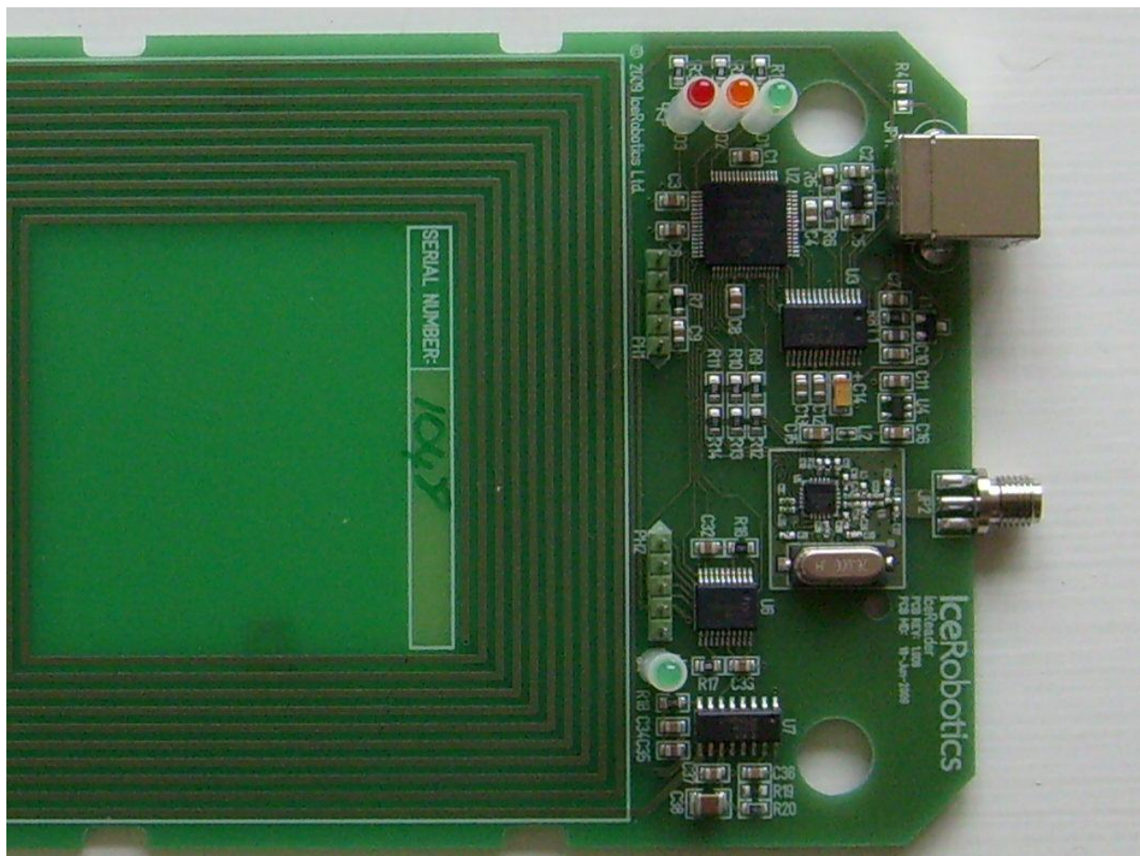
Internal Photograph of IceReader (Top Side Close Up)
