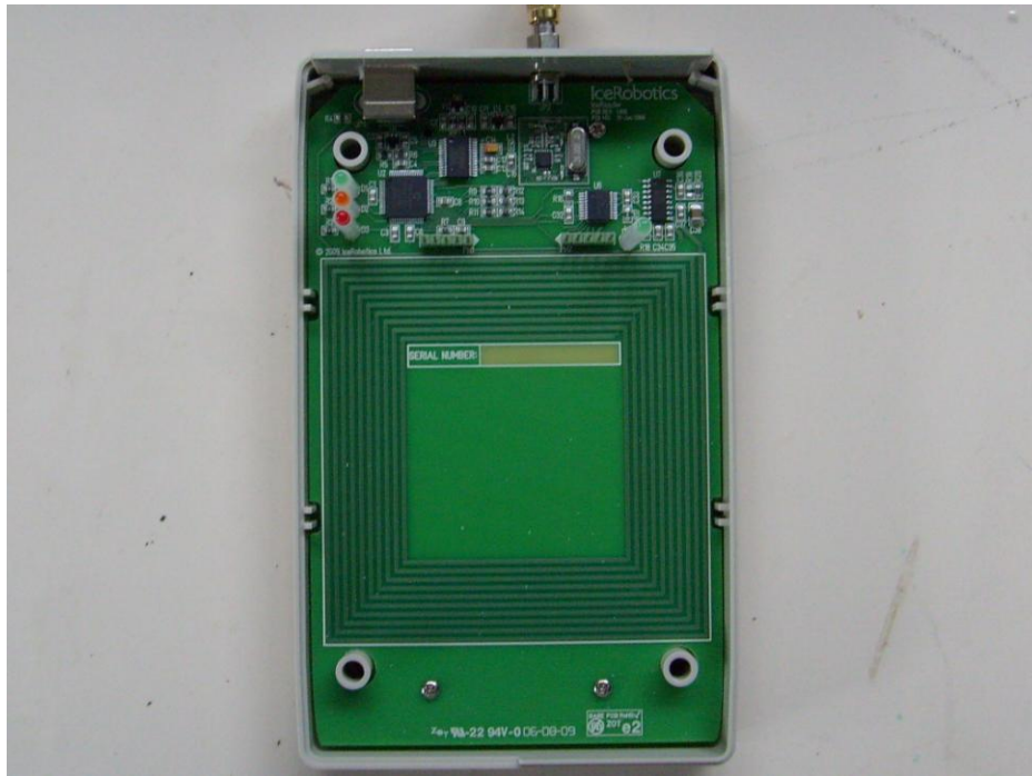
Internal Photograph of IceReader
