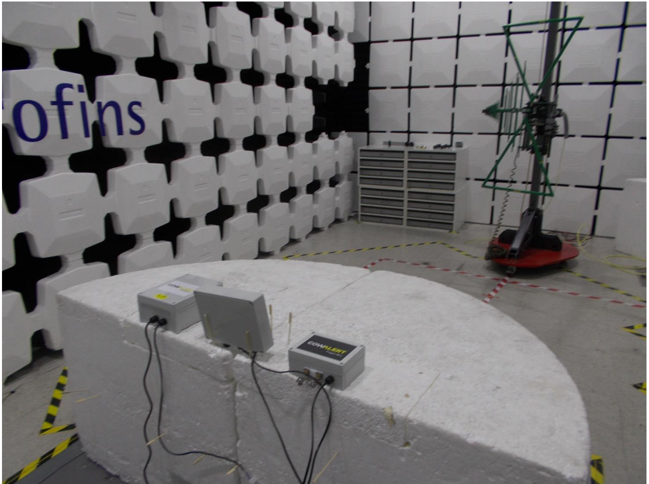
Radiated electric field emissions 30MHz to 1GHz with small antenna
