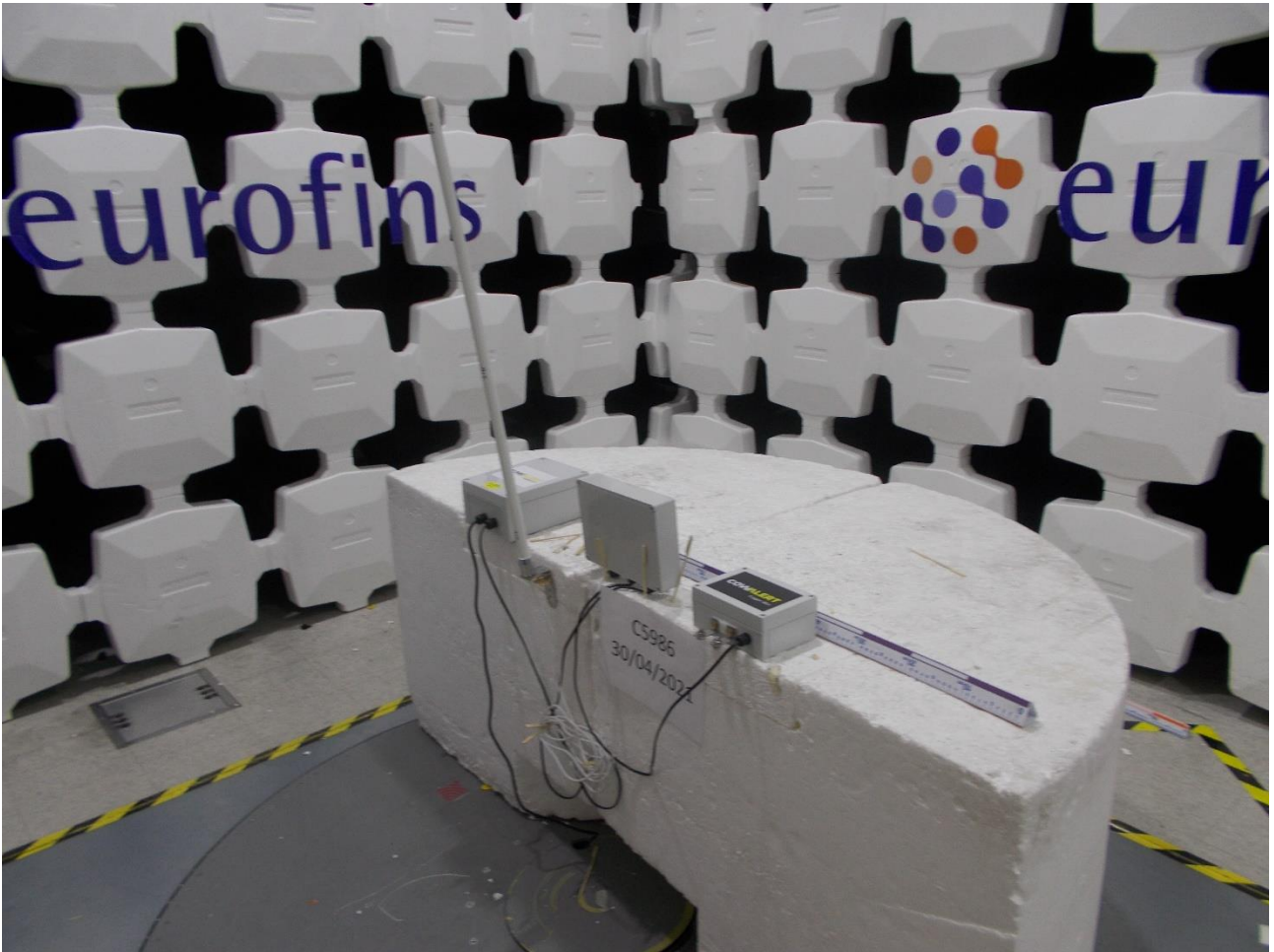
Radiated emissions with large antenna 30MHz to 1GHz
