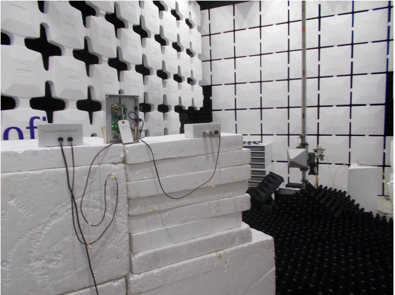
Radiated emissions >1GHz with small antenna
