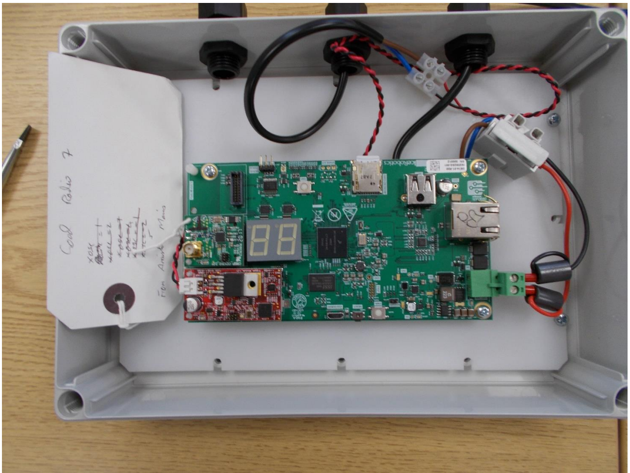
Internal component side
