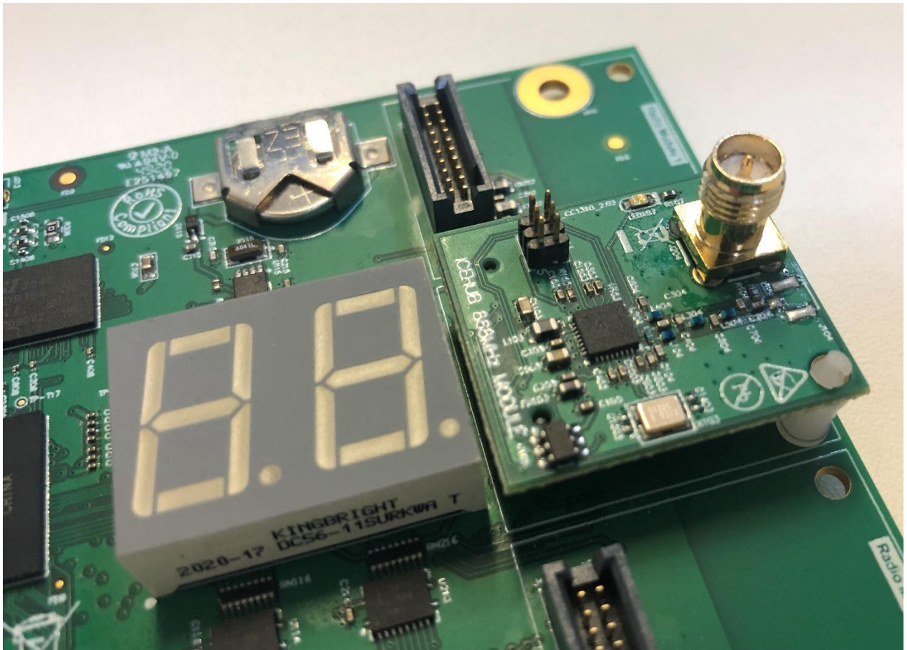
Module board showing antenna connector
