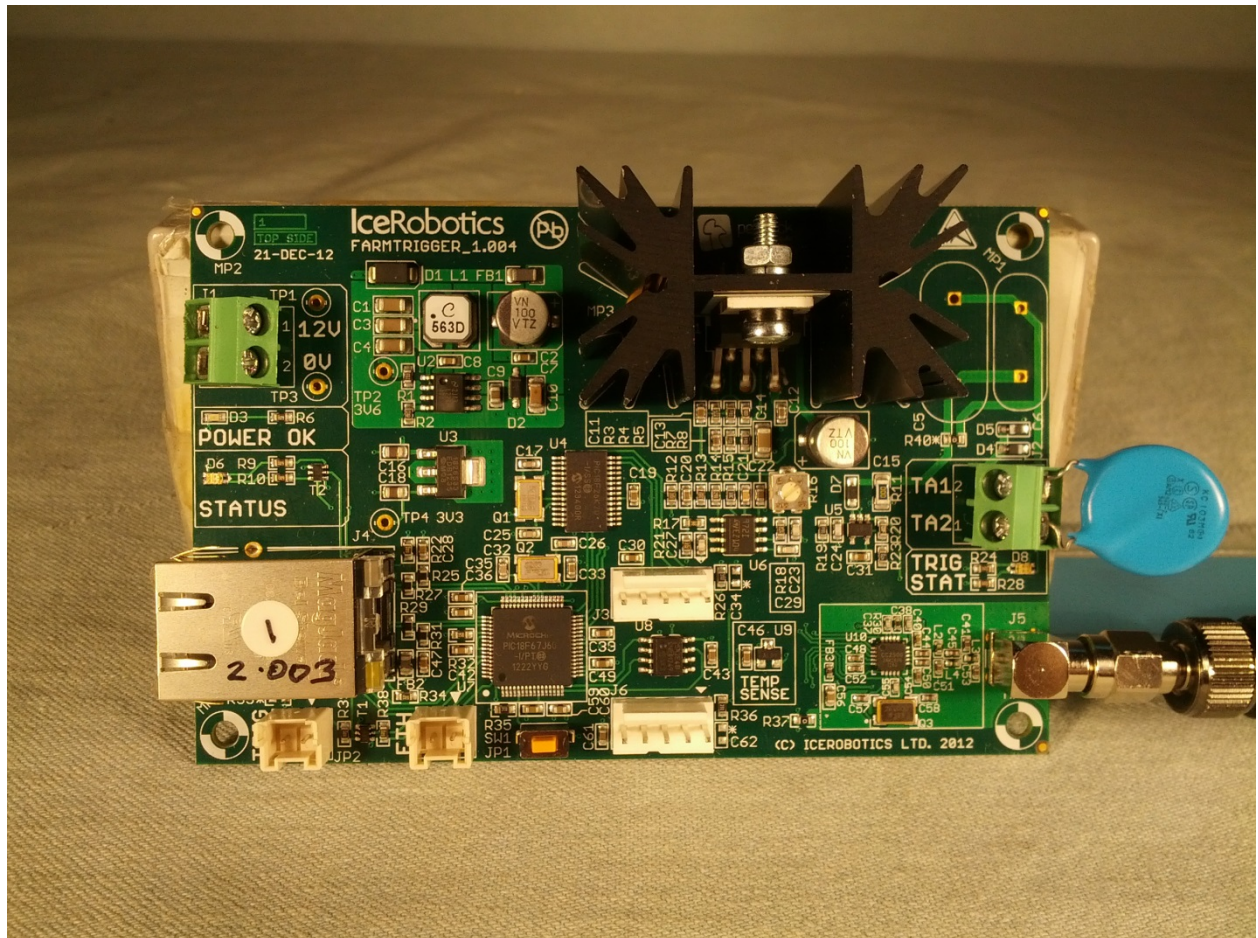
Front View of EtherReader PCB
