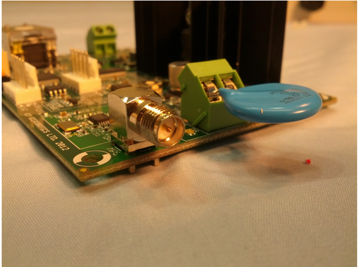
View of the Antenna Connector
