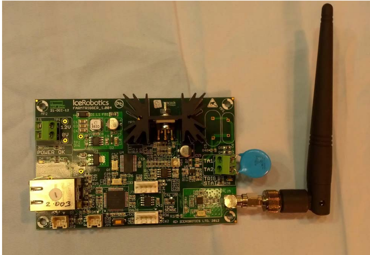
Front View of EtherReader PCB with antenna
