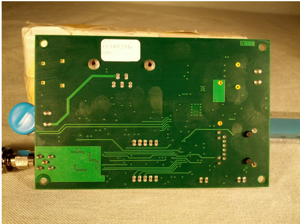
Rear View of EtherReader PCB
