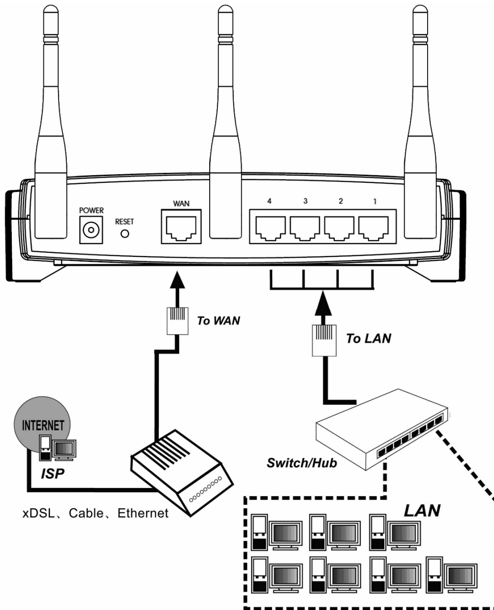
Figure 2-1 Hardware Installation of the MR0-WR941ND Wireless N Router
