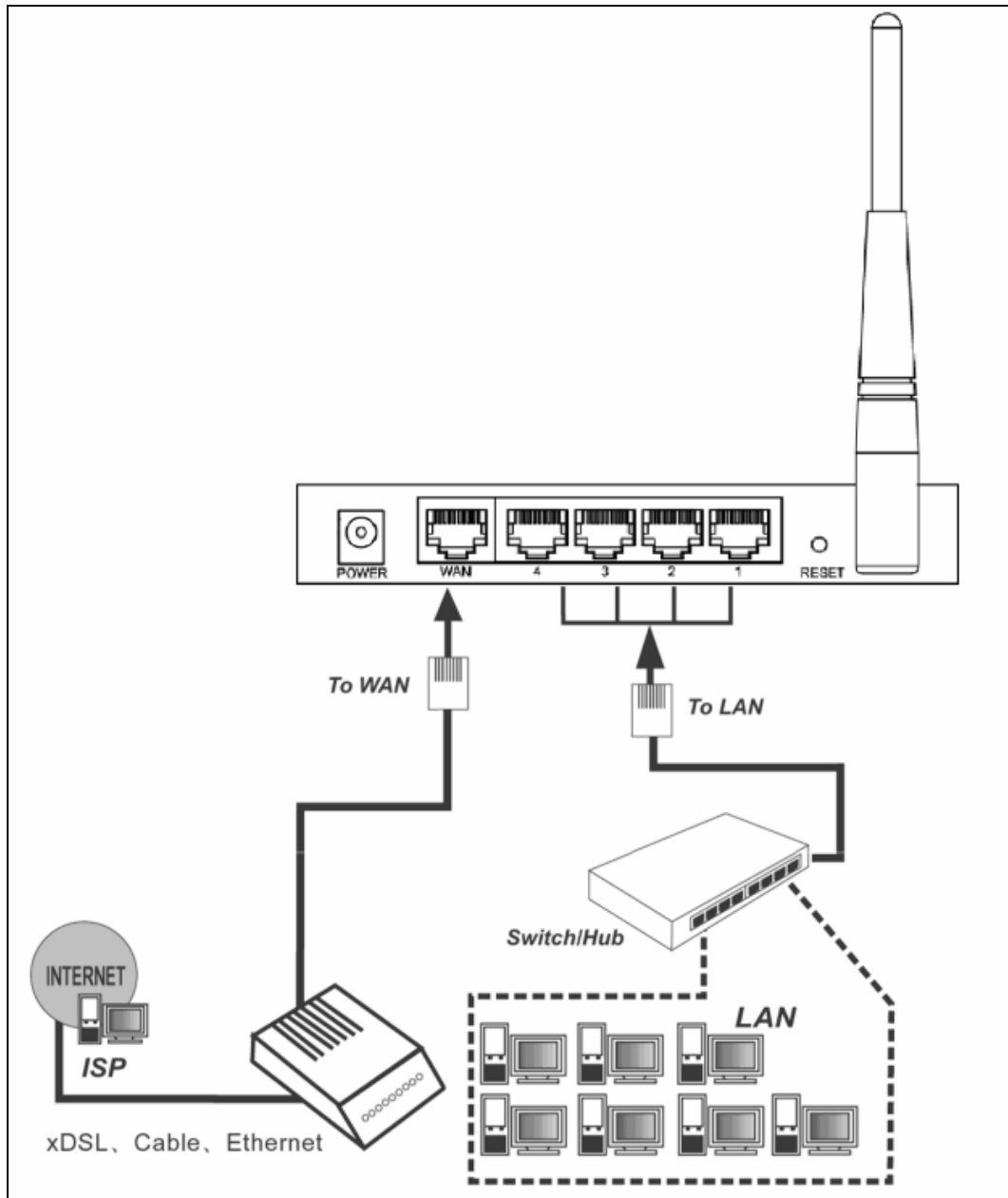
Figure 2-1 Hardware Installation of the M-WR741N/M-WR741ND 150Mbps Wireless Lite-N Router
