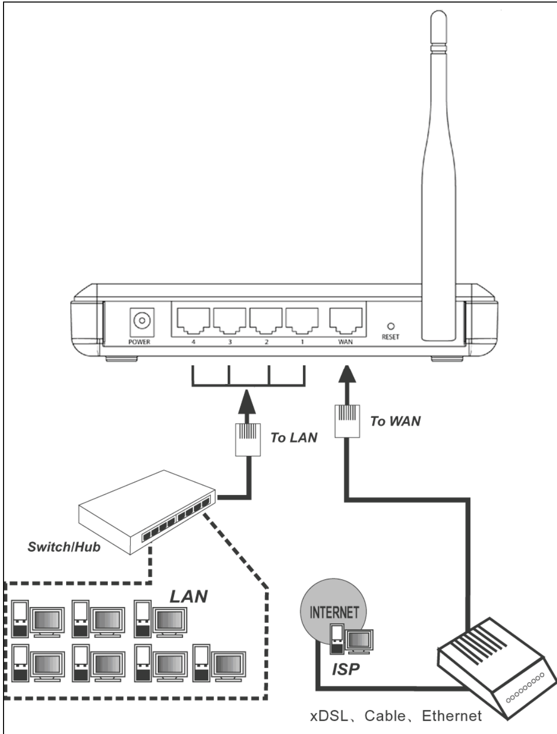
Figure 2-1 Hardware Installation of the MR5-WR542G 54Mbps Wireless Router
