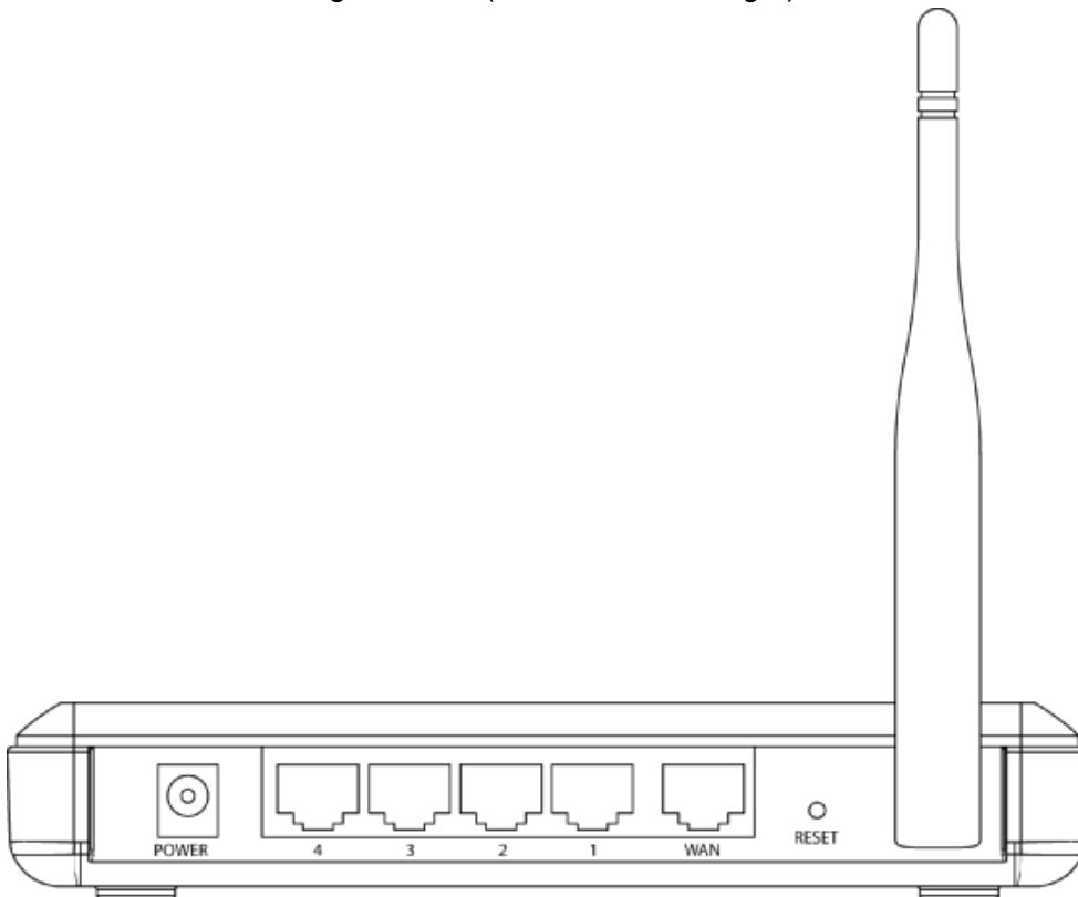
Figure 1-2 Rear Panel sketch
