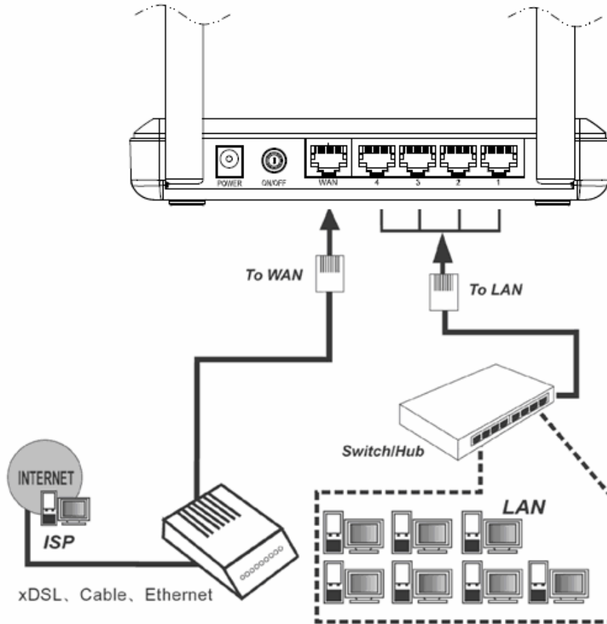
Figure 2-1 Hardware Installation of the PW-RN501D 300Mbps Wireless N Router
