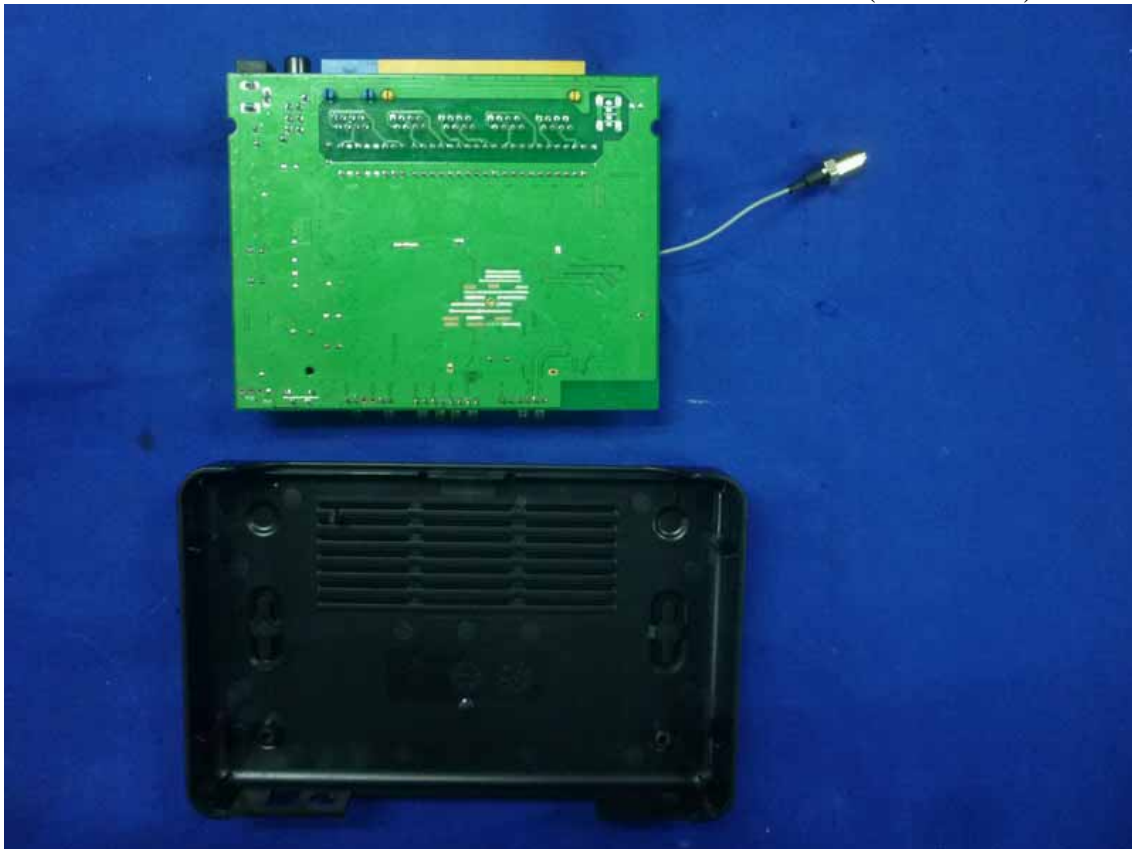
Figure 10 (4PM Flash)Inside of the EUT
