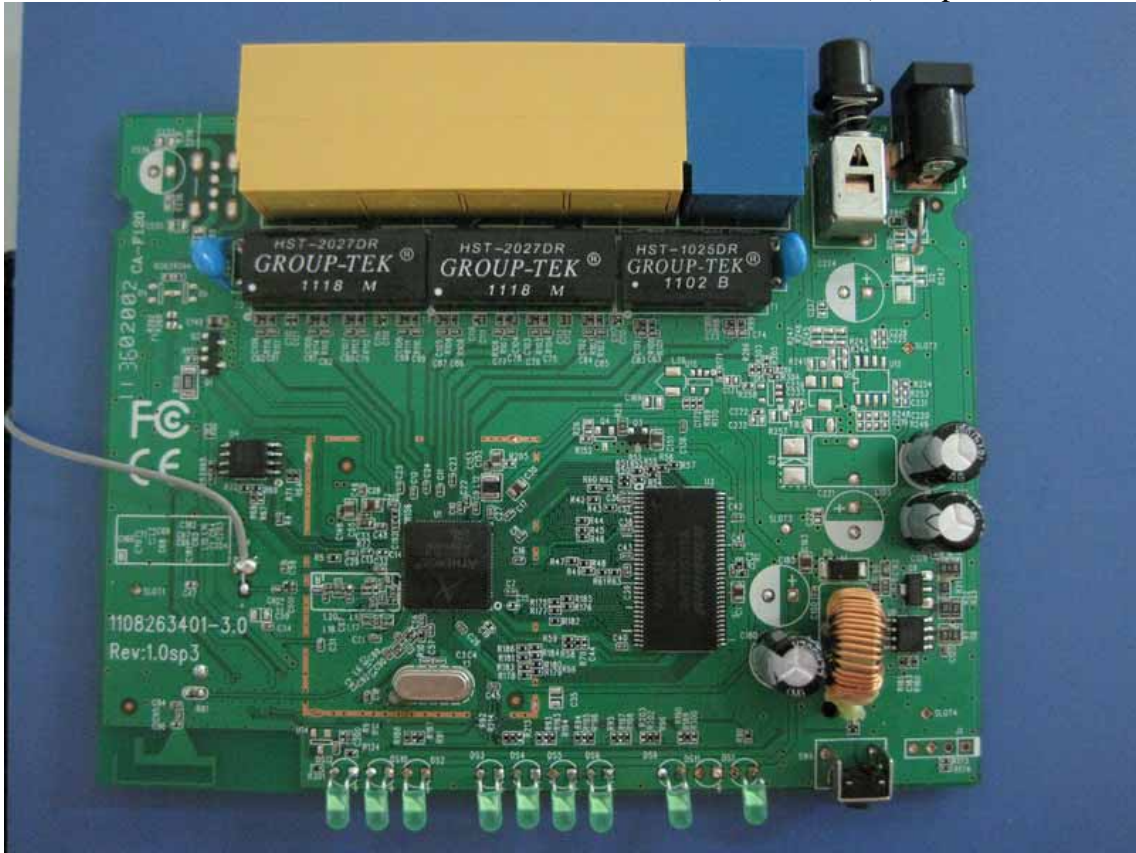
(4PM Flash)Components Side of the PCB
