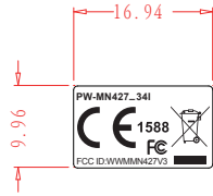
效果图 16.94*9.96mm,0.5R,公差±0.2mm
