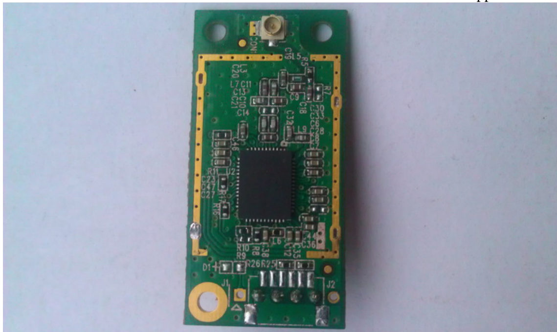
Figure 10 General Appearance of the EUT
