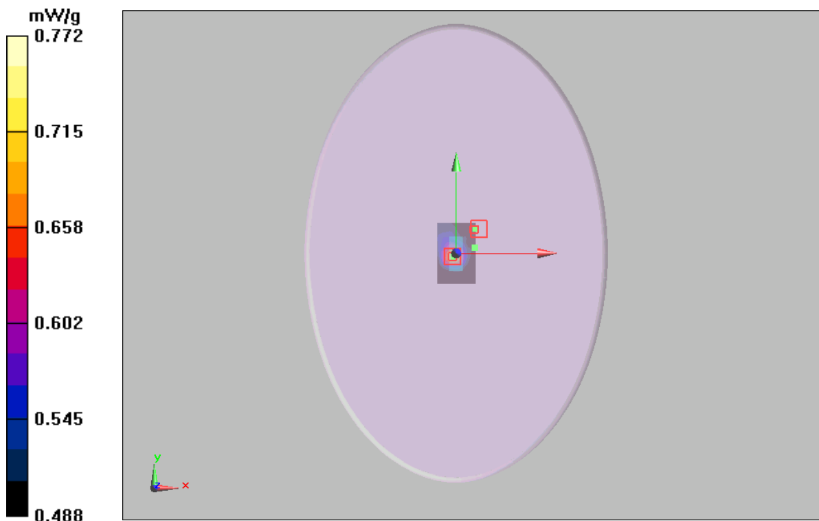
Figure 8 802.11b with IBM T61 Test Position 1 Channel 6
