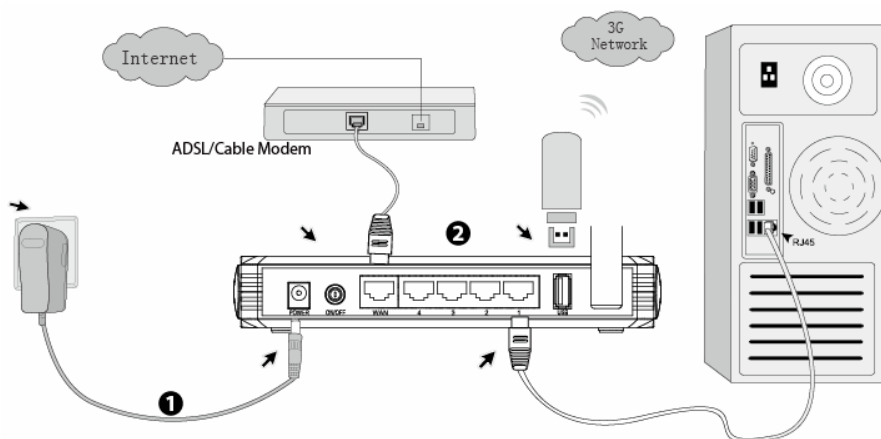
Figure 2-1 Hardware Installation of the PW-3G401/PW-3G401D 3G Wireless N Router
