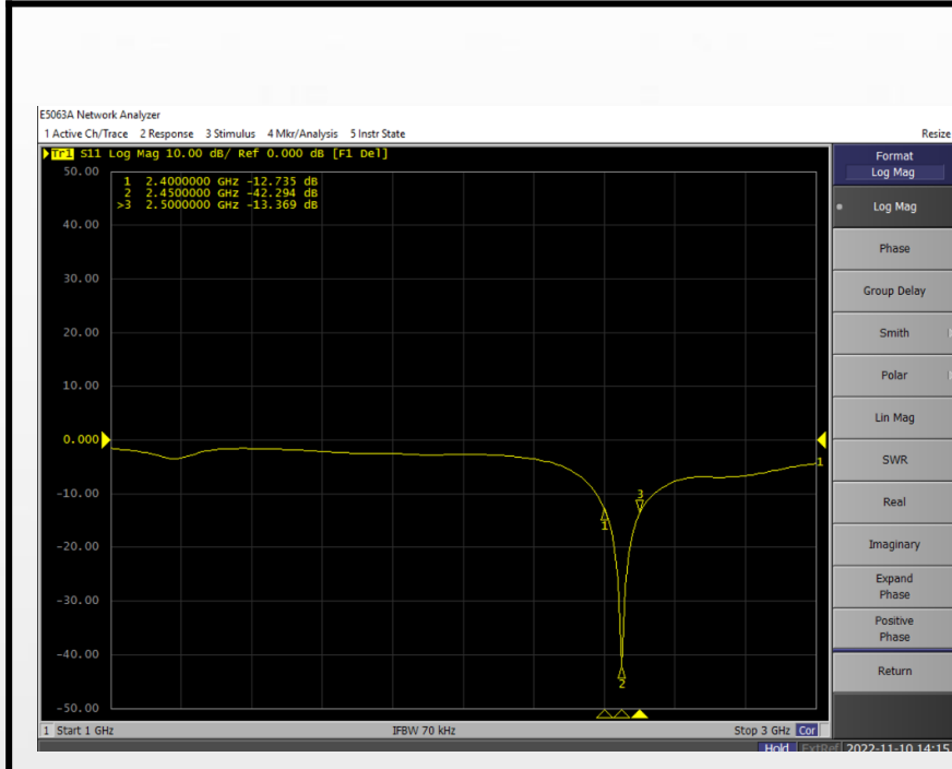
Return loss
