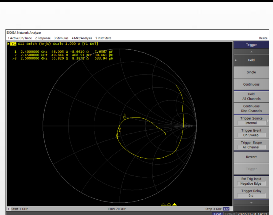
Smith-Chart
