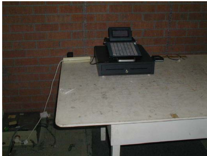
Conducted Disturbance Test Setup (Photo 1)
