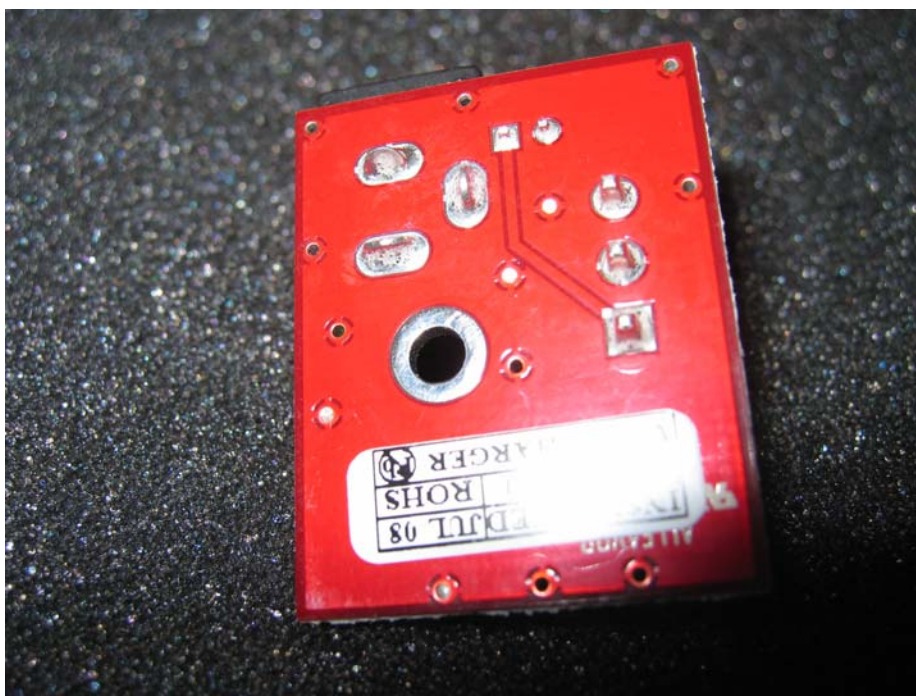
Mains Interface PCB (VX02) (Bottom View)
