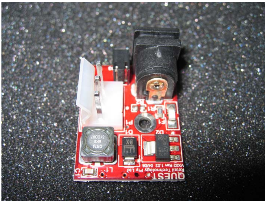
Mains Interface PCB (VX02) (Top View)
