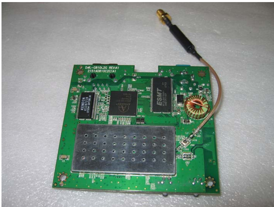
DWL-G810 Wireless Bridge PCB (Bottom View)
