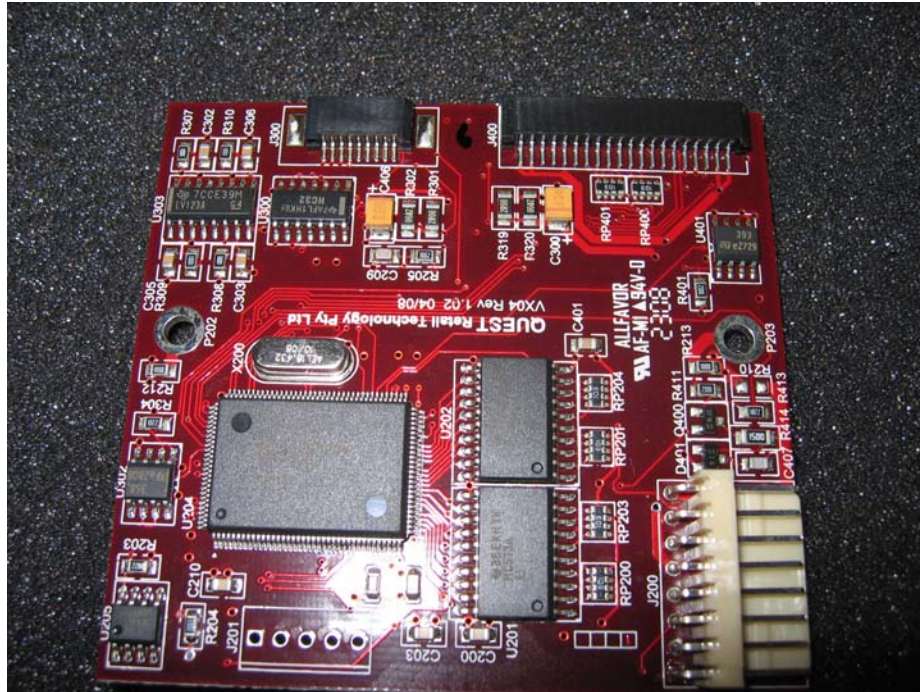
Printer Controller PCB (VX04) (Top View)
