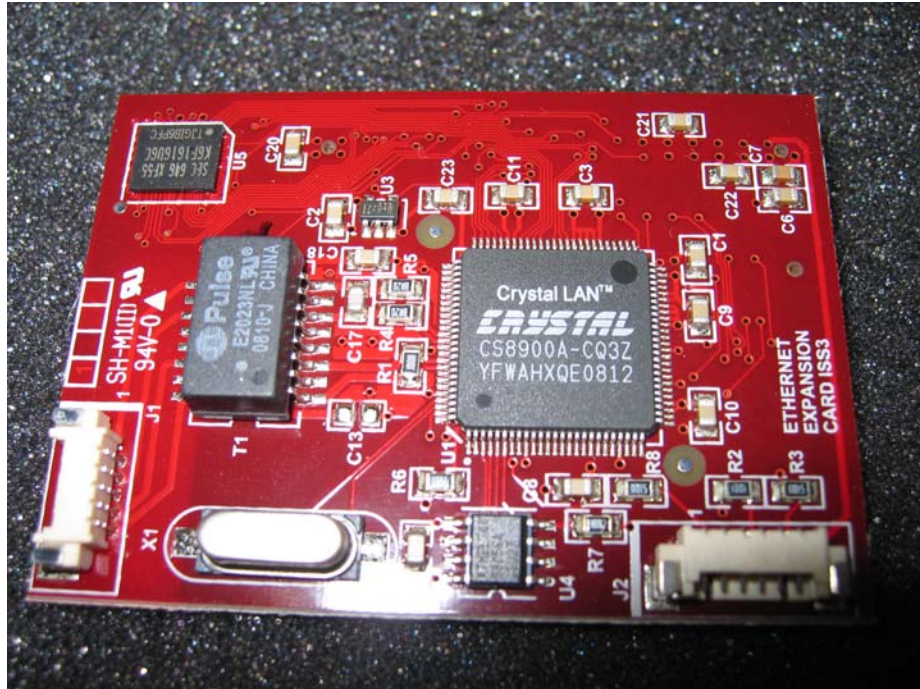
Ethernet Expansion Card (Top View)
