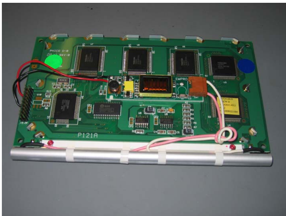
Main User Display PCB (Bottom View)
