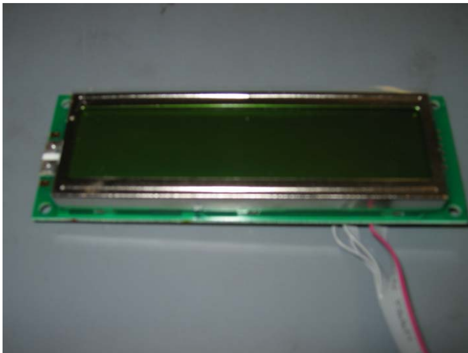
Customer Display PCB (Top View)
