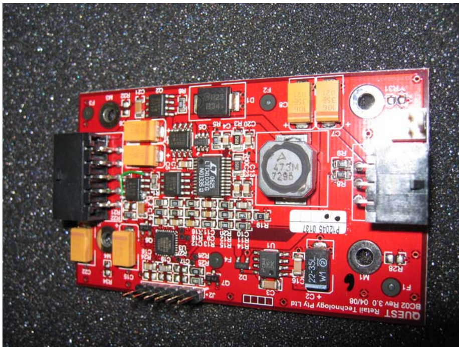
Battery Charger PCB (BC02) (Top View)
