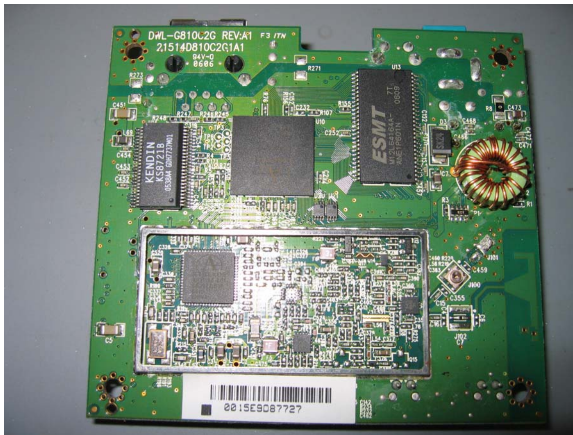
DWL-G810 Wireless Bridge PCB (Bottom View – Shield Removed)
