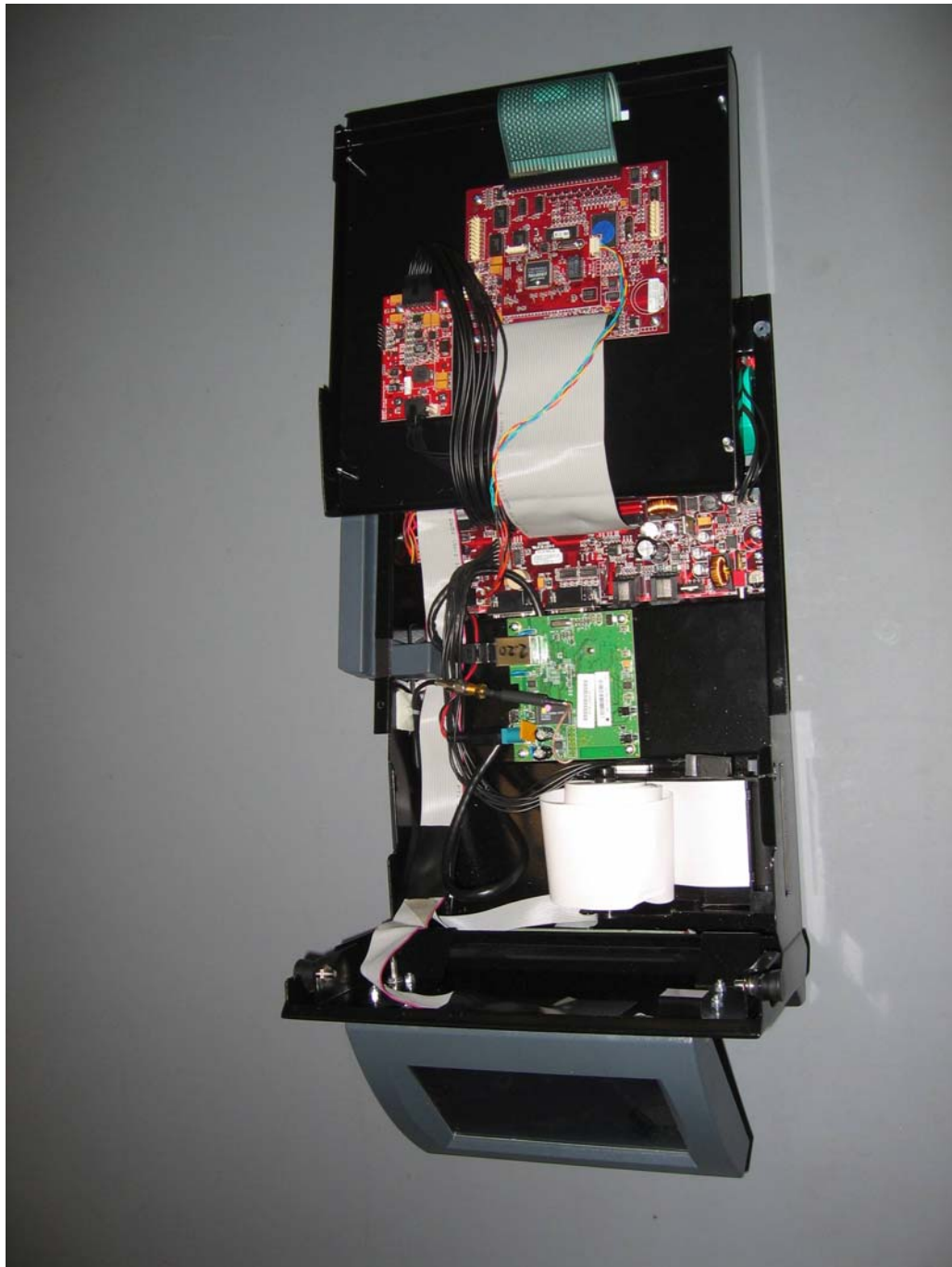
EUT Opened
