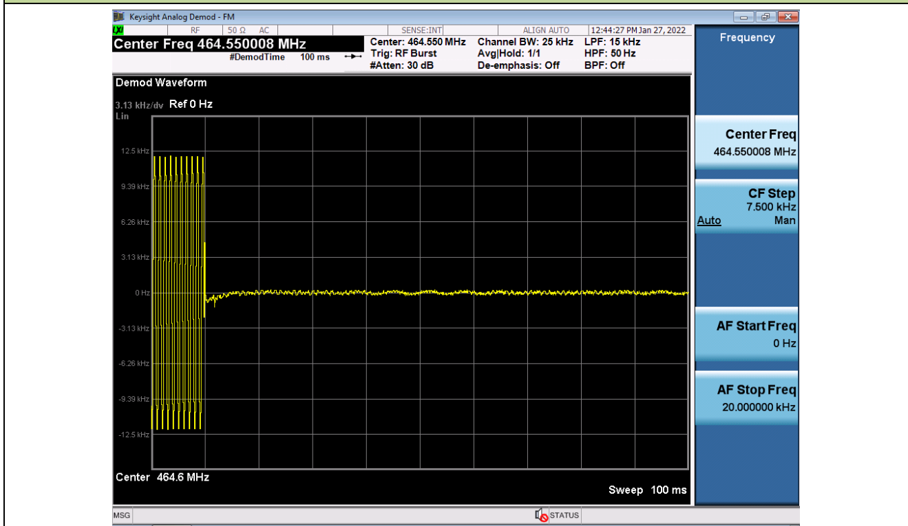
Transmitter Frequency Behavior – on to off
