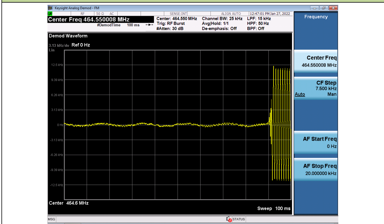
Transmitter Frequency Behavior – on to off
